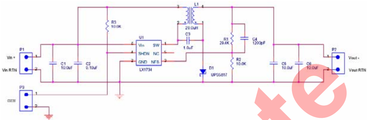
Application Circuit #1
