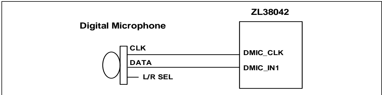
Figure 32 - Single Mono Digital Microphone Interface
