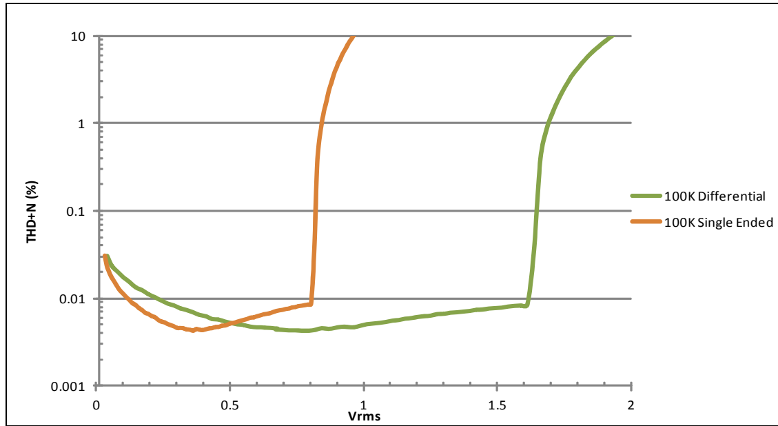
Figure 15 - THD+N Ratio versus V_{RMS} – Driving High Impedance
