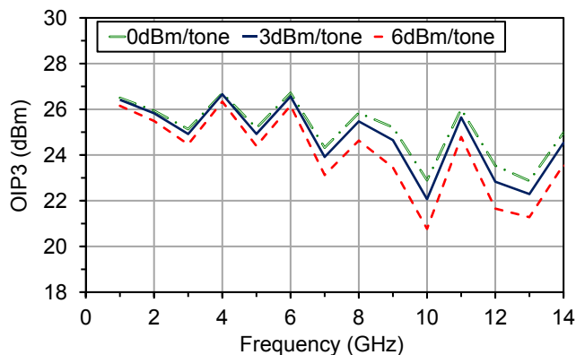
Output IP3
