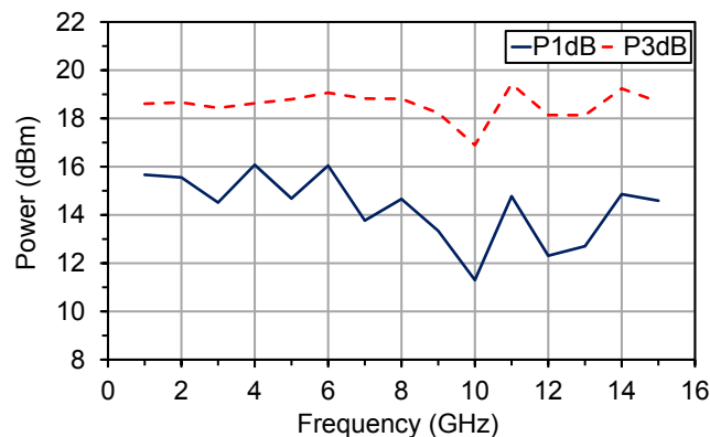
Output Power
