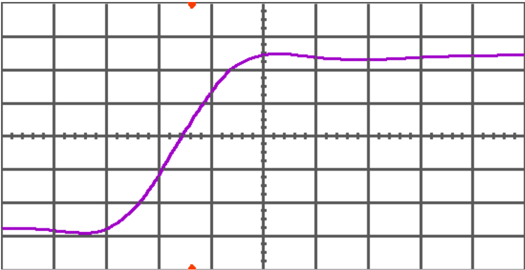
Figure 12(b) DUT 5411 post-annealing rising edge, abscissa scale is 1 V/div and ordinate scale is 0.5 ns/div.
