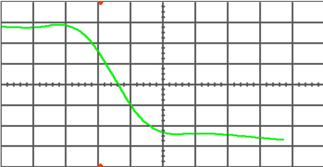
Figure 17(a) DUT 5400 pre-irradiation falling edge, abscissa scale is 1 V/div and ordinate scale is 0.5 ns/div.
