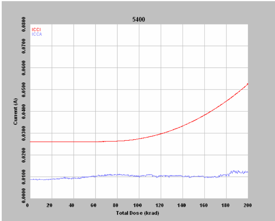
Figure 6 DUT 5400 in-flux I_{CCA} and I_{CCI}
