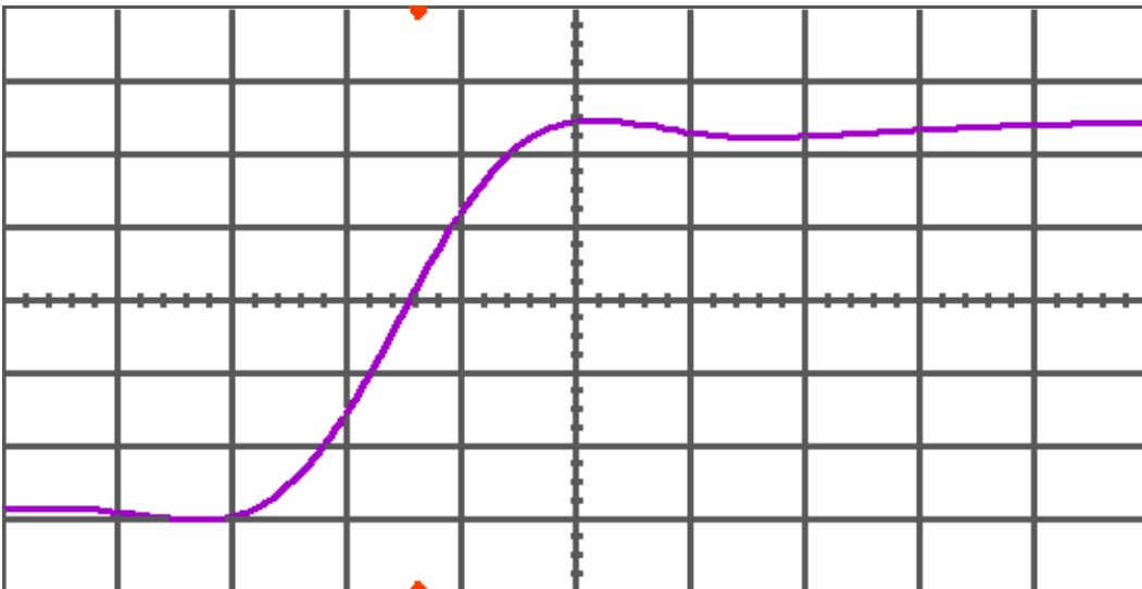
Figure 9(b) DUT 5320 post-annealing rising edge, abscissa scale is 1 V/div and ordinate scale is 0.5 ns/div.
