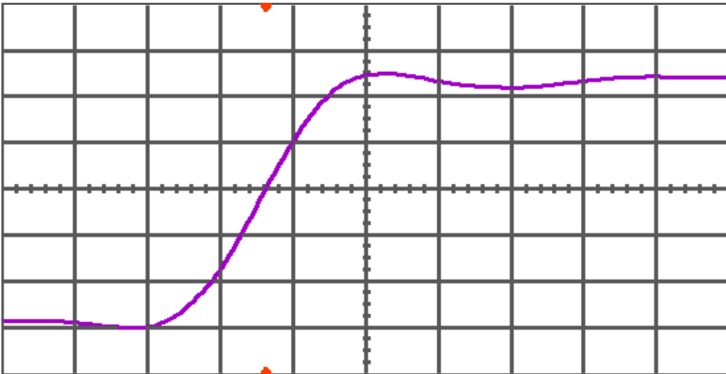
Figure 10(b) DUT 5377 post-annealing rising edge, abscissa scale is 1 V/div and ordinate scale is 0.5 ns/div.
