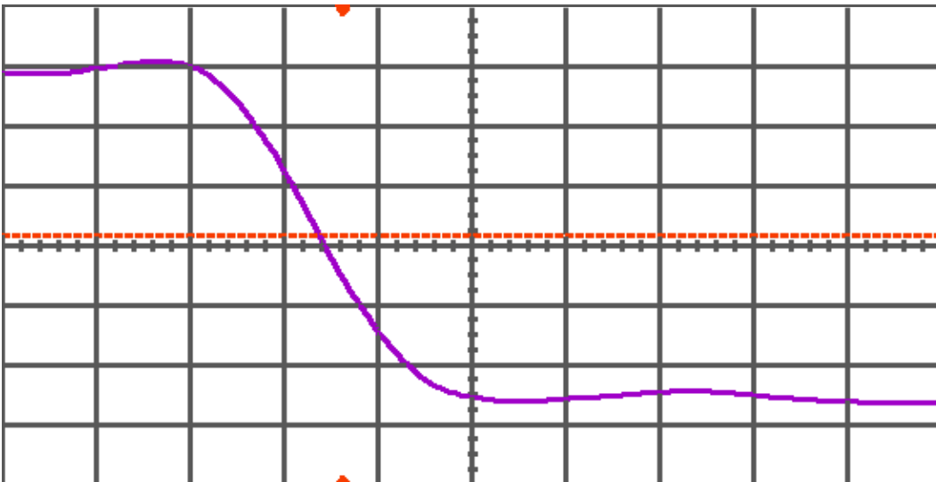
Figure 15(b) DUT 5320 post-annealing falling edge, abscissa scale is 1 V/div and ordinate scale is 0.5 ns/div.
