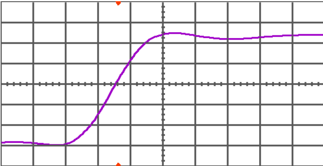
Figure 8(b) DUT 5306 post-annealing rising edge, abscissa scale is 1 V/div and ordinate scale is 0.5 ns/div.
