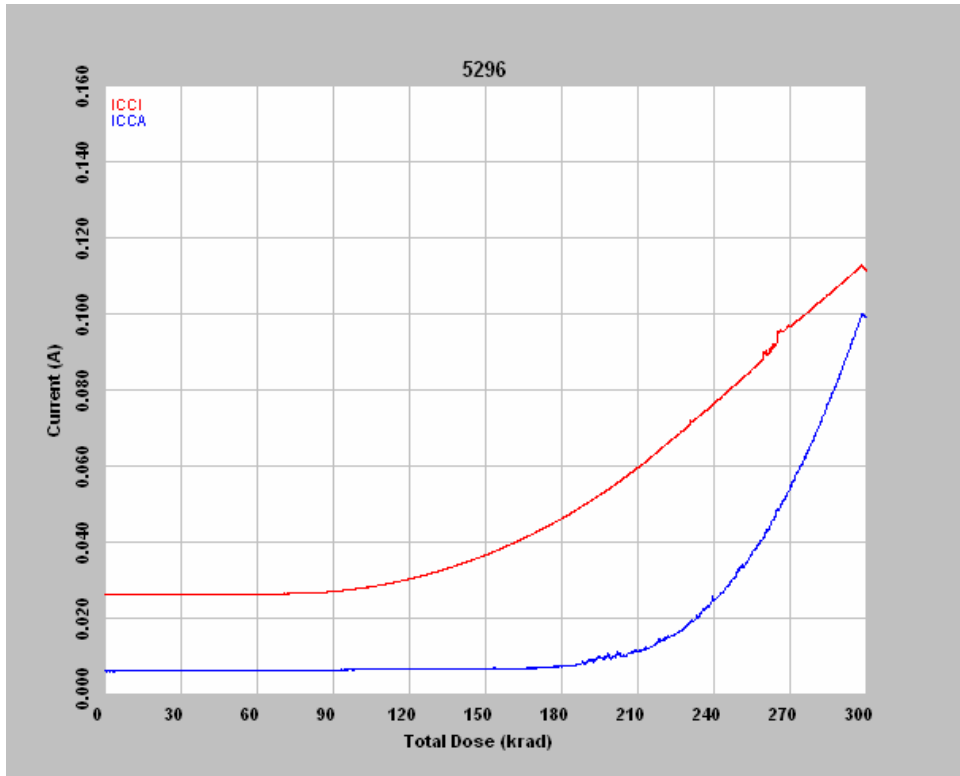
Figure 2 DUT 5296 in-flux I_{CCA} and I_{CCI}
