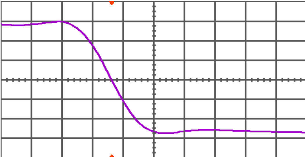
Figure 17(b) DUT 5400 post-annealing falling edge, abscissa scale is 1 V/div and ordinate scale is 0.5 ns/div.
