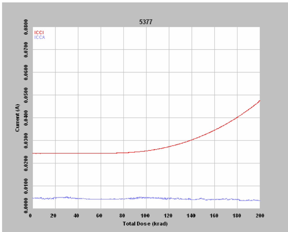
Figure 5 DUT 5377 in-flux I_{CCA} and I_{CCI}
