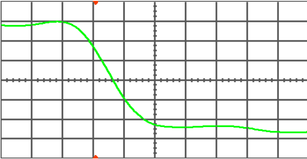
Figure 13(a) DUT 5296 pre-irradiation falling edge, abscissa scale is 1 V/div and ordinate scale is 0.5 ns/div.
