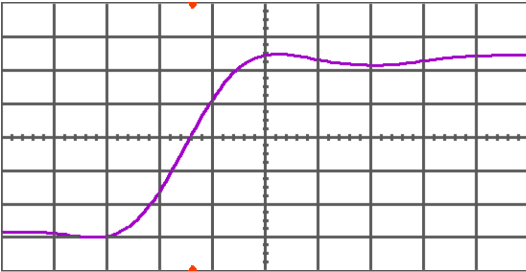
Figure 11(b) DUT 5400 post-annealing rising edge, abscissa scale is 1 V/div and ordinate scale is 0.5 ns/div.
