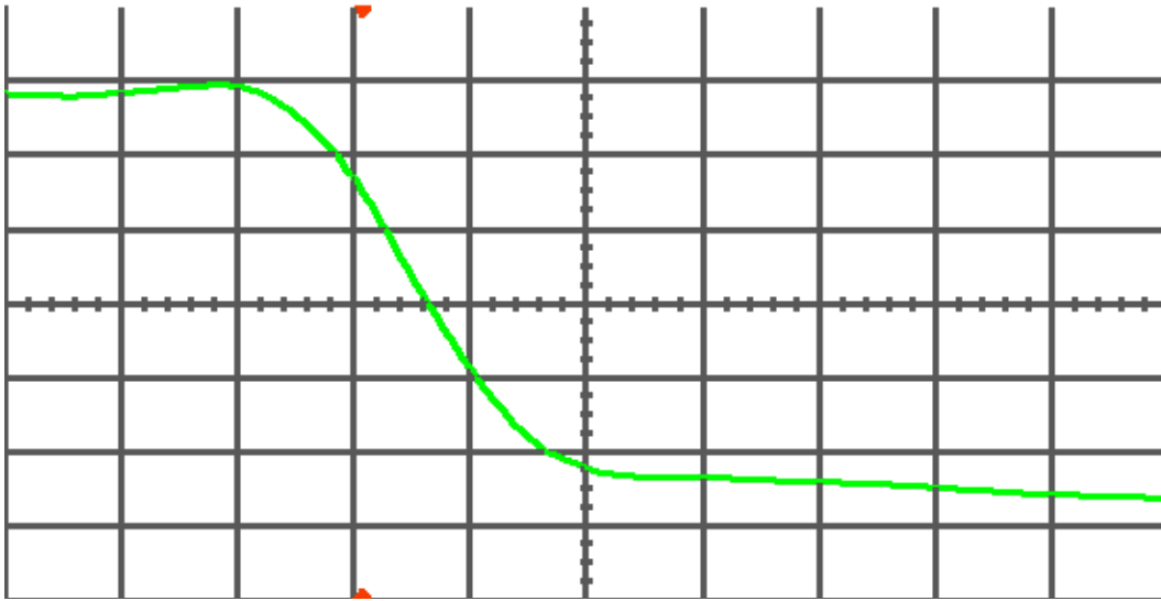
Figure 18(a) DUT 5411 pre-irradiation falling edge, abscissa scale is 1 V/div and ordinate scale is 0.5 ns/div.
