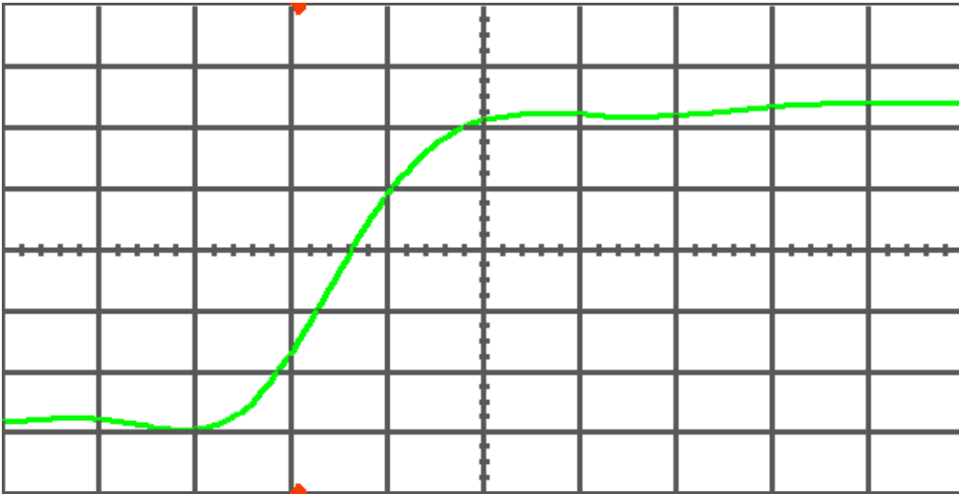
Figure 9(a) DUT 5320 pre-radiation rising edge, abscissa scale is 1 V/div and ordinate scale is 0.5 ns/div.
