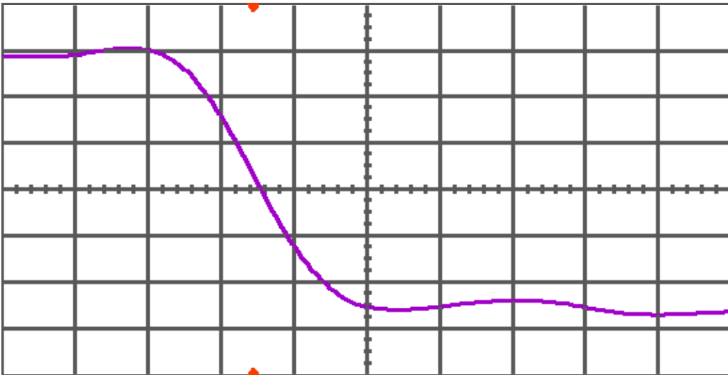
Figure 14(b) DUT 5306 post-annealing falling edge, abscissa scale is 1 V/div and ordinate scale is 0.5 ns/div.
