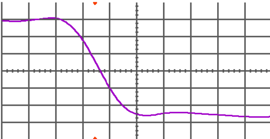
Figure 13(b) DUT 5296 post-annealing falling edge, abscissa scale is 1 V/div and ordinate scale is 0.5 ns/div.
