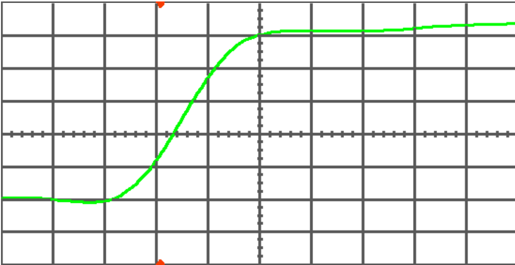
Figure 10(a) DUT 5377 pre-irradiation rising edge, abscissa scale is 1 V/div and ordinate scale is 0.5 ns/div.
