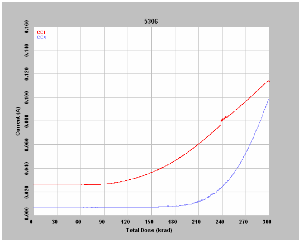
Figure 3 DUT 5306 in-flux I_{CCA} and I_{CCI}
