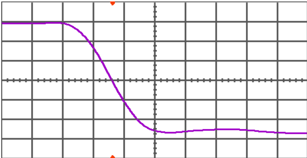
Figure 18(b) DUT 5411 post-annealing falling edge, abscissa scale is 1 V/div and ordinate scale is 0.5 ns/div.
