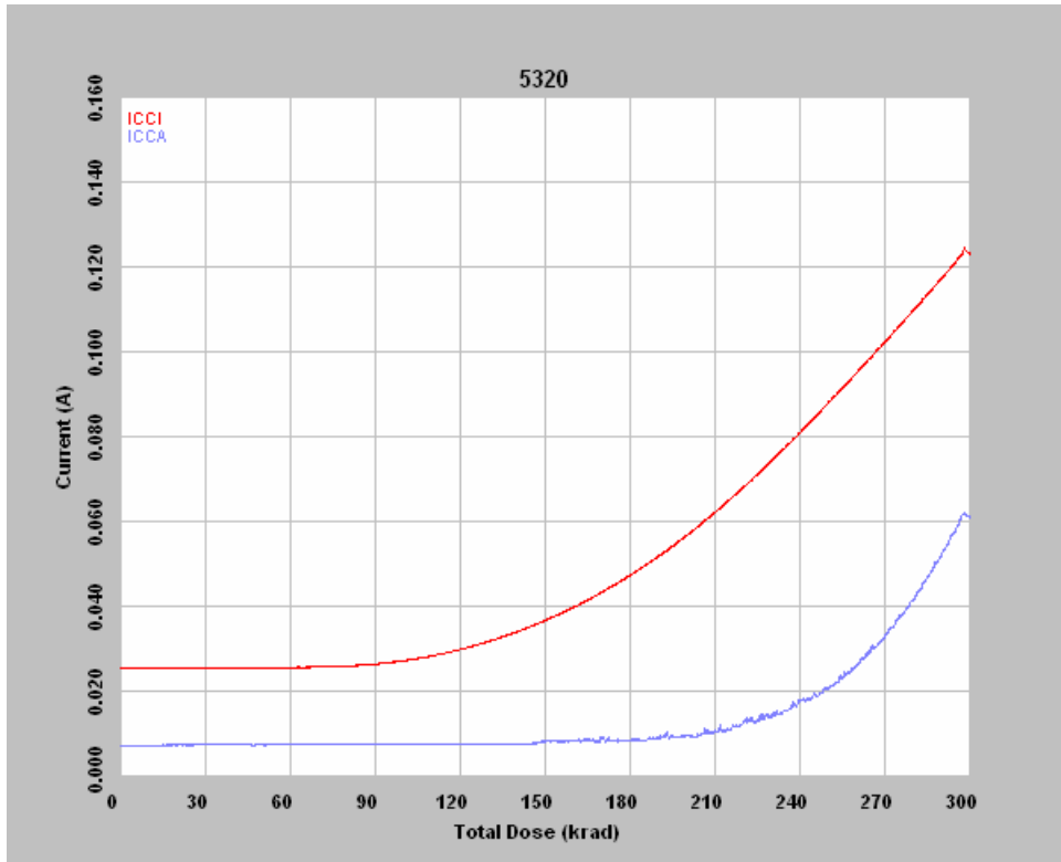
Figure 4 DUT 5320 in-flux I_{CCA} and I_{CCI}
