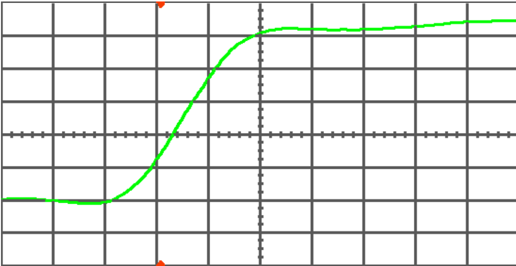
Figure 11(a) DUT 5400 pre-irradiation rising edge, abscissa scale is 1 V/div and ordinate scale is 0.5 ns/div.
