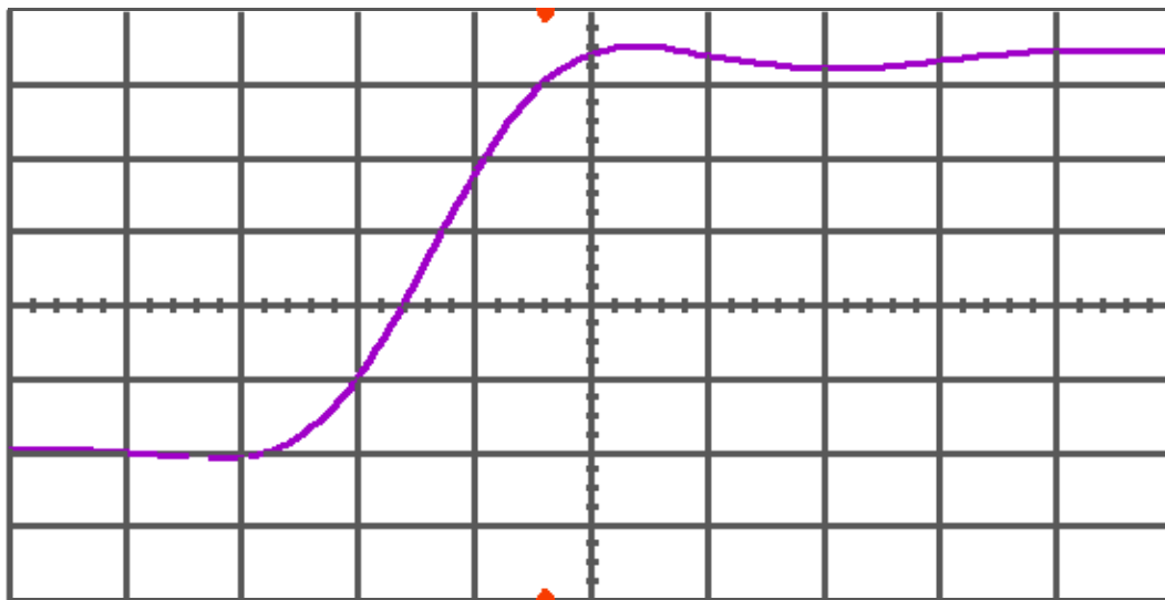
Figure 7(b) DUT 5296 post-annealing rising edge, abscissa scale is 1 V/div and ordinate scale is 0.5 ns/div.
