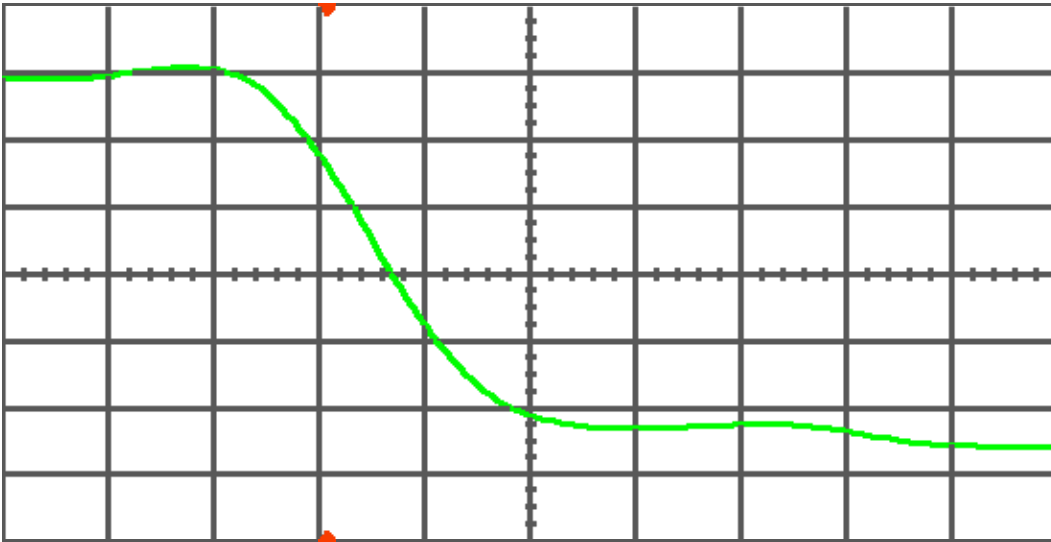
Figure 14(a) DUT 5306 pre-irradiation falling edge, abscissa scale is 1 V/div and ordinate scale is 0.5 ns/div.
