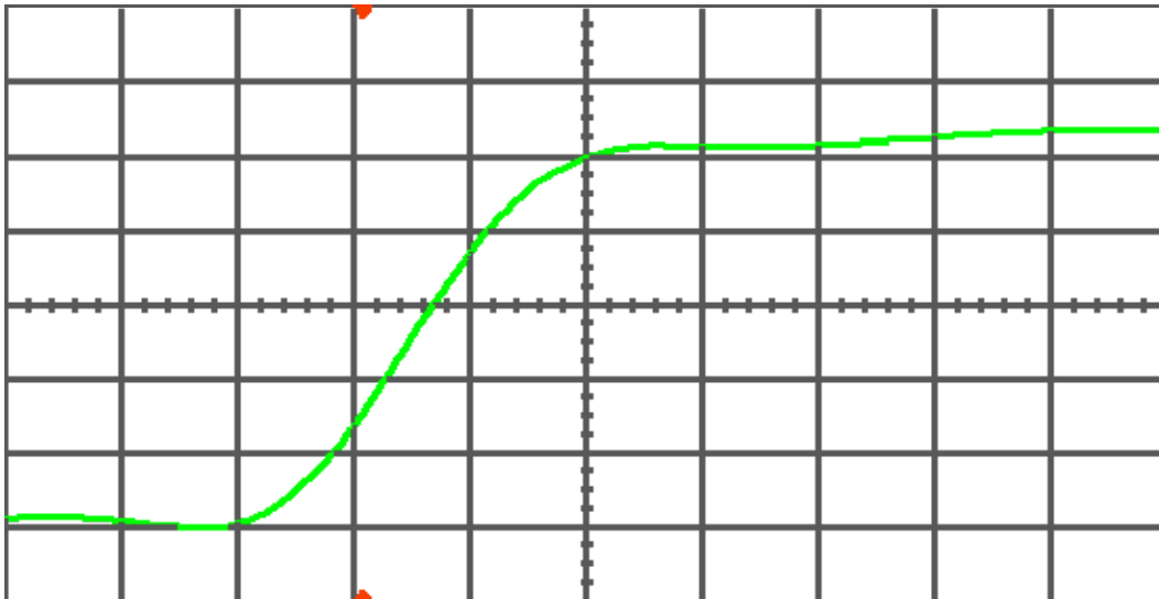
Figure 7(a) DUT 5296 pre-irradiation rising edge, abscissa scale is 1 V/div and ordinate scale is 0.5 ns/div.
