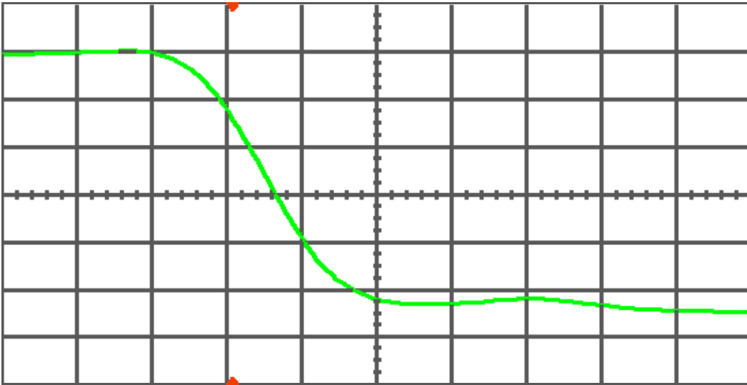
Figure 16(a) DUT 5377 pre-irradiation falling edge, abscissa scale is 1 V/div and ordinate scale is 0.5 ns/div.
