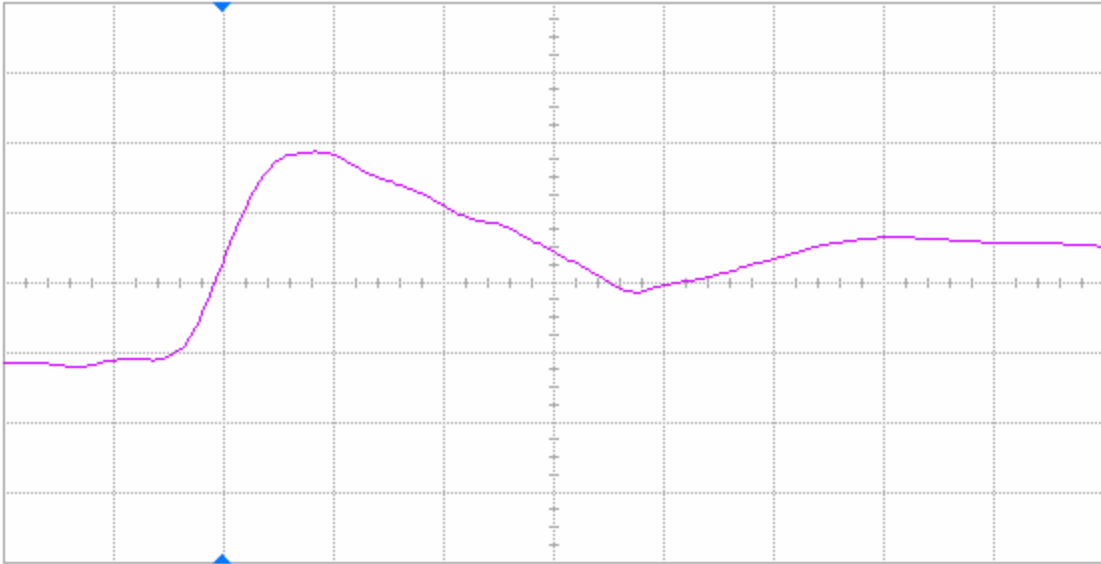
Figure 13(a) DUT 73025 pre-irradiation rising edge, abscissa scale is 2 V/div and ordinate scale is 2 ns/div.
