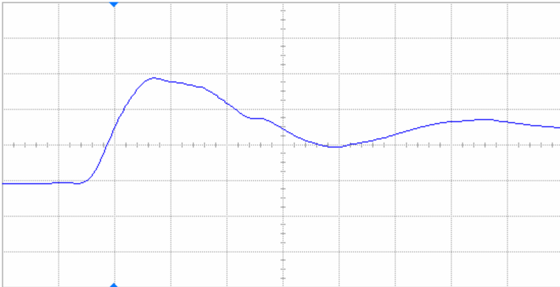
Figure 10(b) DUT 72992 post-annealing rising edge, abscissa scale is 2 V/div and ordinate scale is 2 ns/div.
