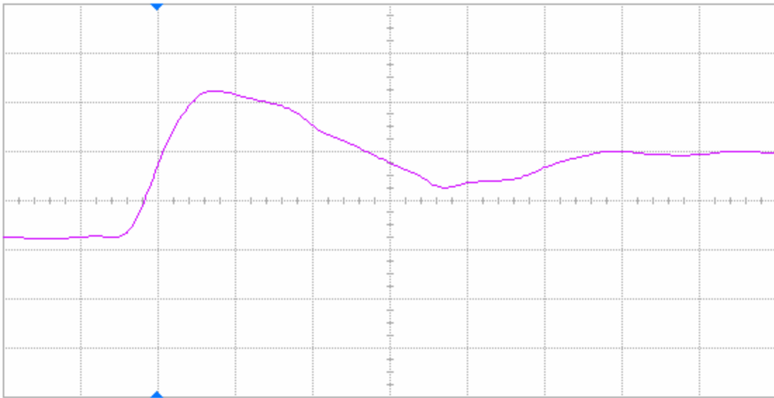
Figure 8(a) DUT 72887 pre-irradiation rising edge, abscissa scale is 2 V/div and ordinate scale is 2 ns/div.
