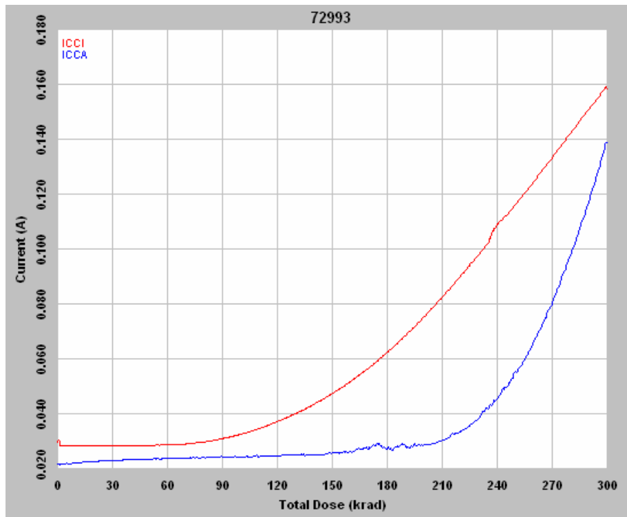
Figure 5 DUT 72993 in-flux I_{CCA} and I_{CCI}
