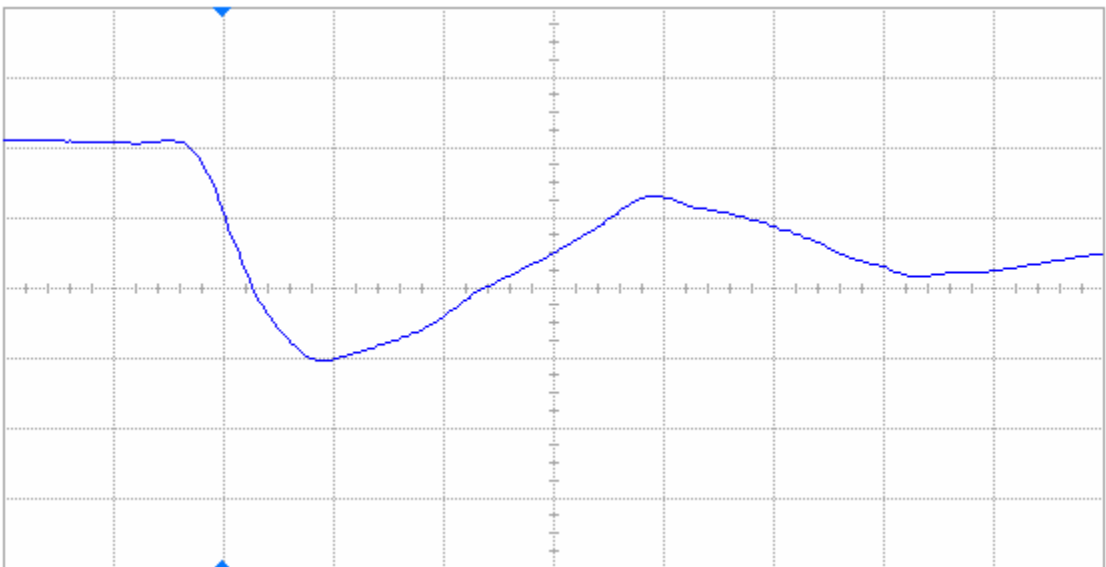
Figure 18(b) DUT 73001 post-annealing falling edge, abscissa scale is 2 V/div and ordinate scale is 2 ns/div.
