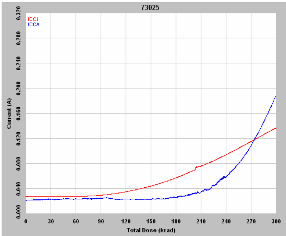
Figure 7 DUT 73025 in-flux I_{CCA} and I_{CCI}
