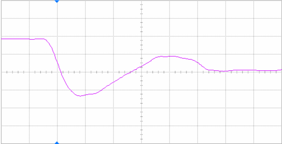
Figure 17(a) DUT 72993 pre-irradiation falling edge, abscissa scale is 2 V/div and ordinate scale is 2 ns/div.
