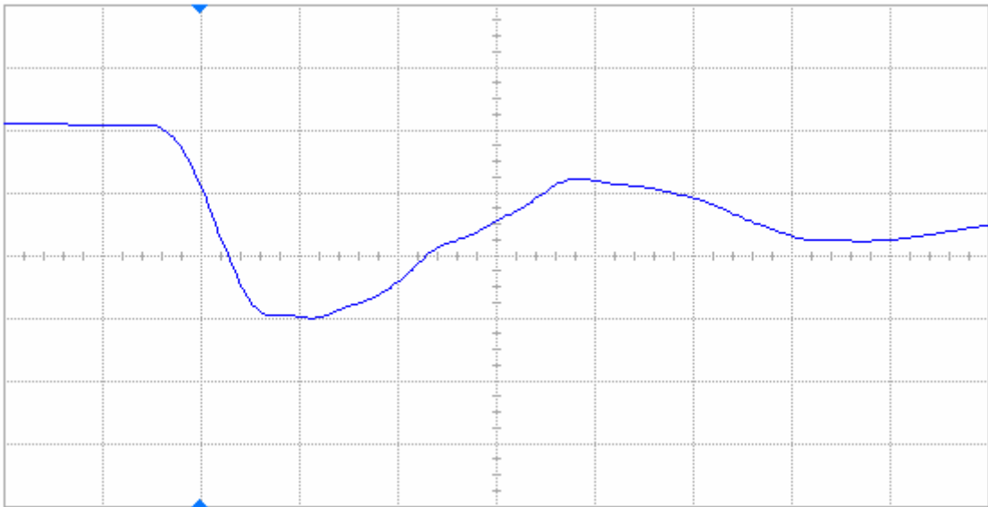
Figure 17(b) DUT 72993 post-annealing falling edge, abscissa scale is 2 V/div and ordinate scale is 2 ns/div.
