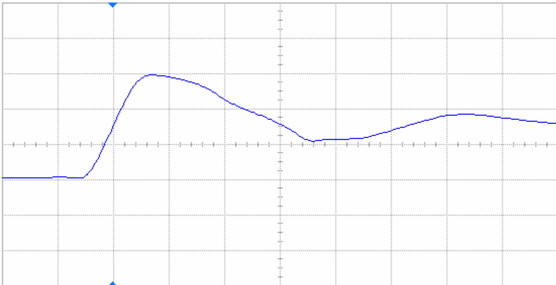
Figure 13(b) DUT 73025 post-annealing rising edge, abscissa scale is 2 V/div and ordinate scale is 2 ns/div.
