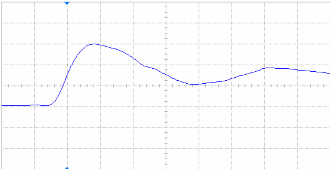
Figure 9(b) DUT 72939 post-annealing rising edge, abscissa scale is 2 V/div and ordinate scale is 2 ns/div.
