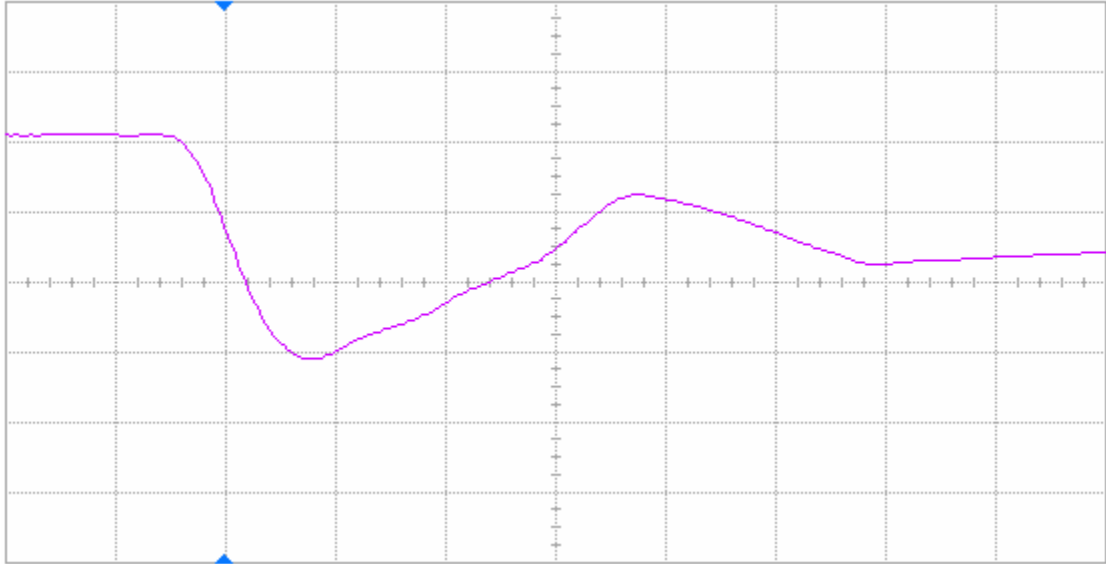
Figure 19(a) DUT 73025 pre-irradiation falling edge, abscissa scale is 2 V/div and ordinate scale is 2 ns/div.
