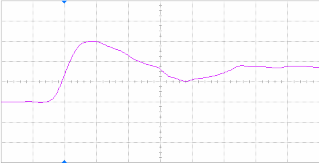
Figure 12(a) DUT 73001 pre-irradiation rising edge, abscissa scale is 2 V/div and ordinate scale is 2 ns/div.
