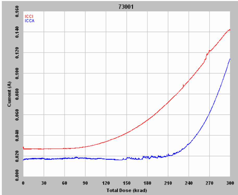
Figure 6 DUT 73001 in-flux I_{CCA} and I_{CCI}
