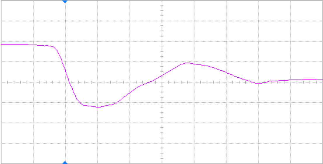
Figure 16(a) DUT 72992 pre-irradiation falling edge, abscissa scale is 2 V/div and ordinate scale is 2 ns/div.
