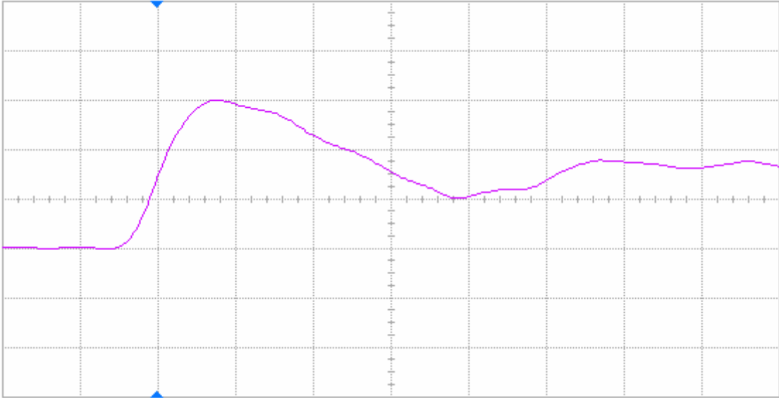
Figure 9(a) DUT 72939 pre-irradiation rising edge, abscissa scale is 2 V/div and ordinate scale is 2 ns/div.
