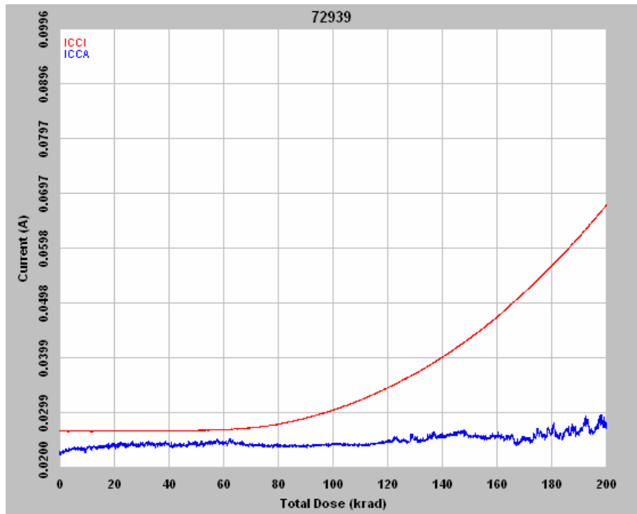
Figure 3 DUT 72939 in-flux I_{CCA} and I_{CCI}
