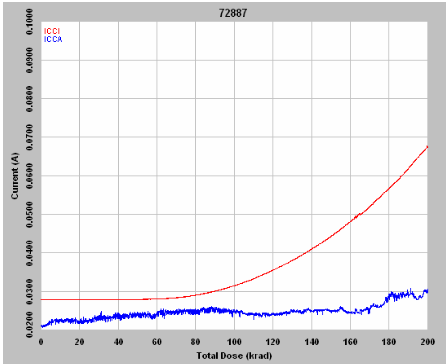
Figure 2 DUT 72887 in-flux I_{CCA} and I_{CCI}
