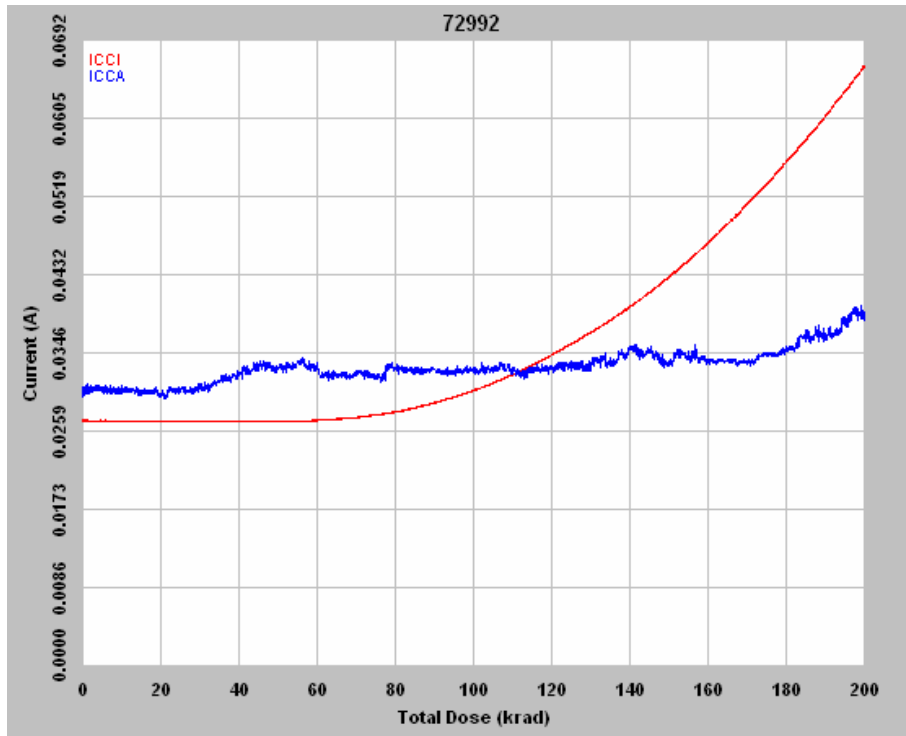
Figure 4 DUT 72992 in-flux I_{CCA} and I_{CCI}
