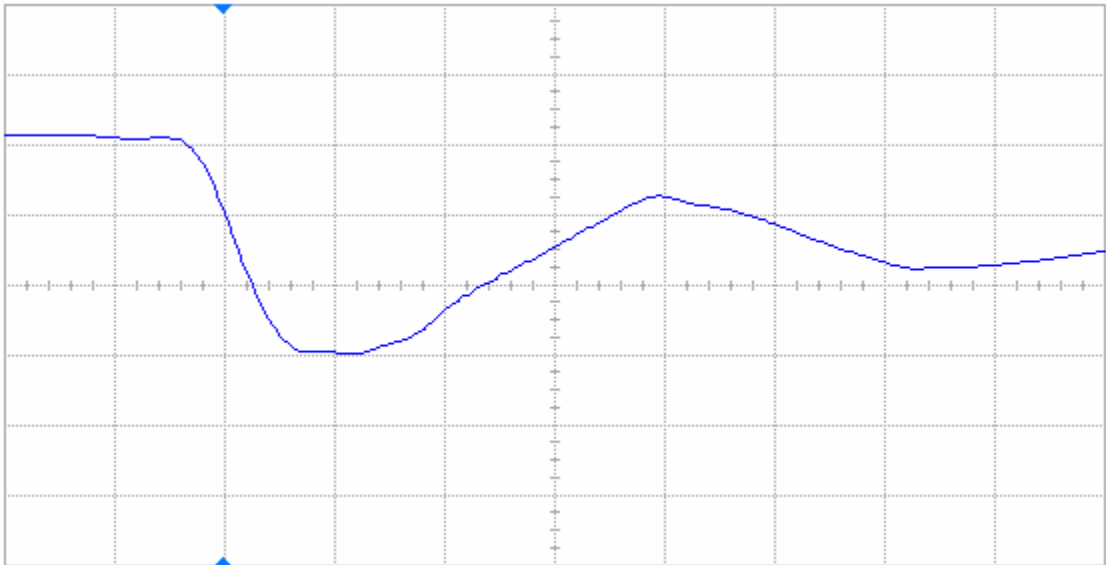
Figure 19(b) DUT 73025 post-annealing falling edge, abscissa scale is 2 V/div and ordinate scale is 2 ns/div.
