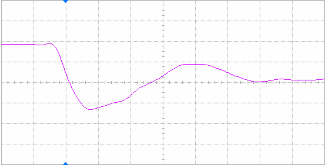
Figure 15(a) DUT 72939 pre-irradiation falling edge, abscissa scale is 2 V/div and ordinate scale is 2 ns/div.
