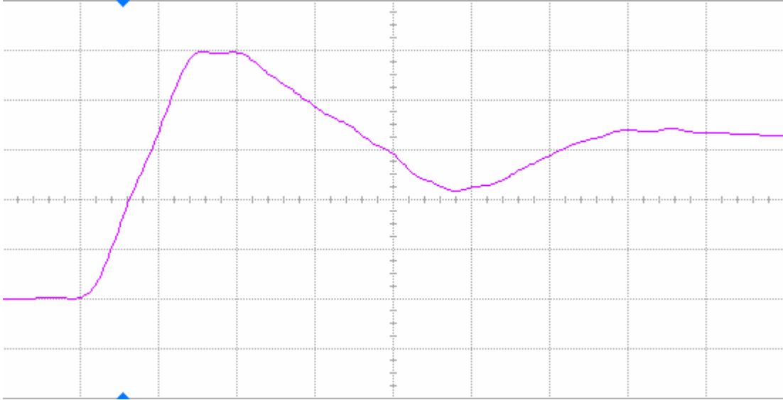
Figure 12(a) DUT 2242 pre-irradiation rising edge, abscissa scale is 1 V/div and ordinate scale is 2 ns/div.
