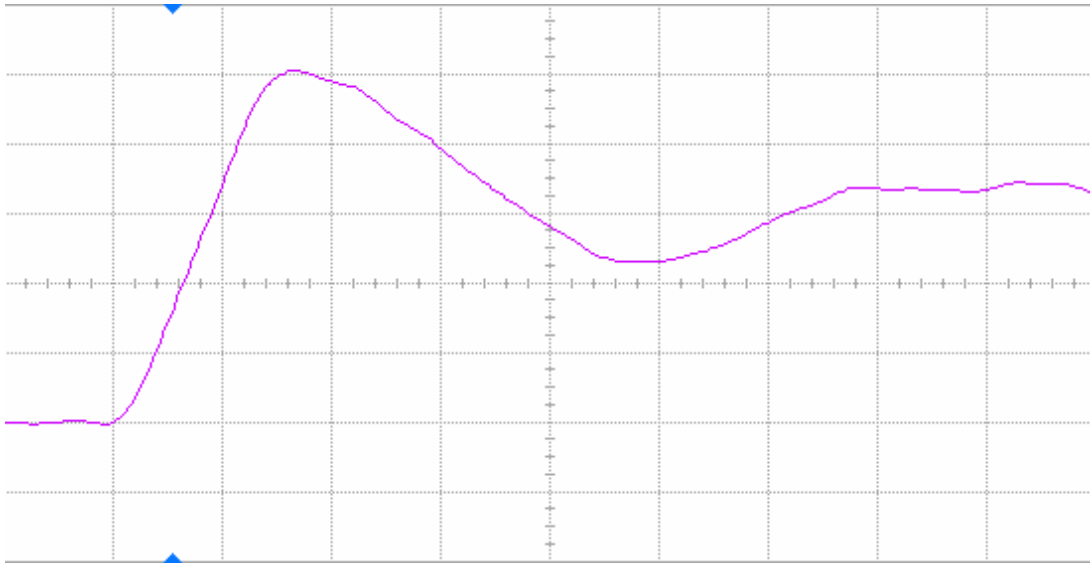
Figure 8(a) DUT 2185 pre-irradiation rising edge, abscissa scale is 1 V/div and ordinate scale is 2 ns/div.
