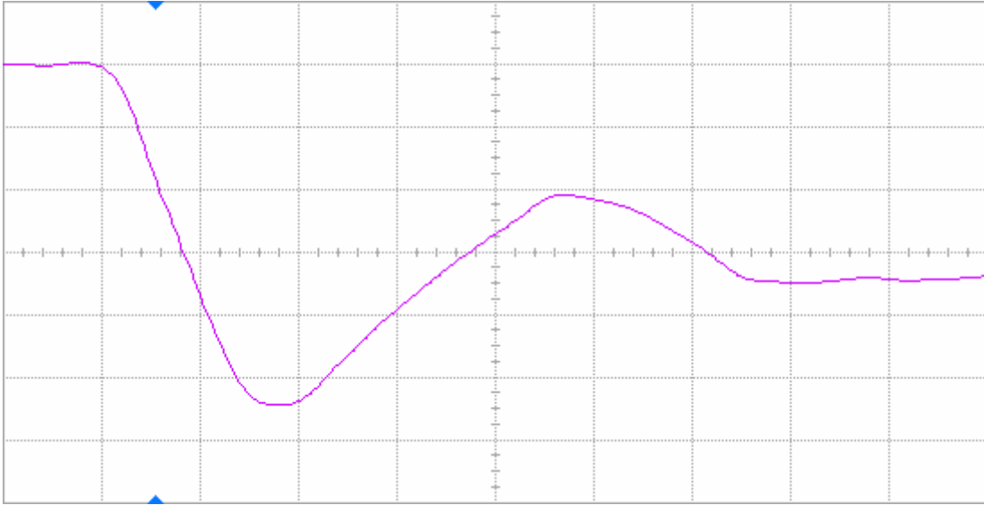
Figure 17(a) DUT 2200 pre-irradiation falling edge, abscissa scale is 1 V/div and ordinate scale is 2 ns/div.
