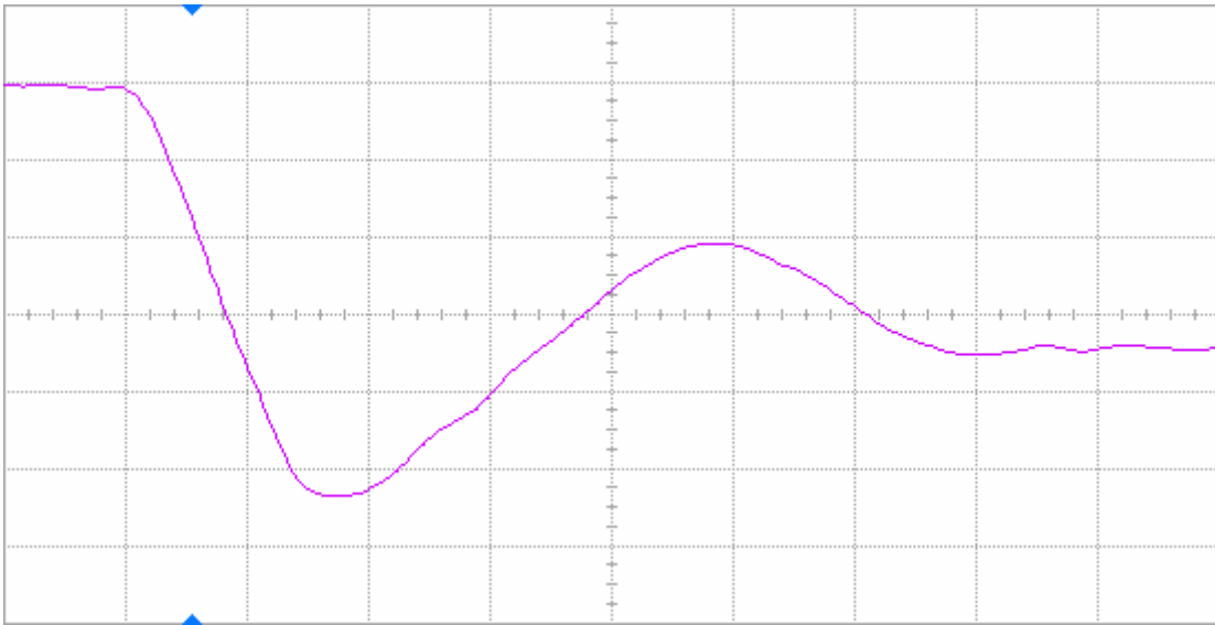
Figure 15(a) DUT 2195 pre-irradiation falling edge, abscissa scale is 1 V/div and ordinate scale is 2 ns/div.
