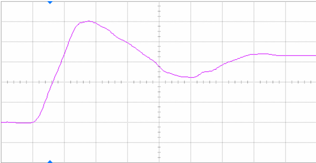
Figure 13(a) DUT 2264 pre-irradiation rising edge, abscissa scale is 1 V/div and ordinate scale is 2 ns/div.
