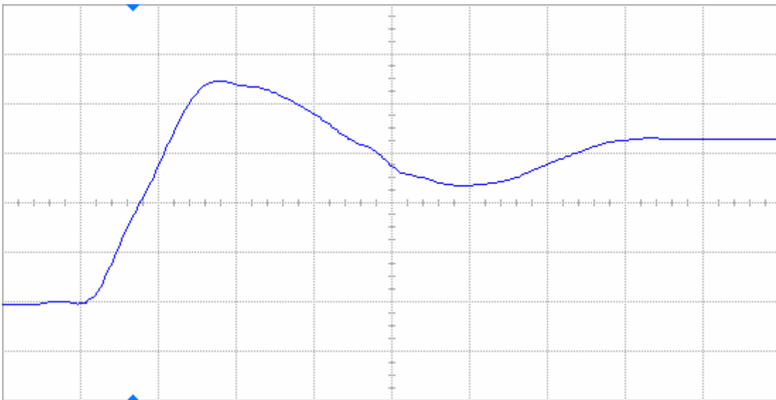
Figure 10(b) DUT 2199 post-annealing rising edge, abscissa scale is 1 V/div and ordinate scale is 2 ns/div.
