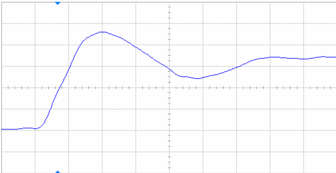
Figure 9(b) DUT 2195 post-annealing rising edge, abscissa scale is 1 V/div and ordinate scale is 2 ns/div.
