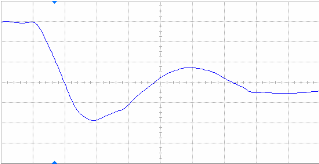
Figure 19(b) DUT 2264 post-annealing falling edge, abscissa scale is 1 V/div and ordinate scale is 2 ns/div.
