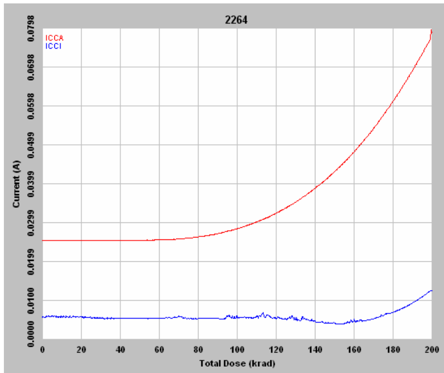
Figure 7 DUT 2264 in-flux I_{CCA} and I_{CCI}
