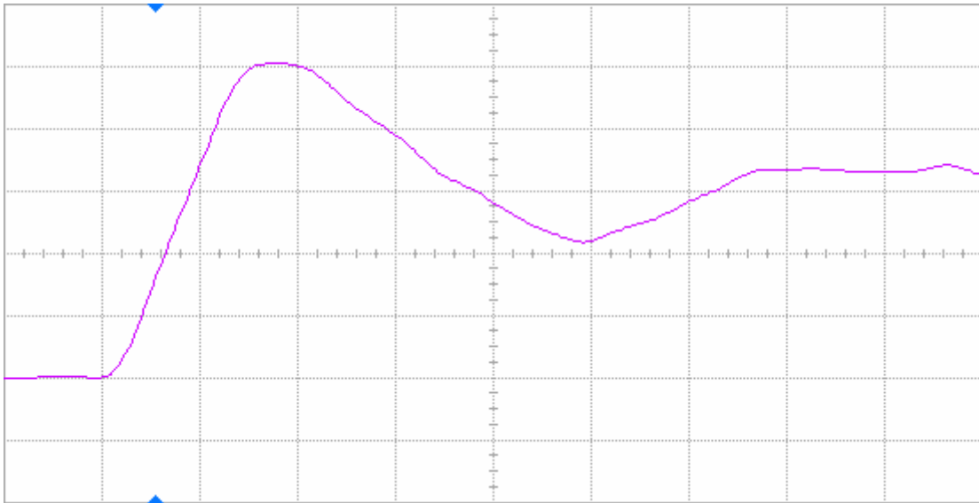
Figure 9(a) DUT 2195 pre-irradiation rising edge, abscissa scale is 1 V/div and ordinate scale is 2 ns/div.
