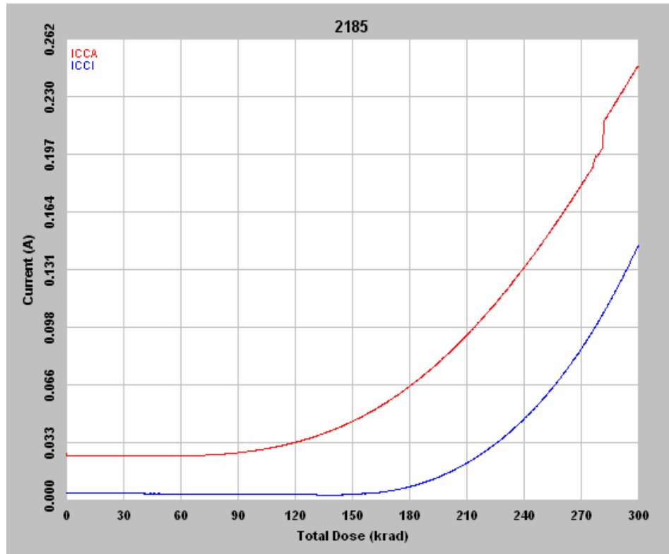
Figure 2 DUT 2185 in-flux I_{CCA} and I_{CCI}
