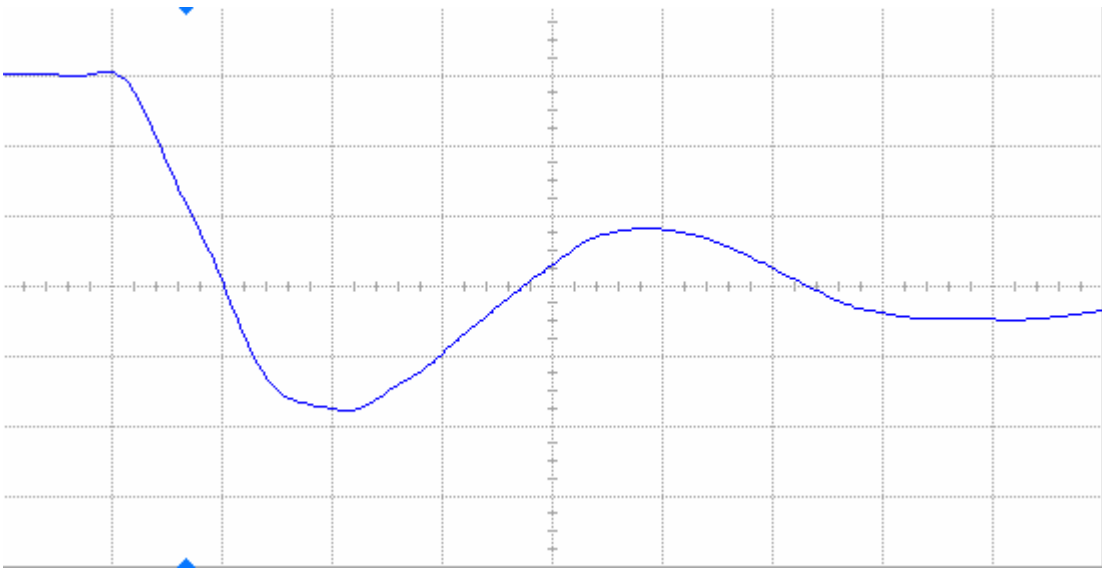
Figure 15(b) DUT 2195 post-annealing falling edge, abscissa scale is 1 V/div and ordinate scale is 2 ns/div.
