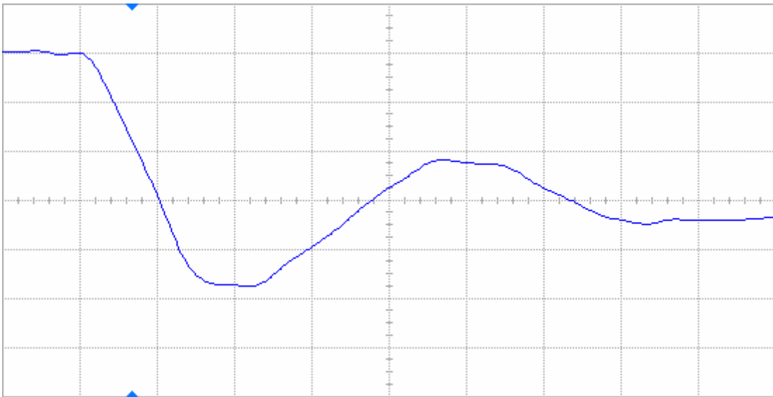
Figure 16(b) DUT 2199 post-annealing falling edge, abscissa scale is 1 V/div and ordinate scale is 2 ns/div.
