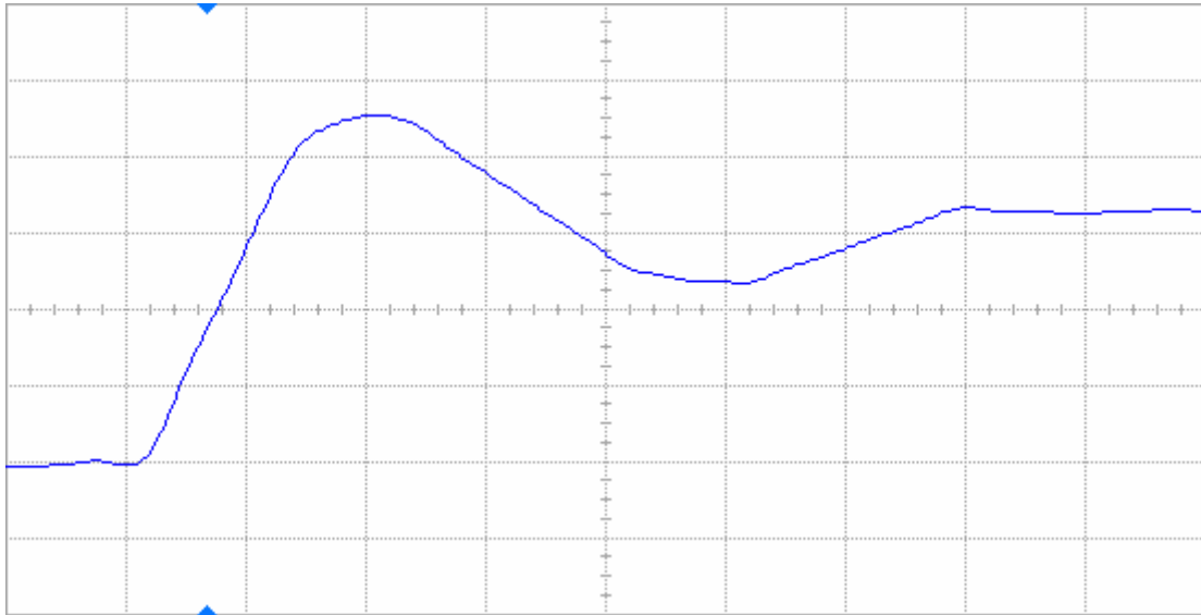
Figure 11(b) DUT 2200 post-annealing rising edge, abscissa scale is 1 V/div and ordinate scale is 2 ns/div.
