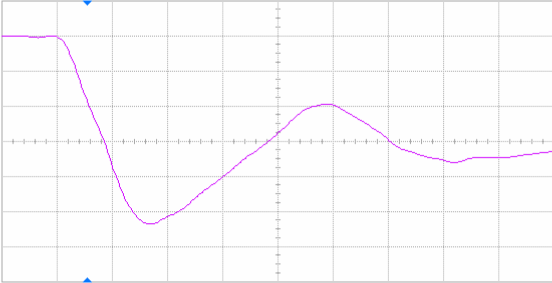
Figure 18(a) DUT 2242 pre-irradiation falling edge, abscissa scale is 1 V/div and ordinate scale is 2 ns/div.
