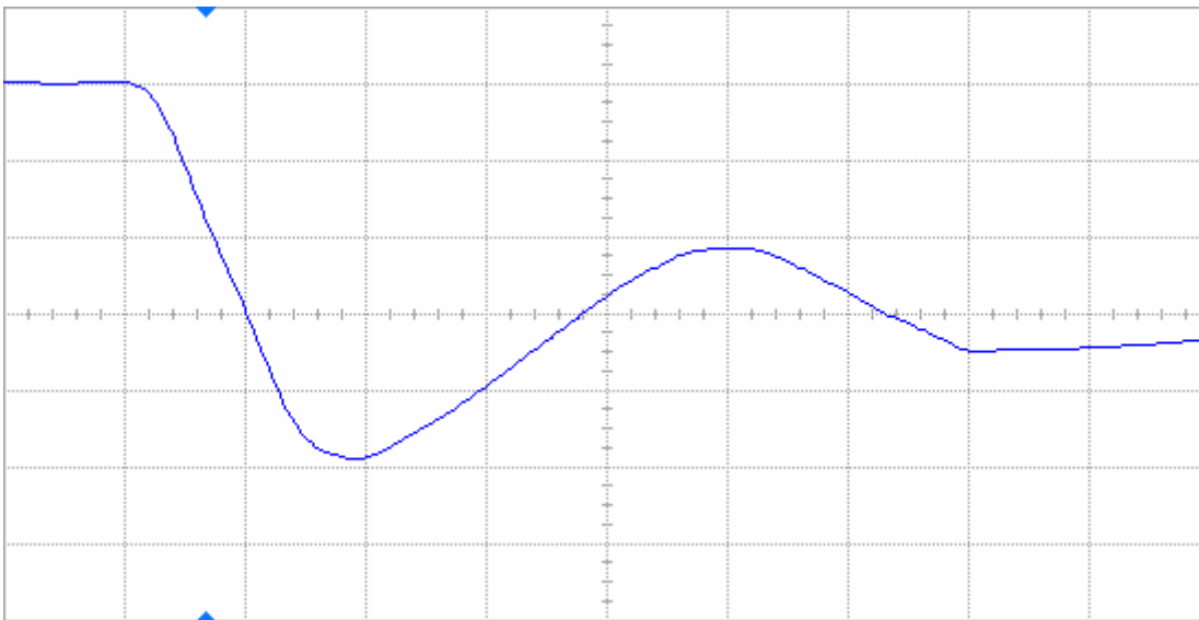
Figure 14(b) DUT 2185 post-annealing falling edge, abscissa scale is 1 V/div and ordinate scale is 2 ns/div.
