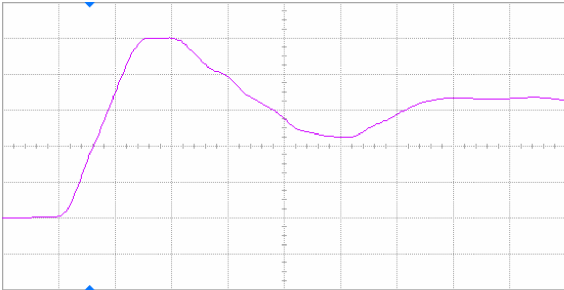
Figure 10(a) DUT 2199 pre-radiation rising edge, abscissa scale is 1 V/div and ordinate scale is 2 ns/div.
