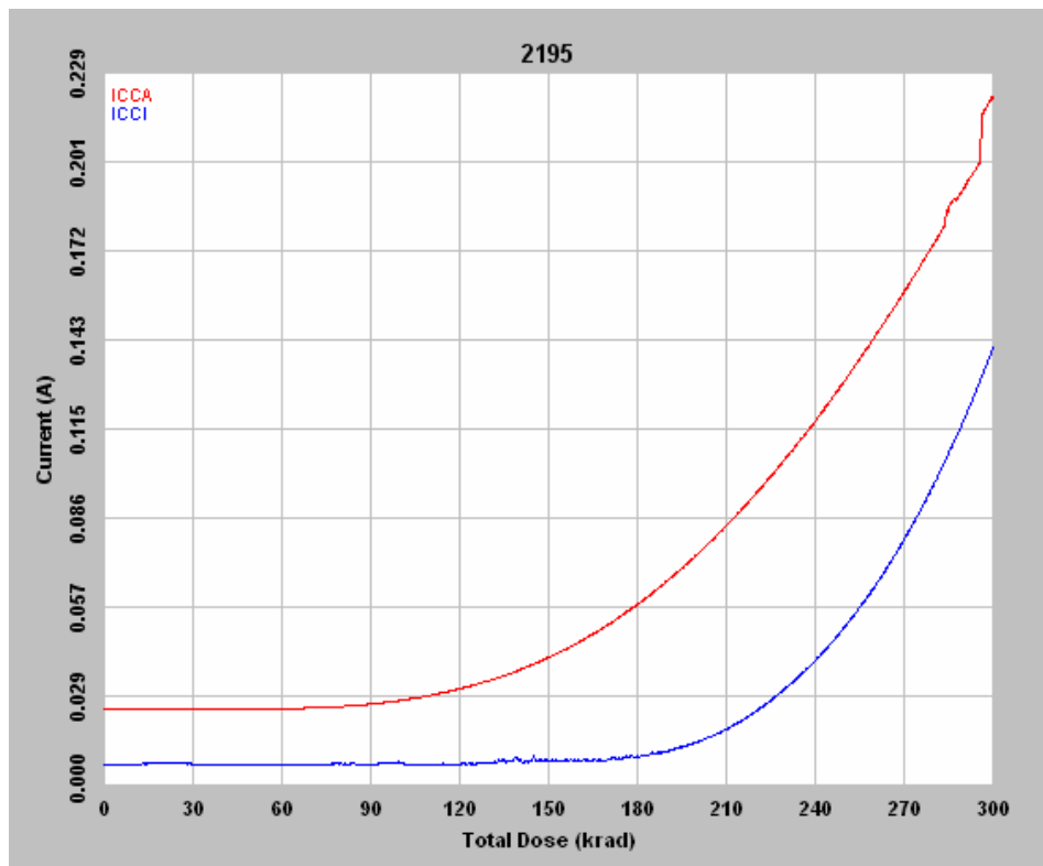
Figure 3 DUT 2195 in-flux I_{CCA} and I_{CCI}
