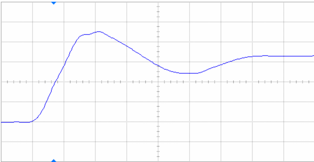
Figure 13(b) DUT 2264 post-annealing rising edge, abscissa scale is 1 V/div and ordinate scale is 2 ns/div.
