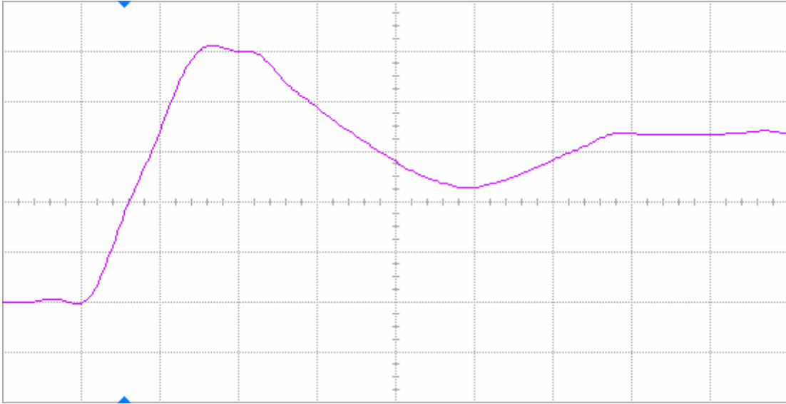
Figure 11(a) DUT 2200 pre-irradiation rising edge, abscissa scale is 1 V/div and ordinate scale is 2 ns/div.
