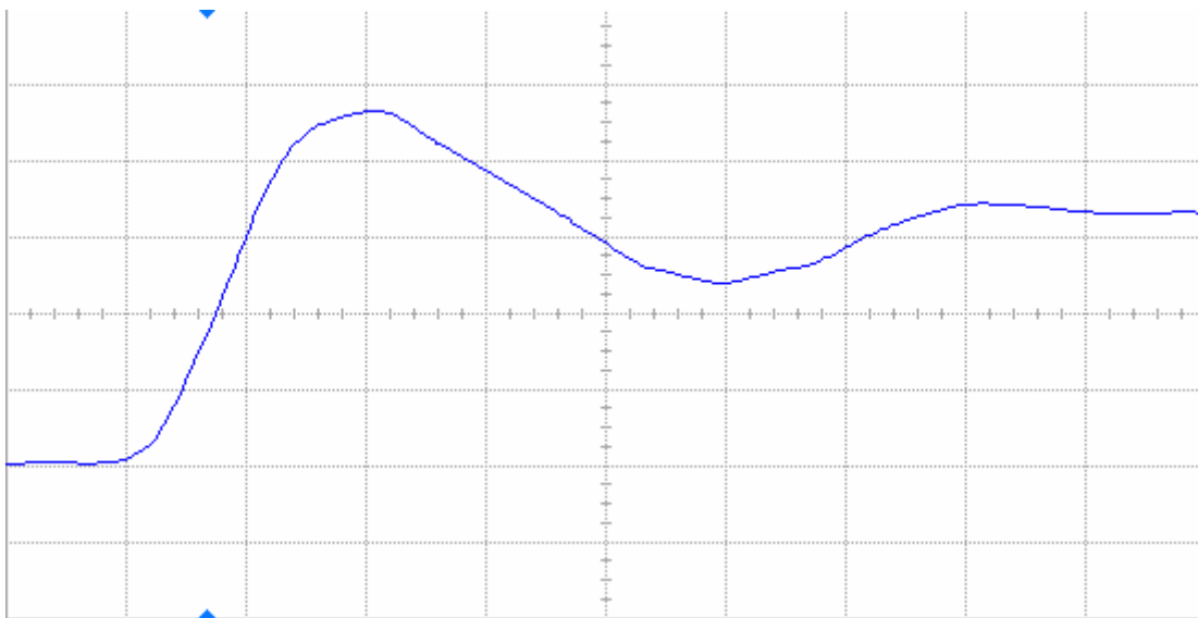
Figure 8(b) DUT 2185 post-annealing rising edge, abscissa scale is 1 V/div and ordinate scale is 2 ns/div.
