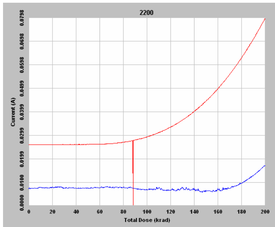
Figure 5 DUT 2200 in-flux I CCA and I CCI
