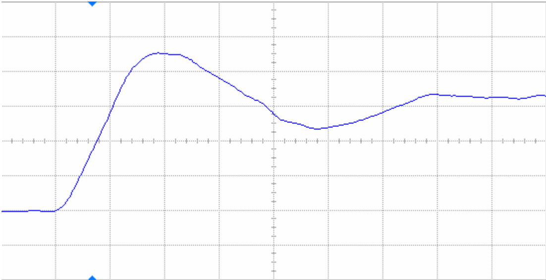
Figure 12(b) DUT 2242 post-annealing rising edge, abscissa scale is 1 V/div and ordinate scale is 2 ns/div.
