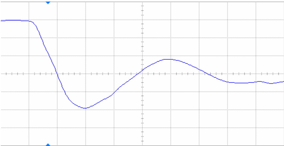
Figure 18(b) DUT 2242 post-annealing falling edge, abscissa scale is 1 V/div and ordinate scale is 2 ns/div.
