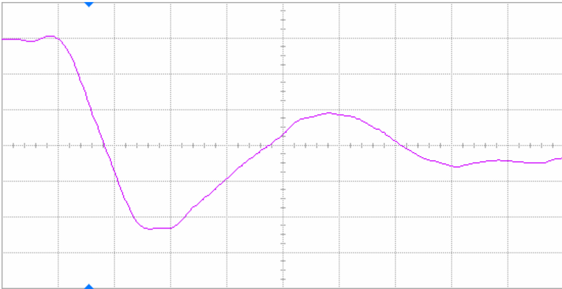
Figure 16(a) DUT 2199 pre-irradiation falling edge, abscissa scale is 1 V/div and ordinate scale is 2 ns/div.
