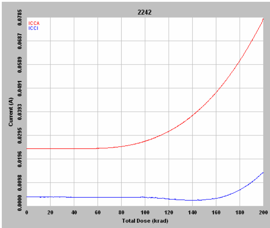
Figure 6 DUT 2242 in-flux I_{CCA} and I_{CCI}
