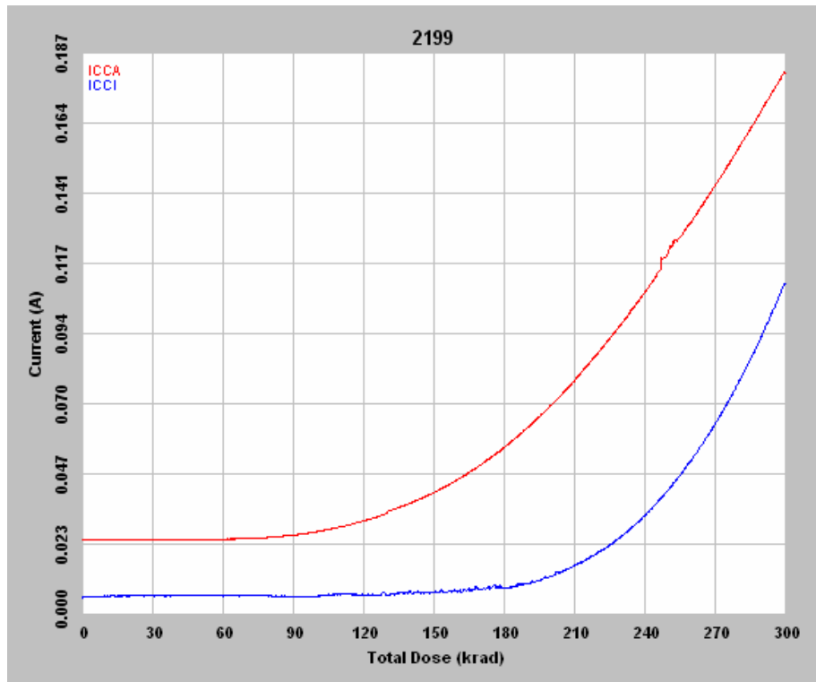
Figure 4 DUT 2199 in-flux I CCA and I CCI
