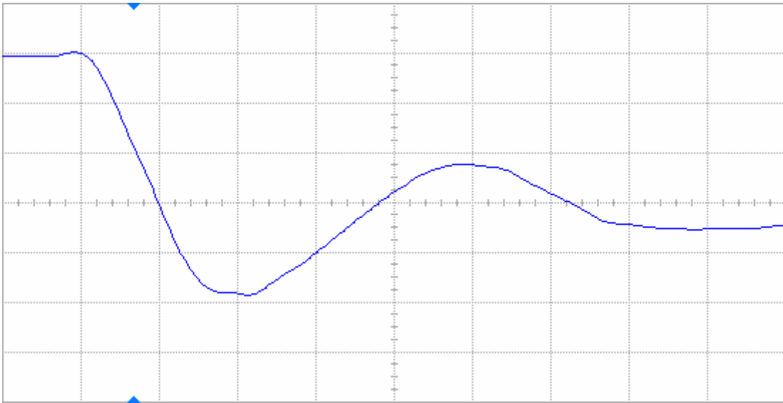
Figure 17(b) DUT 2200 post-annealing falling edge, abscissa scale is 1 V/div and ordinate scale is 2 ns/div.
