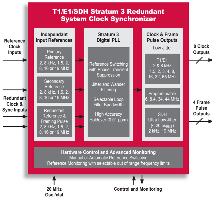
ZL30105 Simplified Block Diagram
