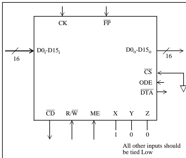
Figure 10 - Counter Mode Pinout
