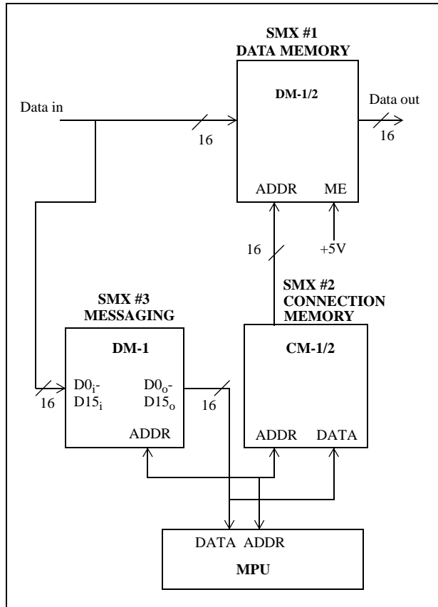
Figure 22 - A 1024 Channel Switch Matrix with Message Capability
