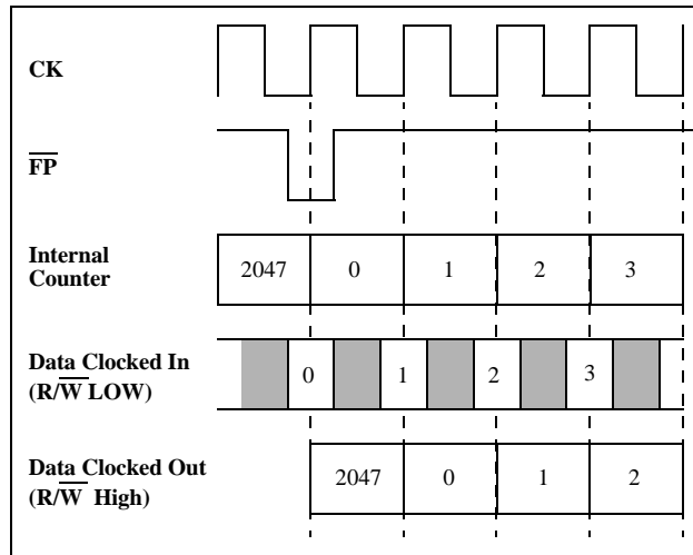
Figure 11 - Counter Mode Functional Timing
