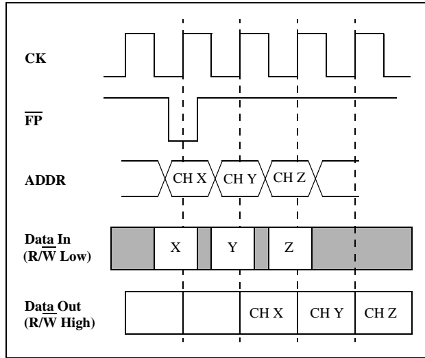
Figure 13 - External Mode Functional Timing
