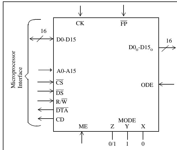
Figure 7 - Connect Memory Modes Pinout
