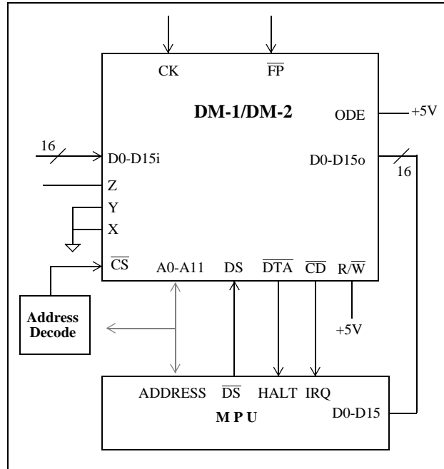
Figure 21 - Reading the Data Memory with a Microprocessor
