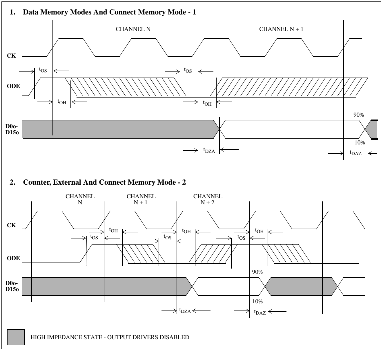
Figure 24 - Output Drive Enable Timing
