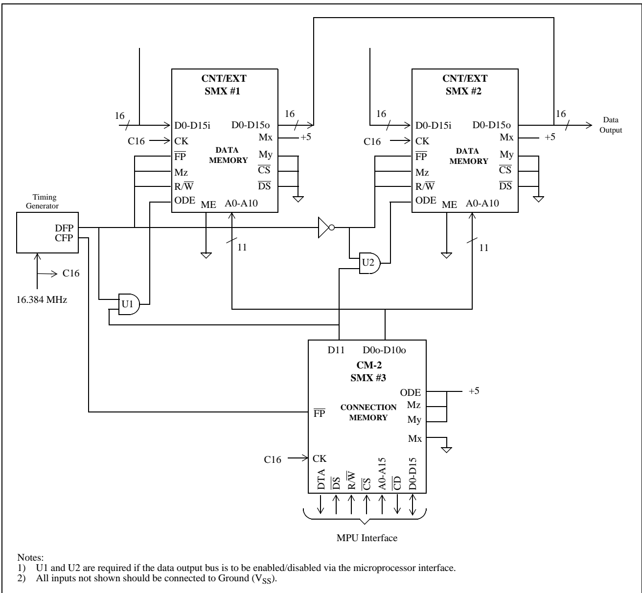
Figure 18 - 2048 Channel Timeslot Interchange Circuit
