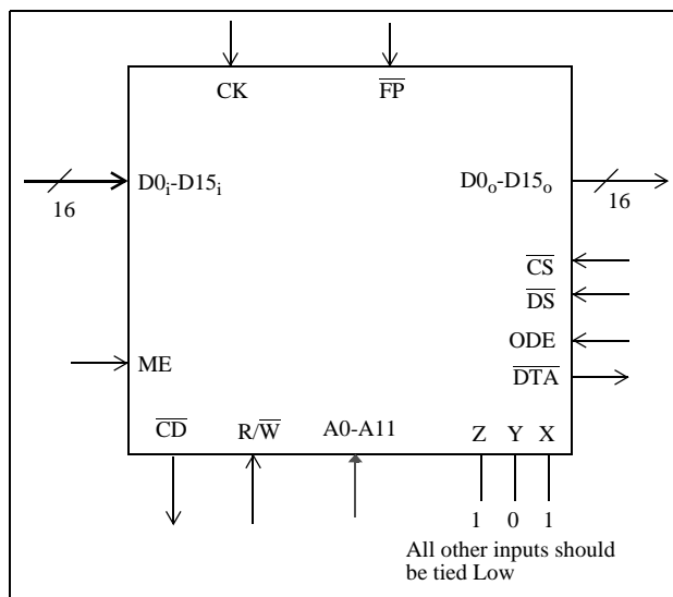
Figure 12 - External Mode Pinout
