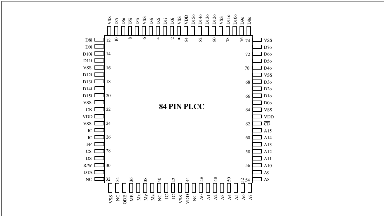
Figure 2 - Pin Connections
