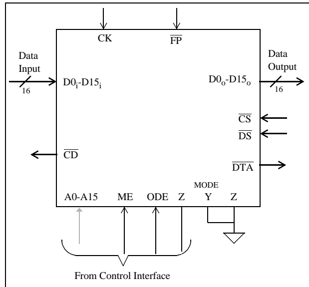
Figure 3 - Data Memory Modes 1 and 2 Pinout
