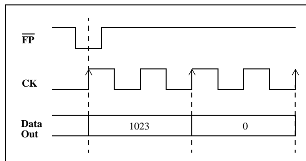
Figure 8 - Connect Memory Mode-1 Functional Timing
