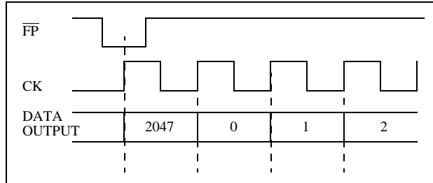
Figure 9 - Connect Memory Mode-2 Functional Timing
