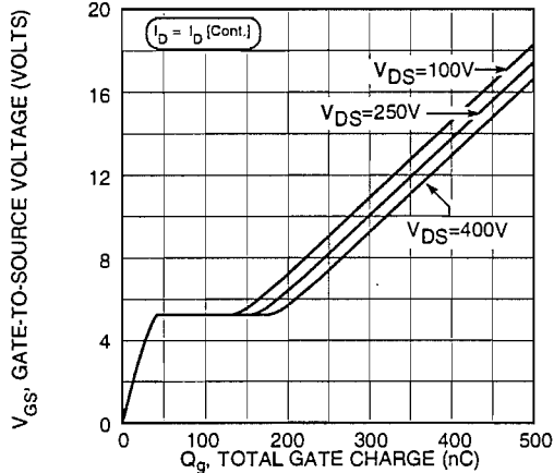
FIGURE 12, GATE CHARGES vs GATE-TO-SOURCE AREA
