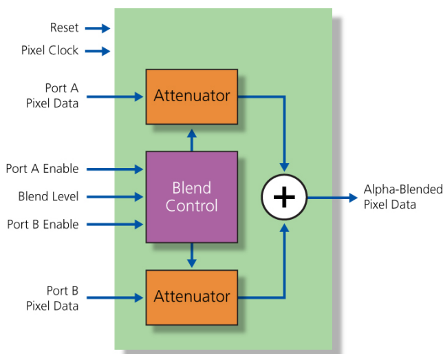
Block Diagram
