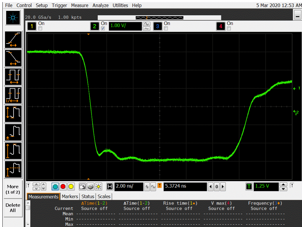
Figure 20a DUT 14045 Pre-Irradiation Falling Edge
