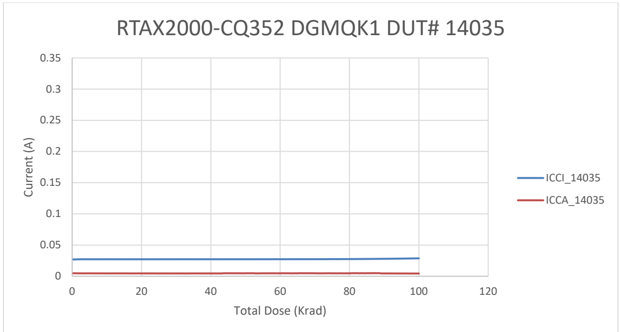
Figure 6 DUT 14035 Influx ICCA and ICCI
