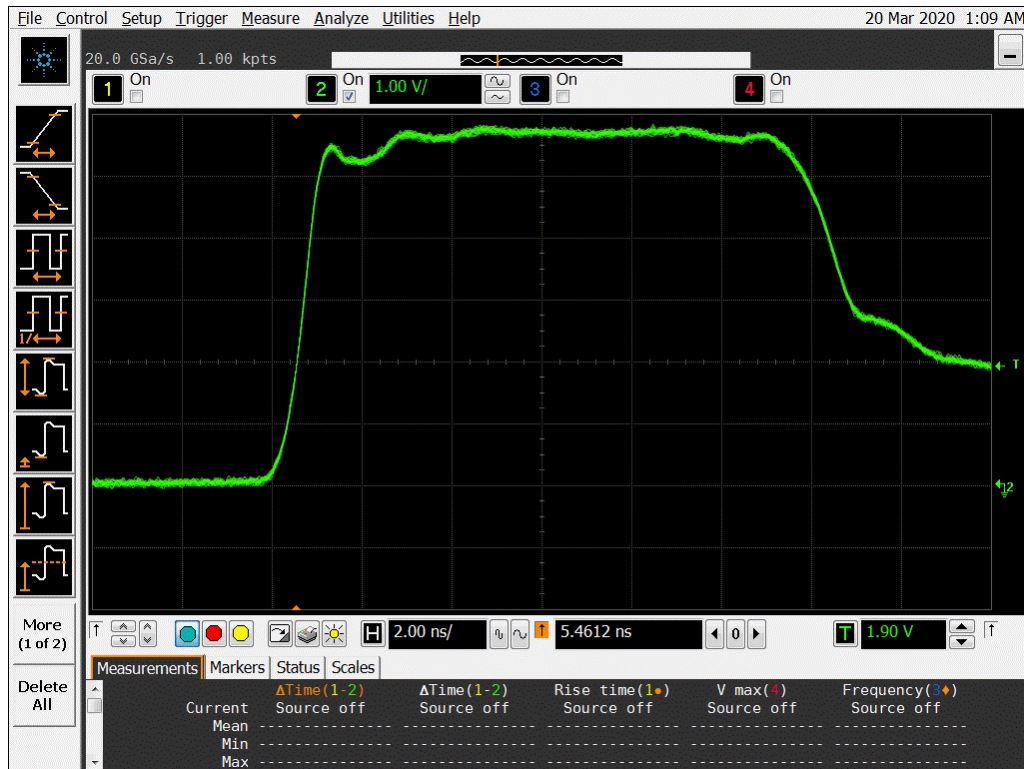
Figure 11b DUT 14049 Post-Annealing Rising edge
