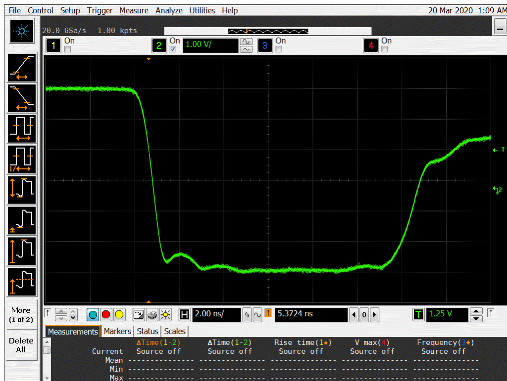
Figure 17b DUT 14049 Post-Annealing Falling Edge
