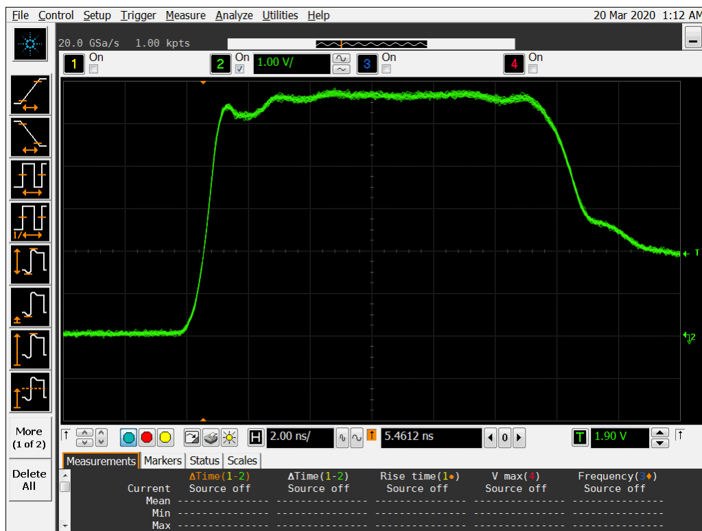
Figure 12b DUT 14062 Post-Annealing Rising Edge
