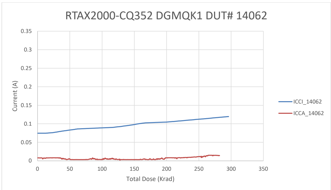
Figure 5 DUT 14062 Influx ICCA and ICCI
