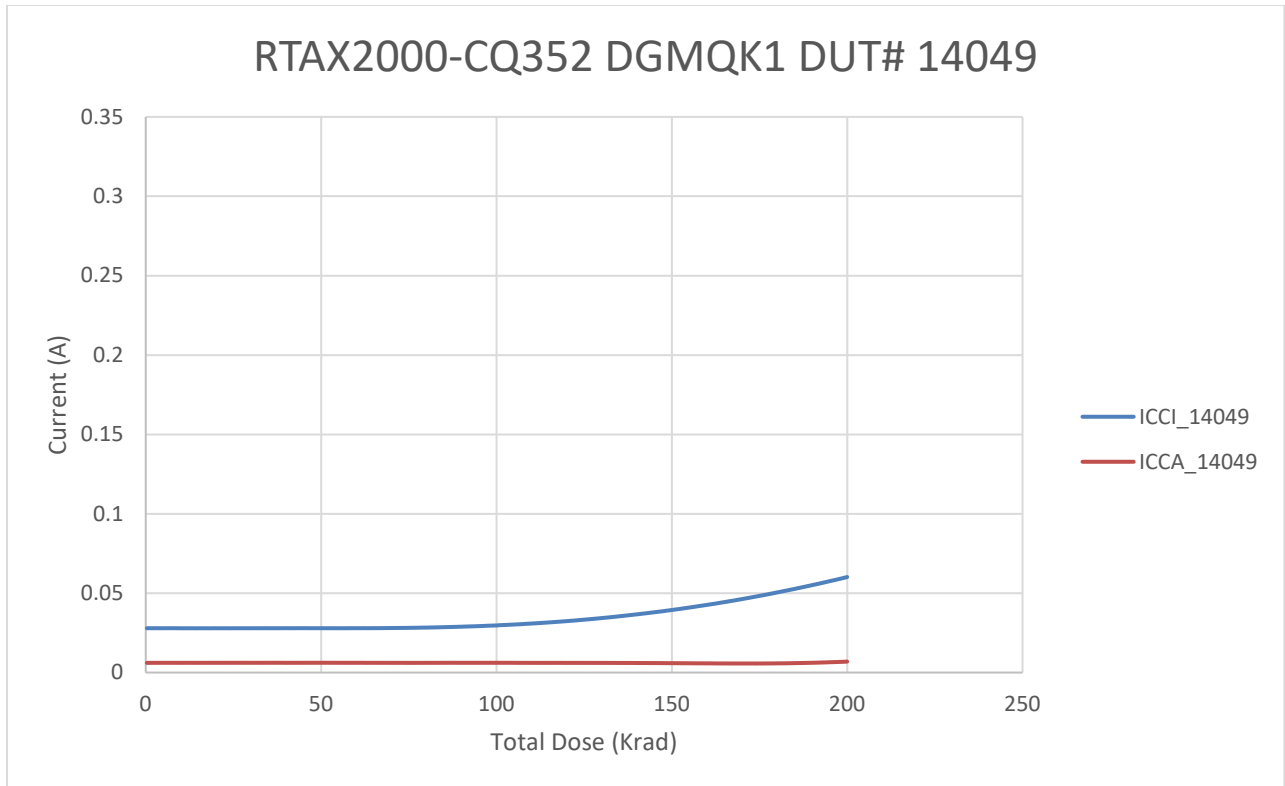
Figure 4 DUT 14049 Influx ICCA and ICCI
