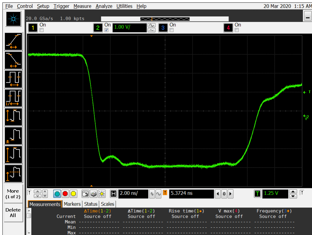
Figure 15b DUT 14063 Post-Annealing Falling Edge
