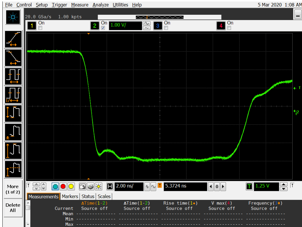
Figure 15a DUT 14063 Pre-Radiation Falling Edge
