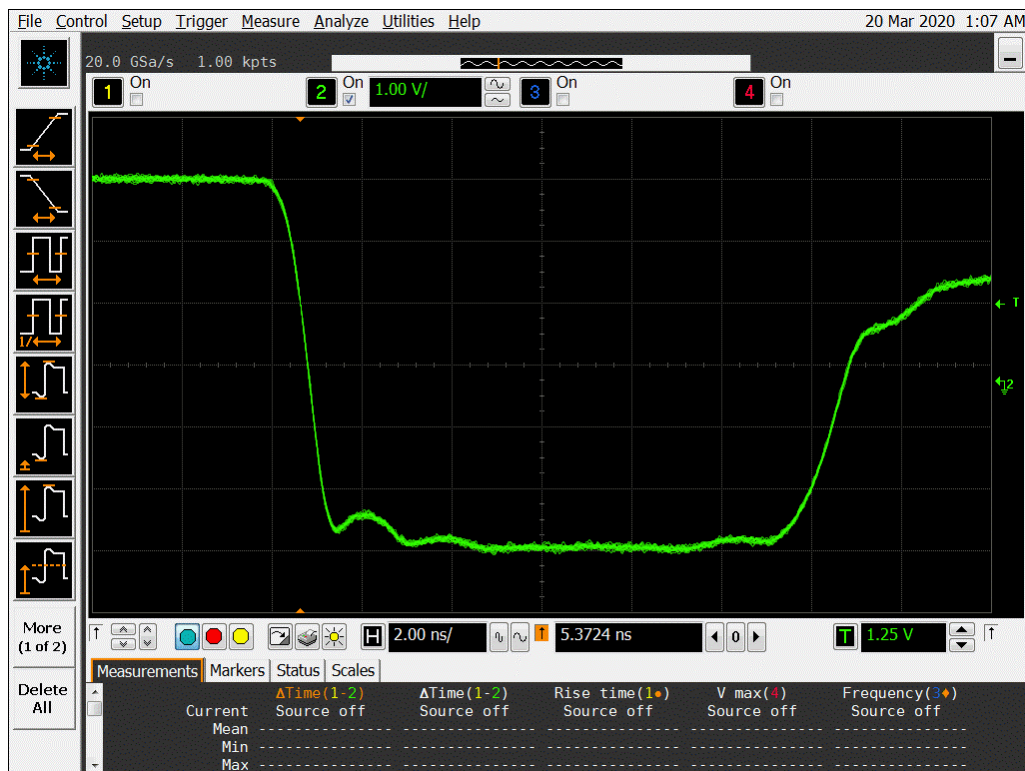
Figure 20b DUT 14045 Post-Annealing Falling Edge
