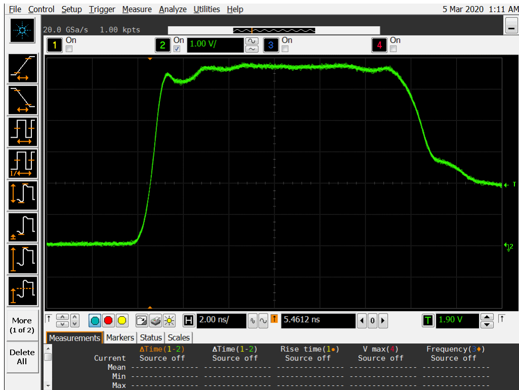
Figure 10a DUT 14064 Pre-Irradiation Rising Edge
