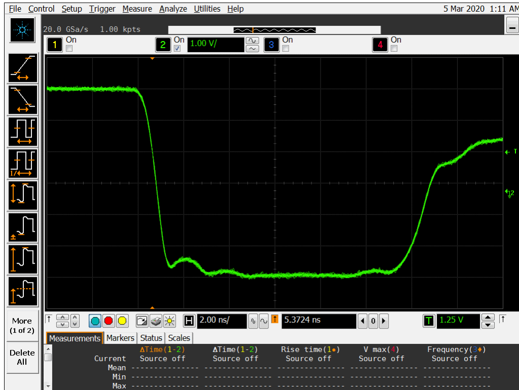
Figure 16a DUT 14064 Pre-Irradiation Falling Edge
