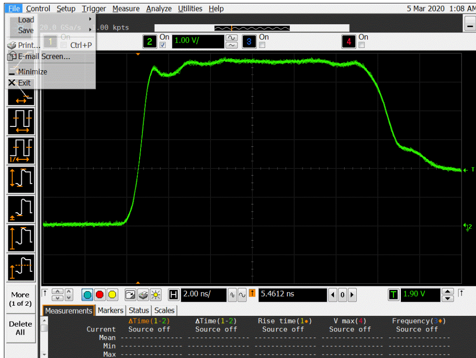
Figure 9a DUT 14063 Pre-Irradiation Rising Edge
