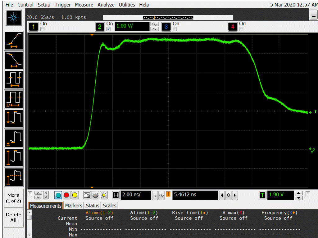
Figure 11a DUT 14049 Pre-Radiation Rising Edge
