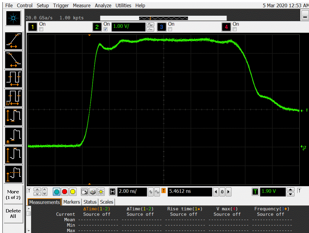
Figure 14a DUT 14045 Pre-Irradiation Rising Edge
