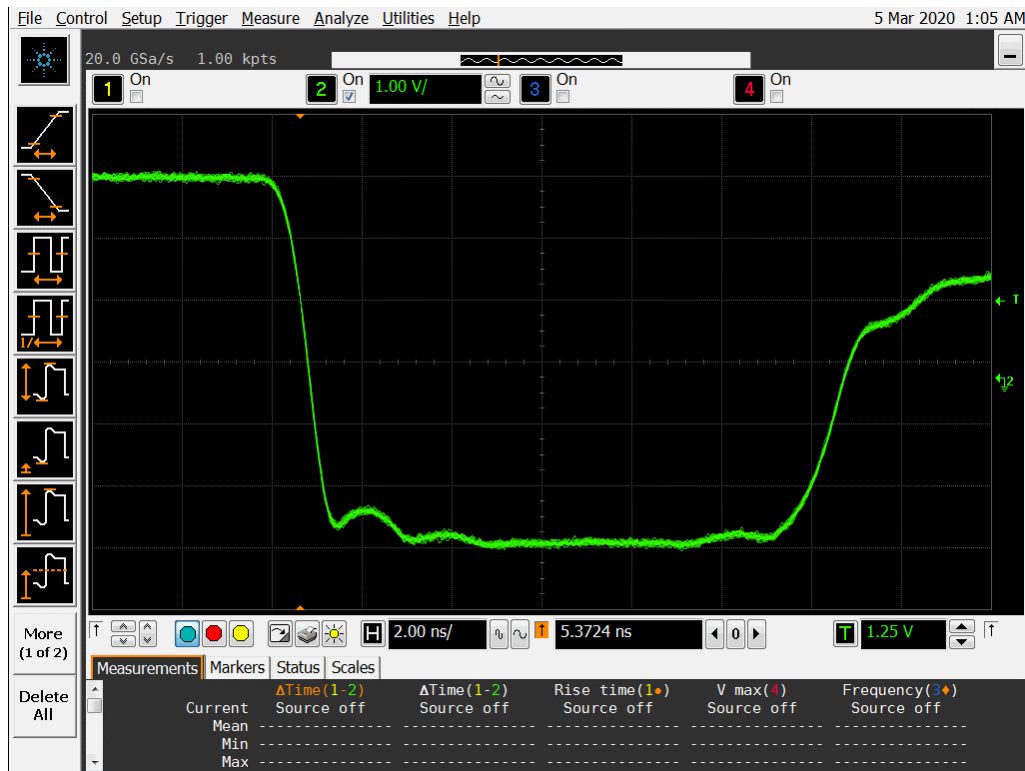
Figure 18a DUT 14062 Pre-Irradiation Falling Edge
