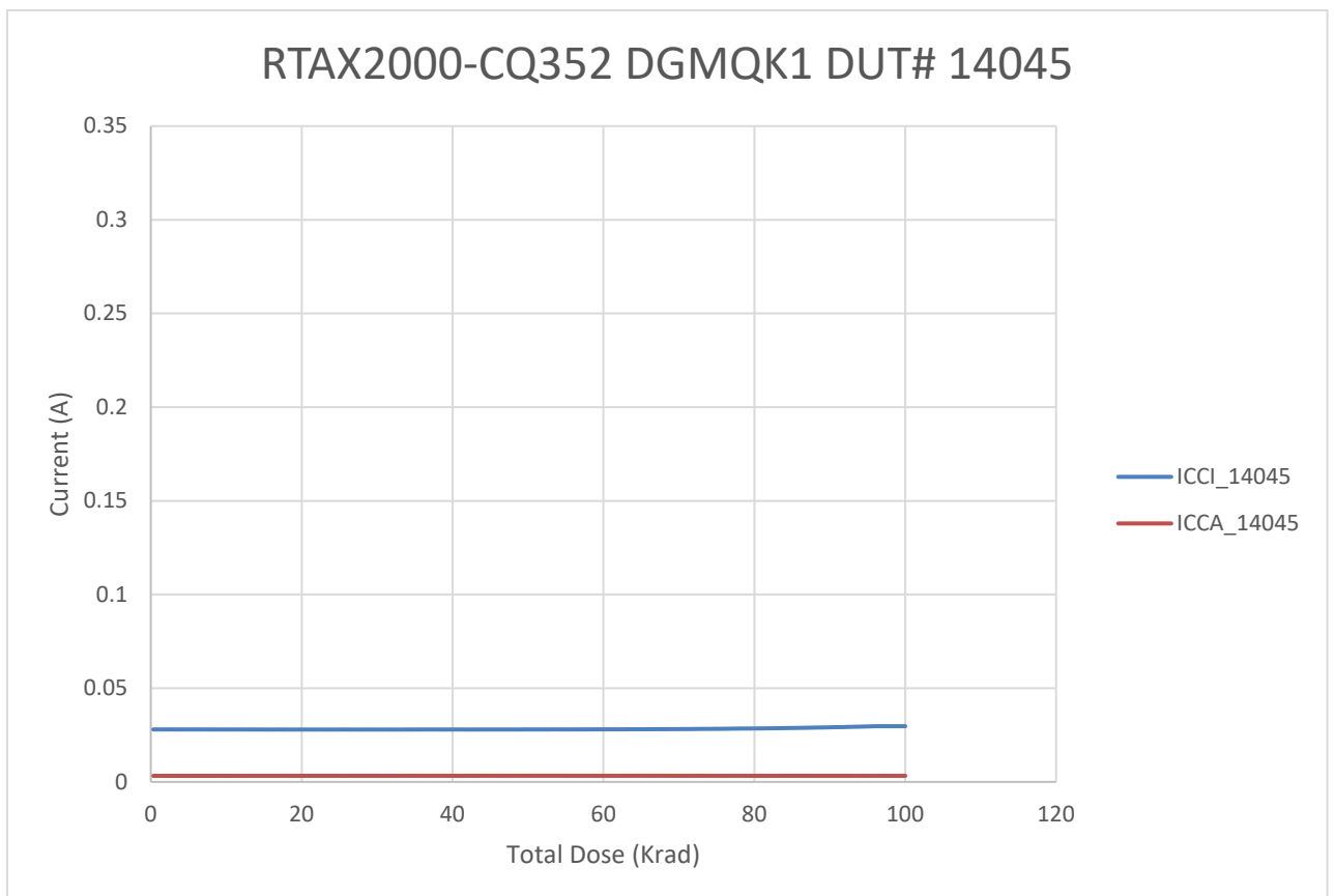
Figure 7 DUT 14045 Influx ICCA and ICCI
