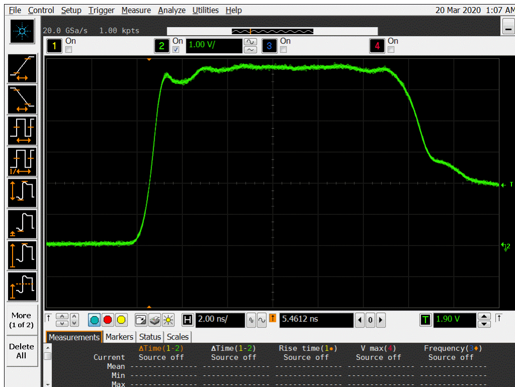
Figure 14b DUT 14045 Post-Annealing Rising Edge
