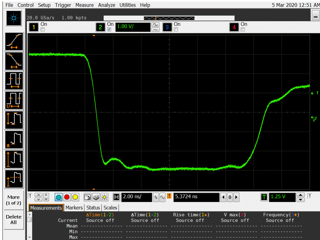
Figure 19a DUT 14035 Pre-Irradiation Falling Edge
