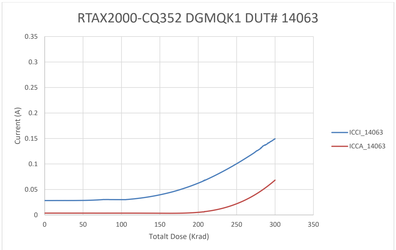
Figure 2 DUT 14063 Influx ICCA and ICCI
