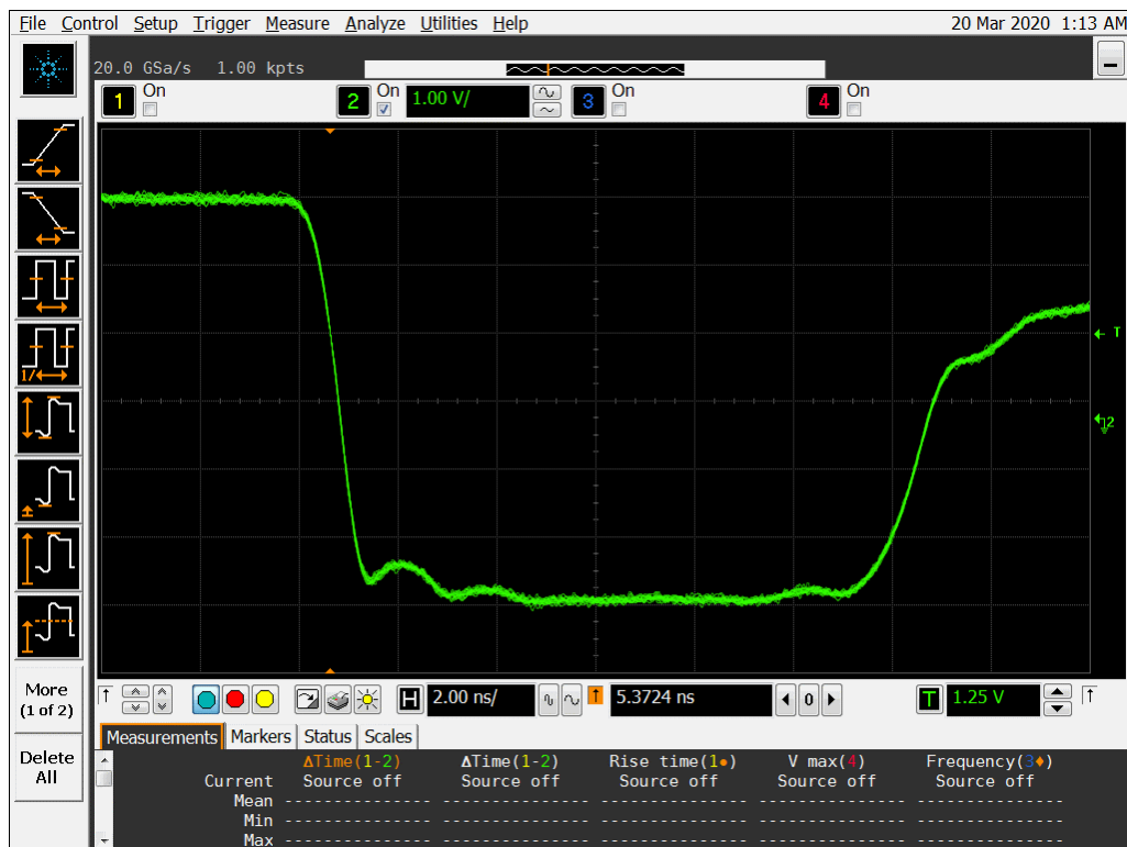
Figure 18b DUT 14062 Post-Annealing Falling Edge
