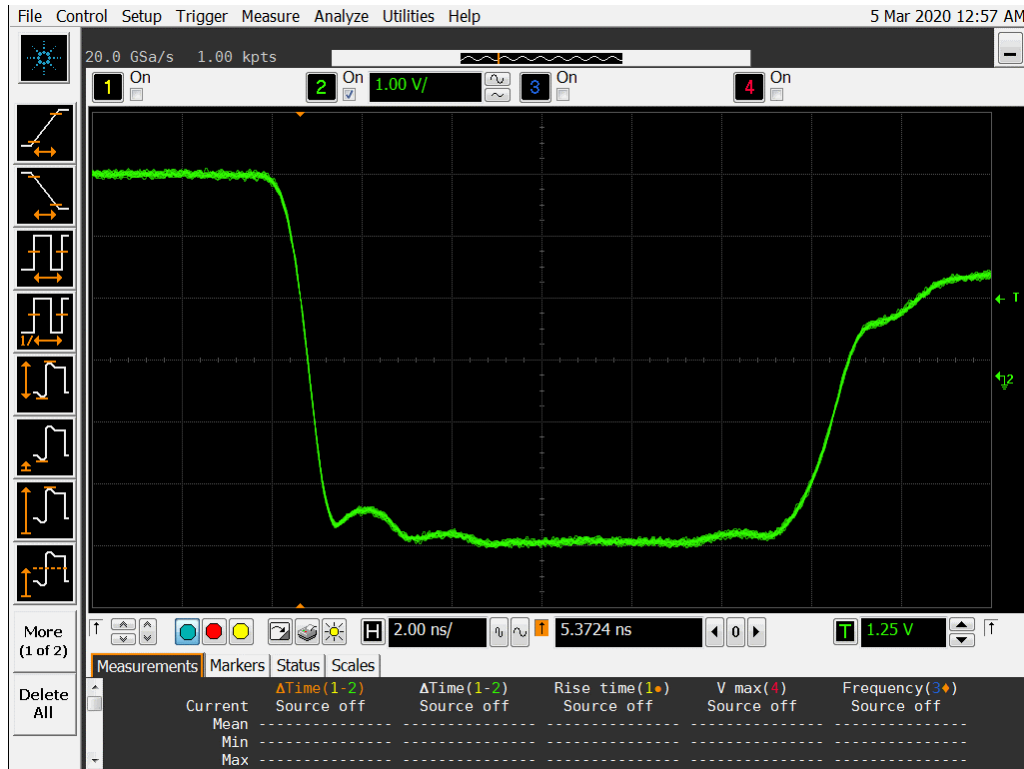
Figure 17a DUT 14049 Pre-Irradiation Falling Edge
