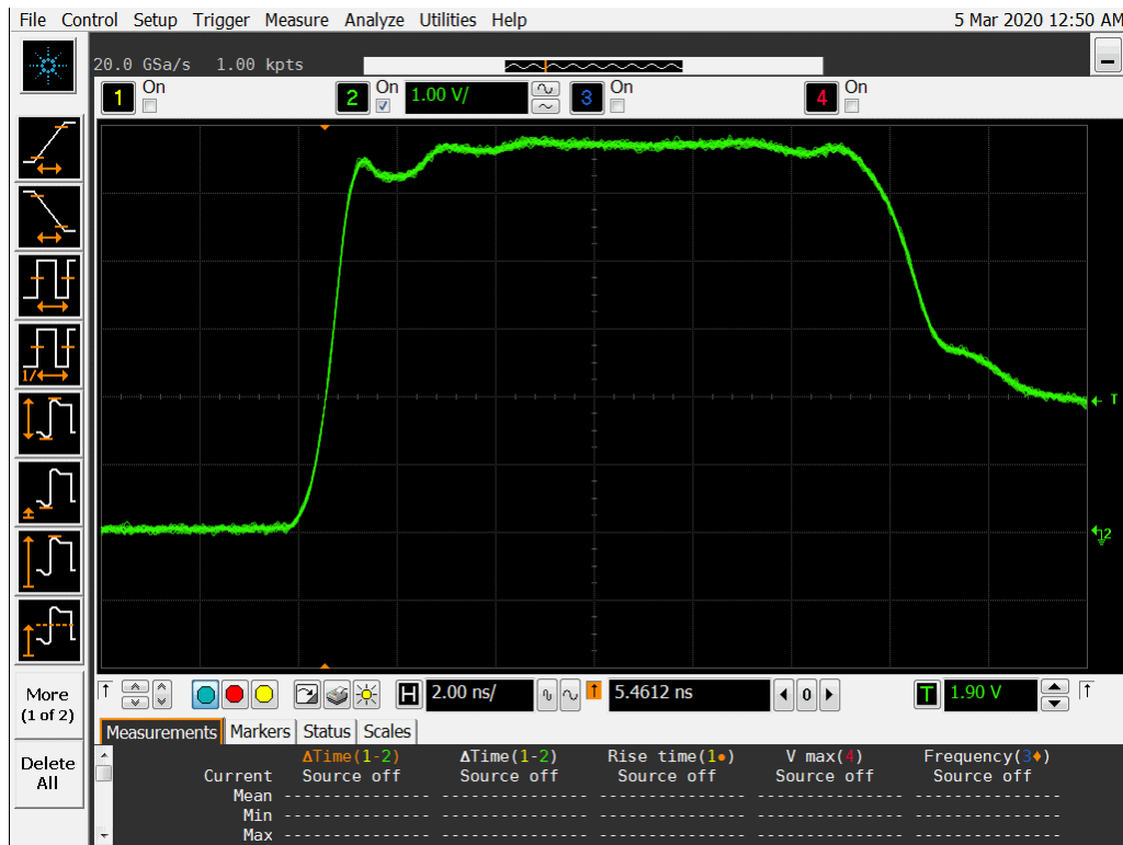
Figure 13a DUT 14035 Pre-Irradiation Rising Edge
