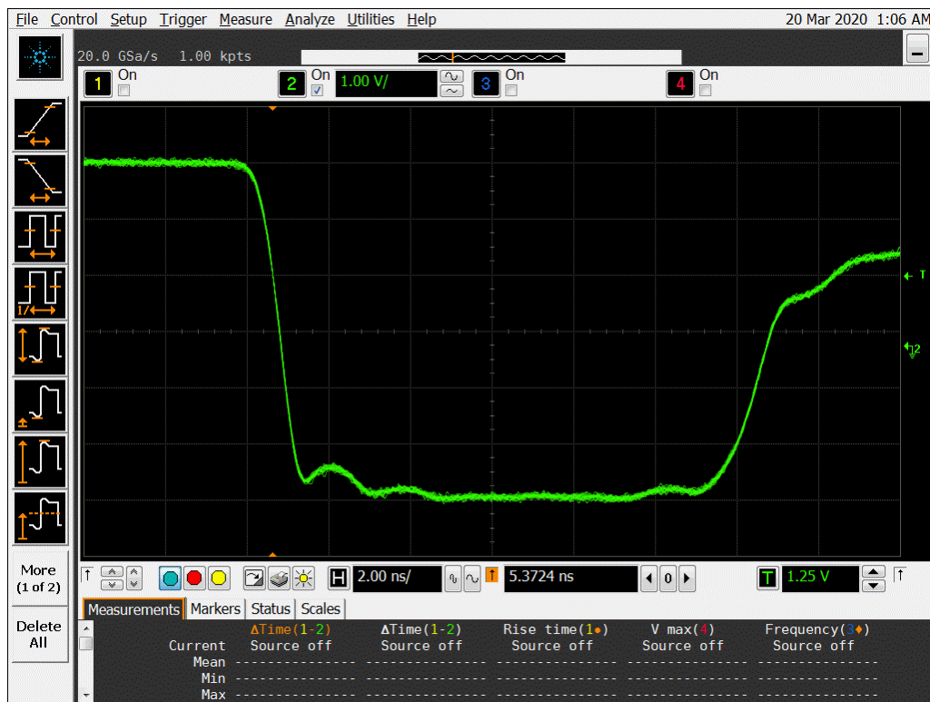
Figure 19b DUT 14035 Post-Annealing Falling Edge
