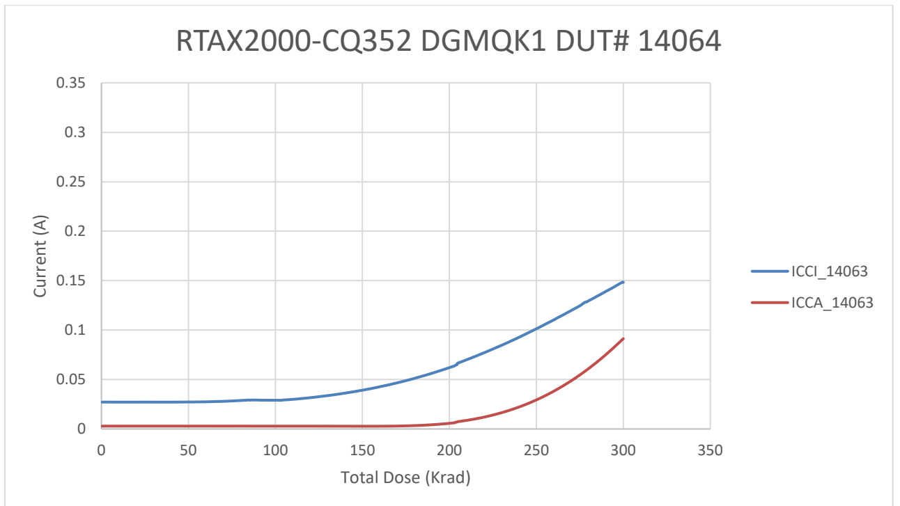
Figure 3 DUT 14064 Influx ICCA and ICCI
