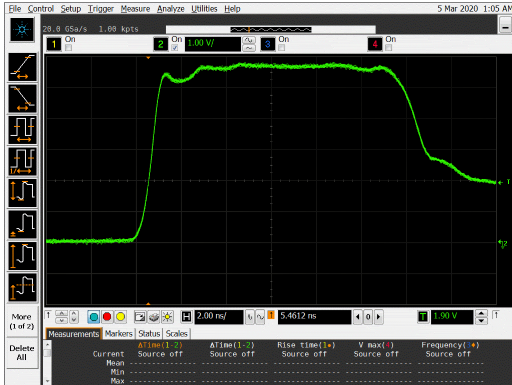
Figure 12a DUT 14062 Pre-Irradiation Rising Edge
