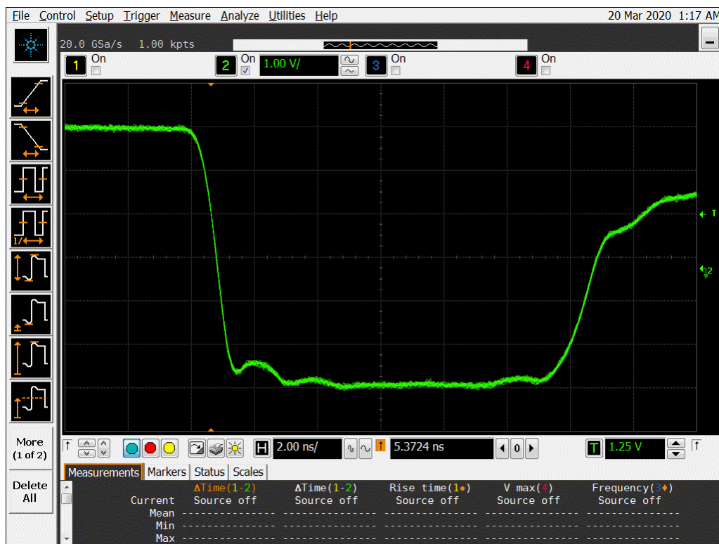
Figure 16b DUT 14064 Post-Annealing Falling Edge
