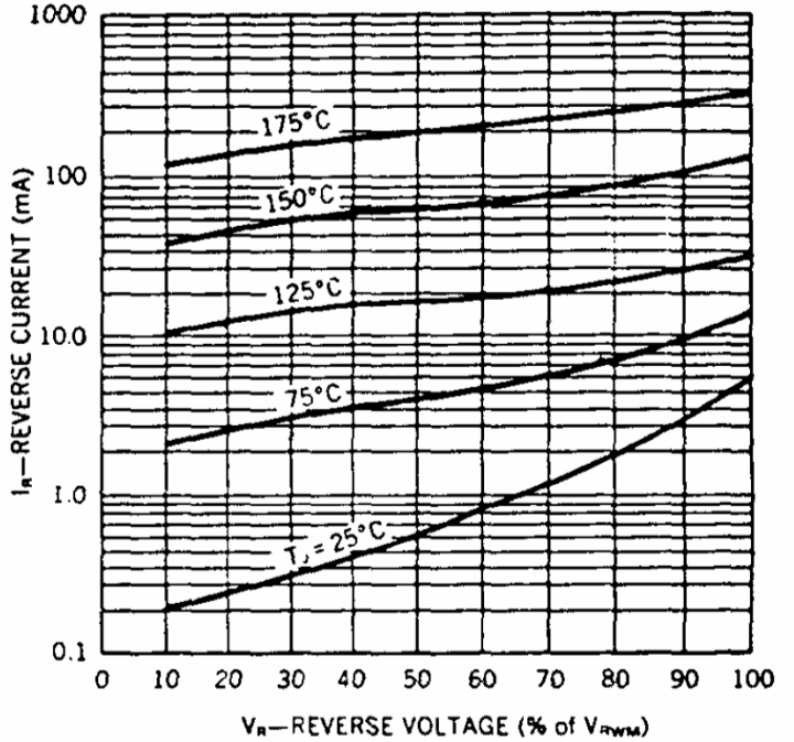
Typical Reverse Current vs Reverse Voltage
