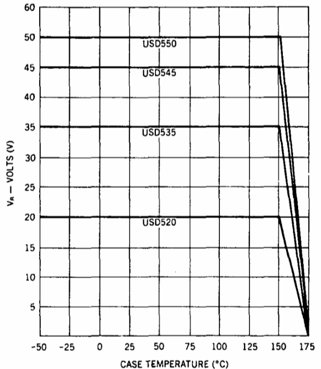
V R(MAX) Rating vs Case Temperature
