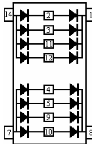
CIRCUIT CONFIGURATION
