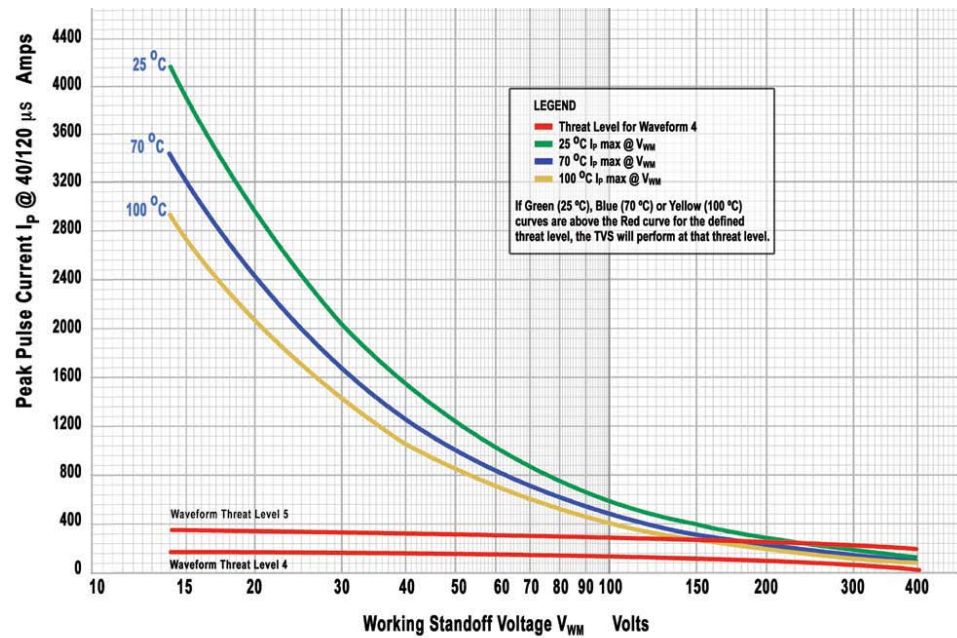
Graph 10: RTCA/DO-160G, Waveform 4, Levels 4 through 5, 30000 W TVS Series
