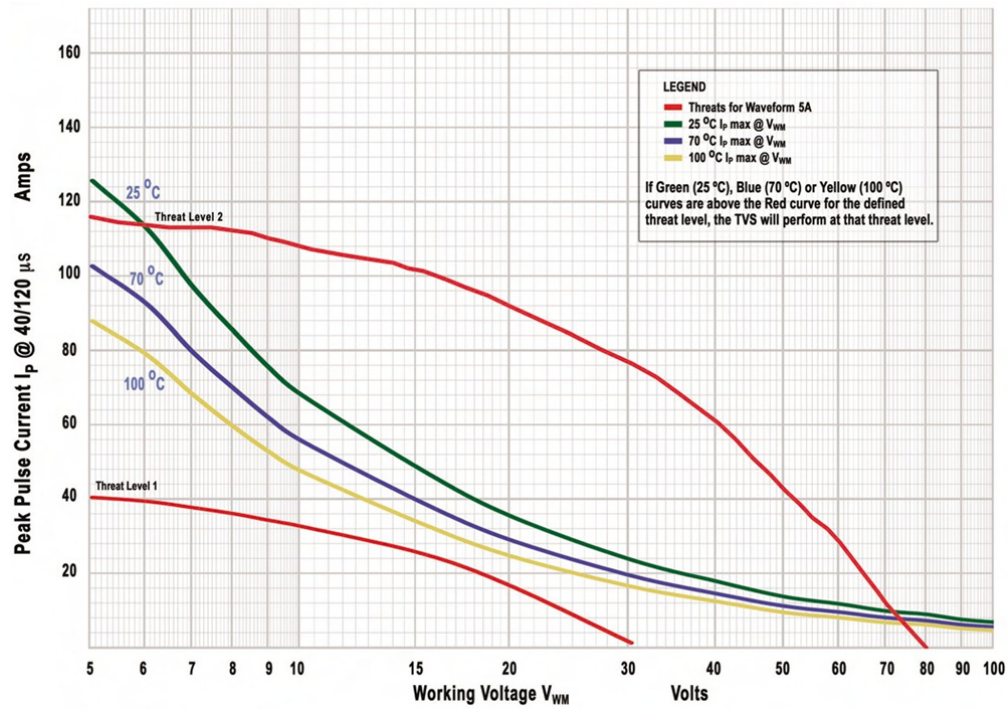
Graph 12: RTCA/DO-160G, Waveform 5A, Levels 1 through 2, 500 W TVS Series
