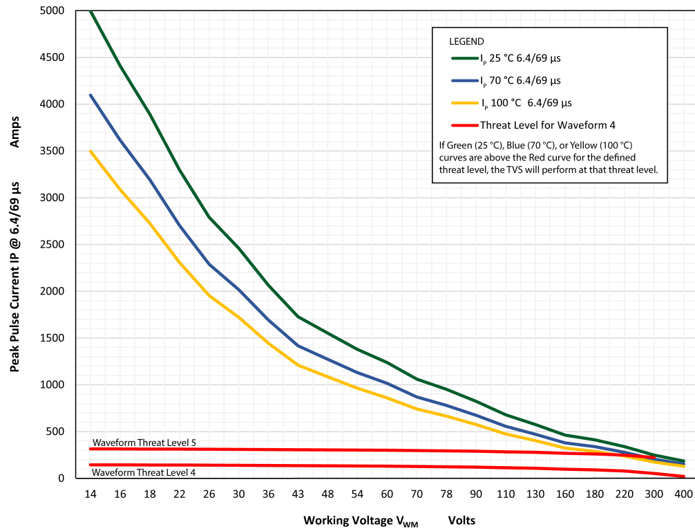
Graph 11: RTCA/DO-160, Waveform 4, Levels 4 through 5, Using 36,000 W TVS Diodes
