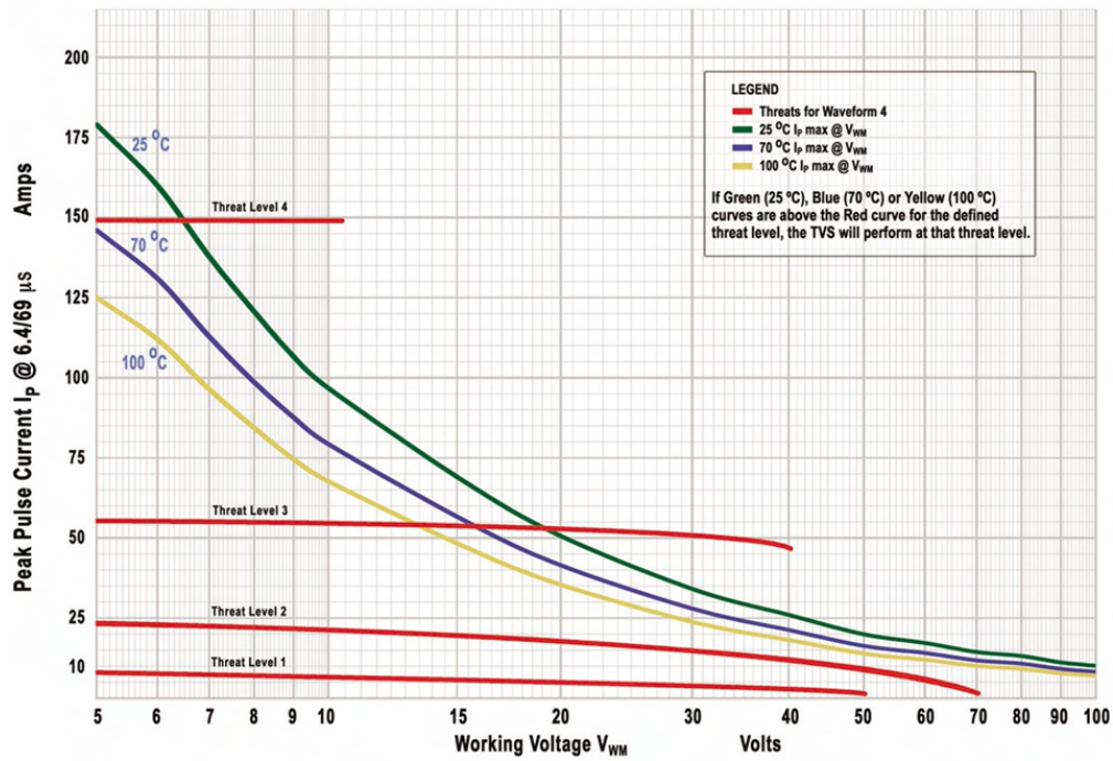
Graph 1: RTCA/DO-160G, Waveform 4, Levels 1 through 4, 500 W TVS Series
