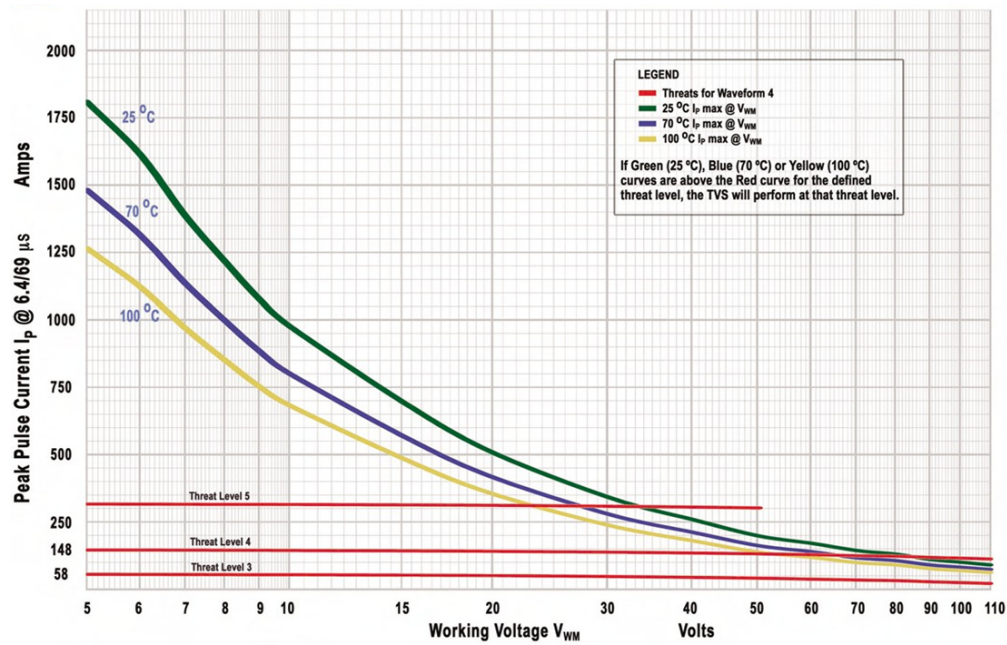
Graph 5: RTCA/DO-160G, Waveform 4, Levels 3 through 5, 5000 W TVS Series
