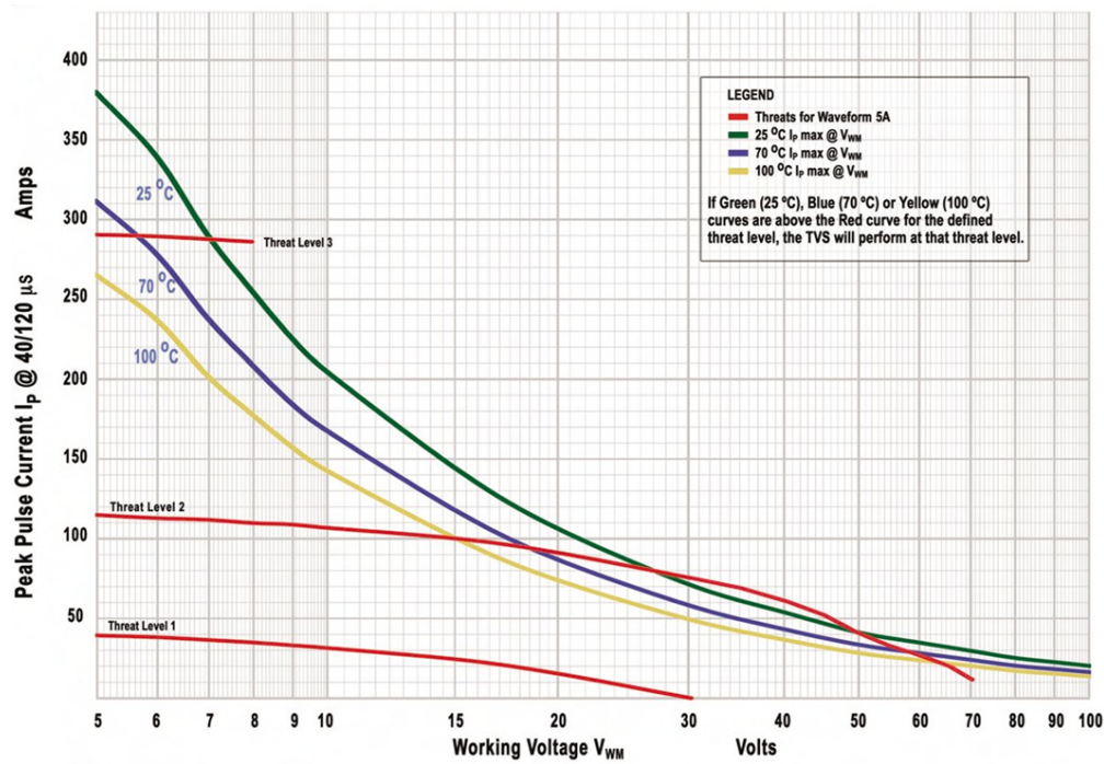
Graph 14: RTCA/DO-160G, Waveform 5A, Levels 1 through 3, 1500 W TVS Series
