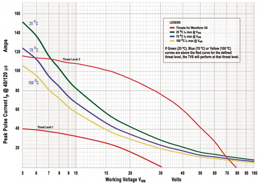
Graph 13: RTCA/DO-160G, Waveform 5A, Levels 1 through 2, 600 W TVS Series
