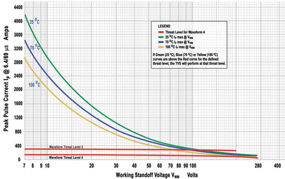
Graph 8: RTCA/DO-160G, Waveform 4, Levels 4 through 5, 15,000 W TVS Series
