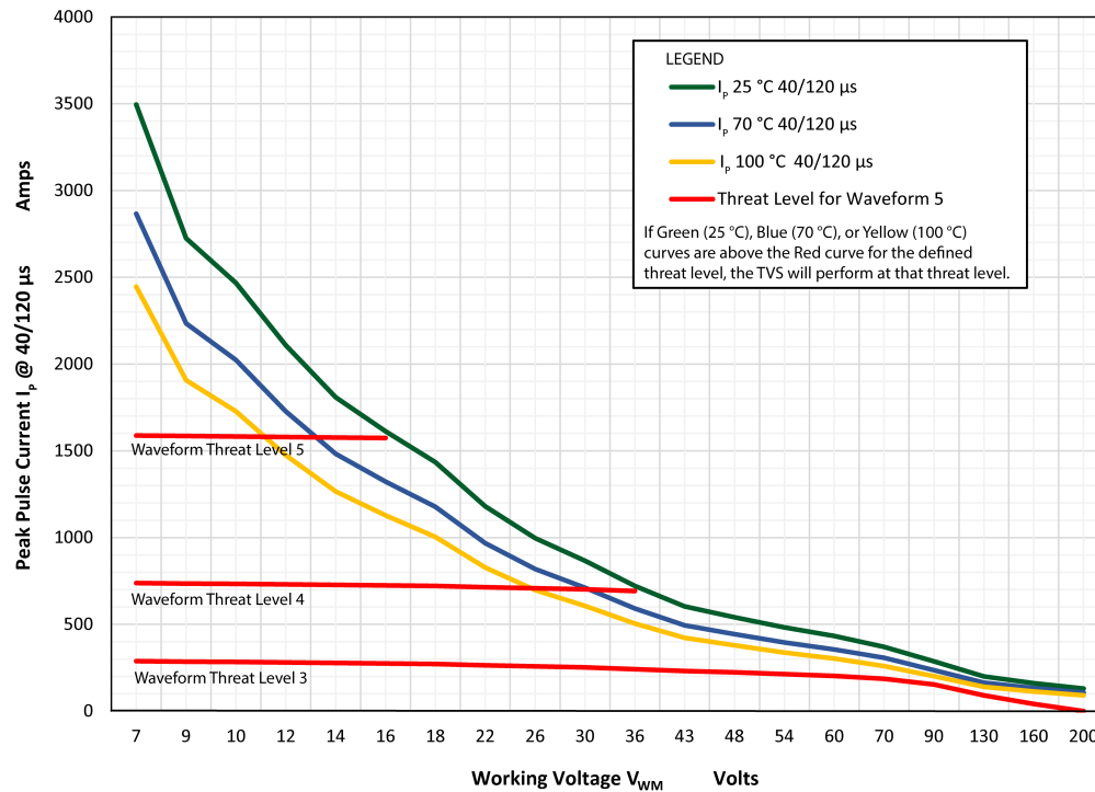
Graph 20: RTCA/DO-160, Waveform 5A, Levels 3 through 5, Using 18,000 W TVS Diodes
