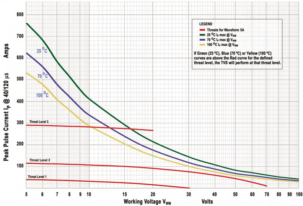
Graph 15: TVS Selection Guide for: RTCA/DO-160G, Waveform 5A, Levels 1 through 3, 3000 W TVS Series
