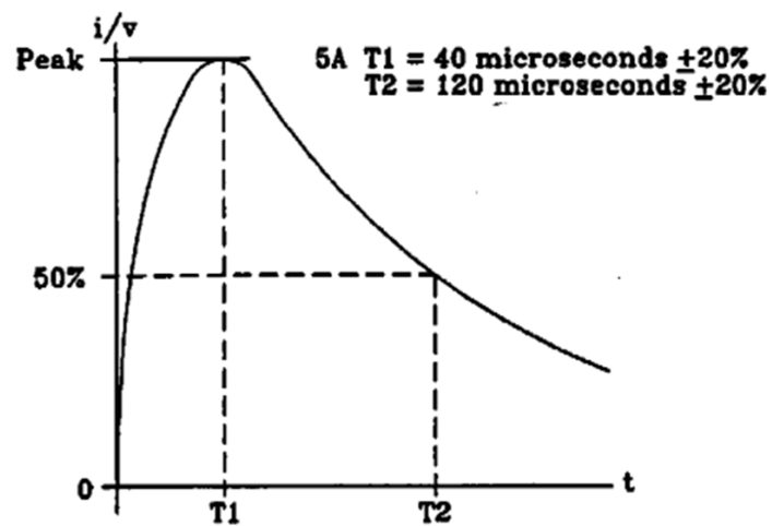
Figure 3 • Waveform 5A
