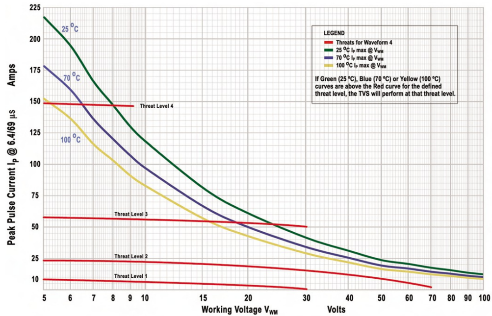
Graph 2: RTCA/DO-160G, Waveform 4, Levels 1 through 4, 600 W TVS Series
