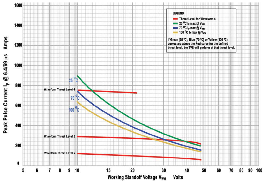
Graph 17: RTCA/DO-160, Waveform 5A, Levels 2 through 4, 6500 W TVS Series
