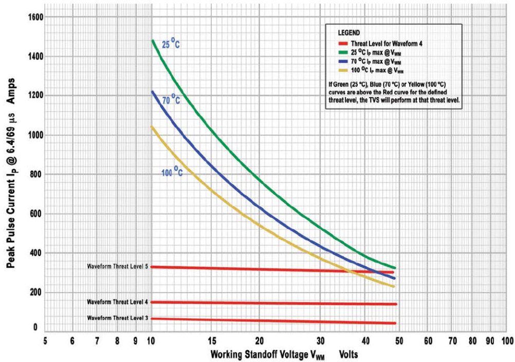
Graph 7: RTCA/DO-160, Waveform 4, Levels 3 through 5, 7500 W TVS Series
