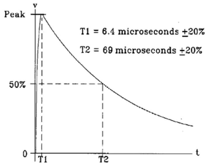
Figure 2 • Waveform 4
