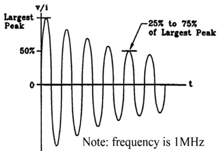
Figure 1 • Waveform 3
