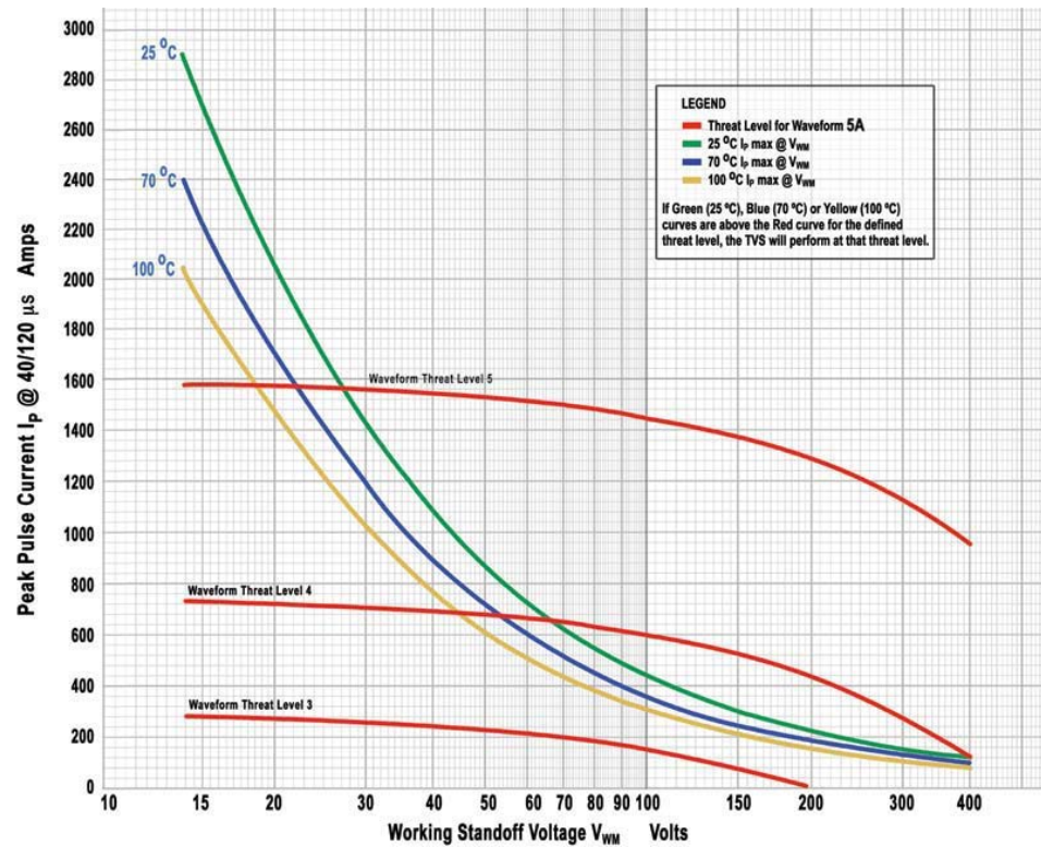
Graph 21: RTCA/DO-160G, Waveform 5A, Levels 3 through 5, 30000 W TVS Series
