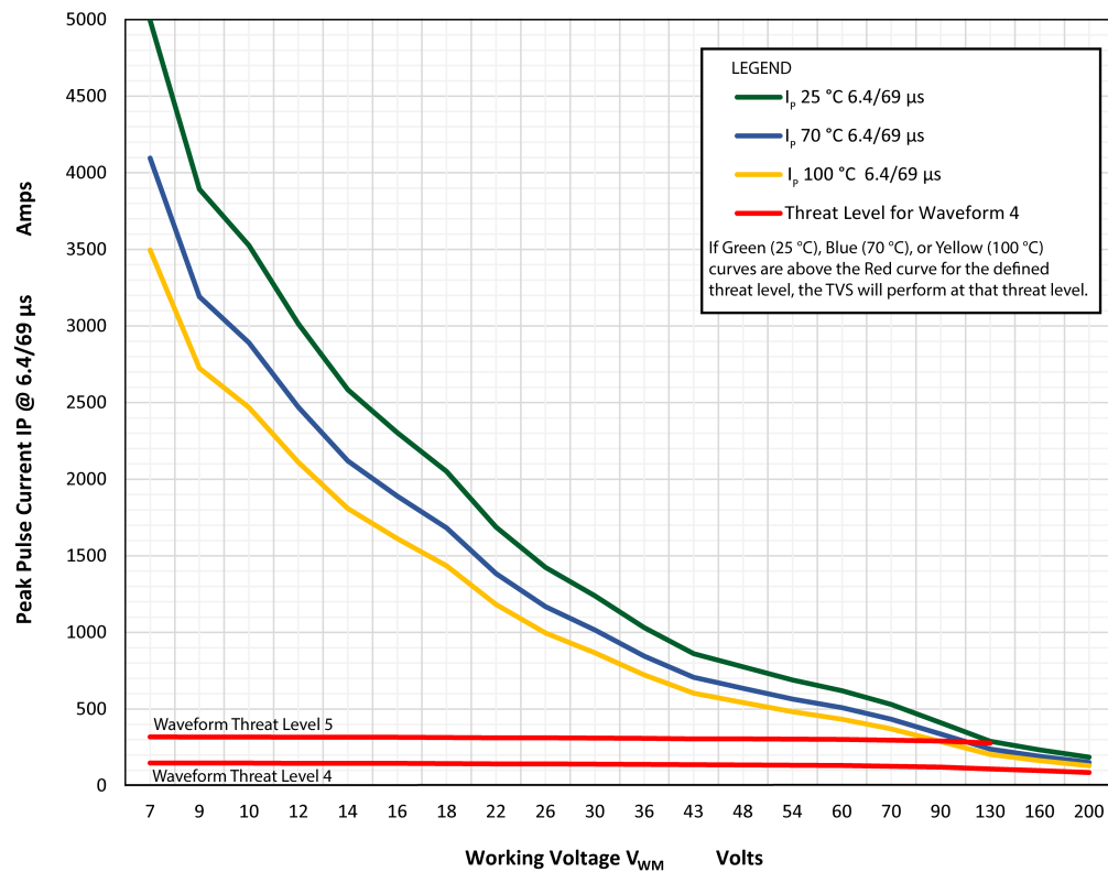
Graph 9: RTCA/DO-160, Waveform 4, Levels 4 through 5, 18,000 W TVS Diodes
