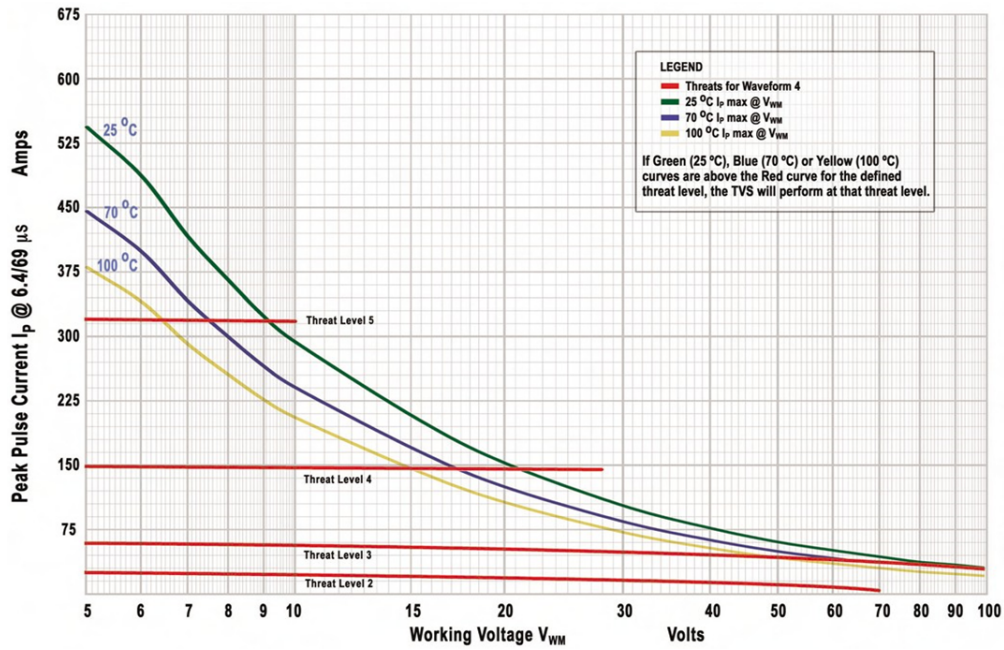
Graph 3: RTCA/DO-160G, Waveform 4, Levels 2 through 5, 1500 W TVS Series
