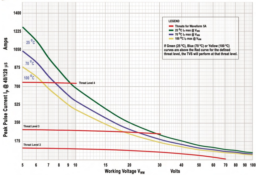
Graph 16: RTCA/DO-160G, Waveform 5A, Levels 2 through 4, 5000 W TVS Series
