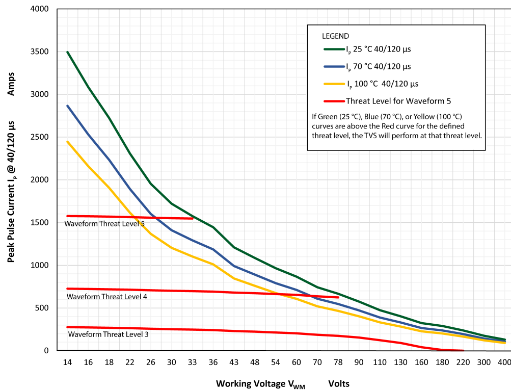
Graph 22: RTCA/DO-160, Waveform 5A, Levels 3 through 5, Using 36,000 W TVS Diodes
