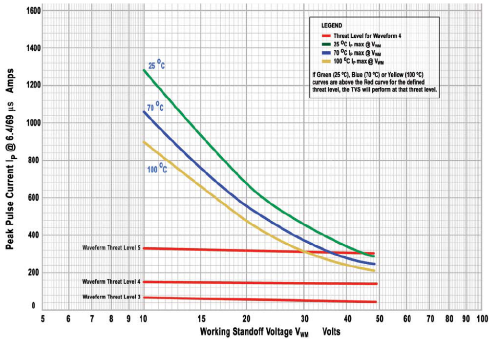
Graph 6: RTCA/DO-160, Waveform 4, Levels 3 through 5, 6500 W TVS Series
