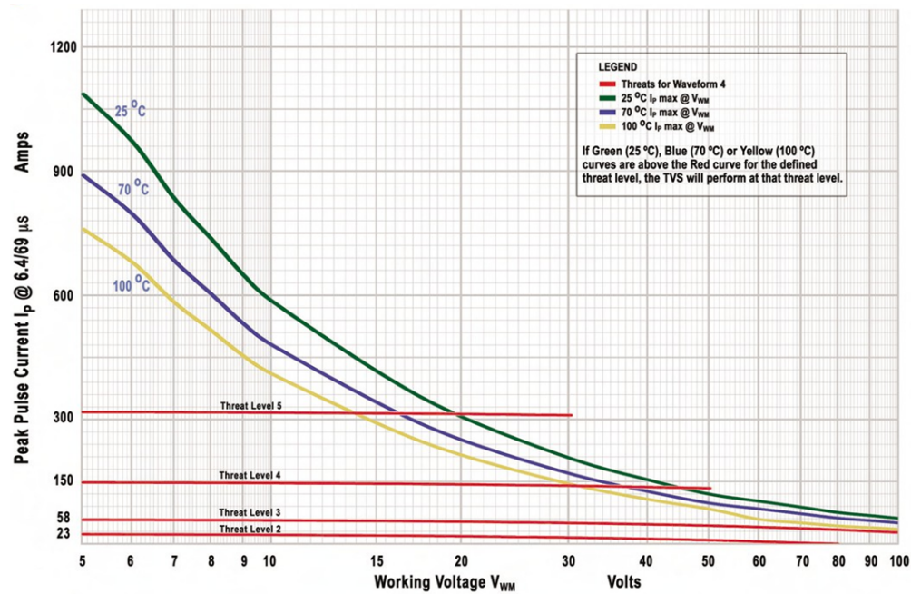
Graph 4: RTCA/DO-160G, Waveform 4, Levels 2 through 5, 3000 W TVS Series
