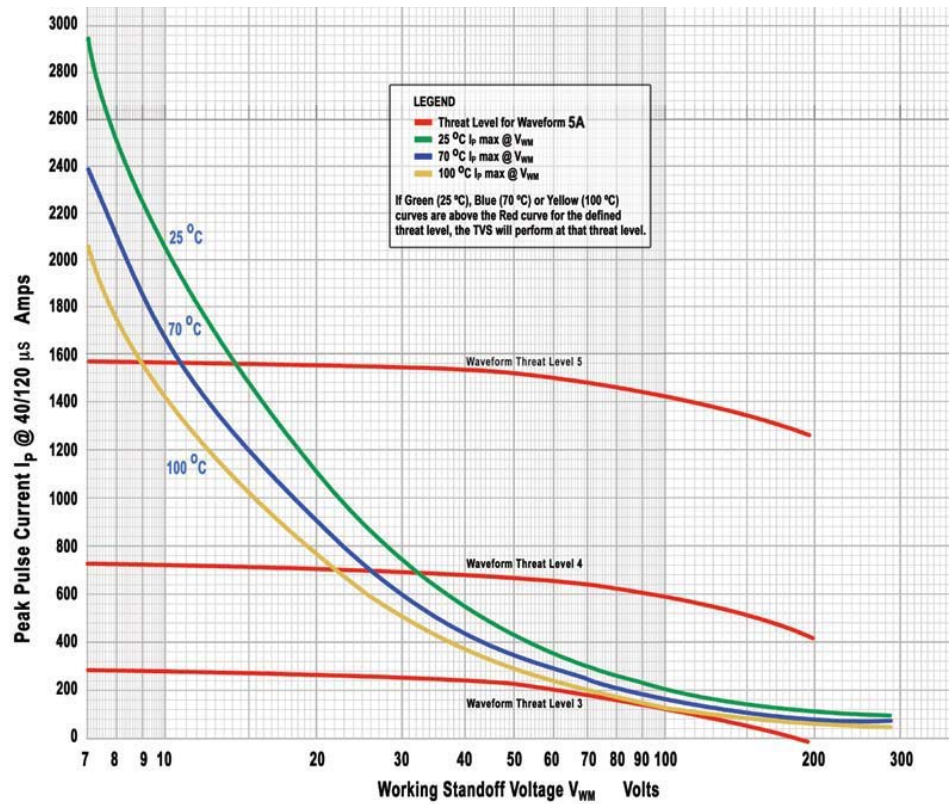
Data Points for Curves in Graph 19 - Waveform 5A RTCA/DO-160 using 15,000 W TVS Diodes
