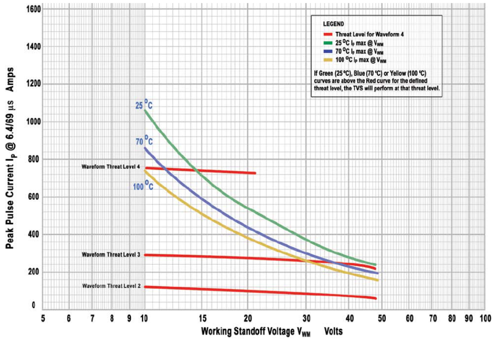
Graph 18: RTCA/DO-160, Waveform 5A, Levels 2 through 4, 7500 W TVS Series
