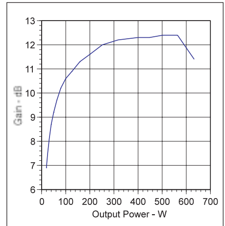
■ Figure 11. Gain of the amplifier during 50 percent duty cycle operation.
