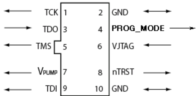
Figure 161 · FlashPro4 10-Pin Connector
