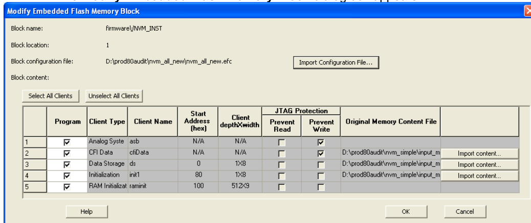
Figure 144 · Modify Embedded Flash Memory Block Content Dialog Box
