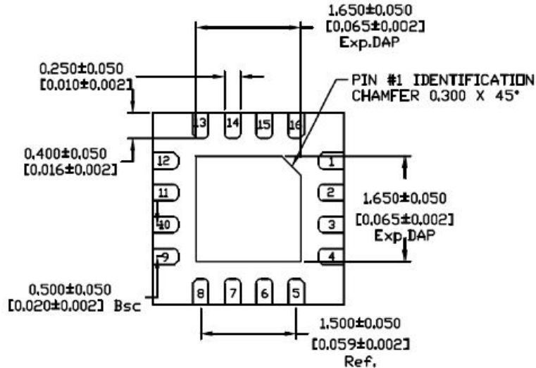
BOTTOM VIEW
