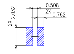
DETAIL e (12X)
