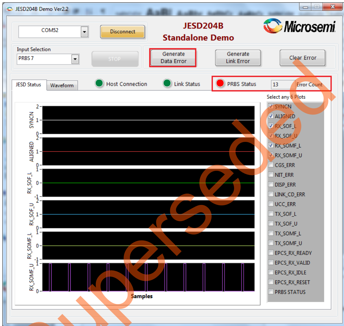
Figure 15 • Data Error Generation
