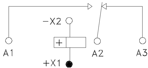
CIRCUIT
