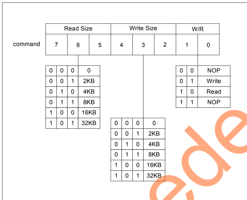
Figure 6 • Command Decoding
