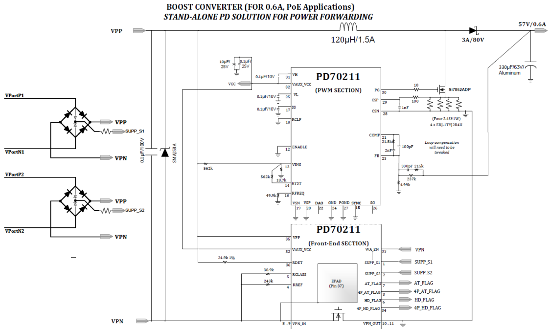
Figure 1 • Typical Applications Diagram
