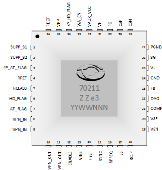
Figure 4 • PD70211 Pinout
