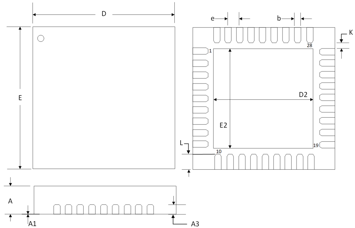
Figure 5 • QFN Package
