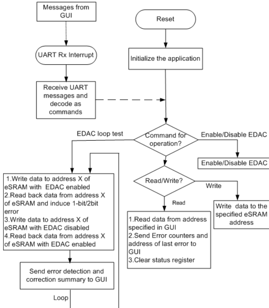
Figure 2. Design Flow
