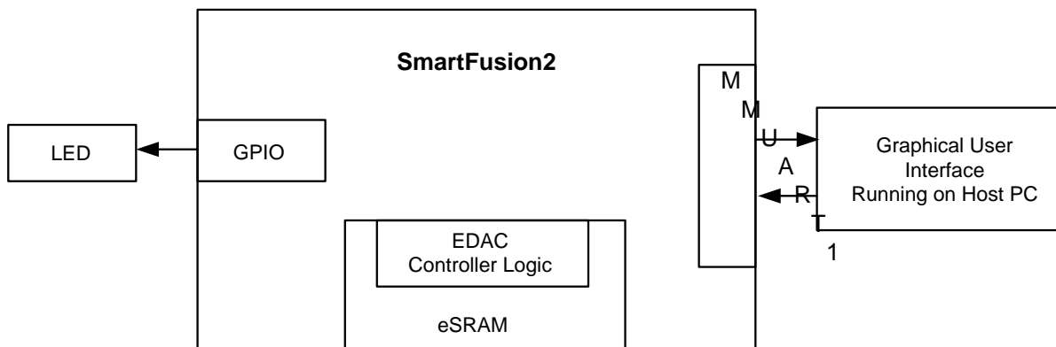
Figure 1. Top Level Block Diagram of the Demo
