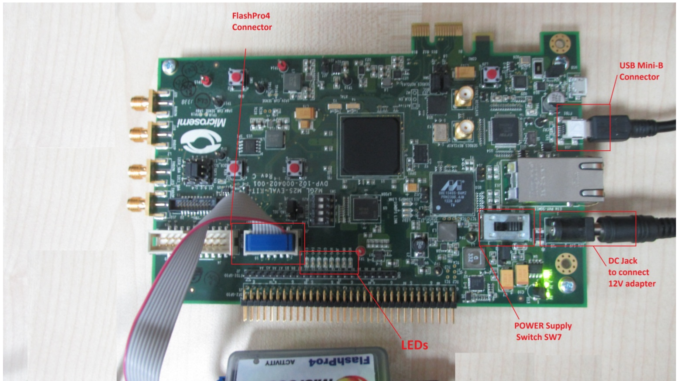
Figure 4. SmartFusion2 SoC FPGA Evaluation Kit Board Setup
