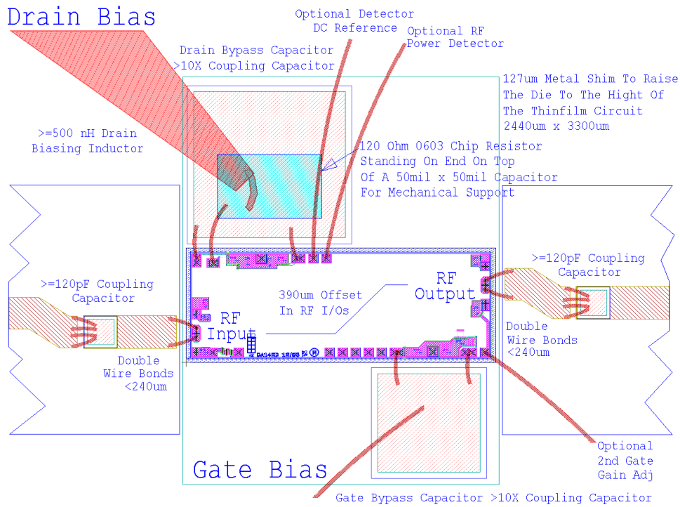
Figure 4. 40MHz - 30GHz bonding diagram
