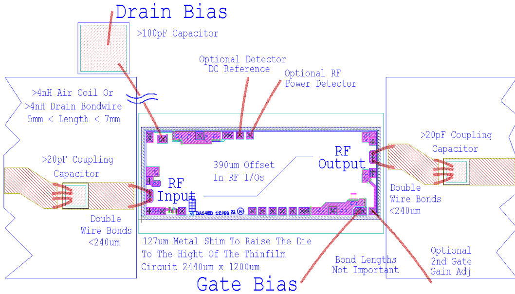
Figure 3.2 - 30GHz bonding diagram
