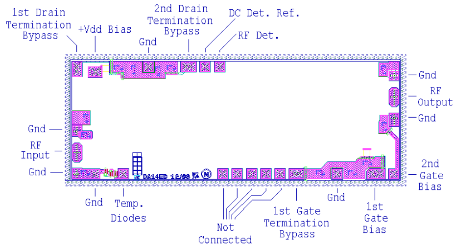
Figure 2. Pad Locations and Pad Descriptions
