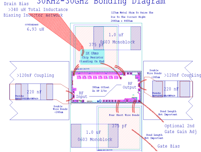
Figure 3. 30KHz-30GHz bonding diagram
