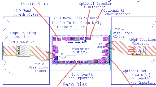
Figure 2. 2-30GHz bonding diagram
