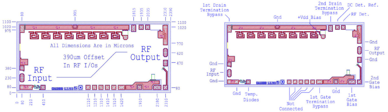
Figure 1. Die size, pad locations, and pad descriptions
