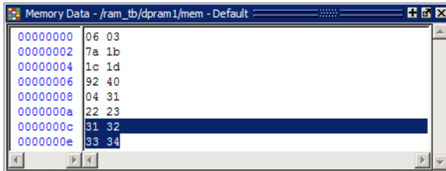
Figure 7-21. Changed Memory Contents for the Specified Addresses
