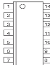
14 Pin Package
