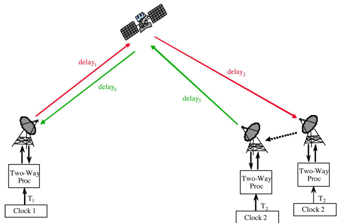
FIG.2 Dynamic Two-Way Time Transfer Configuration
