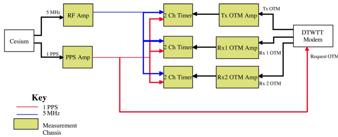
FIG.5 Measurement Chassis Hardware
