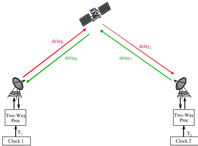
FIG.1 Static Two-Way Time Transfer
