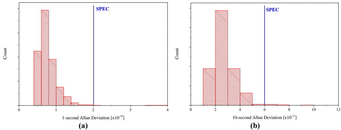
Figure 8: Variance of production SA.45s Allan deviation (a) \tau=1 s and (b) \tau=10 s
