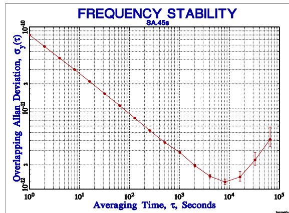
Figure 4: SA.45s typical short-term stability
