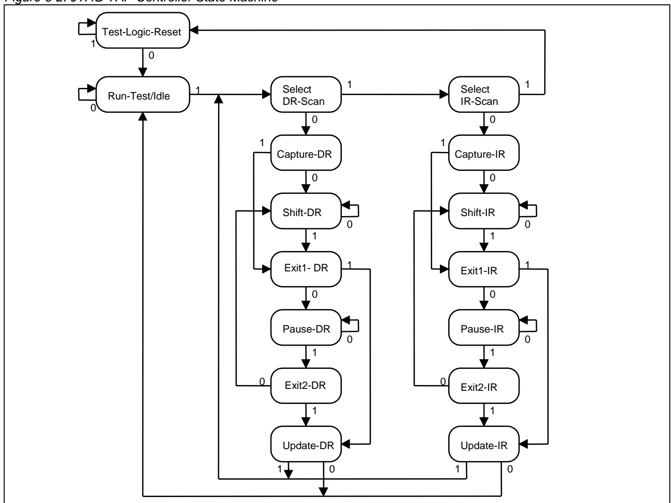
Figure 6-2. JTAG TAP Controller State Machine
