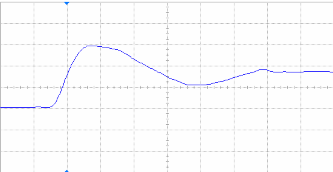
Figure 8(b) DUT 71864 post-annealing rising edge, abscissa scale is 2 V/div and ordinate scale is 2 ns/div.
