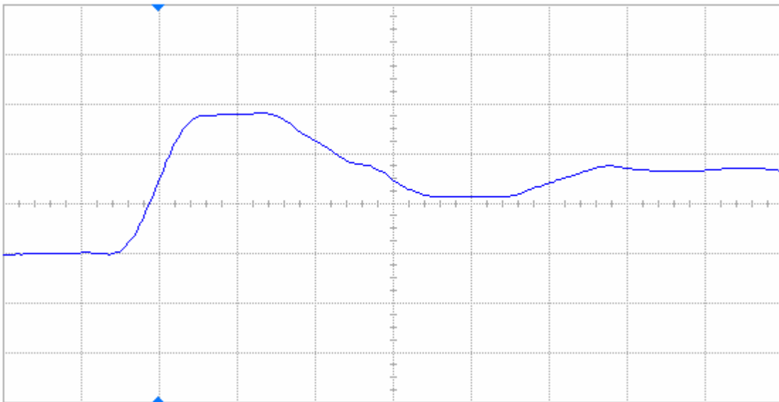
Figure 7(b) DUT 71833 post-annealing rising edge, abscissa scale is 2 V/div and ordinate scale is 2 ns/div.
