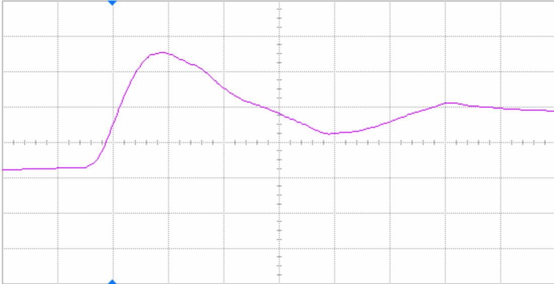
Figure 9(a) DUT 71865 pre-irradiation rising edge, abscissa scale is 2 V/div and ordinate scale is 2 ns/div.
