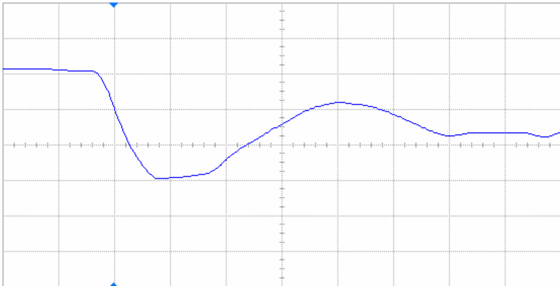
Figure 15(b) DUT 71885 post-annealing falling edge, abscissa scale is 2 V/div and ordinate scale is 2 ns/div.
