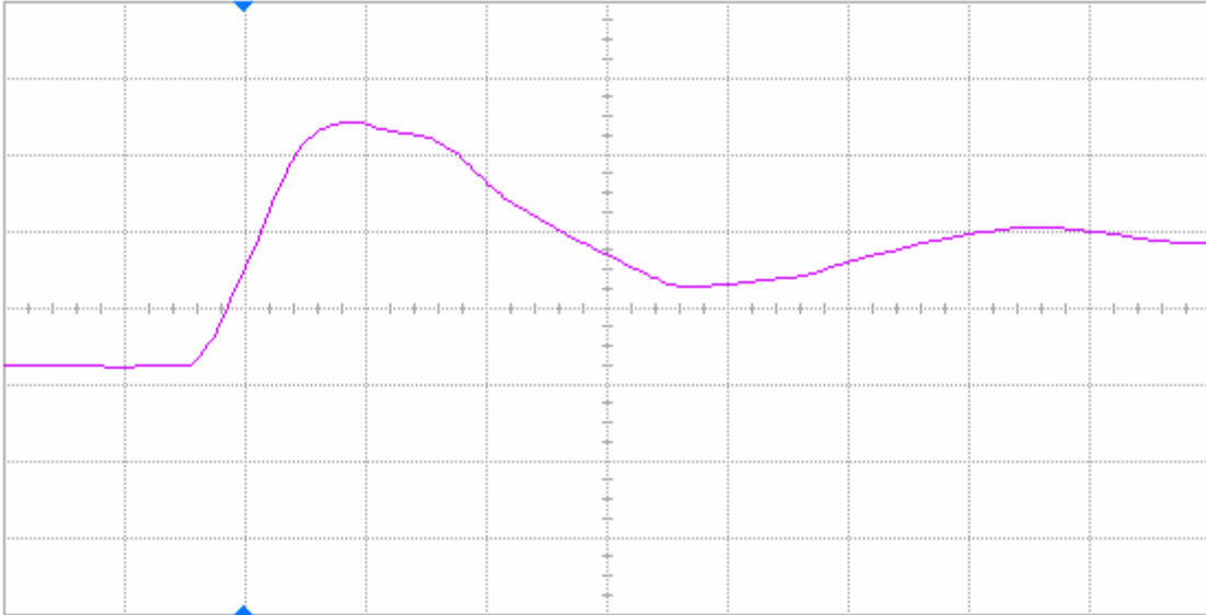
Figure 10(a) DUT 71885 pre-irradiation rising edge, abscissa scale is 2 V/div and ordinate scale is 2 ns/div.
