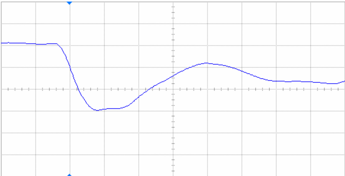
Figure 14(b) DUT 71865 post-annealing falling edge, abscissa scale is 2 V/div and ordinate scale is 2 ns/div.
