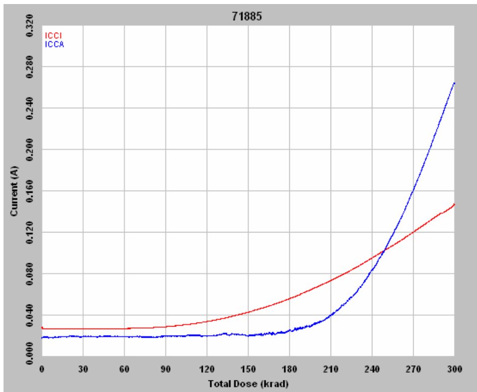
Figure 5 DUT 71885 in-flux I_{CCA} and I_{CCI}
