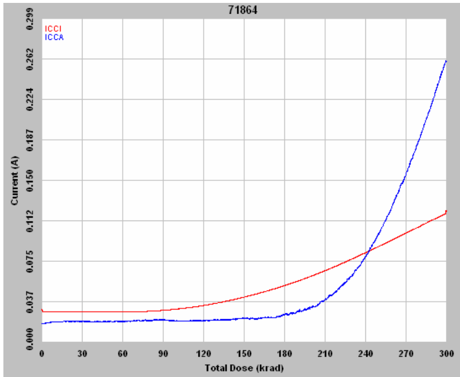
Figure 4 DUT 71864 in-flux I_{CCA} and I_{CCI}
