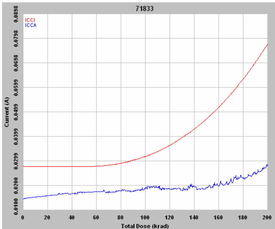
Figure 3 DUT 71833 in-flux I_{CCA} and I_{CCI}
