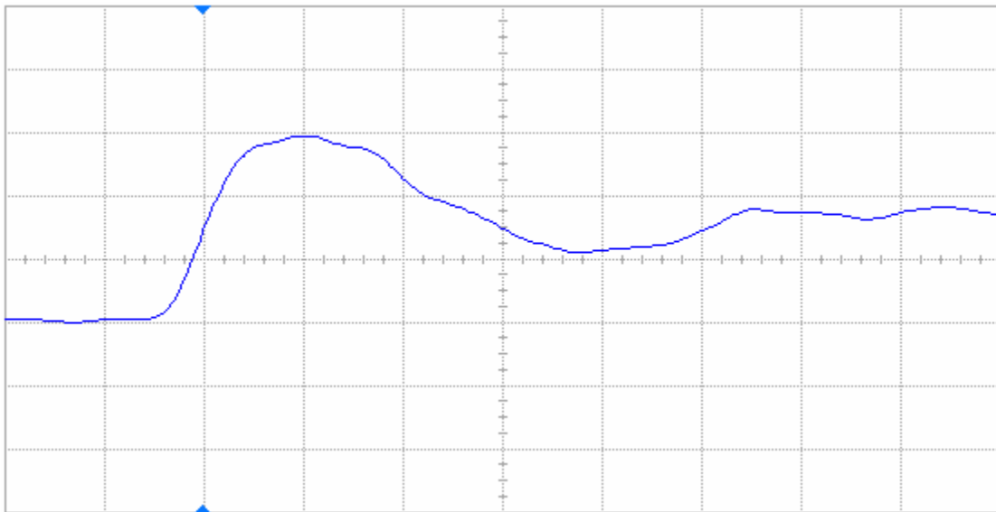
Figure 9(b) DUT 71865 post-annealing rising edge, abscissa scale is 2 V/div and ordinate scale is 2 ns/div.
