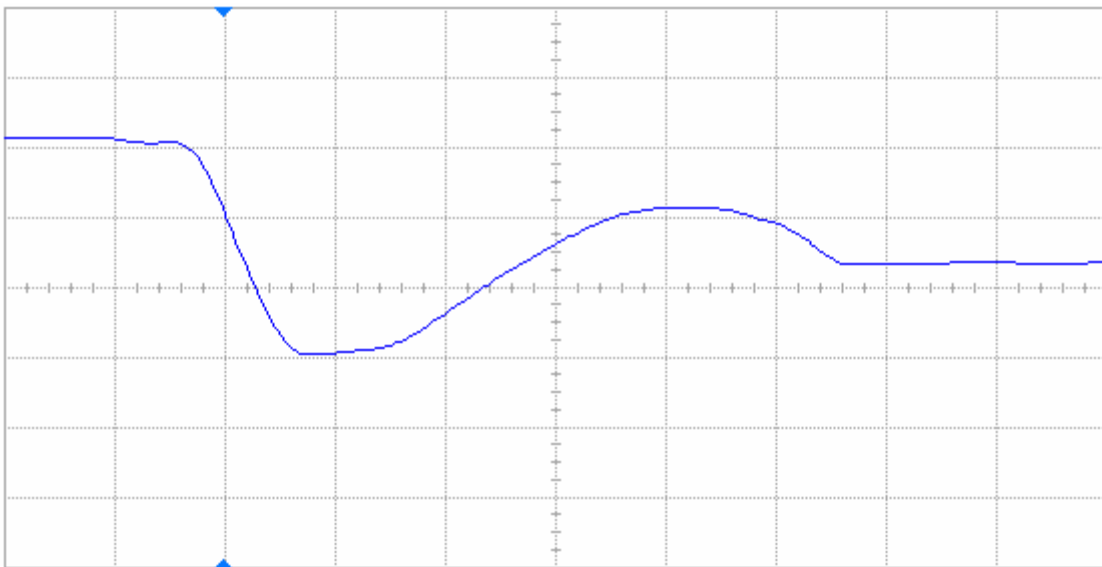
Figure 13(b) DUT 71864 post-annealing falling edge, abscissa scale is 2 V/div and ordinate scale is 2 ns/div.
