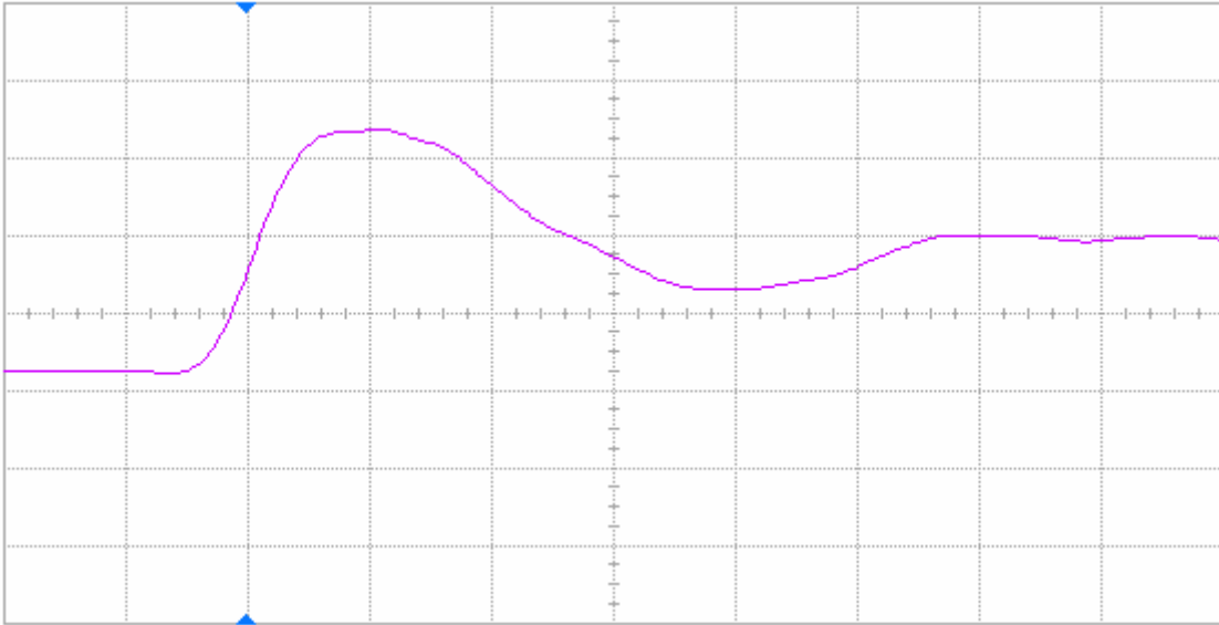
Figure 7(a) DUT 71833 pre-radiation rising edge, abscissa scale is 2 V/div and ordinate scale is 2 ns/div.
