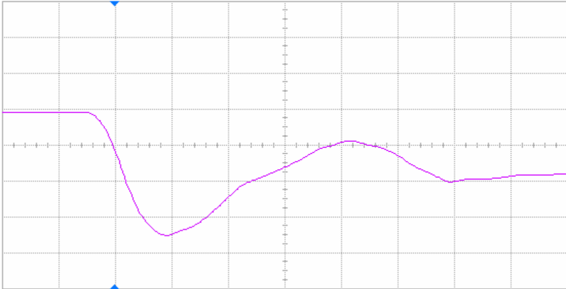
Figure 13(a) DUT 71864 pre-irradiation falling edge, abscissa scale is 2 V/div and ordinate scale is 2 ns/div.
