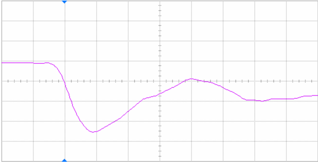
Figure 14(a) DUT 71865 pre-irradiation falling edge, abscissa scale is 2 V/div and ordinate scale is 2 ns/div.
