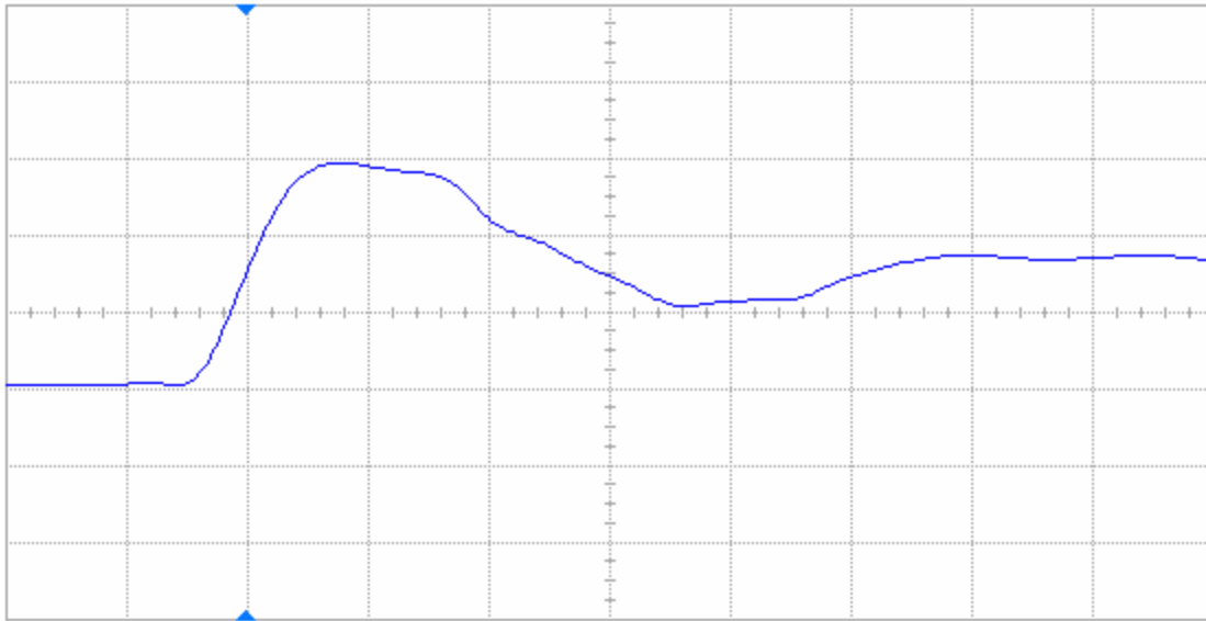
Figure 6 DUT 71808 post-annealing rising edge, abscissa scale is 2 V/div and ordinate scale is 2 ns/div.
