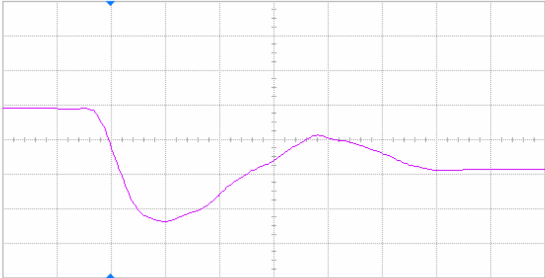
Figure 12(a) DUT 71833 pre-irradiation falling edge, abscissa scale is 2 V/div and ordinate scale is 2 ns/div.
