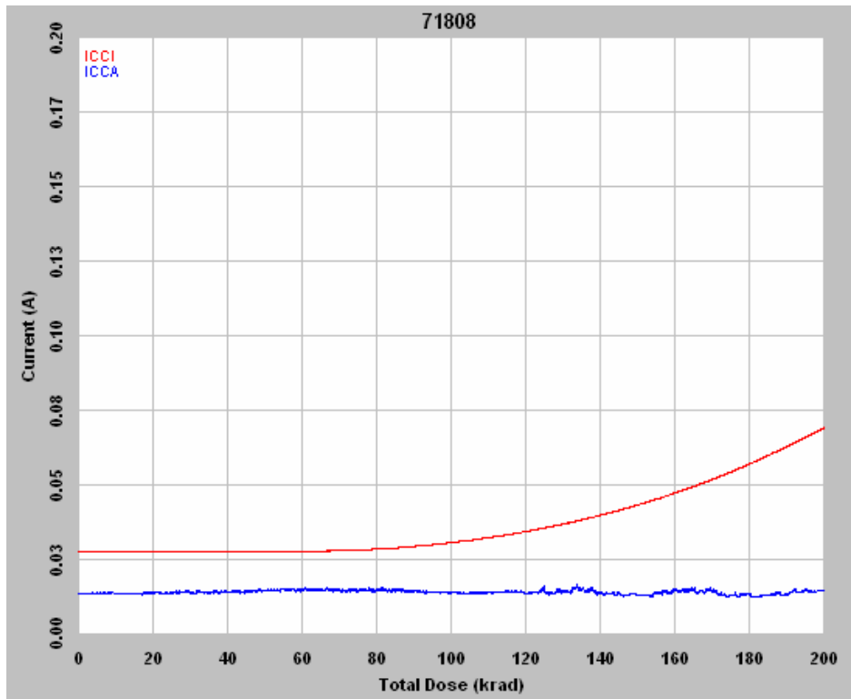
Figure 2 DUT 71808 in-flux I_{CCA} and I_{CCI}
