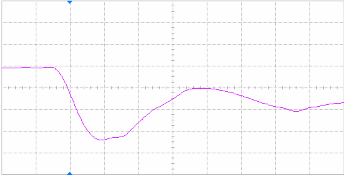
Figure 15(a) DUT 71885 pre-irradiation falling edge, abscissa scale is 2 V/div and ordinate scale is 2 ns/div.
