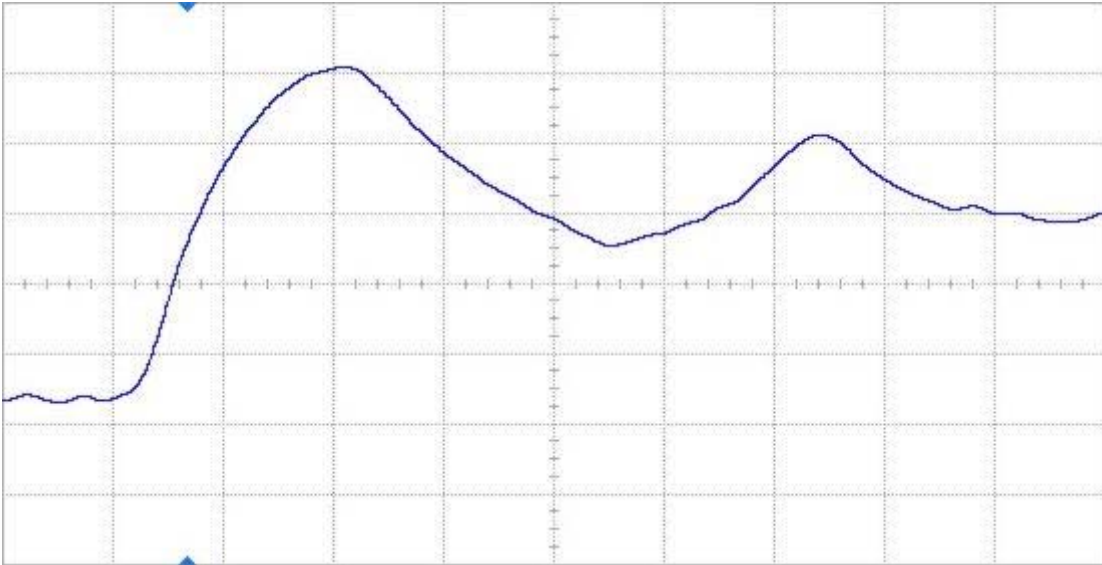
Figure 9(b) DUT 2567 post-annealing rising edge, abscissa scale is 1 V/div and ordinate scale is 2 ns/div.
