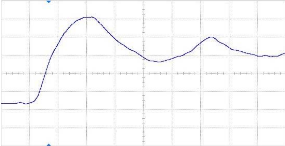
Figure 10(b) DUT 2593 post-annealing rising edge, abscissa scale is 1 V/div and ordinate scale is 2 ns/div.
