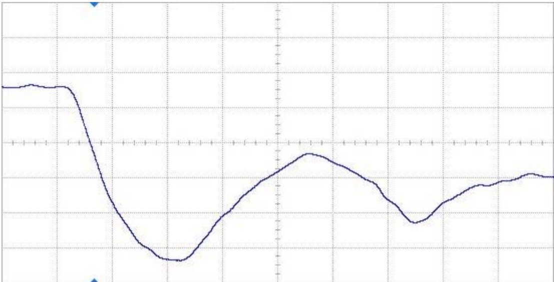
Figure 15(b) DUT 2567 post-annealing falling edge, abscissa scale is 1 V/div and ordinate scale is 2 ns/div.
