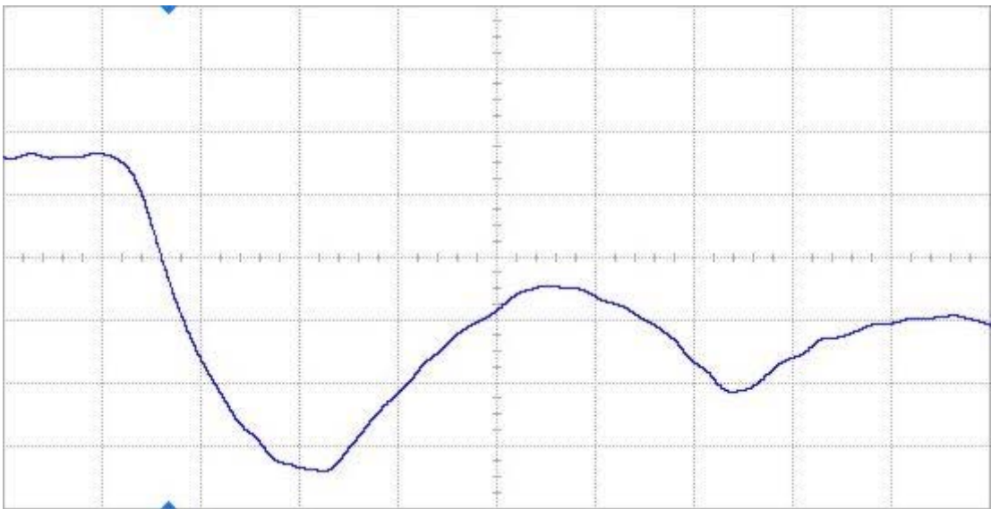
Figure 16(b) DUT 2593 post-annealing falling edge, abscissa scale is 1 V/div and ordinate scale is 2 ns/div.
