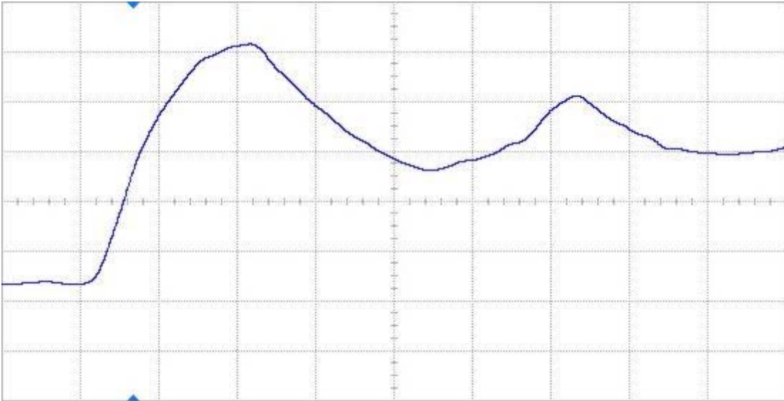
Figure 11(b) DUT 2601 post-annealing rising edge, abscissa scale is 1 V/div and ordinate scale is 2 ns/div.
