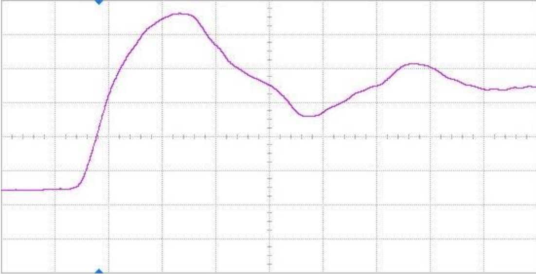
Figure 12(a) DUT 2602 pre-irradiation rising edge, abscissa scale is 1 V/div and ordinate scale is 2 ns/div.
