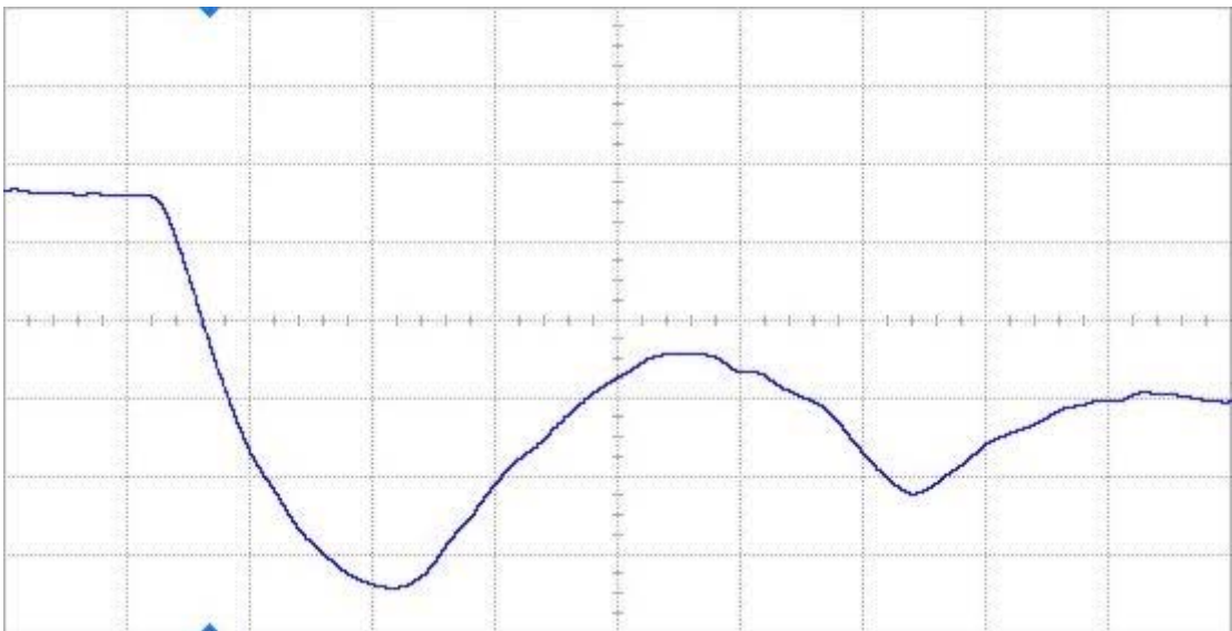
Figure 17(b) DUT 2601 post-annealing falling edge, abscissa scale is 1 V/div and ordinate scale is 2 ns/div.
