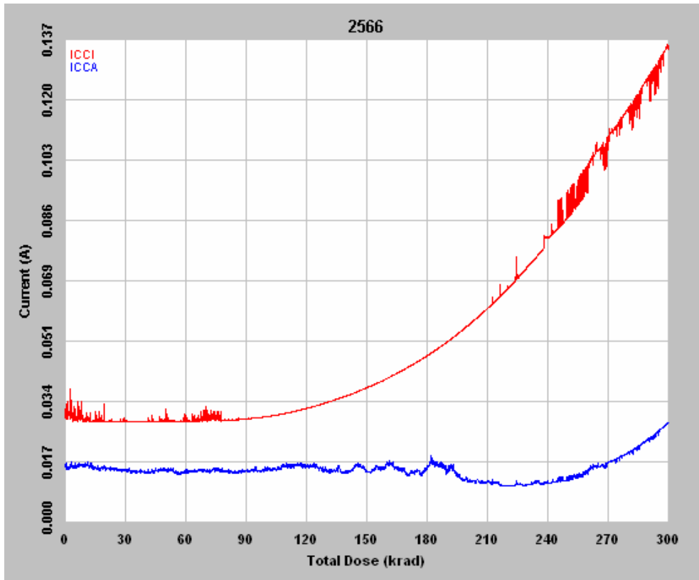
Figure 2 DUT 2566 in-flux I_{CCA} and I_{CCI}
