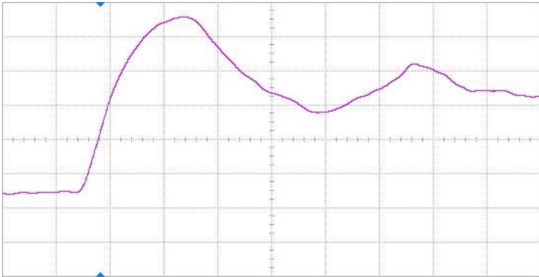
Figure 13(a) DUT 2610 pre-irradiation rising edge, abscissa scale is 1 V/div and ordinate scale is 2 ns/div.
