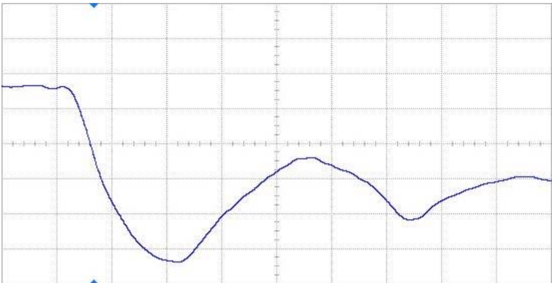
Figure 18(b) DUT 2602 post-annealing falling edge, abscissa scale is 1 V/div and ordinate scale is 2 ns/div.
