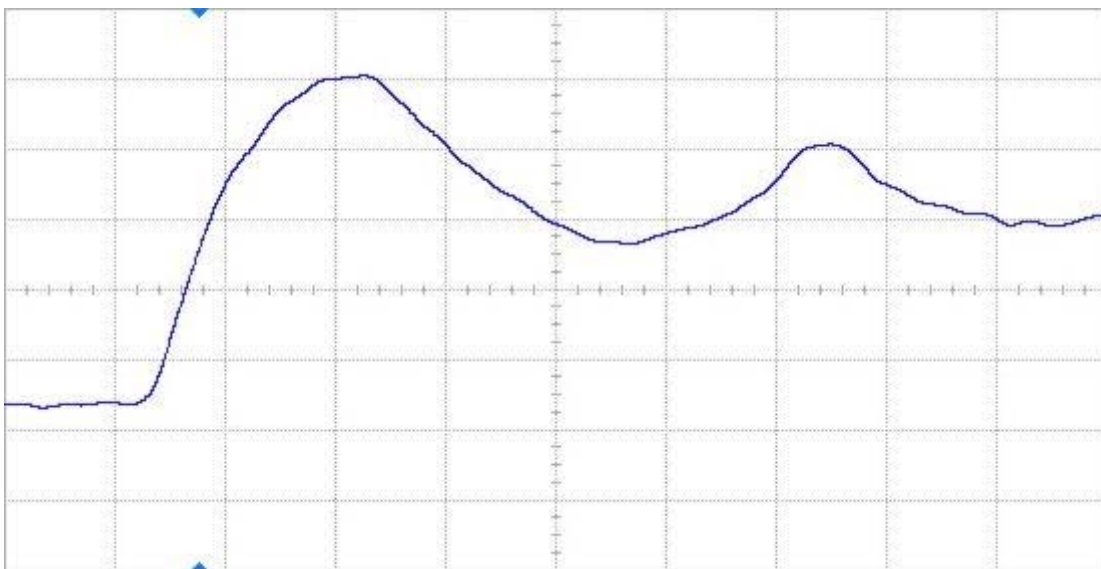
Figure 8(b) DUT 2566 post-annealing rising edge, abscissa scale is 1 V/div and ordinate scale is 2 ns/div.
