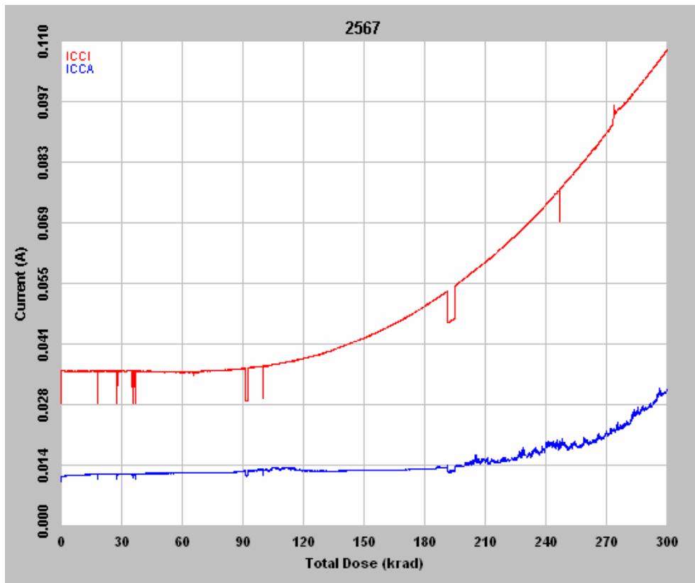
Figure 3 DUT 2567 in-flux I_{CCA} and I_{CCI}
