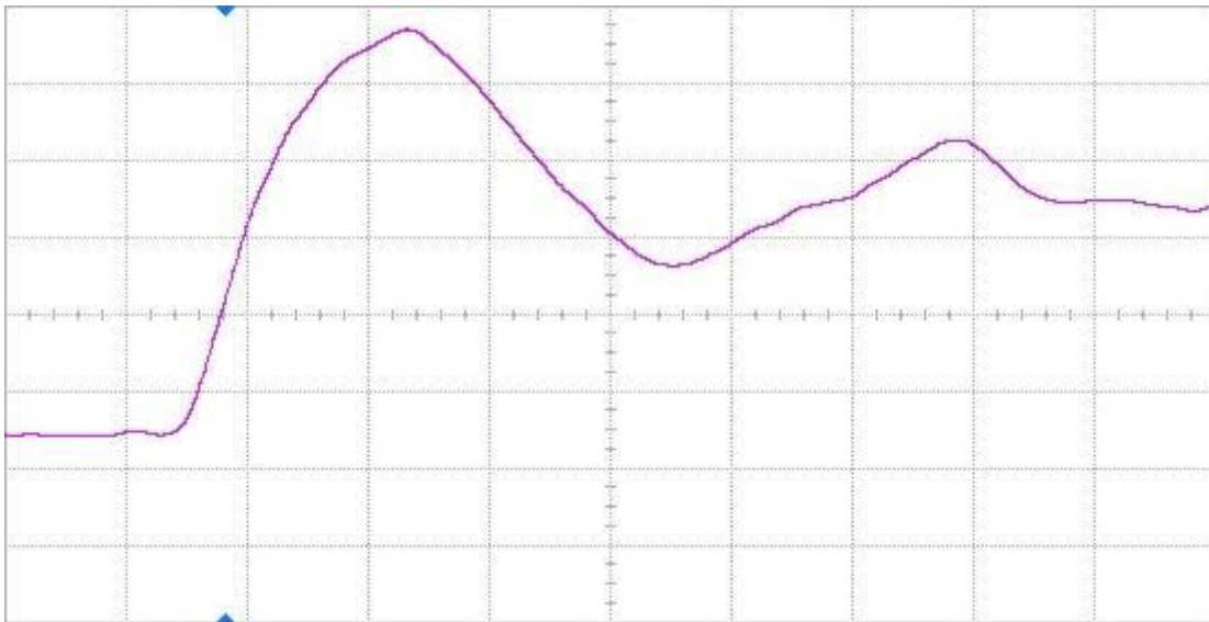
Figure 8(a) DUT 2566 pre-irradiation rising edge, abscissa scale is 1 V/div and ordinate scale is 2 ns/div.
