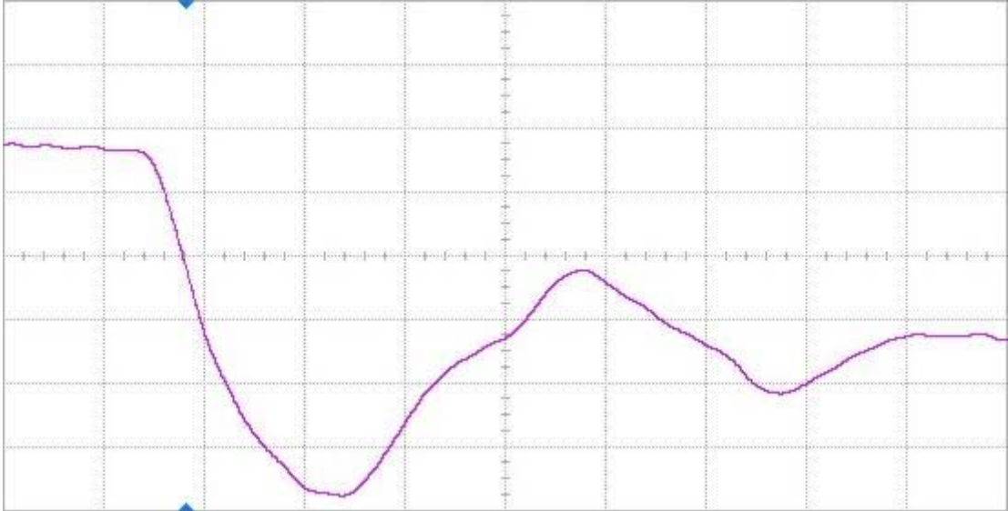
Figure 18(a) DUT 2602 pre-irradiation falling edge, abscissa scale is 1 V/div and ordinate scale is 2 ns/div.
