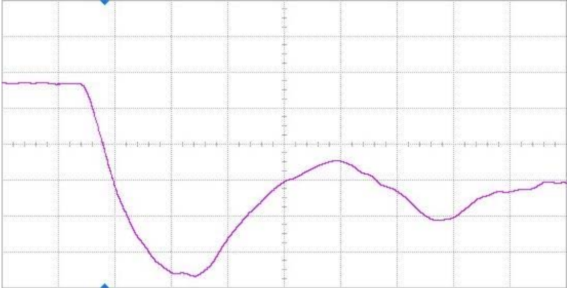
Figure 19(a) DUT 2610 pre-irradiation falling edge, abscissa scale is 1 V/div and ordinate scale is 2 ns/div.
