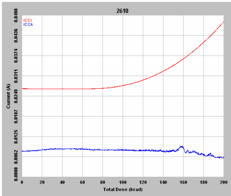
Figure 7 DUT 2610 in-flux I_{CCA} and I_{CCI}
