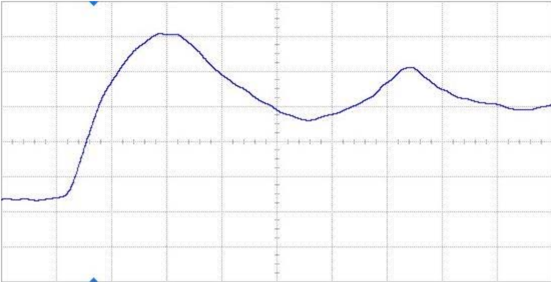
Figure 12(b) DUT 2602 post-annealing rising edge, abscissa scale is 1 V/div and ordinate scale is 2 ns/div.
