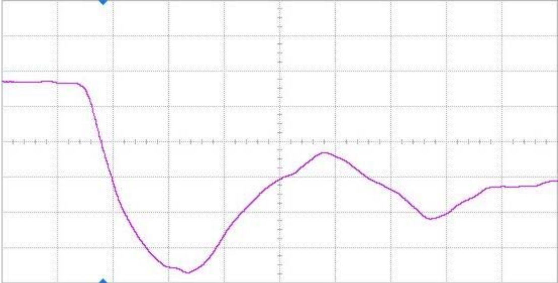
Figure 17(a) DUT 2601 pre-irradiation falling edge, abscissa scale is 1 V/div and ordinate scale is 2 ns/div.
