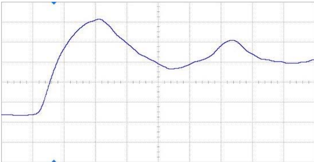
Figure 13(b) DUT 2610 post-annealing rising edge, abscissa scale is 1 V/div and ordinate scale is 2 ns/div.
