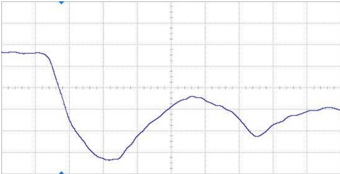
Figure 14(b) DUT 2566 post-annealing falling edge, abscissa scale is 1 V/div and ordinate scale is 2 ns/div.
