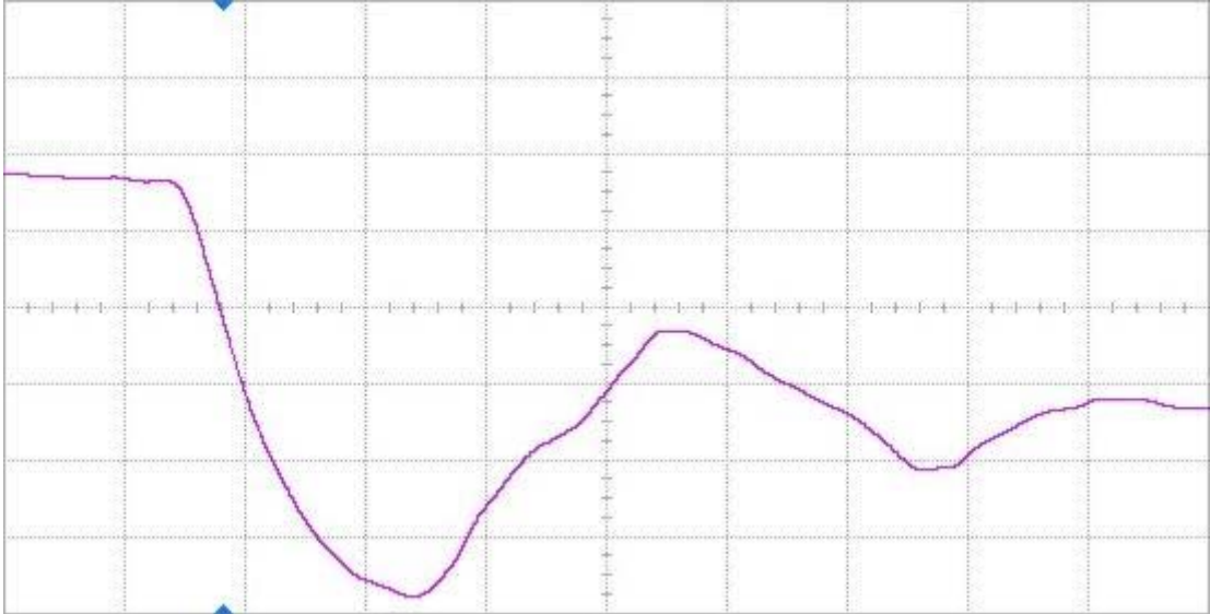
Figure 16(a) DUT 2593 pre-irradiation falling edge, abscissa scale is 1 V/div and ordinate scale is 2 ns/div.
