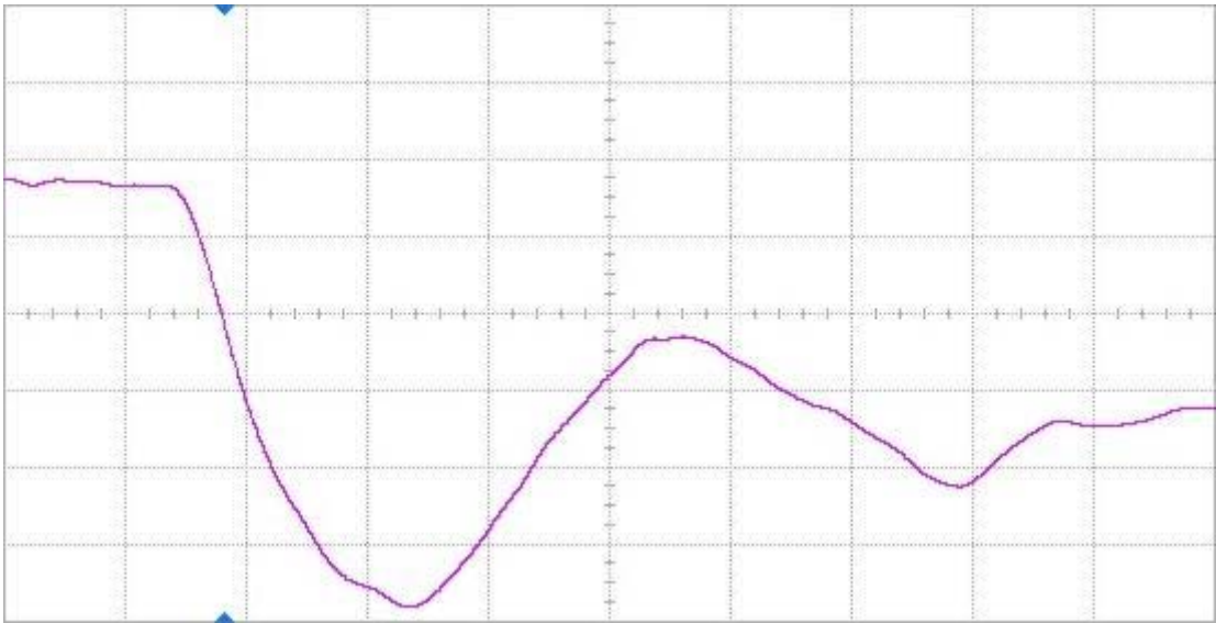
Figure 14(a) DUT 2566 pre-irradiation falling edge, abscissa scale is 1 V/div and ordinate scale is 2 ns/div.
