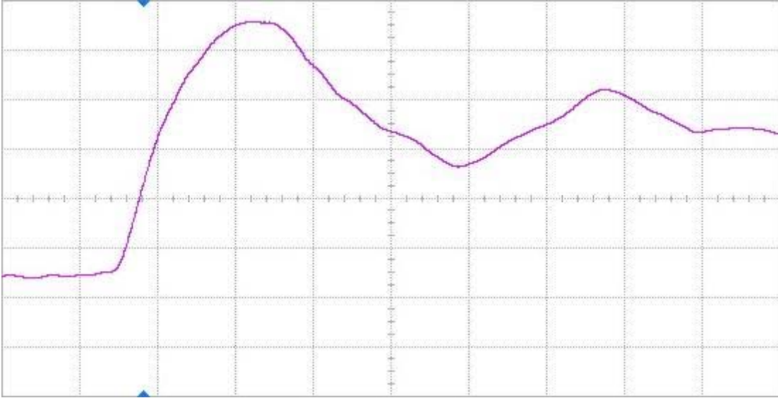
Figure 11(a) DUT 2601 pre-irradiation rising edge, abscissa scale is 1 V/div and ordinate scale is 2 ns/div.
