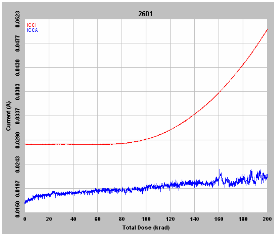
Figure 5 DUT 2601 in-flux I_{CCA} and I_{CCI}
