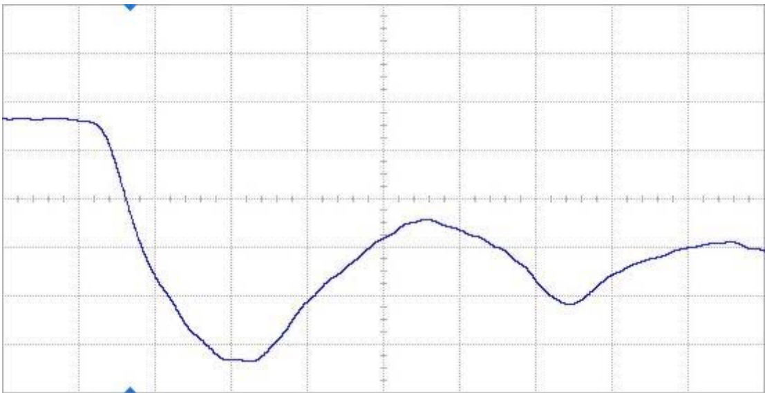
Figure 19(b) DUT 2610 post-annealing falling edge, abscissa scale is 1 V/div and ordinate scale is 2 ns/div.
