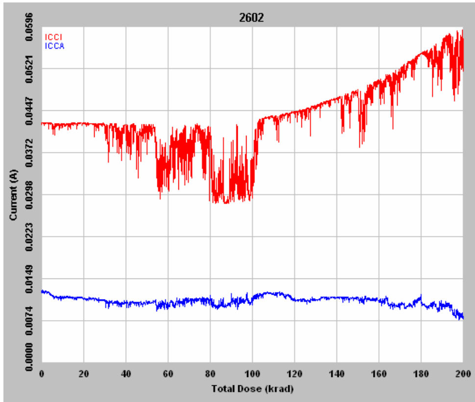
Figure 6 DUT 2602 in-flux I_{CCA} and I_{CCI}
