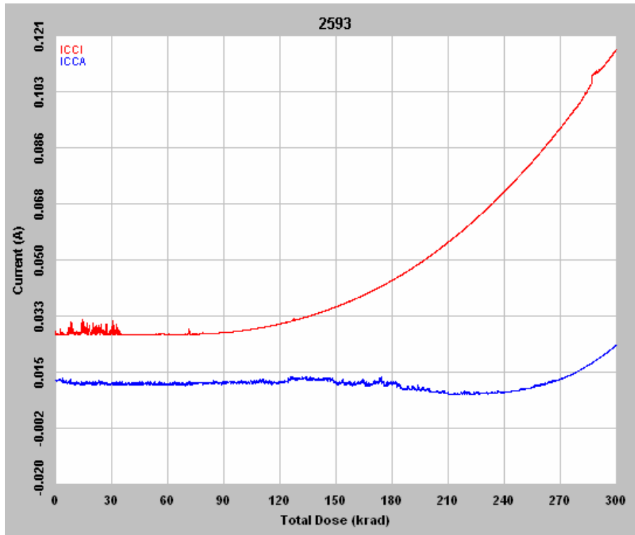
Figure 4 DUT 2593 in-flux I_{CCA} and I_{CCI}
