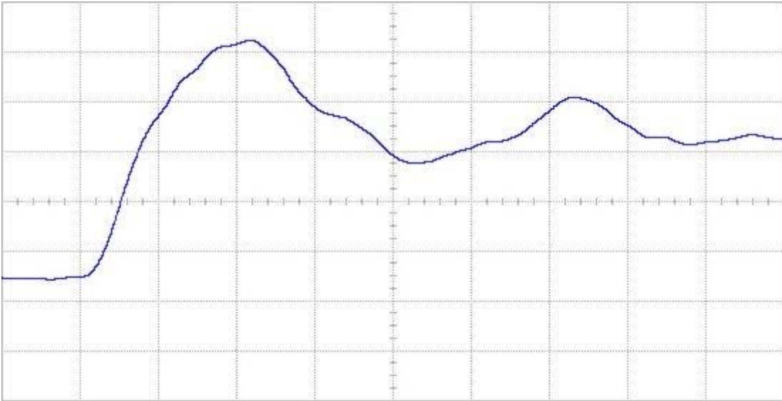
Figure 10(b) DUT 3912 post-annealing rising edge, abscissa scale is 1 V/div and ordinate scale is 2 ns/div.
