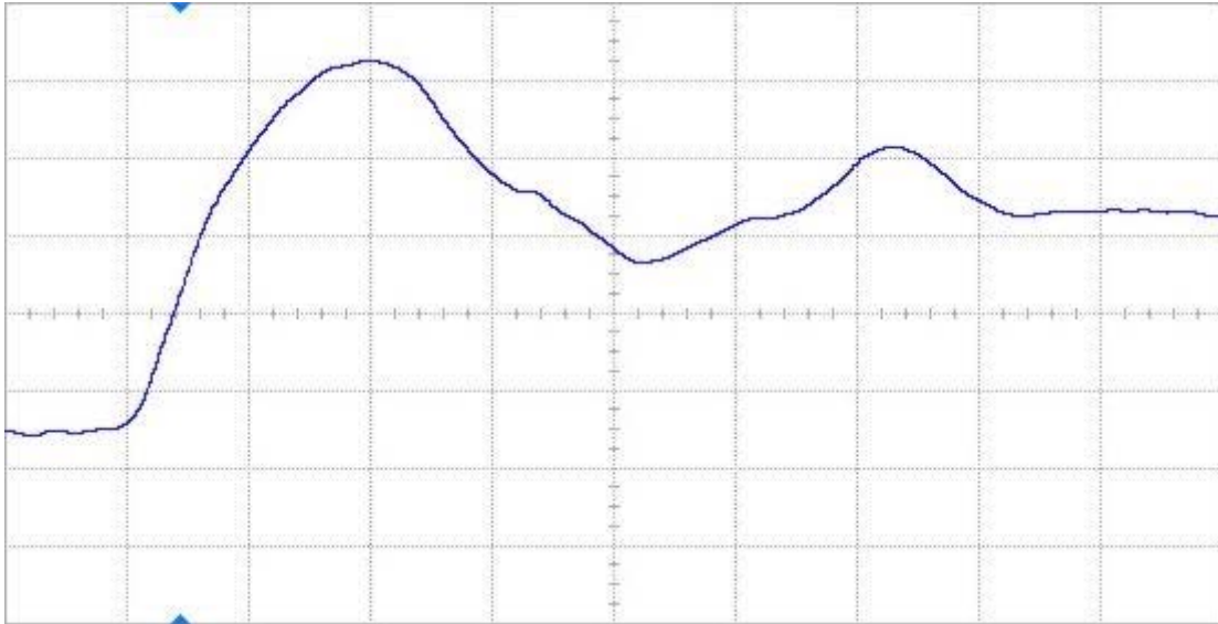
Figure 8(b) DUT 3878 post-annealing rising edge, abscissa scale is 1 V/div and ordinate scale is 2 ns/div.
