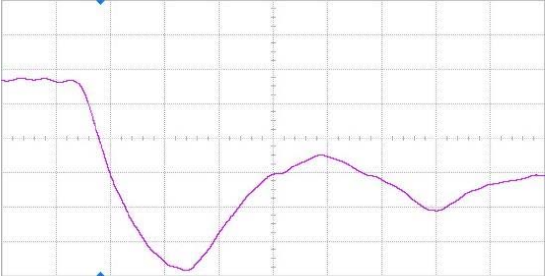
Figure 16(a) DUT 3924 pre-irradiation falling edge, abscissa scale is 1 V/div and ordinate scale is 2 ns/div.
