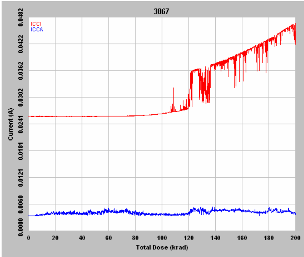
Figure 2 DUT 3867 in-flux I_{CCA} and I_{CCI}
