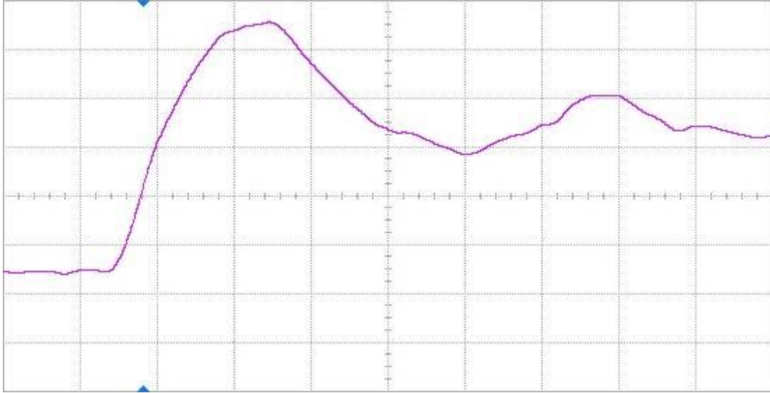
Figure 8(a) DUT 3878 pre-irradiation rising edge, abscissa scale is 1 V/div and ordinate scale is 2 ns/div.
