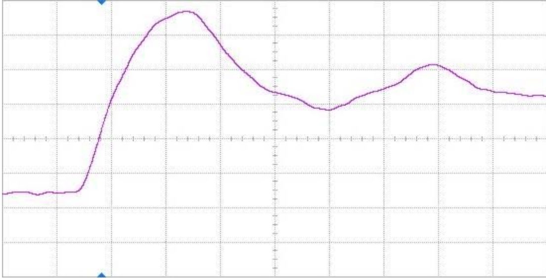
Figure 11(a) DUT 3924 pre-irradiation rising edge, abscissa scale is 1 V/div and ordinate scale is 2 ns/div.
