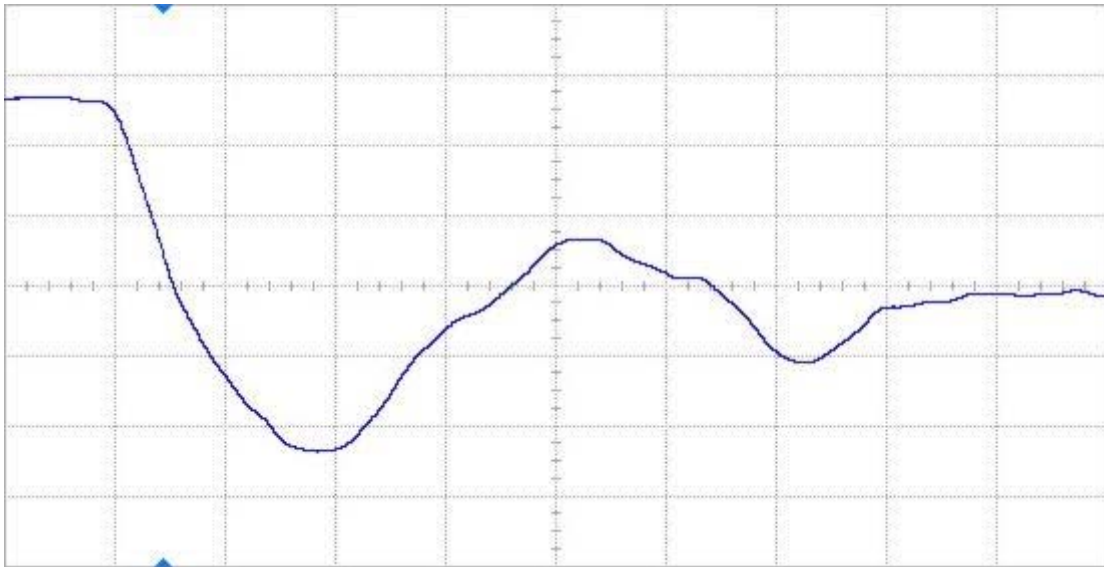
Figure 13(b) DUT 3878 post-annealing falling edge, abscissa scale is 1 V/div and ordinate scale is 2 ns/div.
