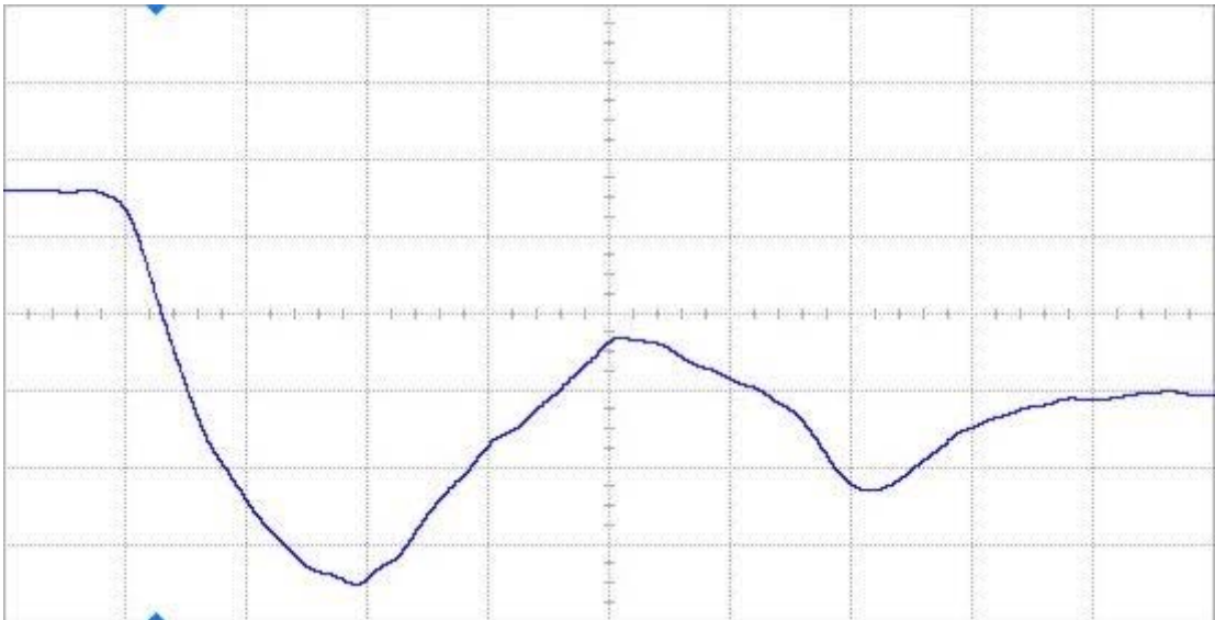
Figure 14(b) DUT 3911 post-annealing falling edge, abscissa scale is 1 V/div and ordinate scale is 2 ns/div.
