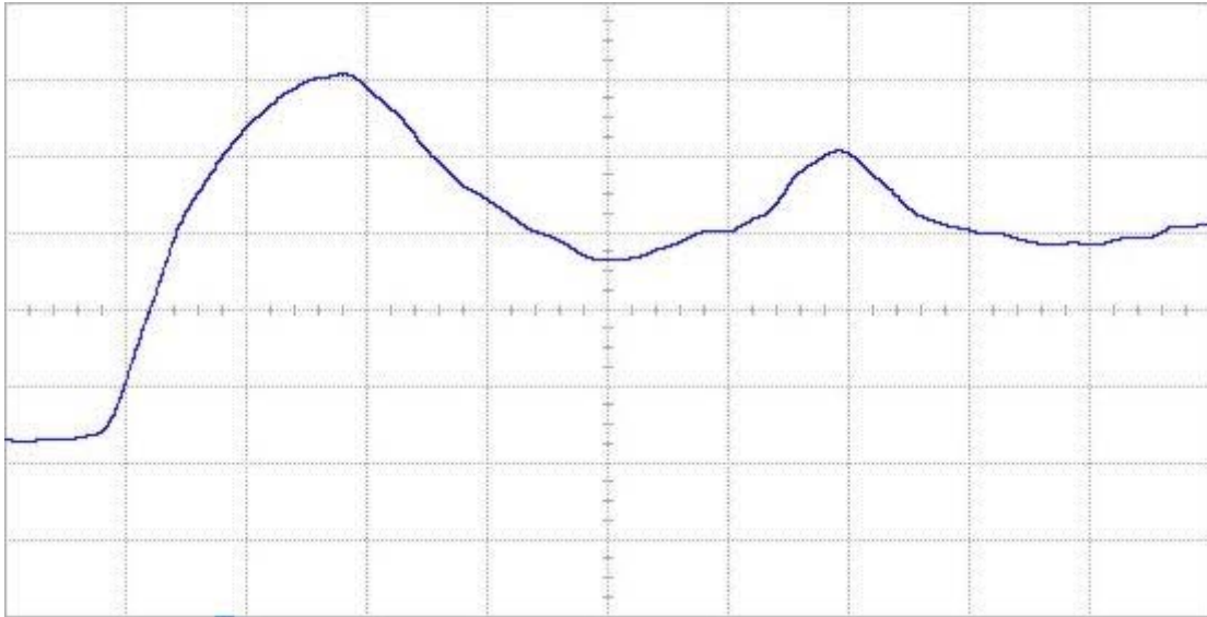
Figure 11(b) DUT 3924 post-annealing rising edge, abscissa scale is 1 V/div and ordinate scale is 2 ns/div.
