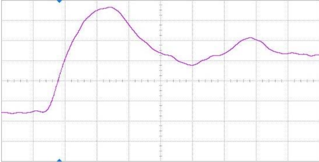
Figure 9(a) DUT 3911 pre-radiation rising edge, abscissa scale is 1 V/div and ordinate scale is 2 ns/div.
