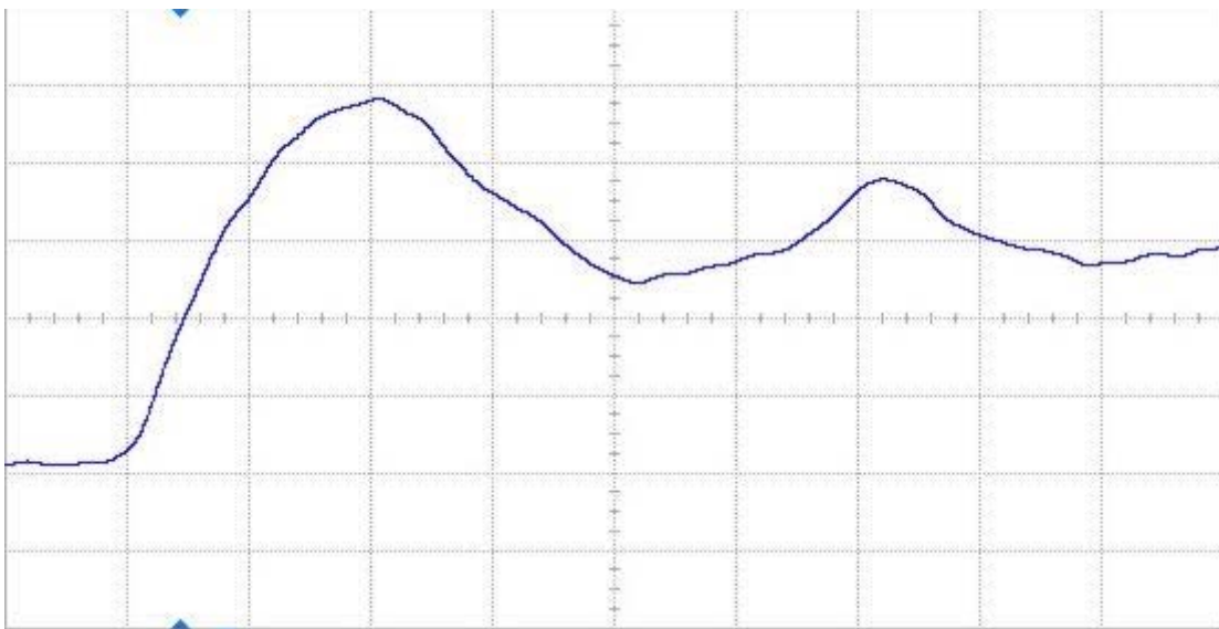
Figure 7(b) DUT 3867 post-annealing rising edge, abscissa scale is 2 V/div and ordinate scale is 2 ns/div.
