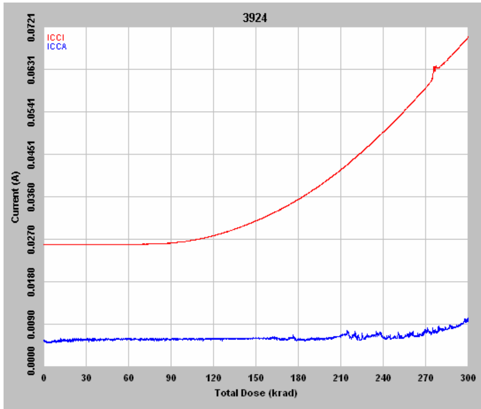
Figure 6 DUT 3924 in-flux I_{CCA} and I_{CCI}
