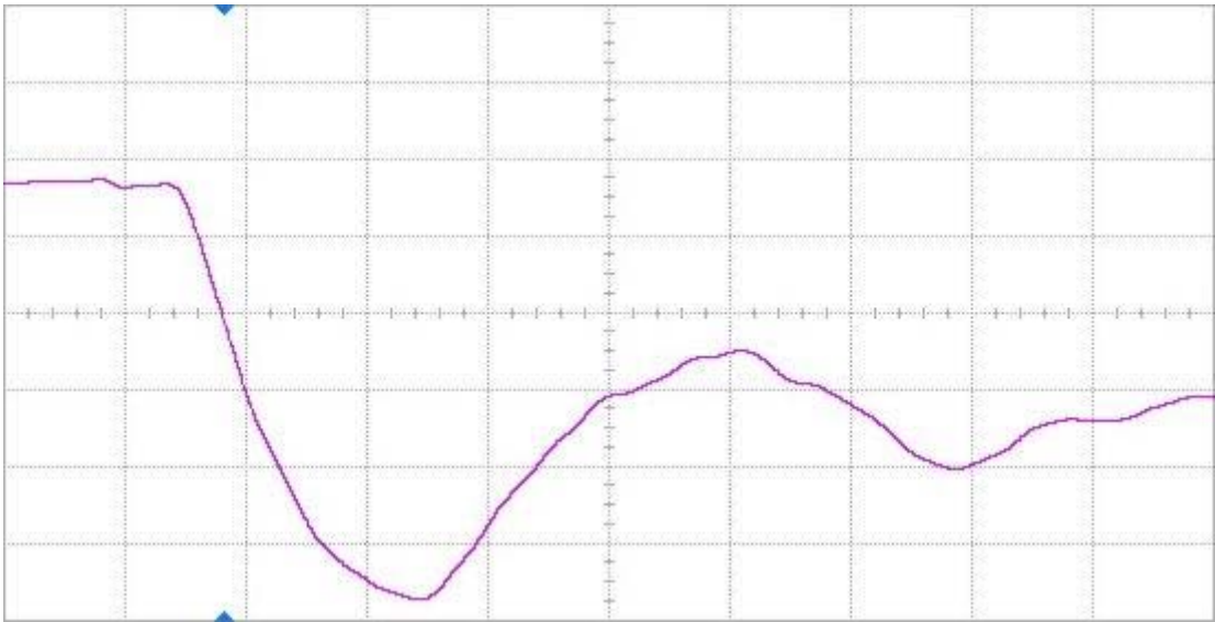
Figure 13(a) DUT 3878 pre-irradiation falling edge, abscissa scale is 1 V/div and ordinate scale is 2 ns/div.
