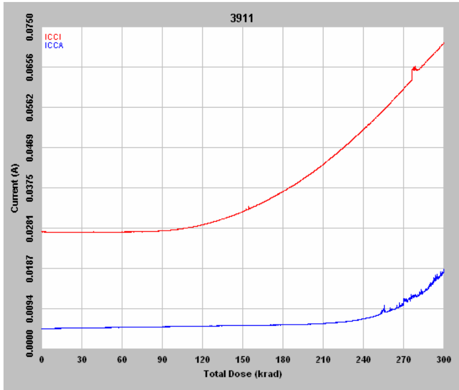
Figure 4 DUT 3911 in-flux I_{CCA} and I_{CCI}
