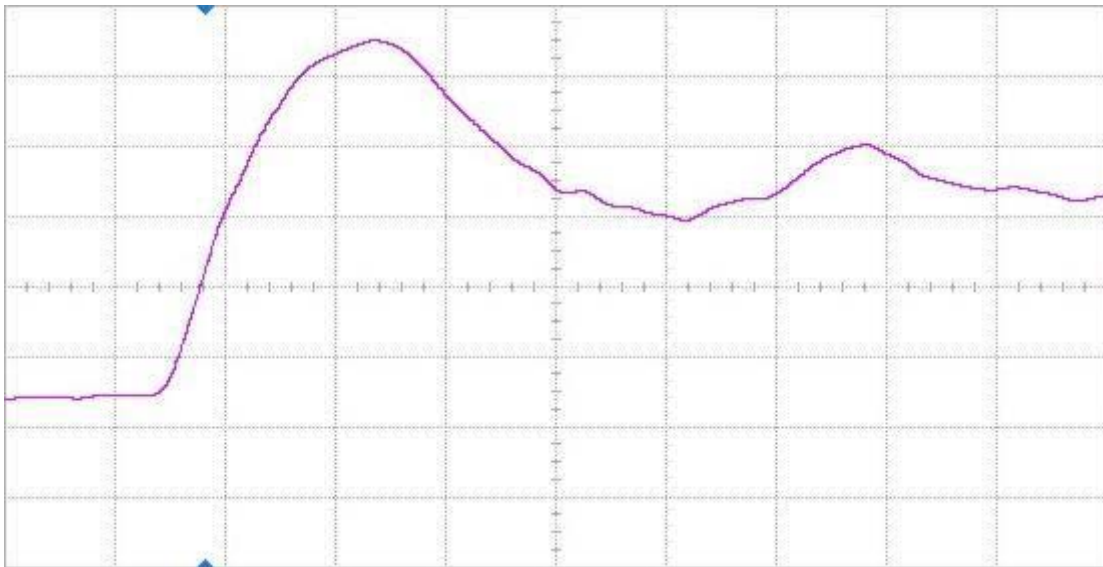
Figure 7(a) DUT 3867 pre-irradiation rising edge, abscissa scale is 1 V/div and ordinate scale is 2 ns/div.
