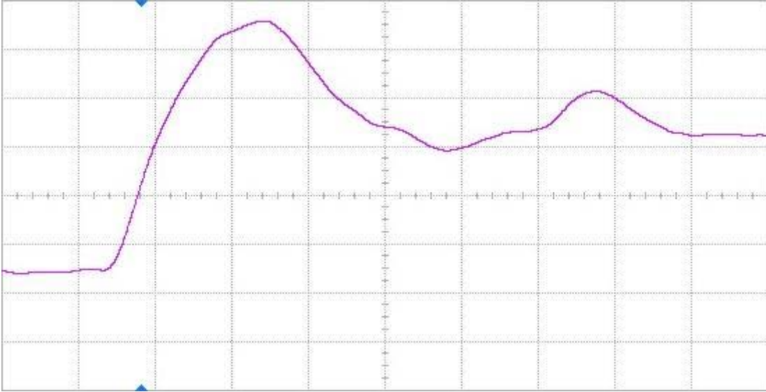
Figure 10(a) DUT 3912 pre-irradiation rising edge, abscissa scale is 1 V/div and ordinate scale is 2 ns/div.
