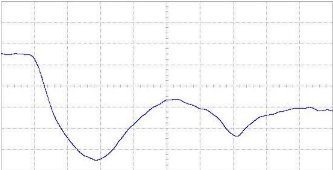
Figure 16(b) DUT 3924 post-annealing falling edge, abscissa scale is 1 V/div and ordinate scale is 2 ns/div.
