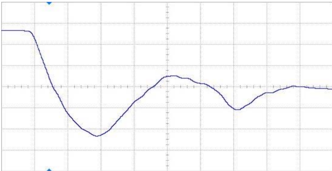
Figure 12(b) DUT 3867 post-annealing falling edge, abscissa scale is 1 V/div and ordinate scale is 2 ns/div.
