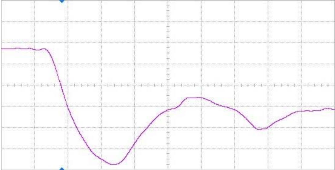
Figure 15(a) DUT 3912 pre-irradiation falling edge, abscissa scale is 1 V/div and ordinate scale is 2 ns/div.
