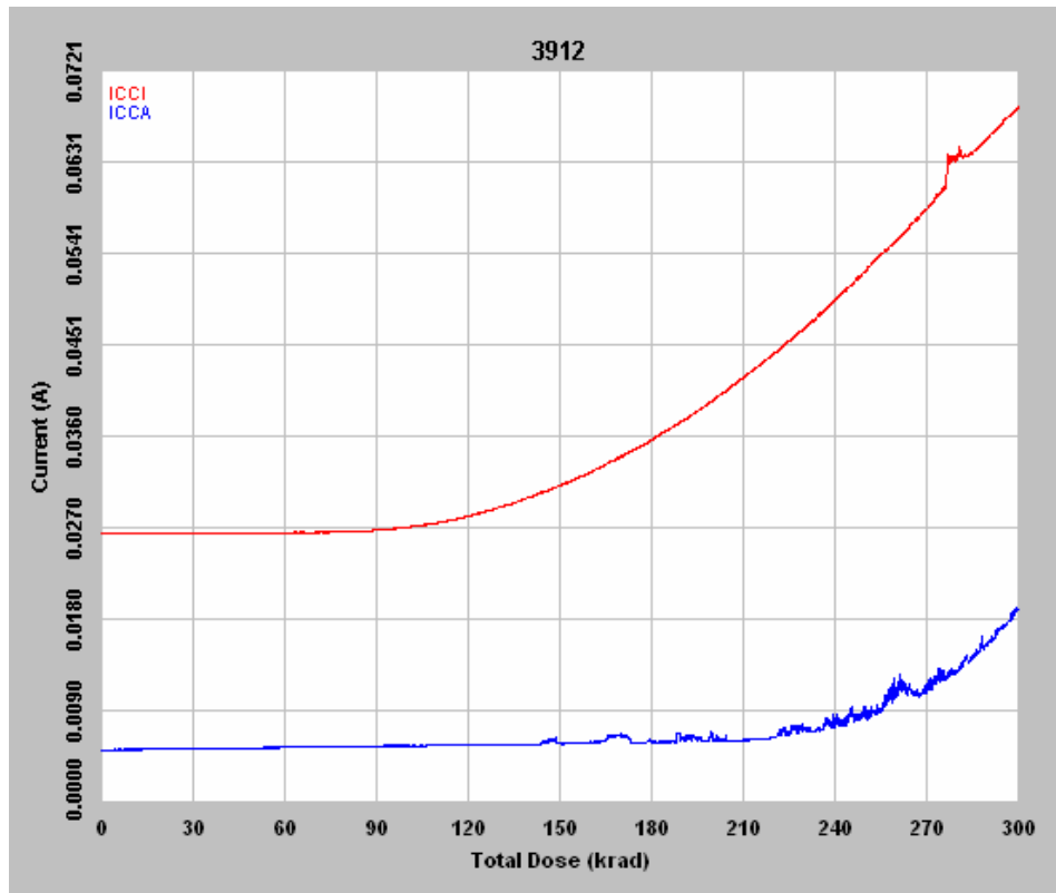
Figure 5 DUT 3912 in-flux I_{CCA} and I_{CCI}
