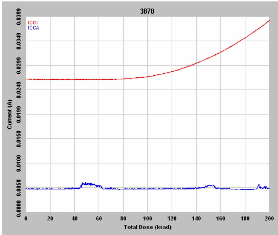
Figure 3 DUT 3878 in-flux I_{CCA} and I_{CCI}
