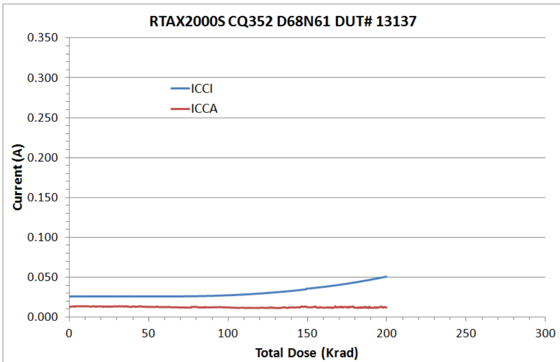
Figure 5 DUT 13137 Influx ICCA and ICCI
