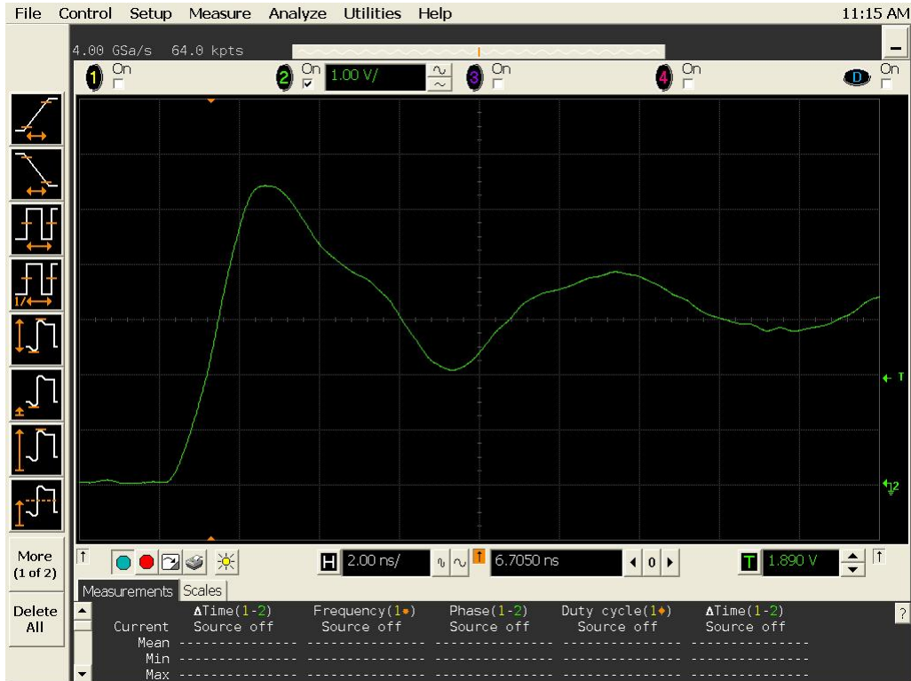
Figure 14b DUT 13150 Post-Annealing Rising Edge
