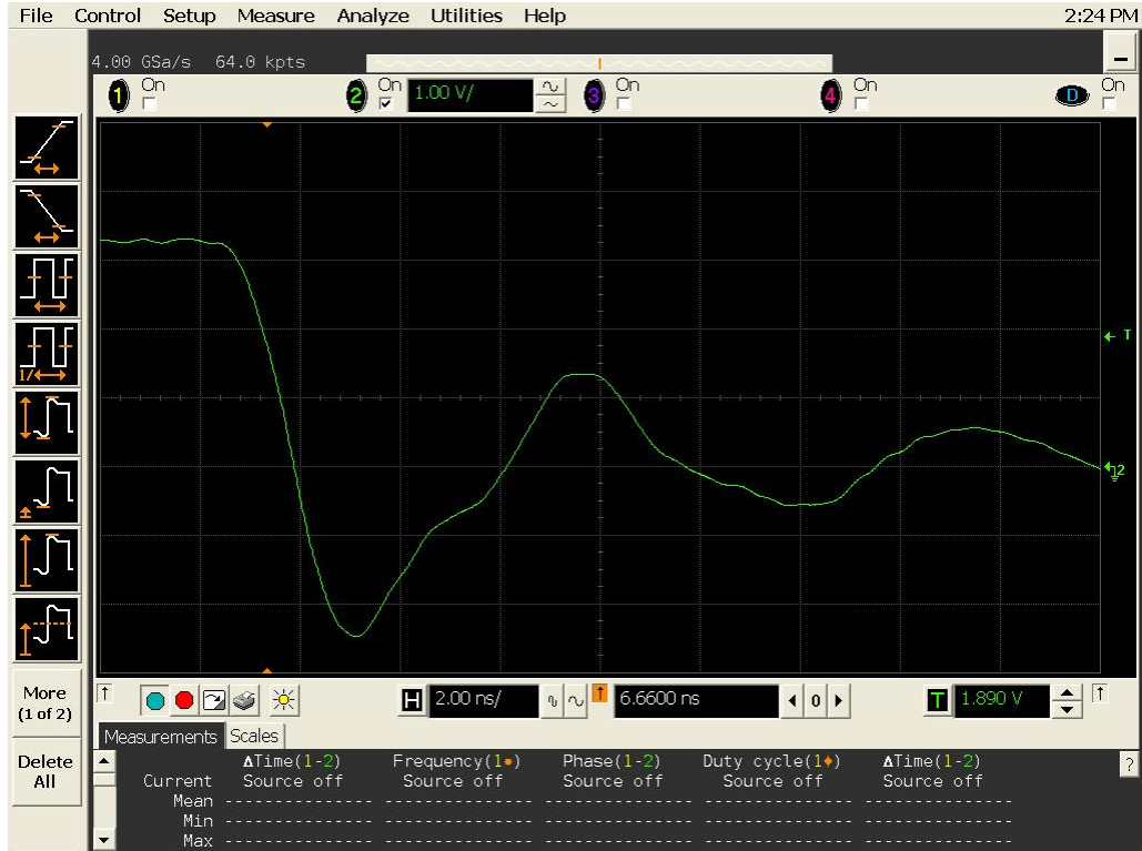
Figure 19a DUT 13148 Pre-Irradiation Falling Edge
