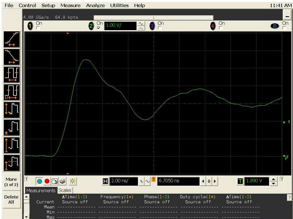
Figure 10b DUT 13132 Post-Annealing Rising Edge
