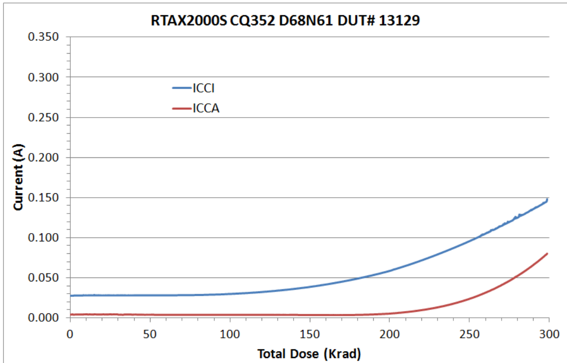
Figure 2 DUT 13129 Influx ICCA and ICCI
