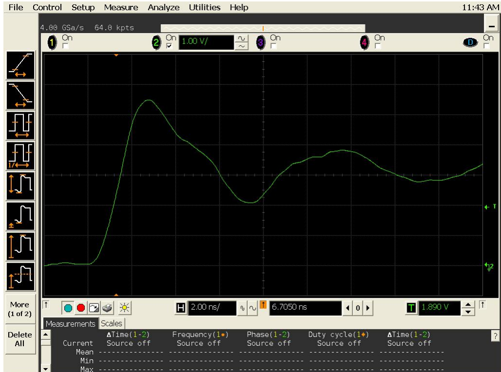
Figure 11b DUT 13134 Post-Annealing Rising edge
