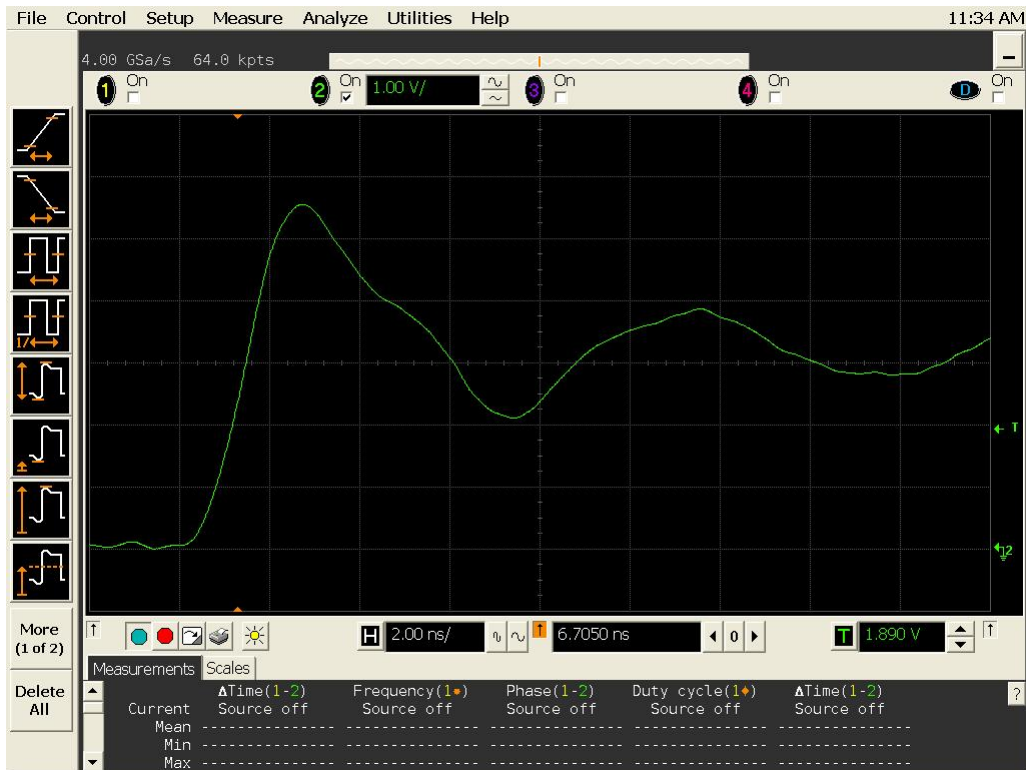
Figure 12b DUT 13137 Post-Annealing Rising Edge
