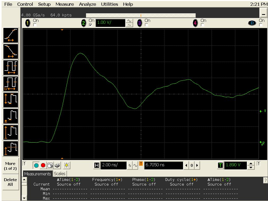
Figure 14a DUT 13150 Pre-Irradiation Rising Edge
