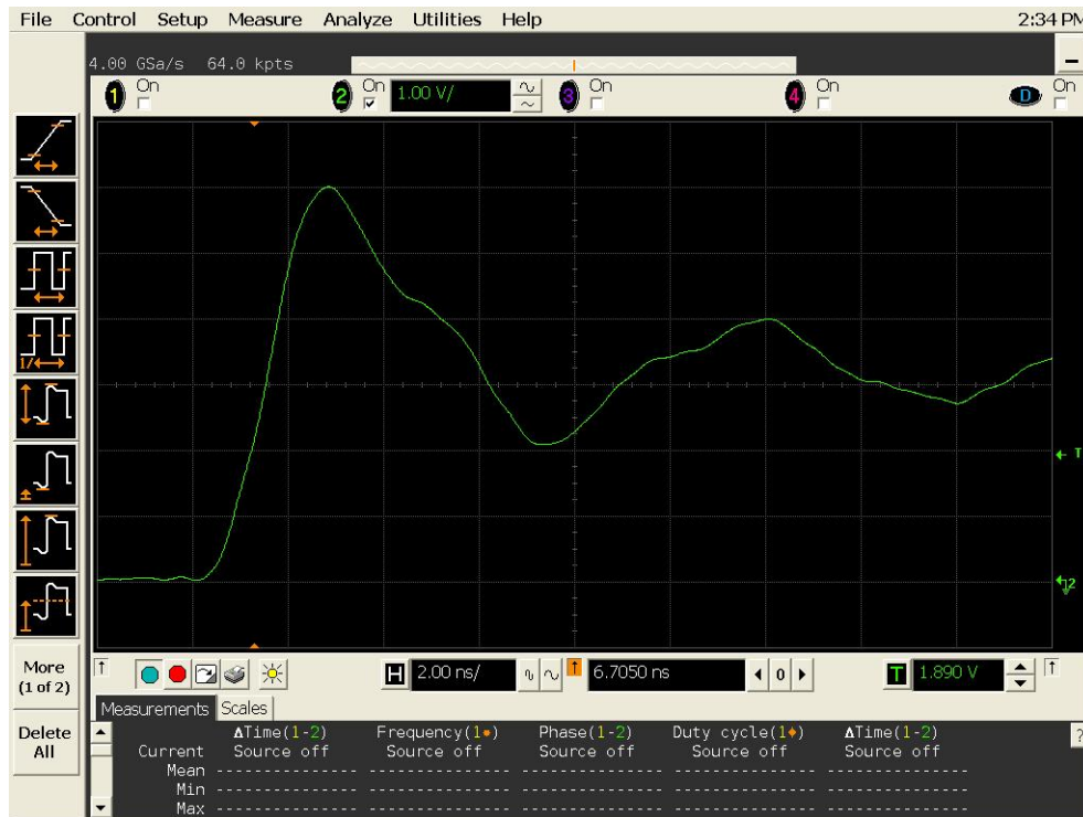
Figure 9a DUT 13129 Pre-Irradiation Rising Edge
