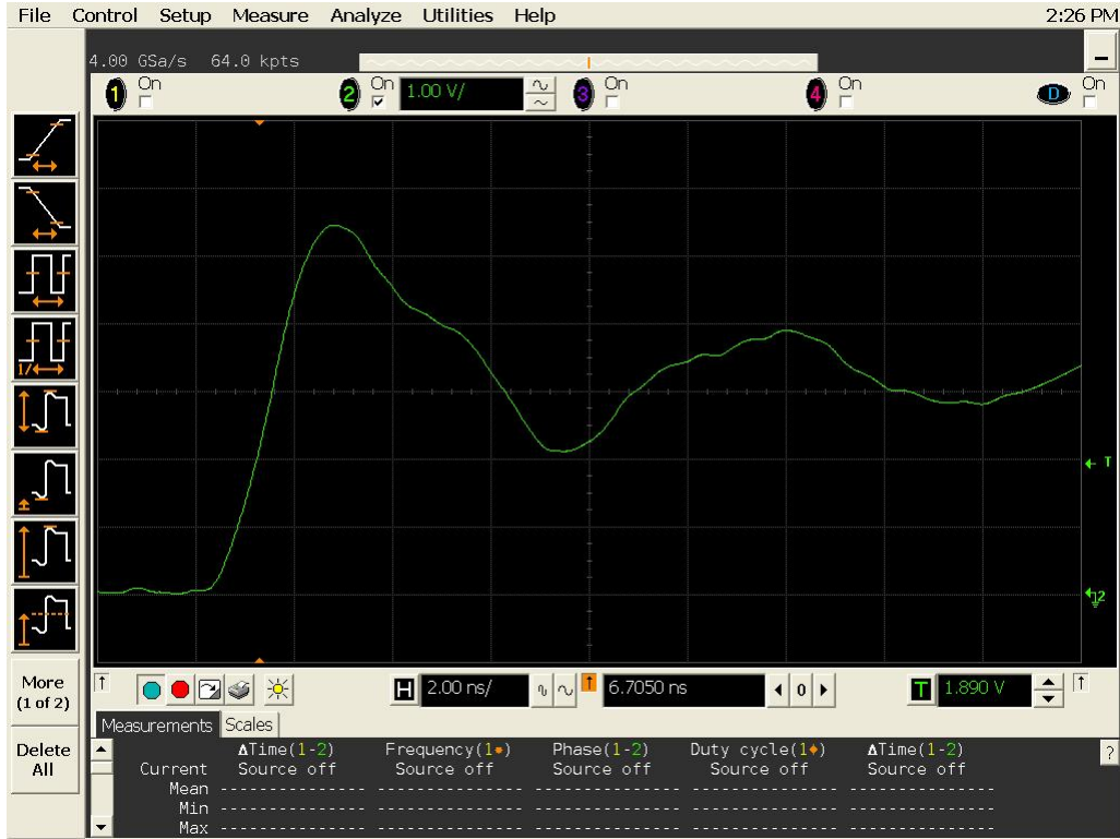
Figure 12a DUT 13137 Pre-Irradiation Rising Edge
