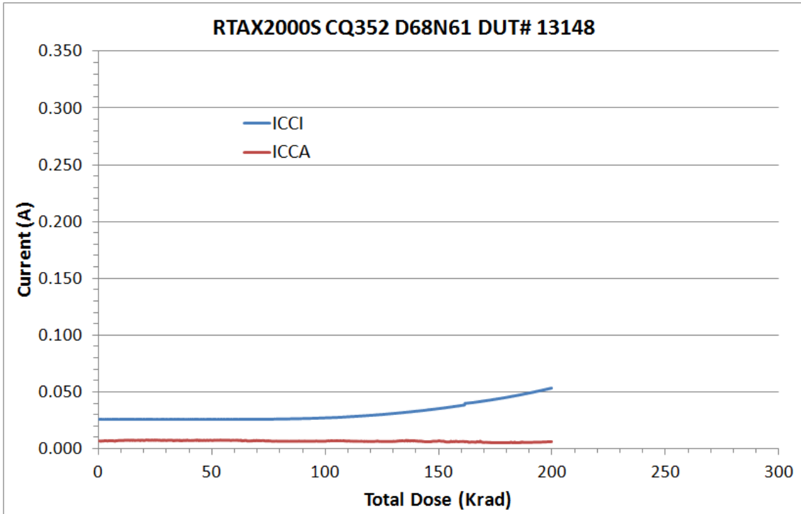
Figure 6 DUT 13148 Influx ICCA and ICCI
