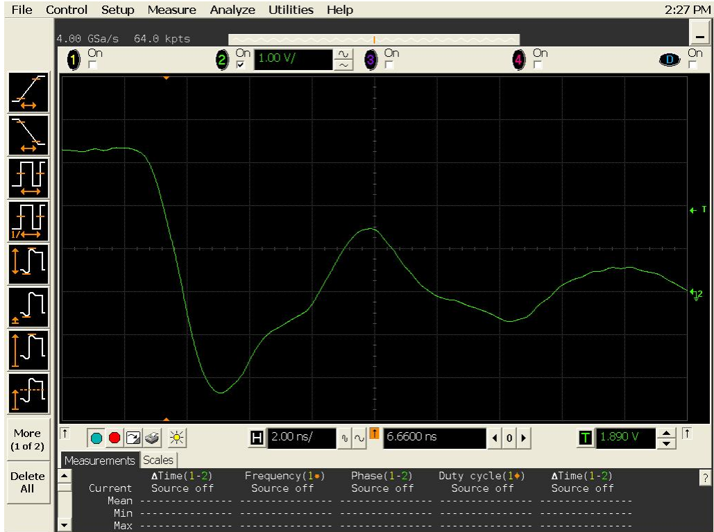
Figure 18a DUT 13137 Pre-Irradiation Falling Edge
