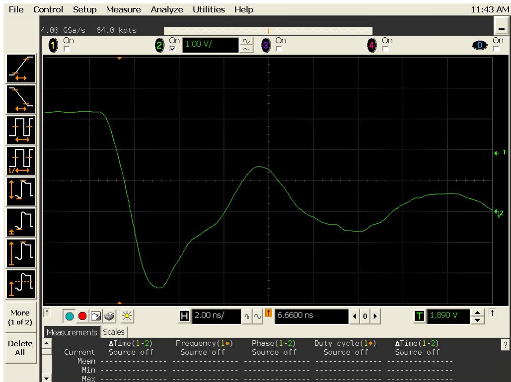
Figure 17b DUT 13134 Post-Annealing Falling Edge
