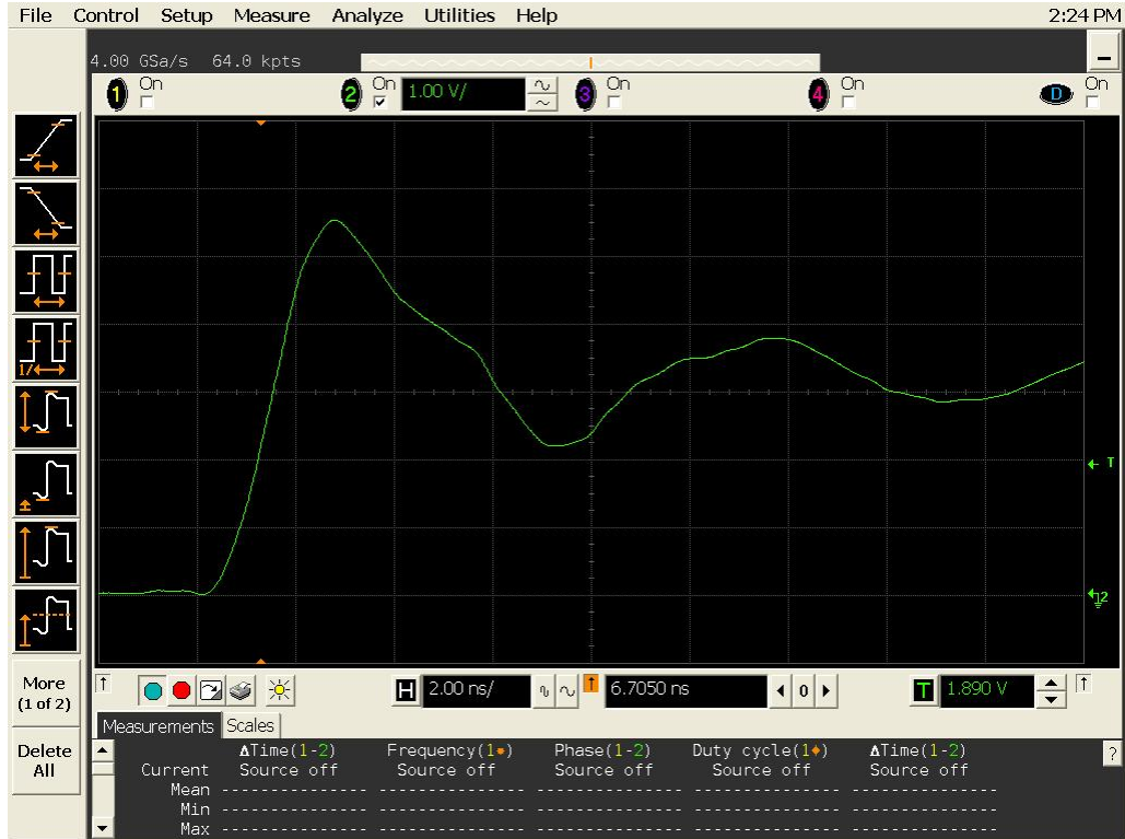
Figure 13a DUT 13148 Pre-Irradiation Rising Edge
