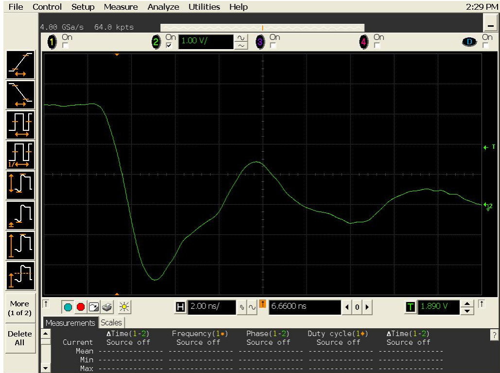
Figure 17a DUT 13134 Pre-Irradiation Falling Edge
