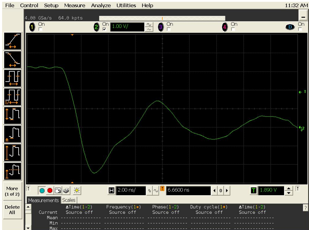
Figure 15b DUT 13129 Post-Annealing Falling Edge
