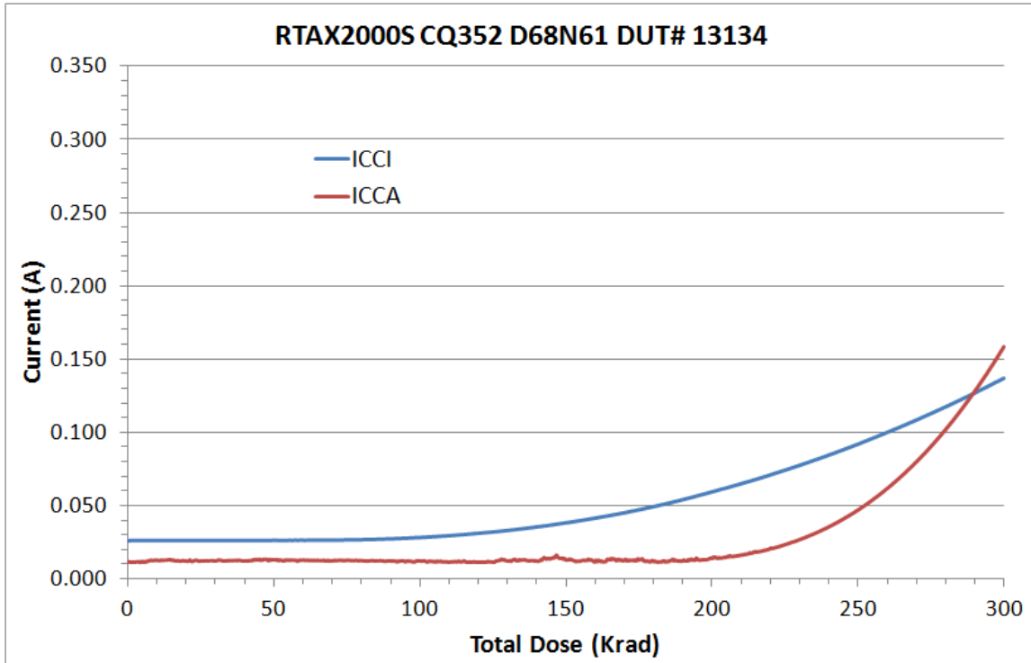
Figure 4 DUT 13134 Influx ICCA and ICCI
