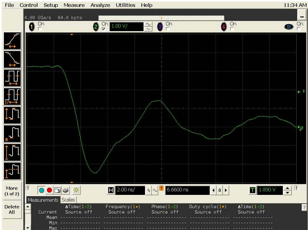
Figure 18b DUT 13137 Post-Annealing Falling Edge
