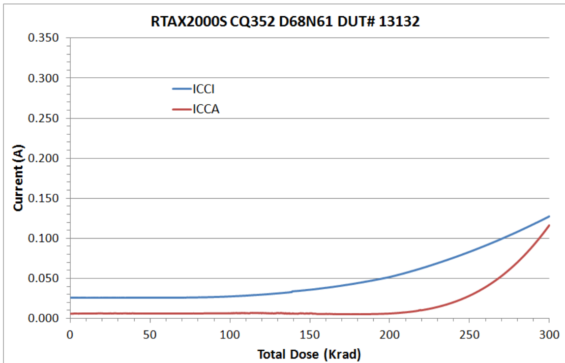
Figure 3 DUT 13132 Influx ICCA and ICCI
