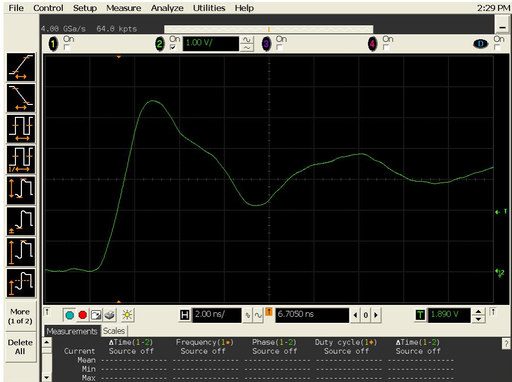
Figure 11a DUT 13134 Pre-Radiation Rising Edge
