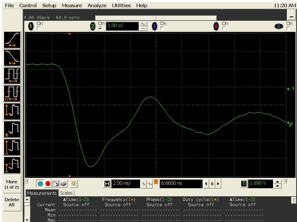
Figure 19b DUT 13148 Post-Annealing Falling Edge
