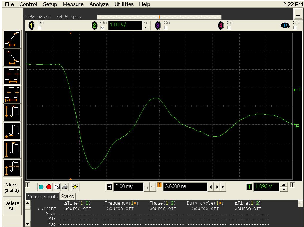
Figure 20a DUT 13150 Pre-Irradiation Falling Edge
