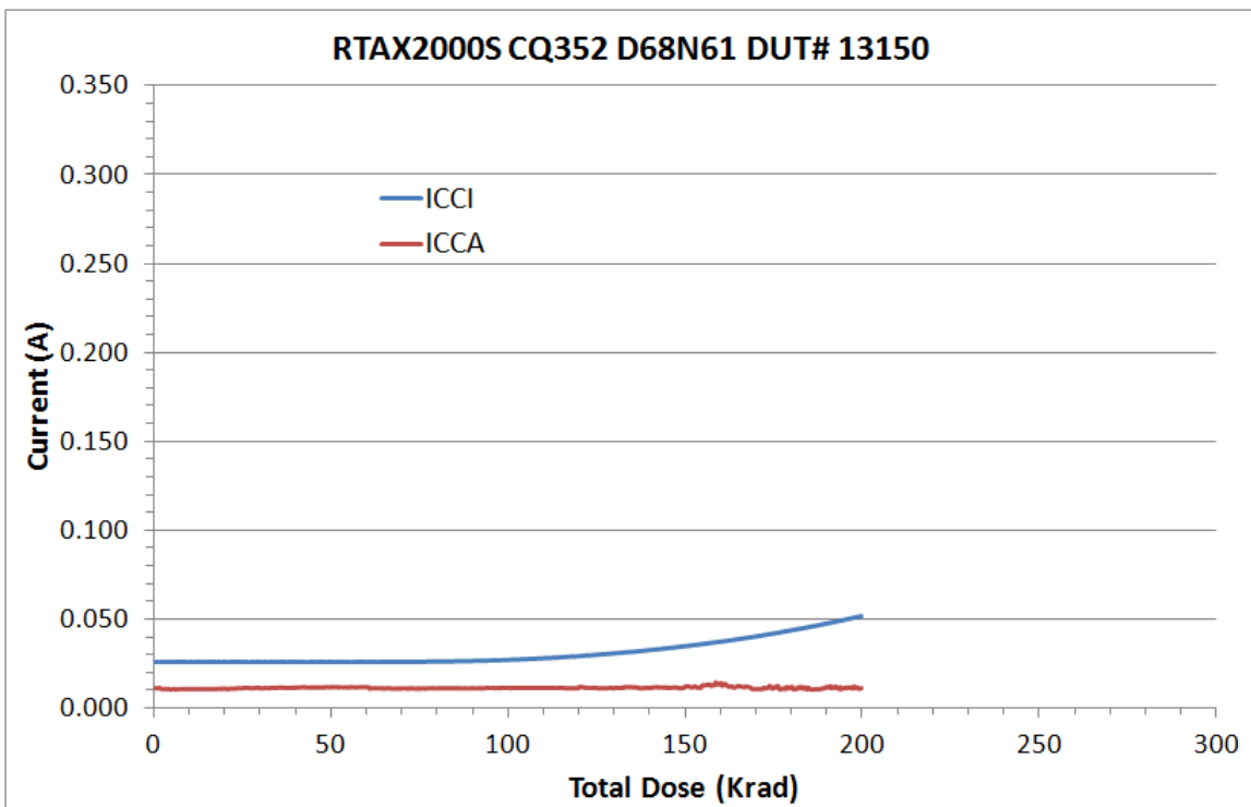
Figure 7 DUT 13150 Influx ICCA and ICCI
