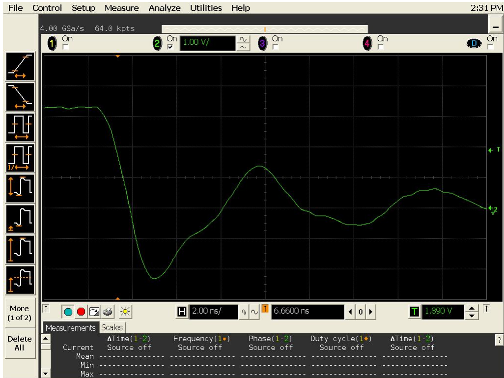
Figure 16a DUT 13132 Pre-Irradiation Falling Edge
