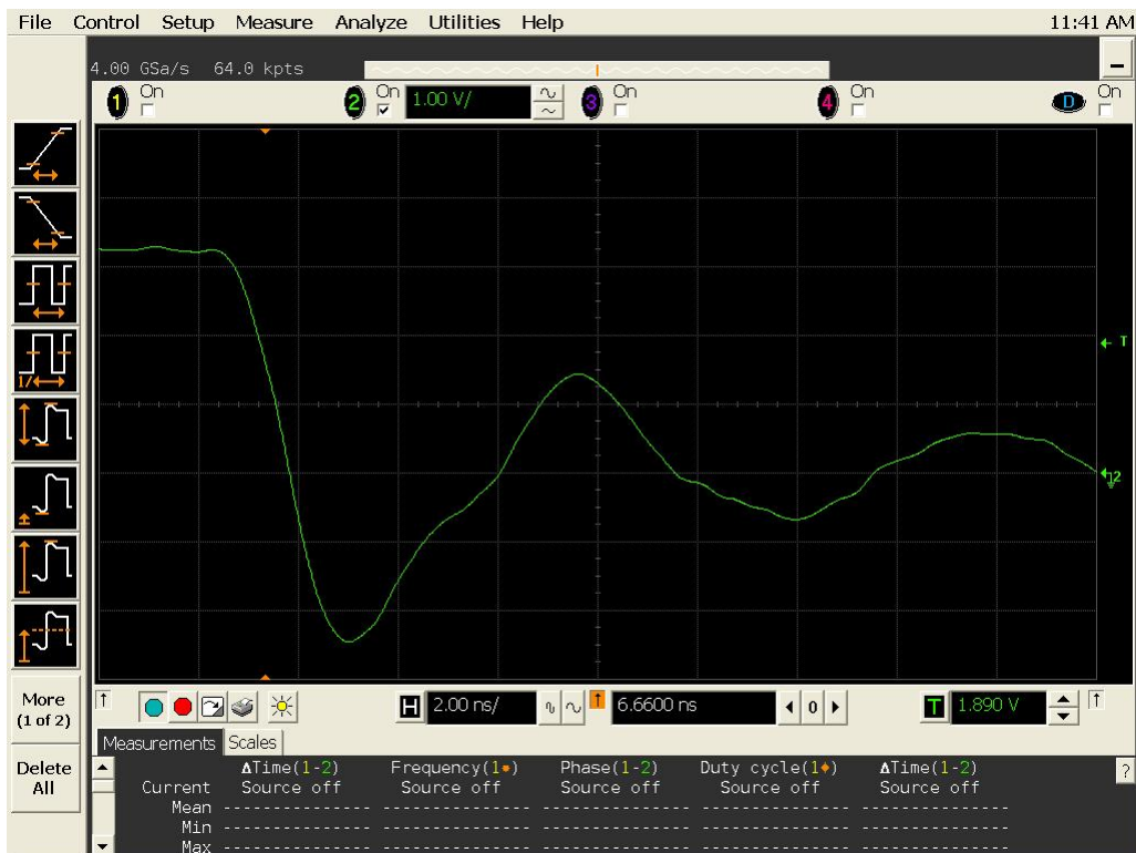
Figure 16b DUT 13132 Post-Annealing Falling Edge
