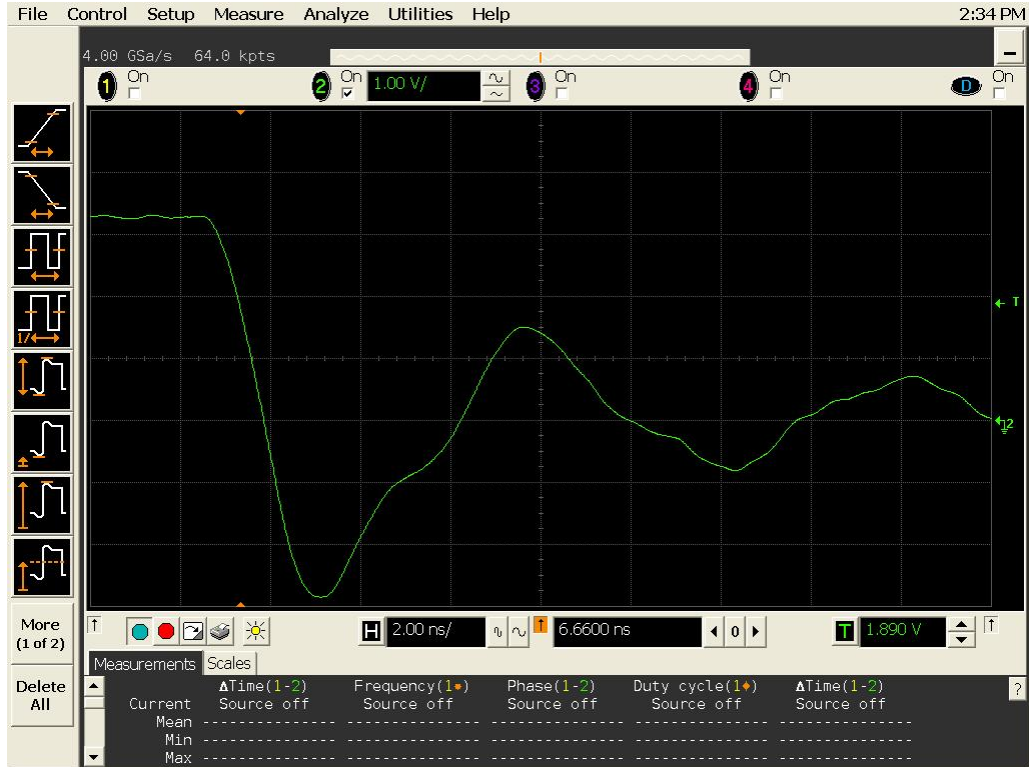
Figure 15a DUT 13129 Pre-Radiation Falling Edge
