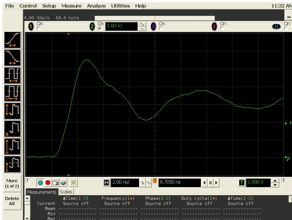
Figure 9b DUT 13129 Post-Annealing Rising Edge
