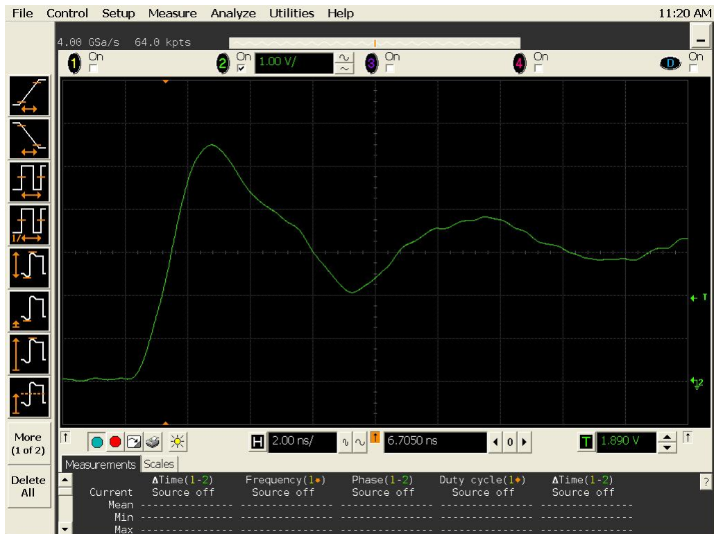
Figure 13b DUT 13148 Post-Annealing Rising Edge
