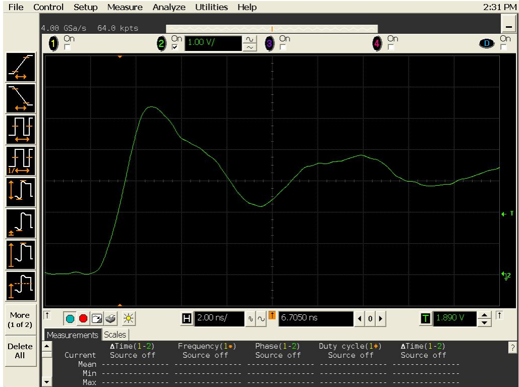
Figure 10a DUT 13132 Pre-Irradiation Rising Edge
