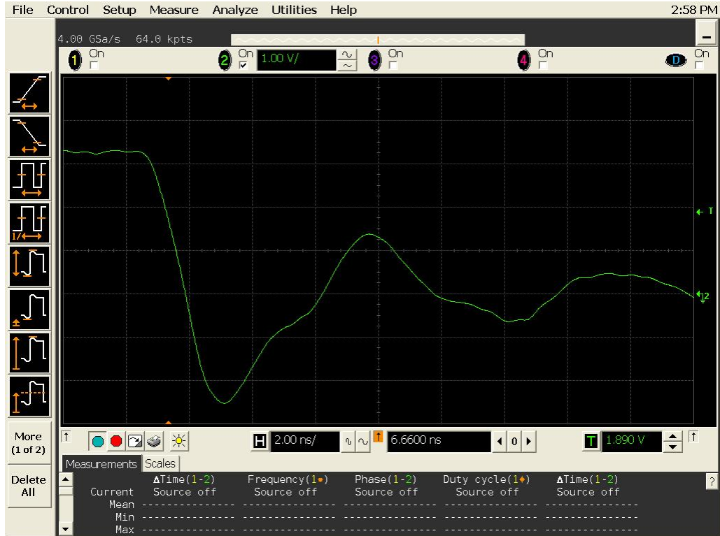
Figure 19a DUT 17216 Pre-Irradiation Falling Edge
