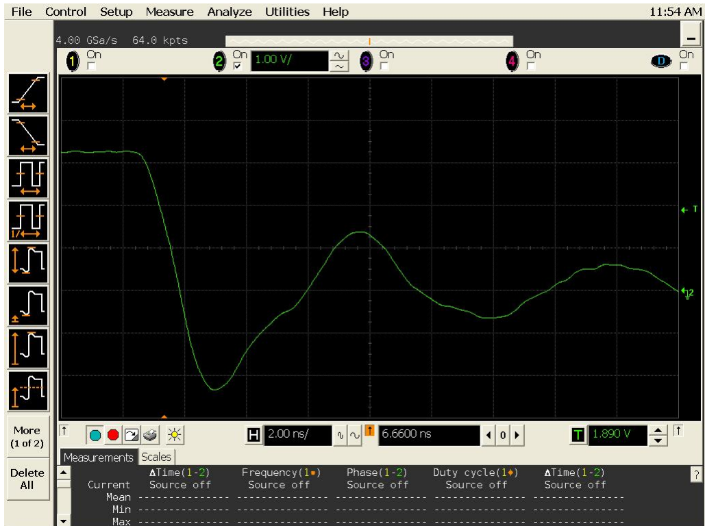
Figure 18b DUT 16373 Post-Annealing Falling Edge
