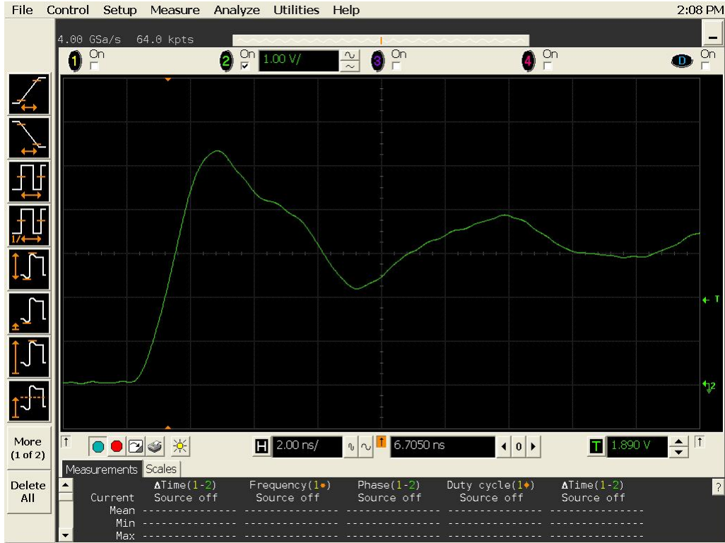
Figure 12a DUT 16373 Pre-Irradiation Rising Edge
