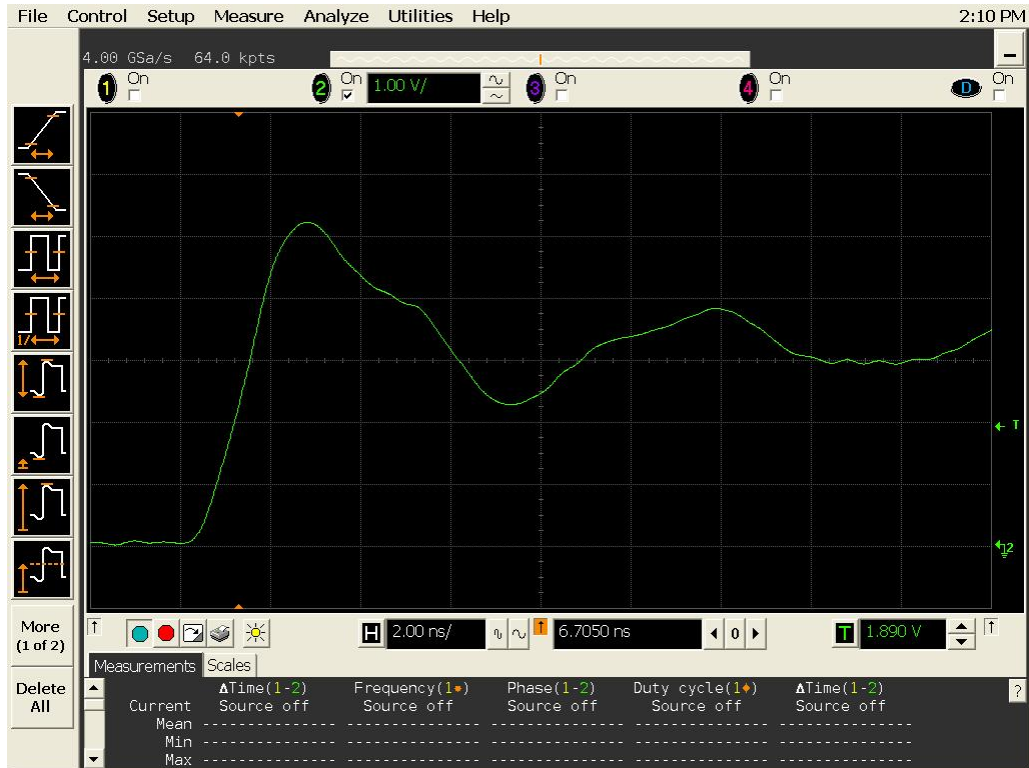
Figure 11a DUT 16365 Pre-Radiation Rising Edge
