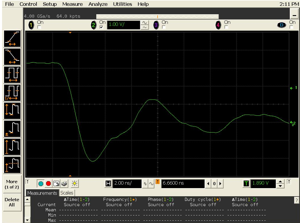
Figure 17a DUT 16365 Pre-Irradiation Falling Edge
