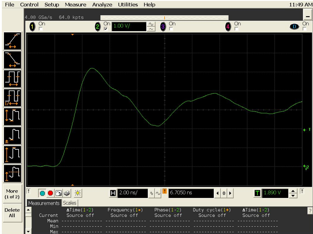
Figure 14b DUT 16402 Post-Annealing Rising Edge
