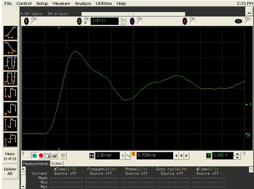
Figure 13a DUT 16387 Pre-Irradiation Rising Edge
