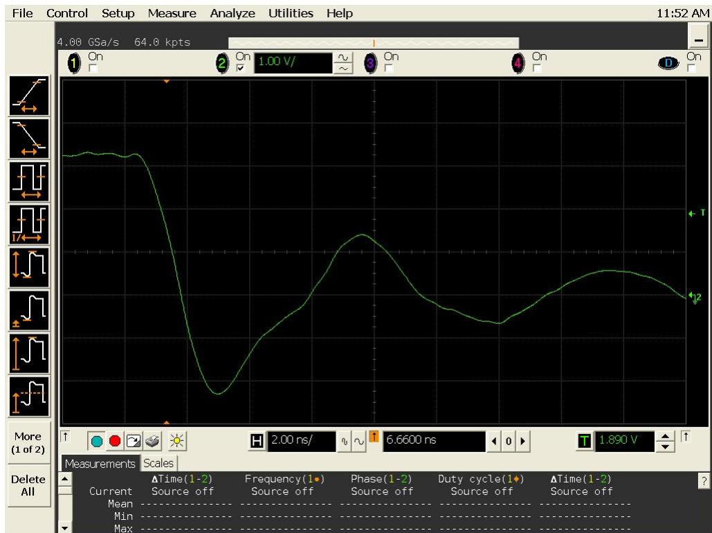
Figure 19b DUT 16387 Post-Annealing Falling Edge
