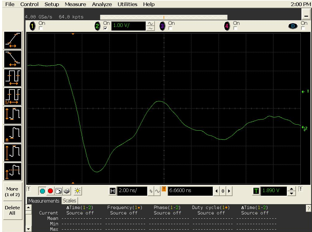
Figure 15a DUT 16353 Pre-Radiation Falling Edge
