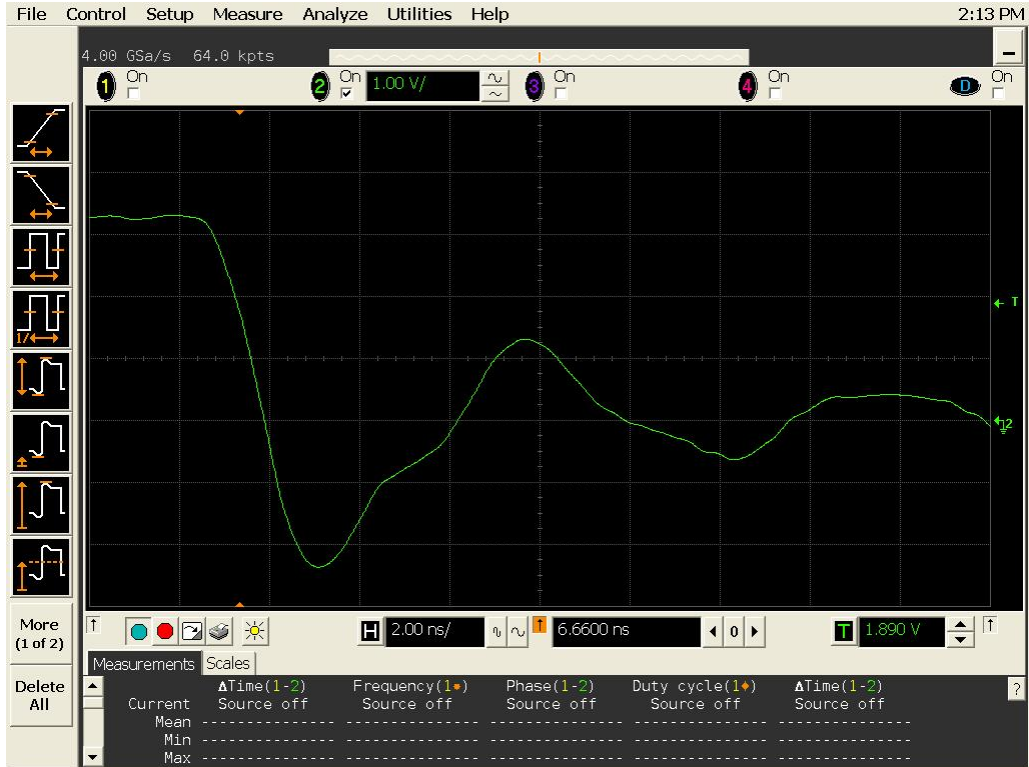
Figure 20a DUT 16402 Pre-Irradiation Falling Edge
