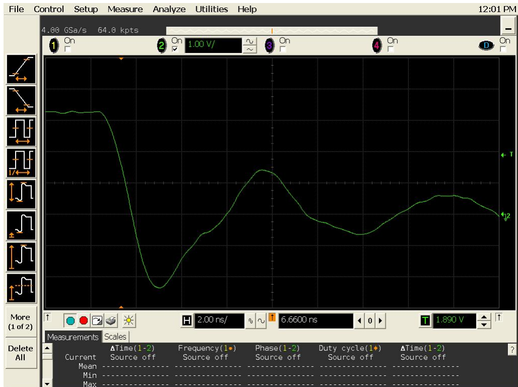
Figure 15b DUT 16353 Post-Annealing Falling Edge
