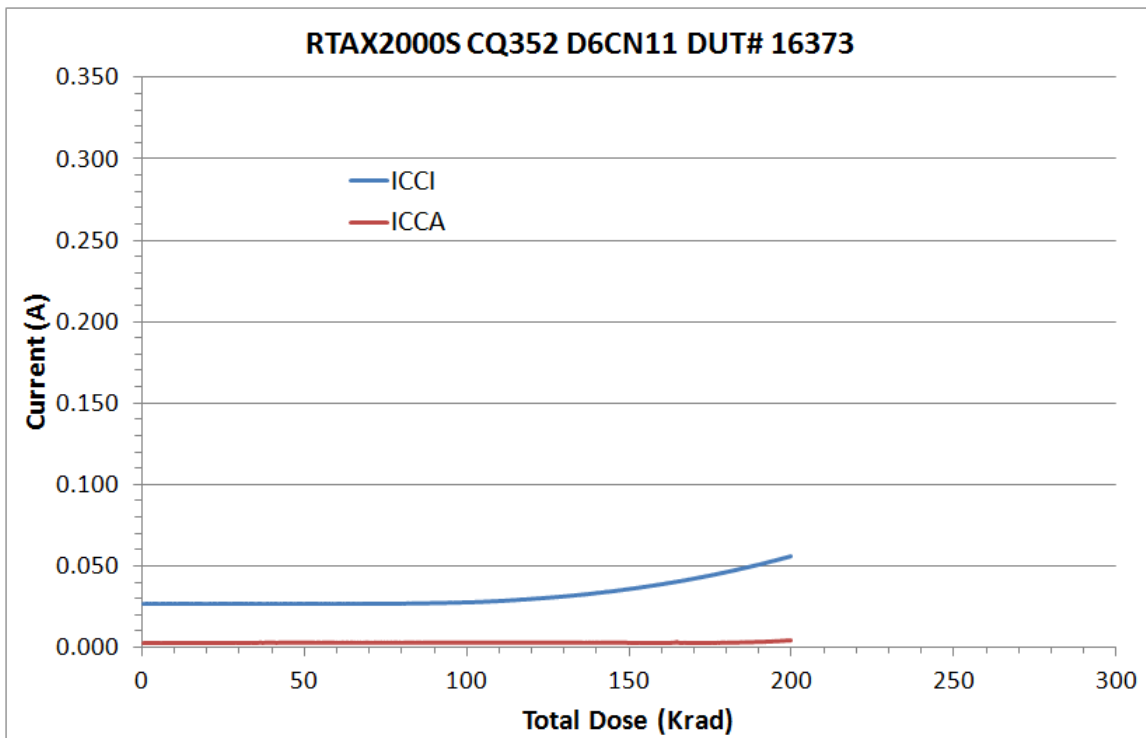
Figure 5 DUT 16373 Influx ICCA and ICCI
