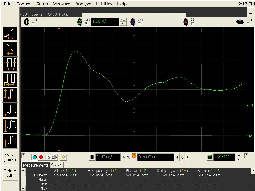
Figure 14a DUT 16402 Pre-Irradiation Rising Edge
