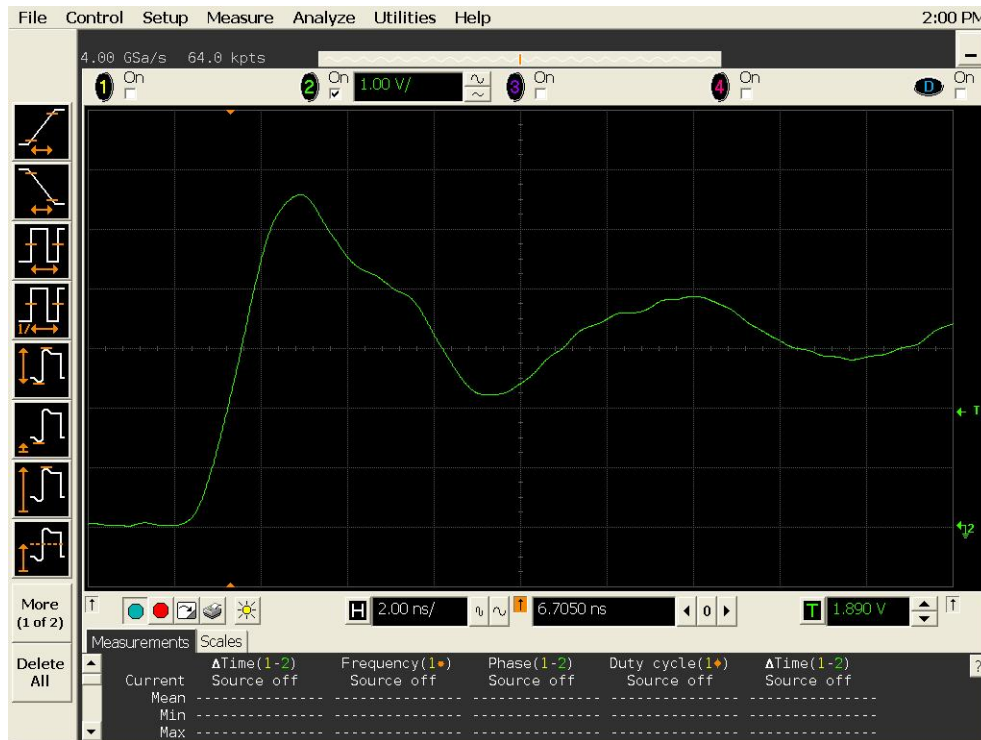
Figure 9a DUT 16353 Pre-Irradiation Rising Edge
