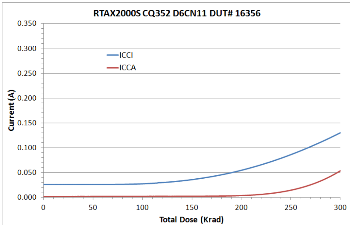
Figure 3 DUT 16356 Influx ICCA and ICCI
