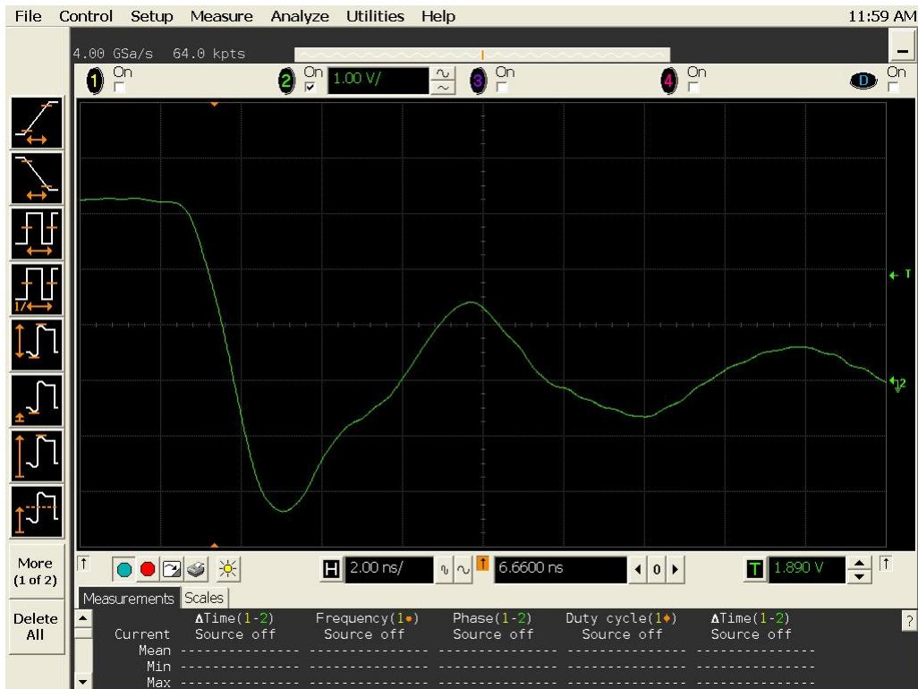
Figure 16b DUT 16356 Post-Annealing Falling Edge
