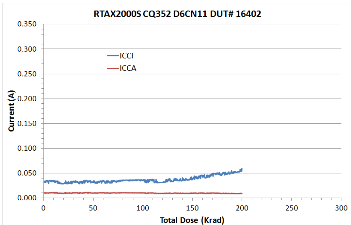
Figure 7 DUT 16402 Influx ICCA and ICCI
