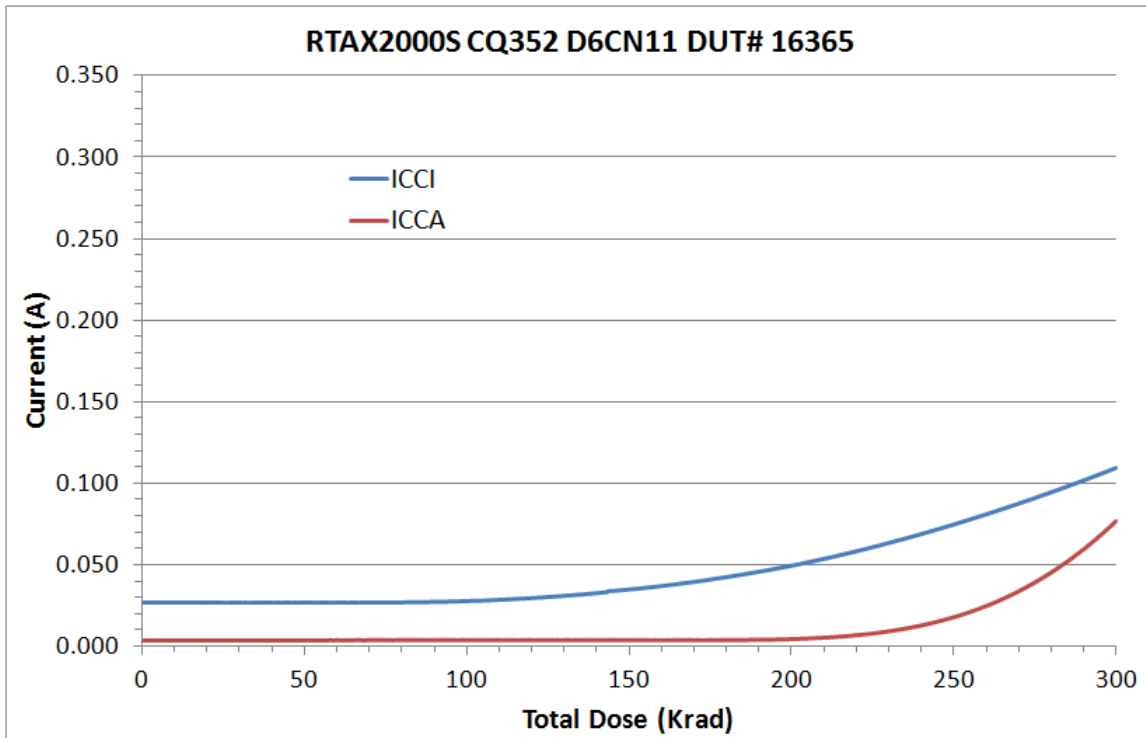
Figure 4 DUT 16365 Influx ICCA and ICCI
