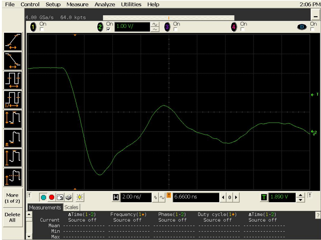
Figure 16a DUT 16356 Pre-Irradiation Falling Edge
