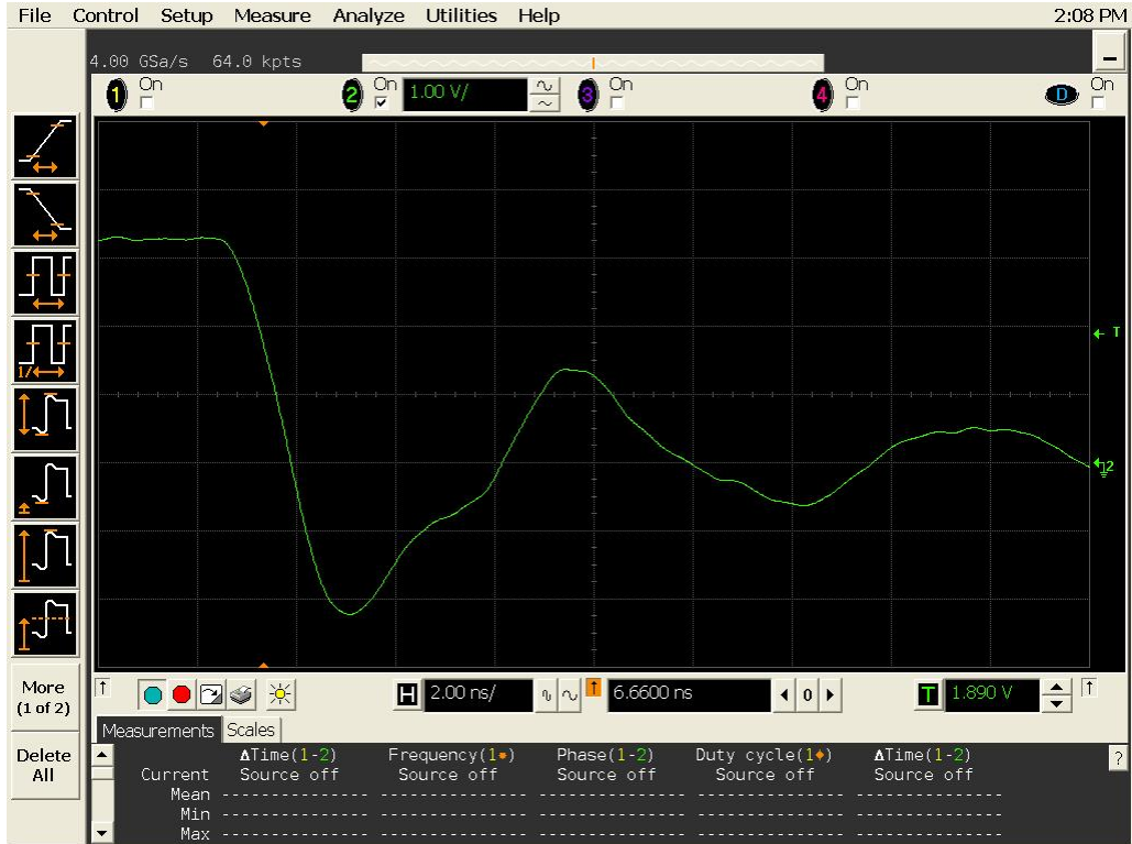
Figure 18a DUT 16373 Pre-Irradiation Falling Edge
