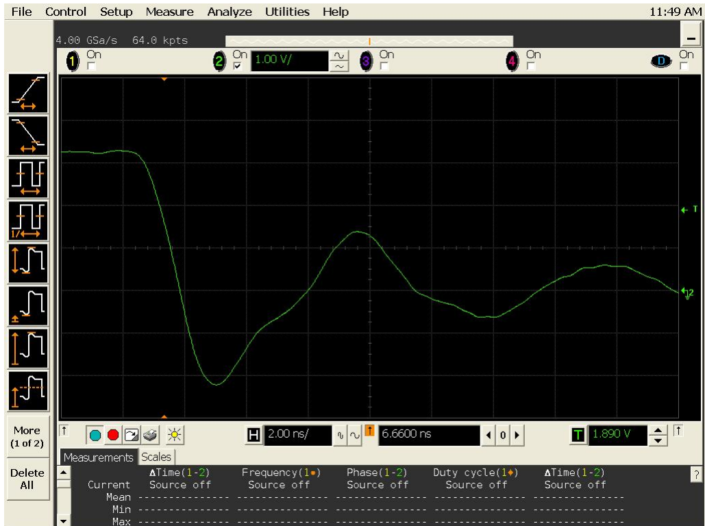
Figure 20b DUT 16402 Post-Annealing Falling Edge
