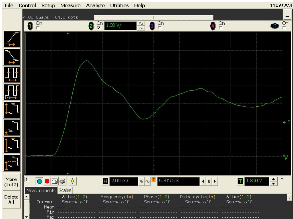
Figure 10b DUT 16356 Post-Annealing Rising Edge
