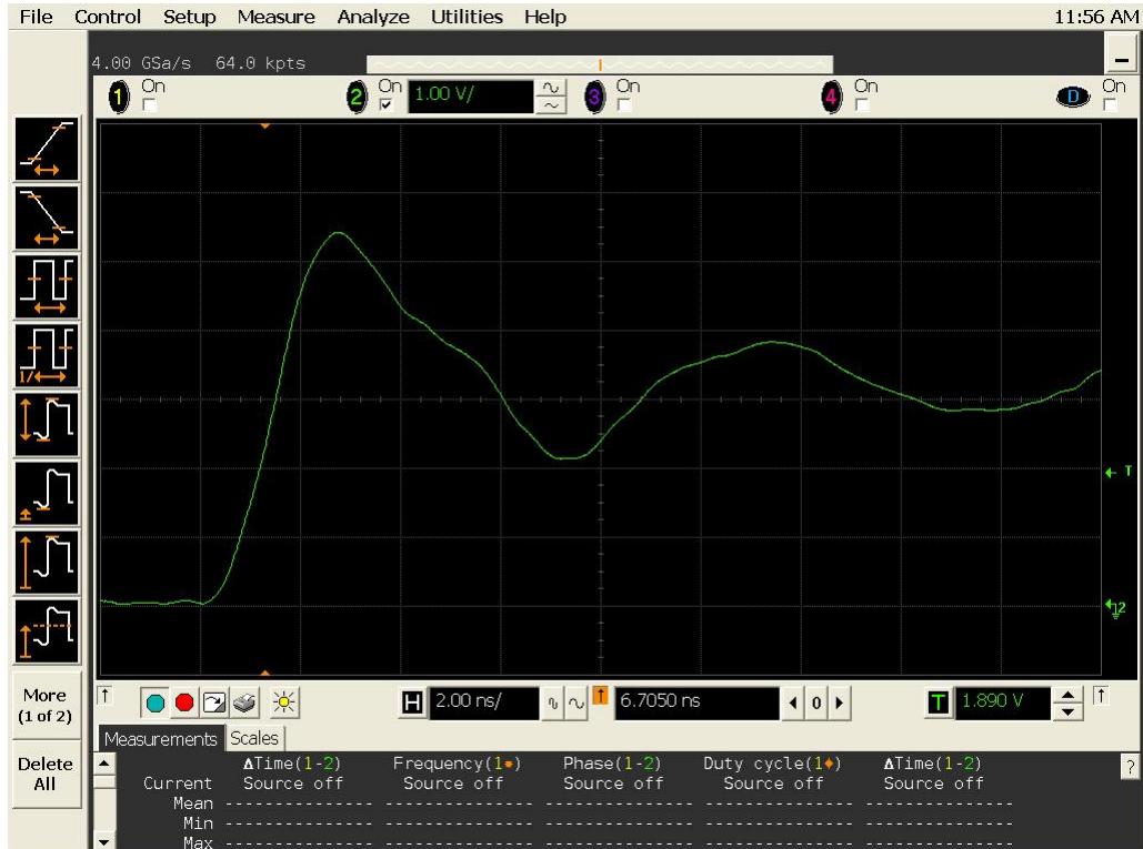
Figure 11b DUT 16365 Post-Annealing Rising edge
