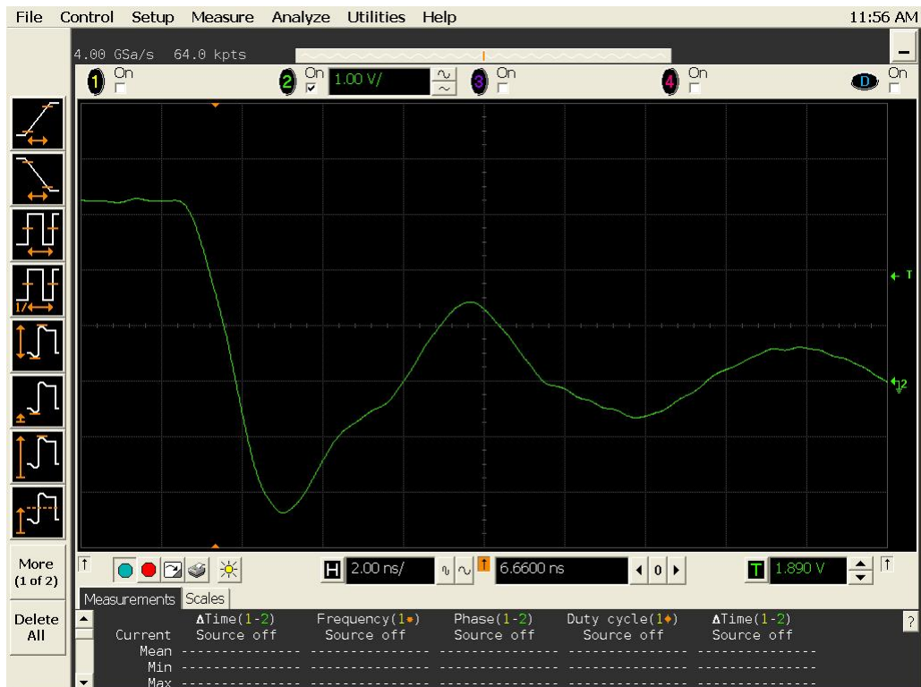
Figure 17b DUT 16365 Post-Annealing Falling Edge
