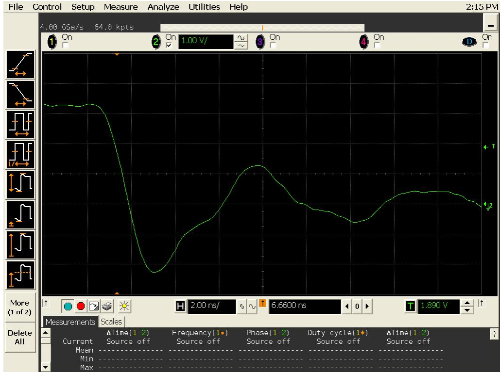
Figure 19a DUT 16387 Pre-Irradiation Falling Edge
