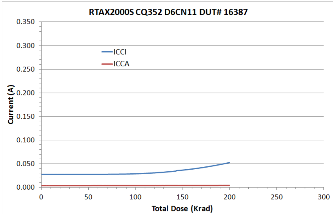
Figure 6 DUT 16387 Influx ICCA and ICCI
