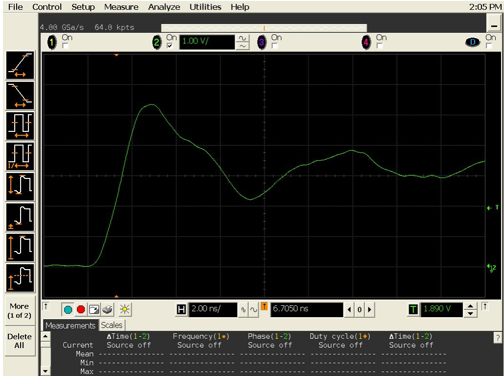
Figure 10a DUT 16356 Pre-Irradiation Rising Edge
