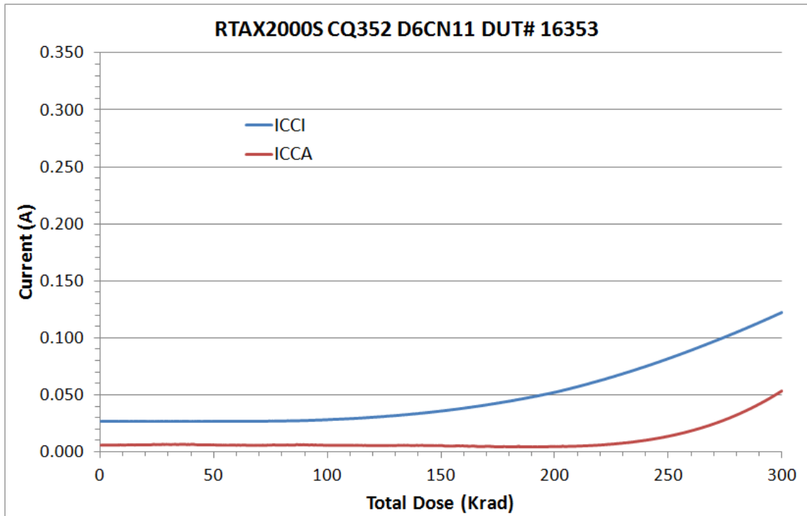
Figure 2 DUT 16353 Influx ICCA and ICCI
