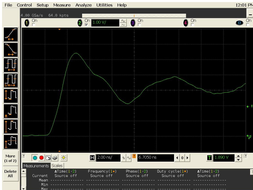
Figure 9b DUT 16353 Post-Annealing Rising Edge
