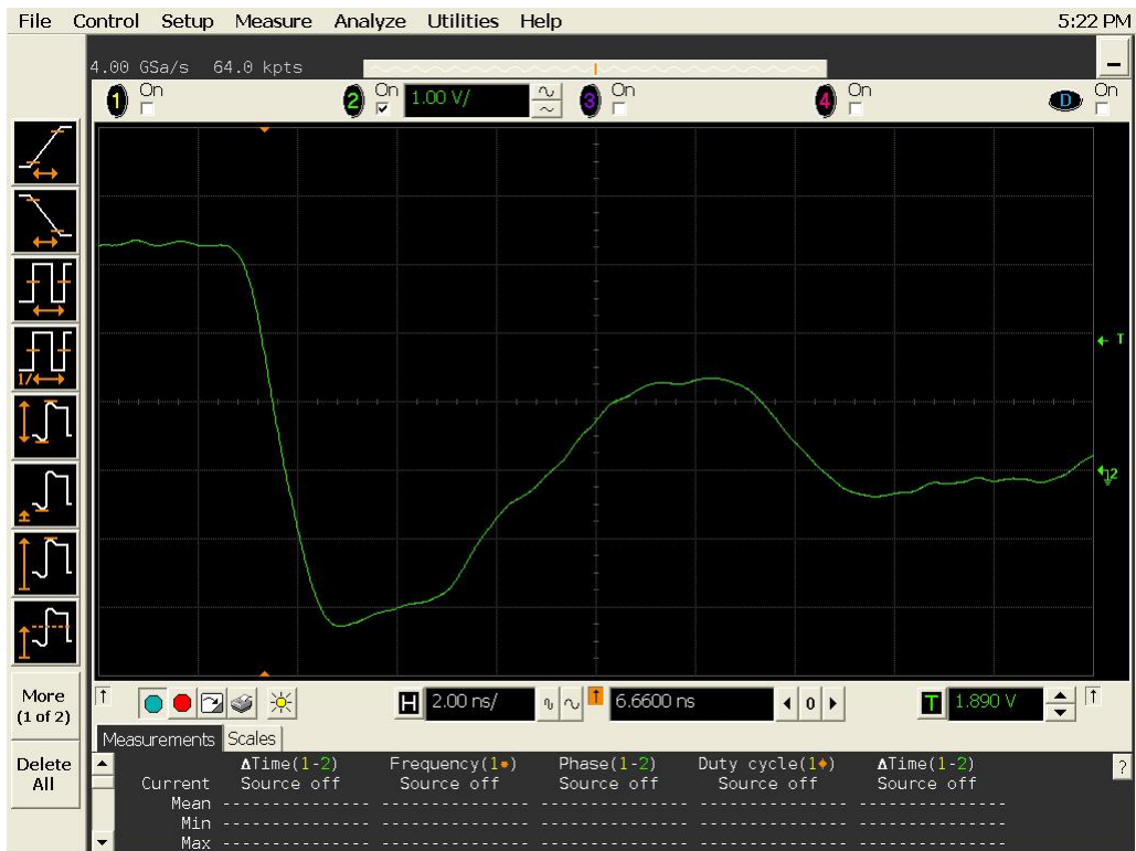
Figure 20b DUT 3319 Post-Annealing Falling Edge
