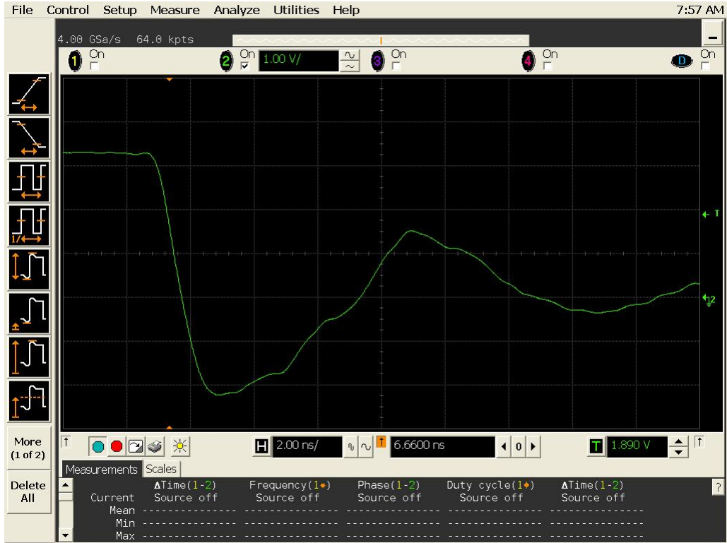
Figure 16a DUT 3259 Pre-Irradiation Falling Edge
