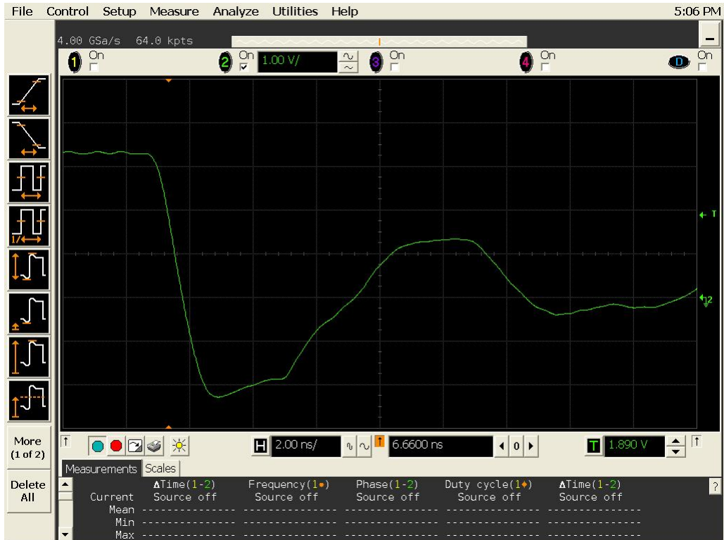
Figure 16b DUT 3259 Post-Annealing Falling Edge
