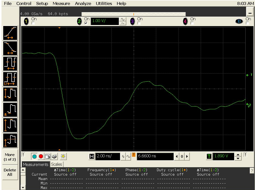
Figure 18a DUT 3299 Pre-Irradiation Falling Edge
