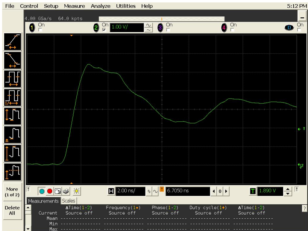
Figure 11b DUT 3298 Post-Annealing Rising edge
