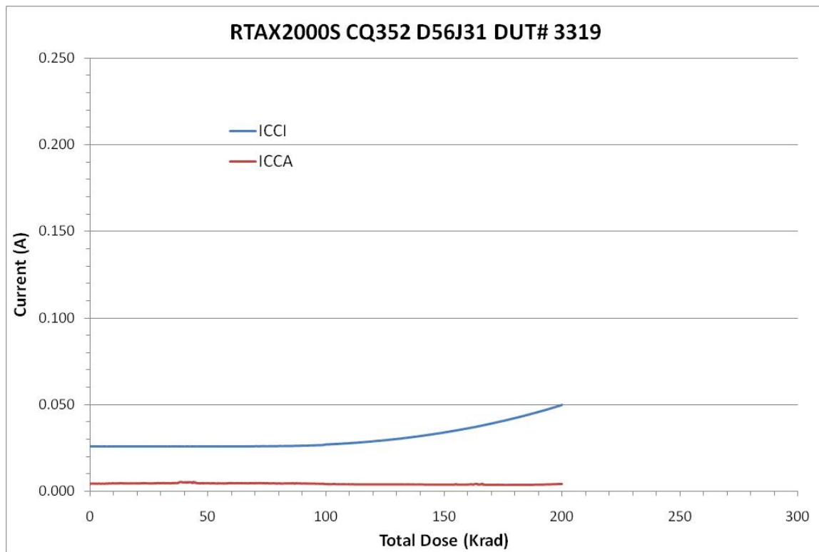
Figure 7 DUT 3319 Influx ICCA and ICCI
