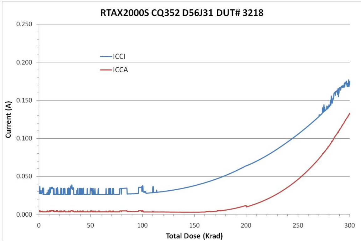
Figure 2 DUT 3218 Influx ICCA and ICCI (some measurement noises are present)
