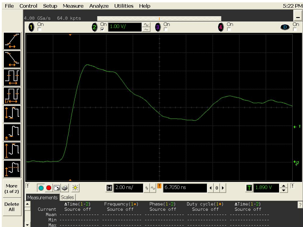
Figure 14b DUT 3319 Post-Annealing Rising Edge
