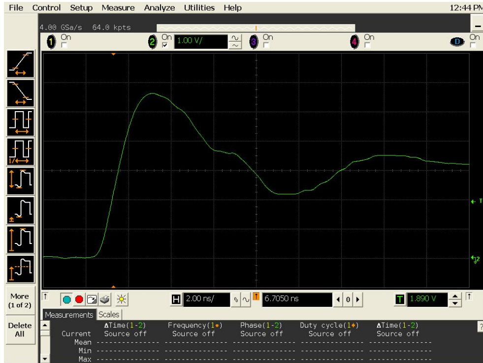
Figure 9a DUT 3218 Pre-Irradiation Rising Edge
