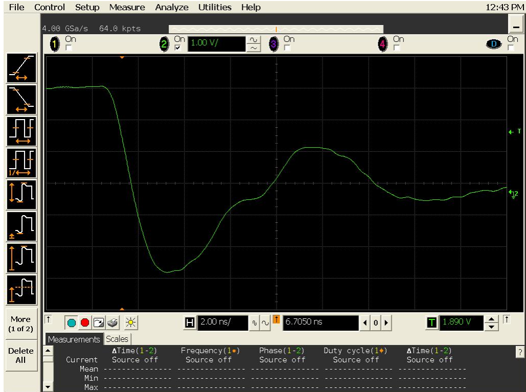
Figure 15a DUT 3218 Pre-Radiation Falling Edge
