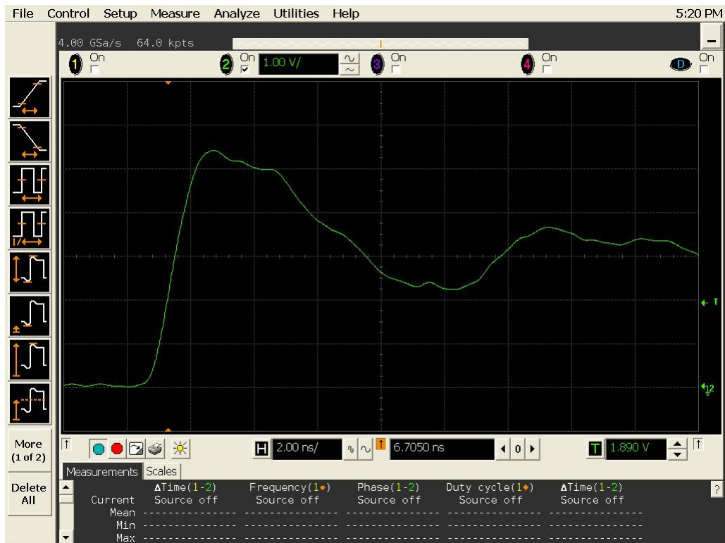
Figure 13b DUT 3303 Post-Annealing Rising Edge
