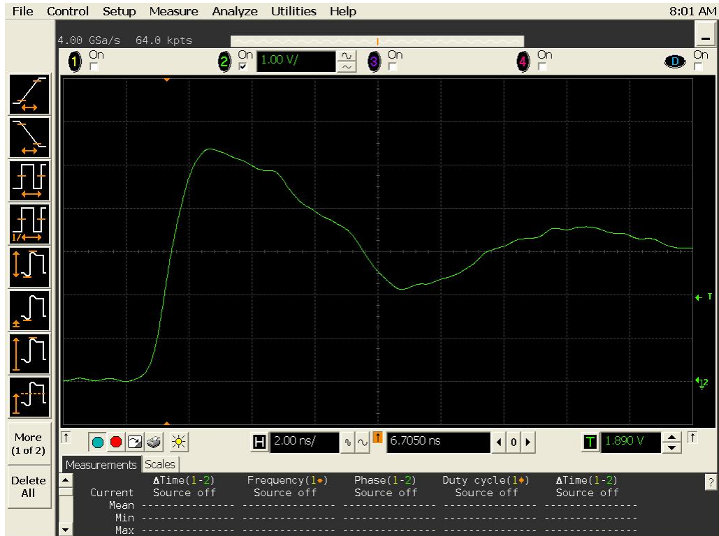
Figure 11a DUT 3298 Pre-Radiation Rising Edge
