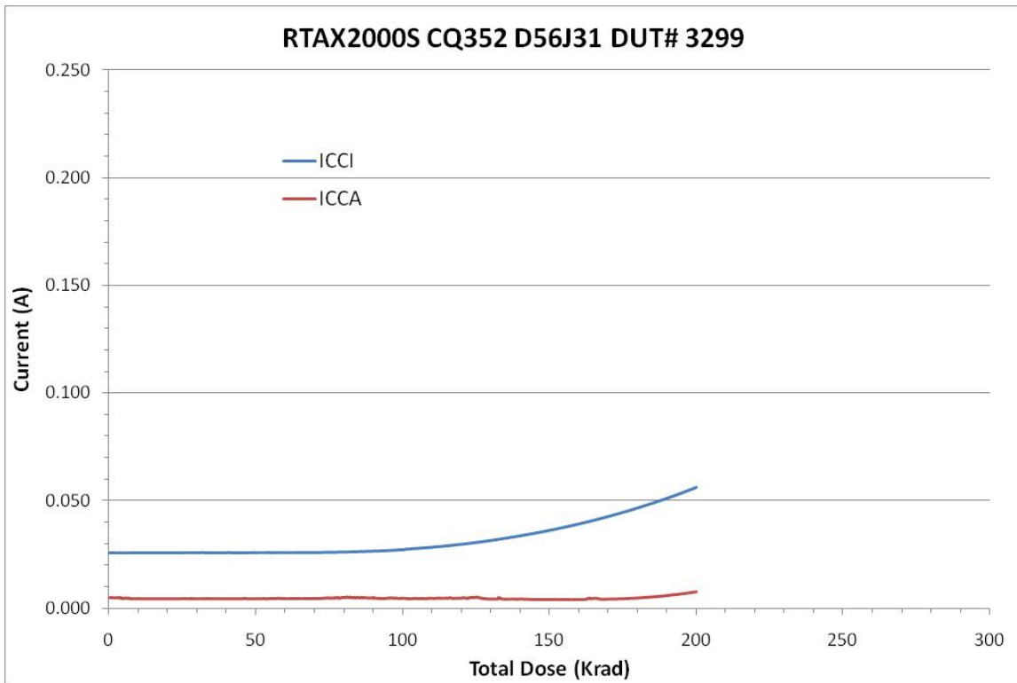
Figure 5 DUT 3299 Influx ICCA and ICCI
