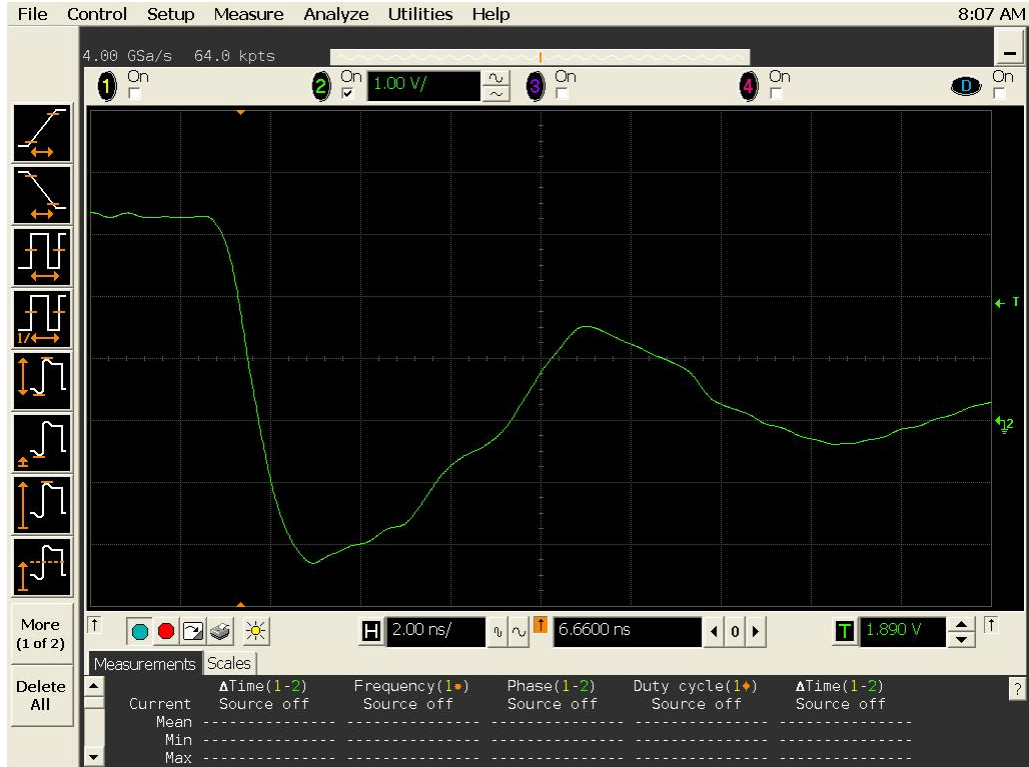
Figure 19a DUT 3303 Pre-Irradiation Falling Edge
