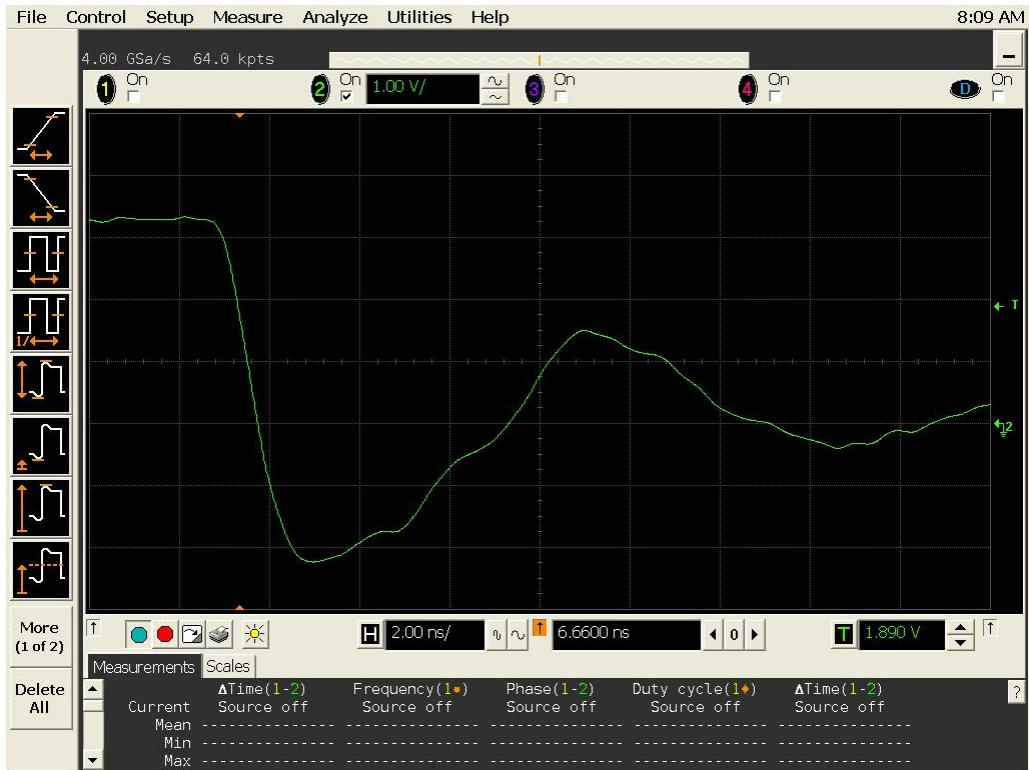
Figure 20a DUT 3319 Pre-Irradiation Falling Edge
