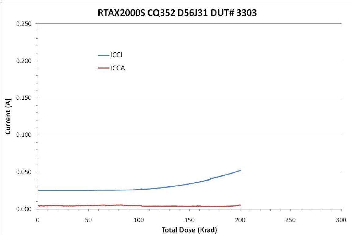
Figure 6 DUT 3303 Influx ICCA and ICCI
