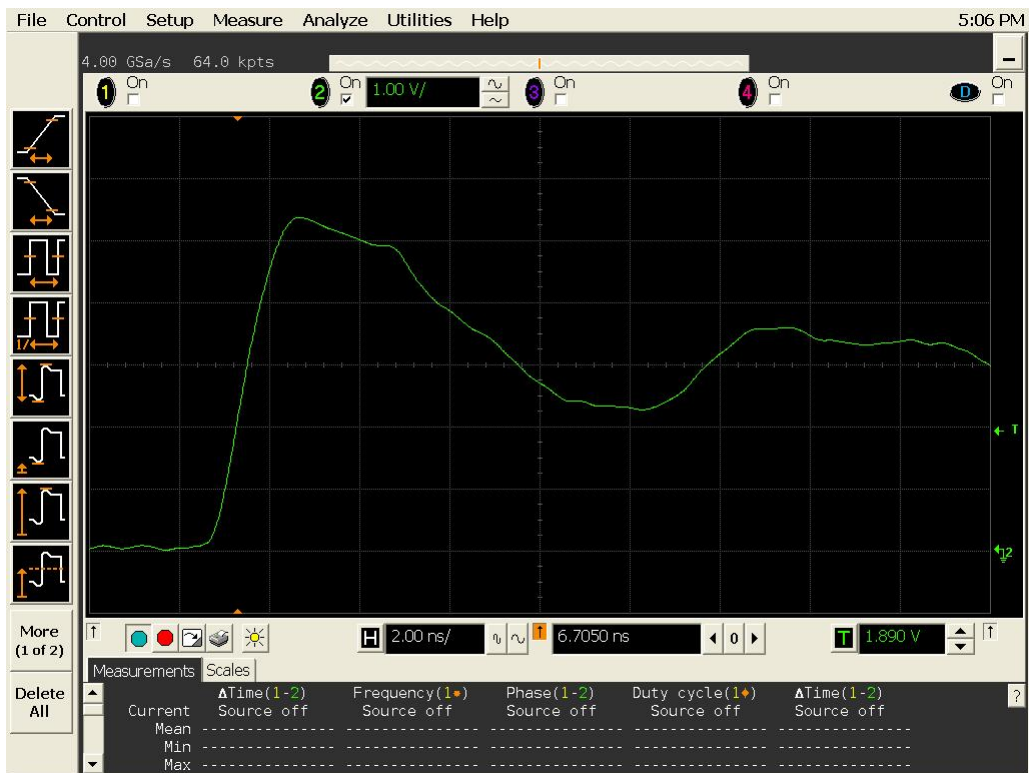
Figure 10b DUT 3259 Post-Annealing Rising Edge
