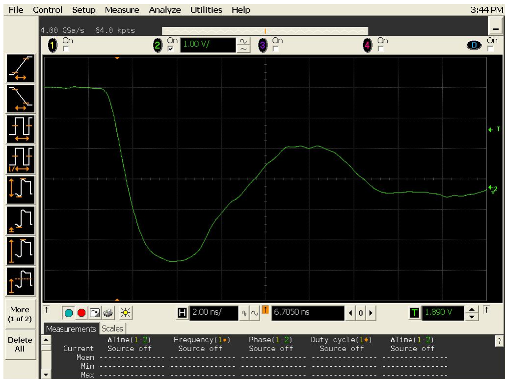
Figure 15b DUT 3218 Post-Annealing Falling Edge
