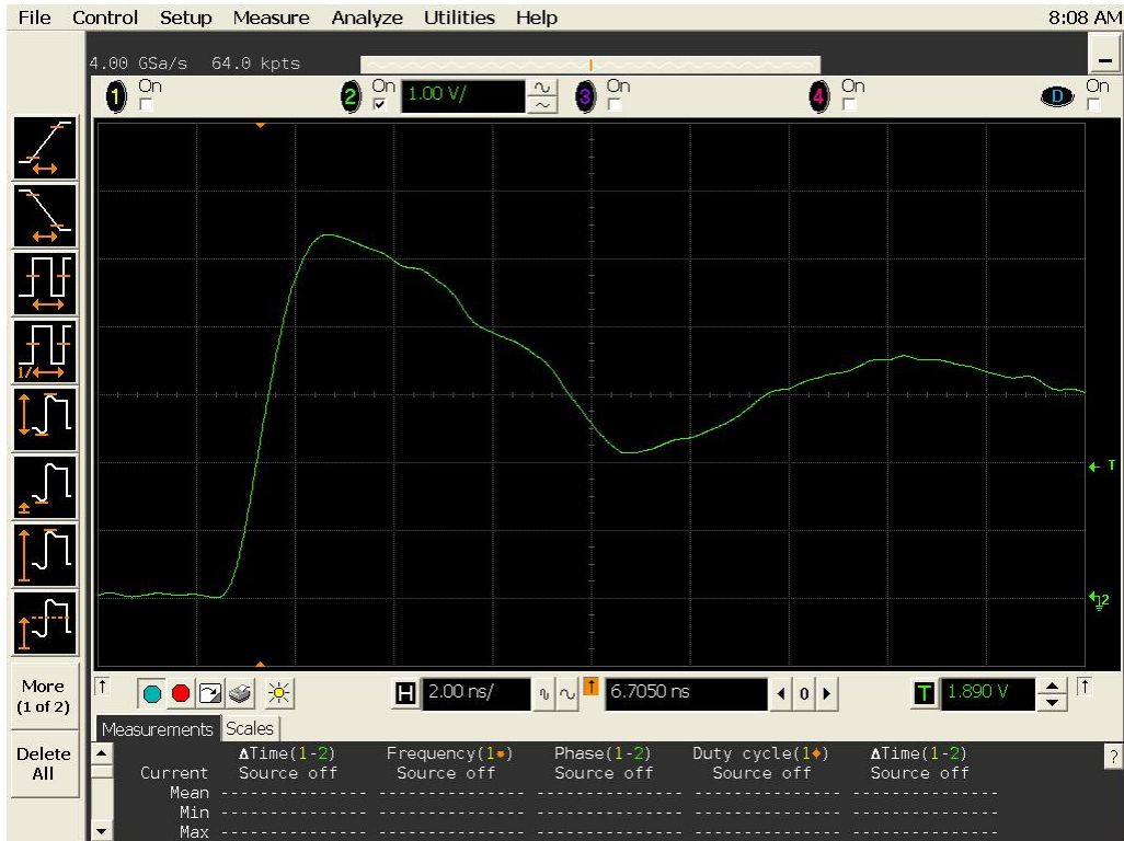
Figure 14a DUT 3319 Pre-Irradiation Rising Edge
