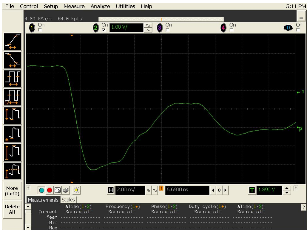
Figure 17b DUT 3298 Post-Annealing Falling Edge
