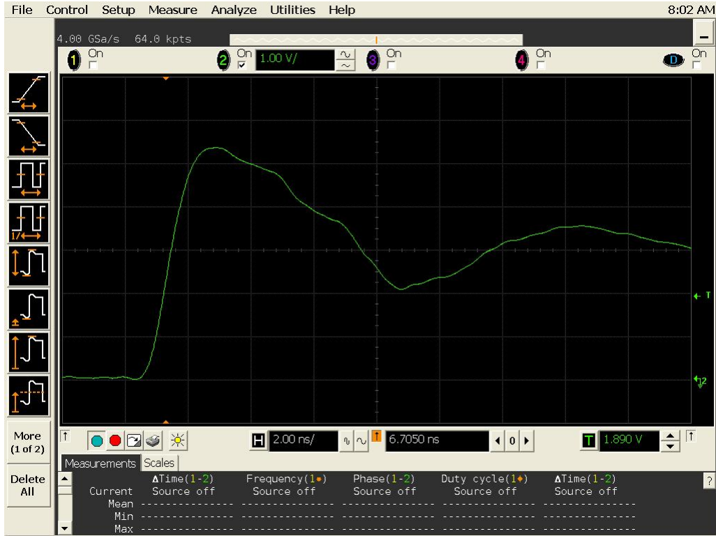
Figure 12a DUT 3299 Pre-Irradiation Rising Edge
