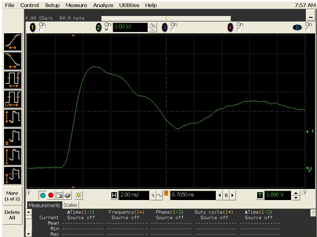
Figure 10a DUT 3259 Pre-Irradiation Rising Edge
