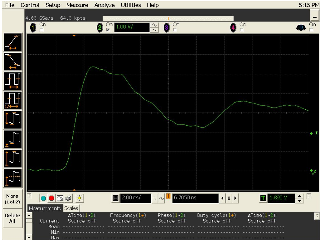
Figure 12b DUT 3299 Post-Annealing Rising Edge
