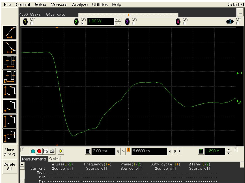
Figure 18b DUT 3299 Post-Annealing Falling Edge
