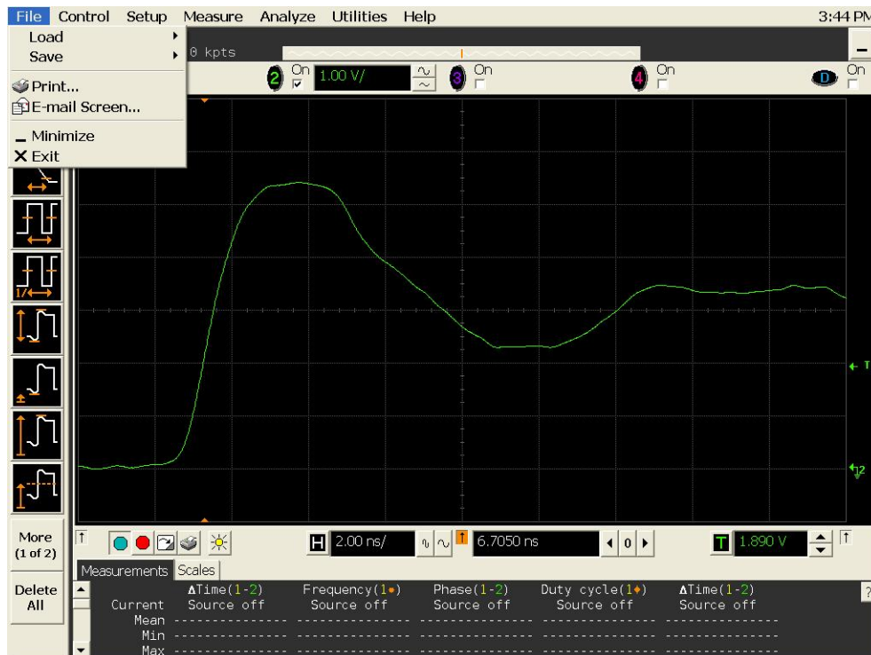
Figure 9b DUT 3218 Post-Annealing Rising Edge
