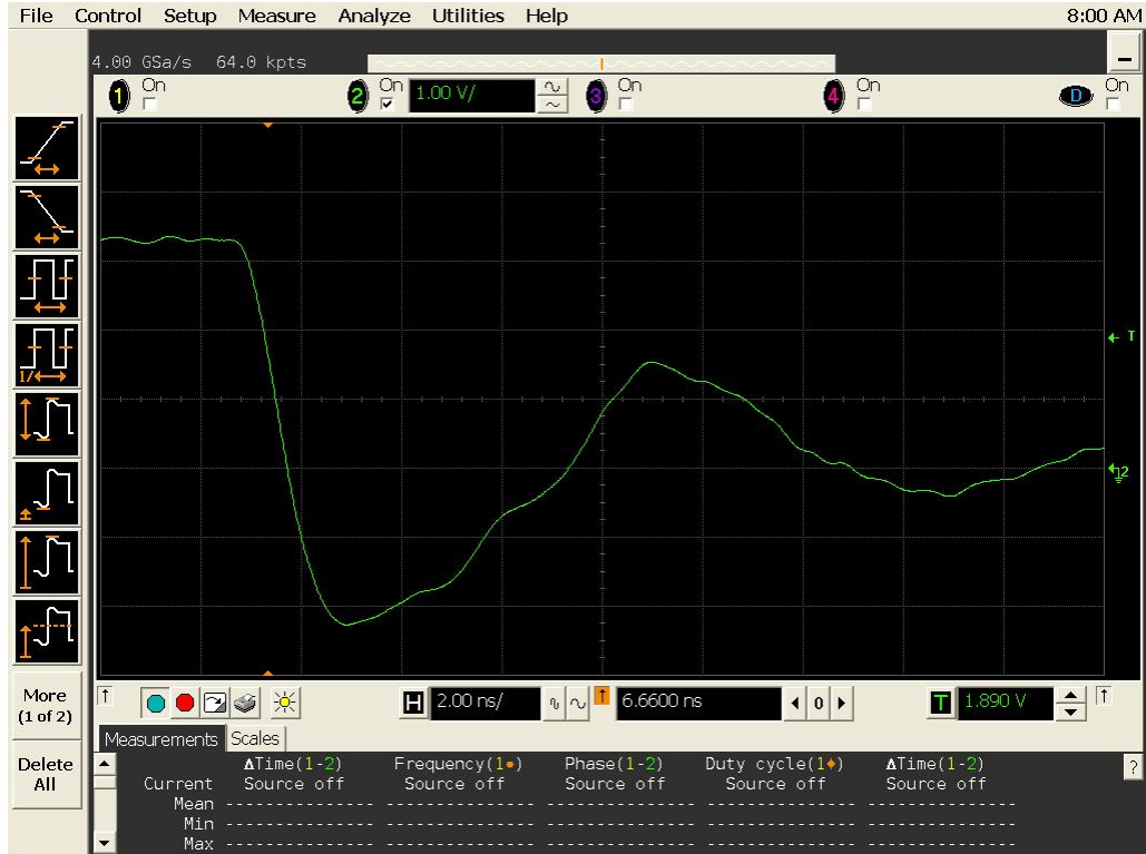
Figure 17a DUT 3298 Pre-Irradiation Falling Edge
