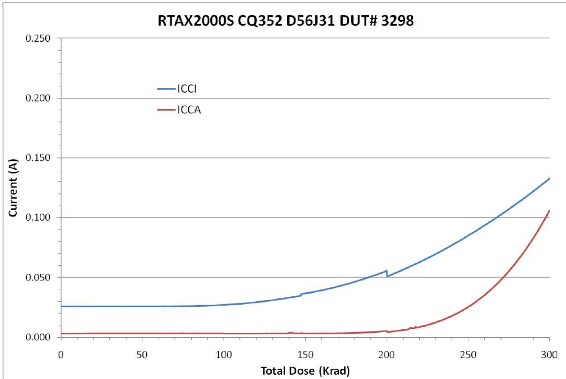
Figure 4 DUT 3298 Influx ICCA and ICCI
