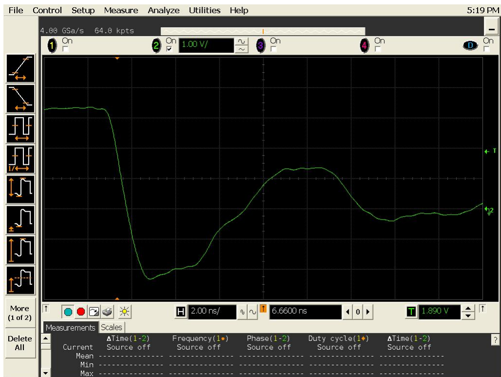
Figure 19b DUT 3303 Post-Annealing Falling Edge
