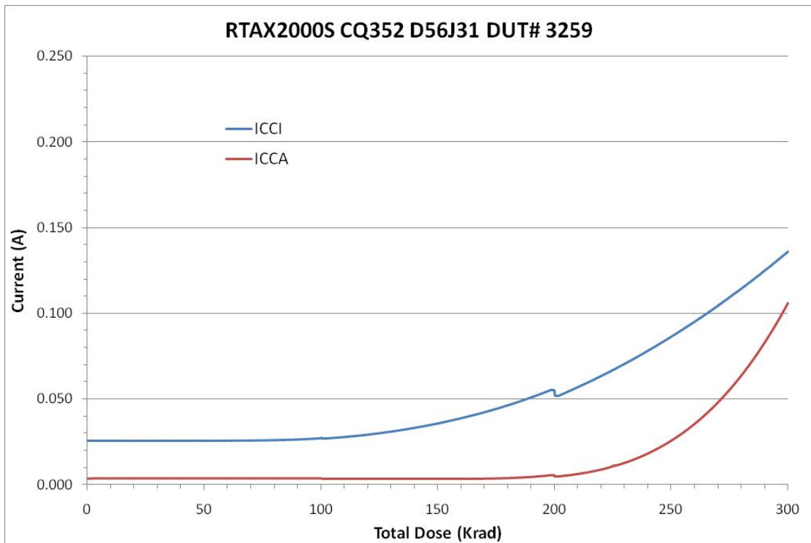
Figure 3 DUT 3259 Influx ICCA and ICCI
