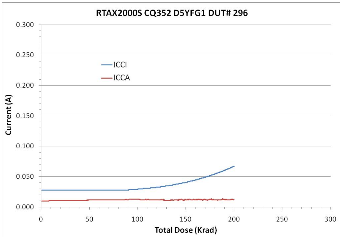
Figure 7 DUT 296 Influx ICCA and ICCI
