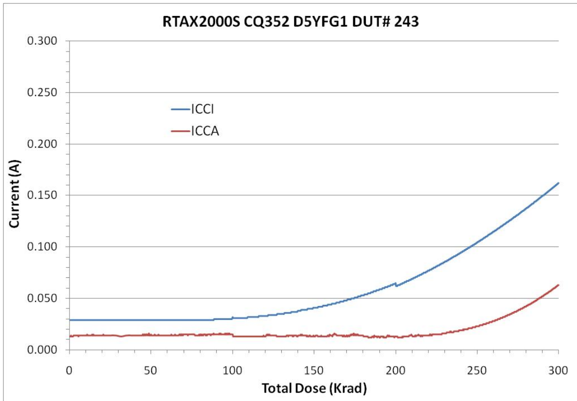
Figure 3 DUT 243 Influx ICCA and ICCI
