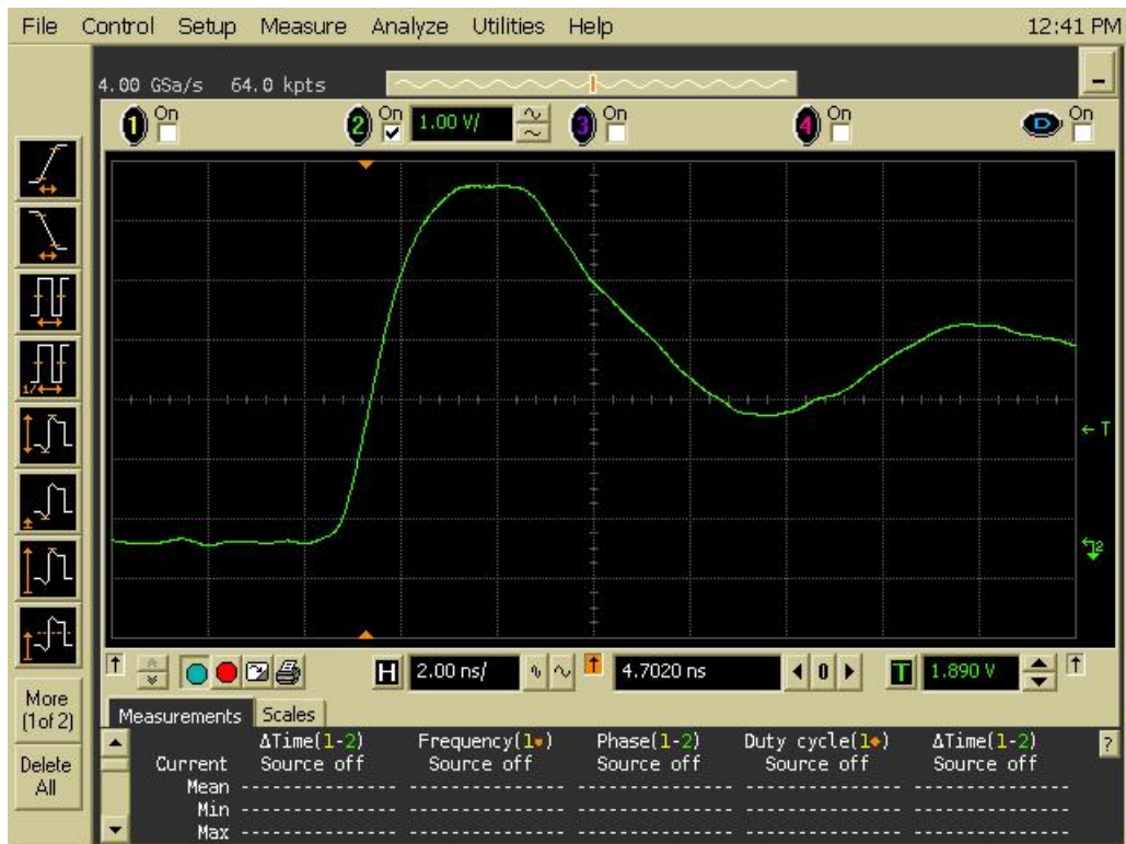
Figure 13b DUT 275 Post-Annealing Rising Edge
