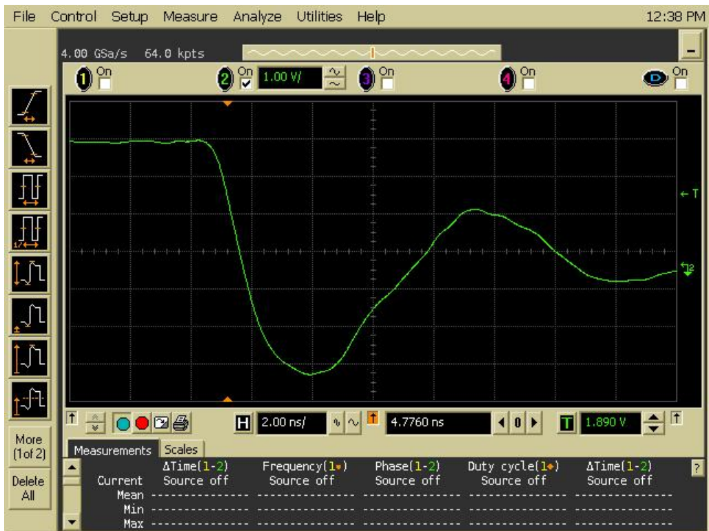
Figure 18b DUT 261 Post-Annealing Falling Edge
