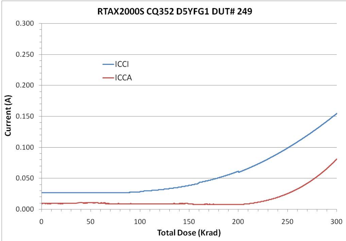
Figure 4 DUT 249 Influx ICCA and ICCI
