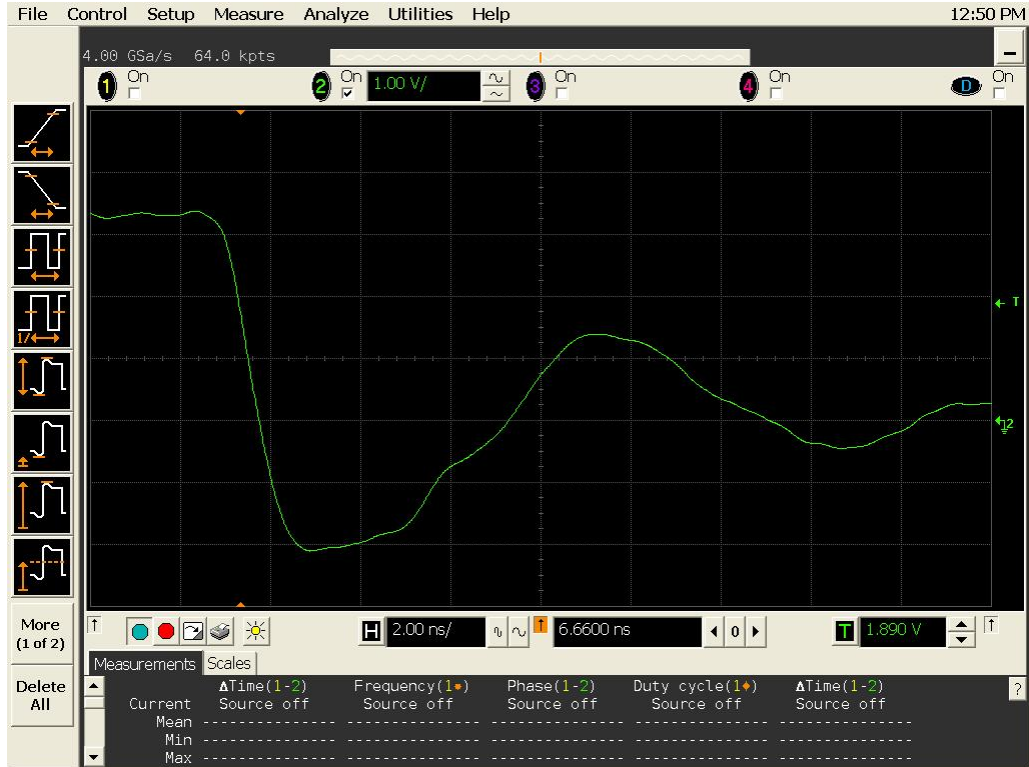
Figure 15a DUT 209 Pre-Radiation Falling Edge
