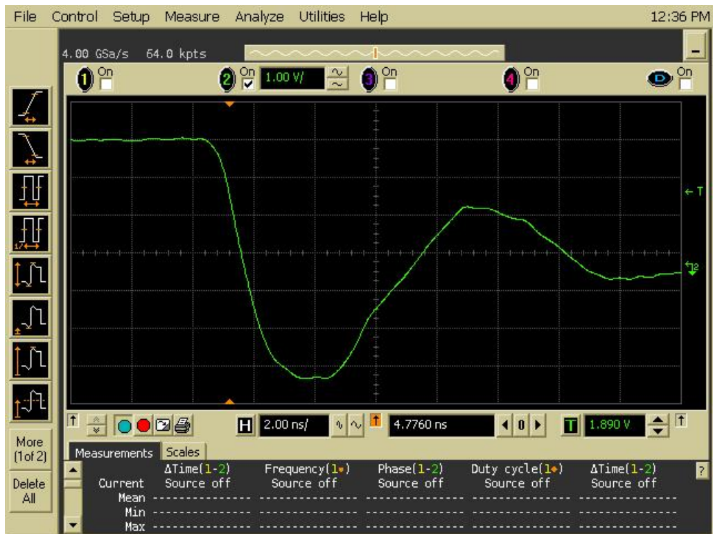
Figure 17b DUT 249 Post-Annealing Falling Edge
