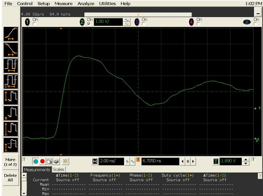
Figure 13a DUT 275 Pre-Irradiation Rising Edge
