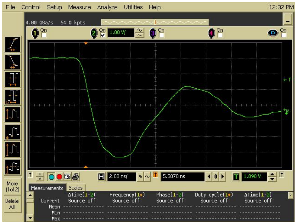
Figure 15b DUT 209 Post-Annealing Falling Edge
