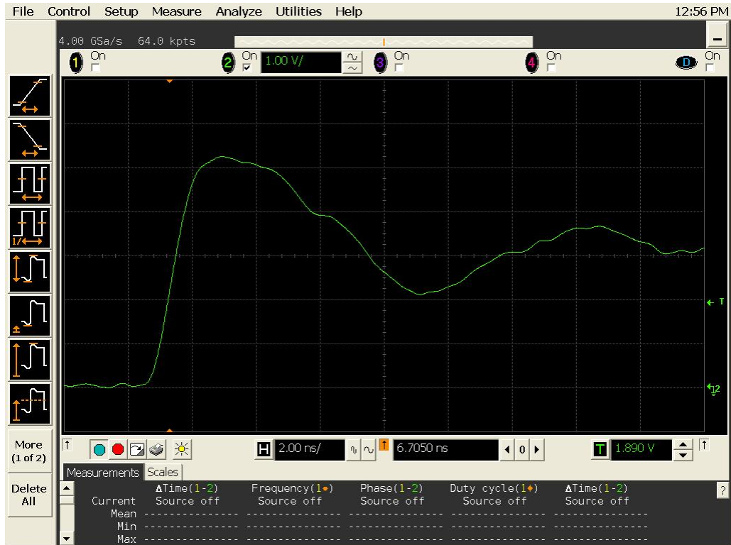
Figure 11a DUT 249 Pre-Radiation Rising Edge
