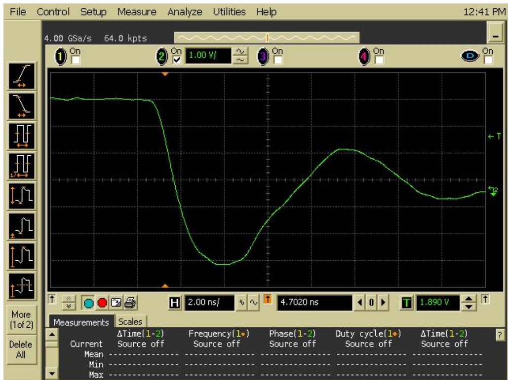
Figure 19b DUT 275 Post-Annealing Falling Edge
