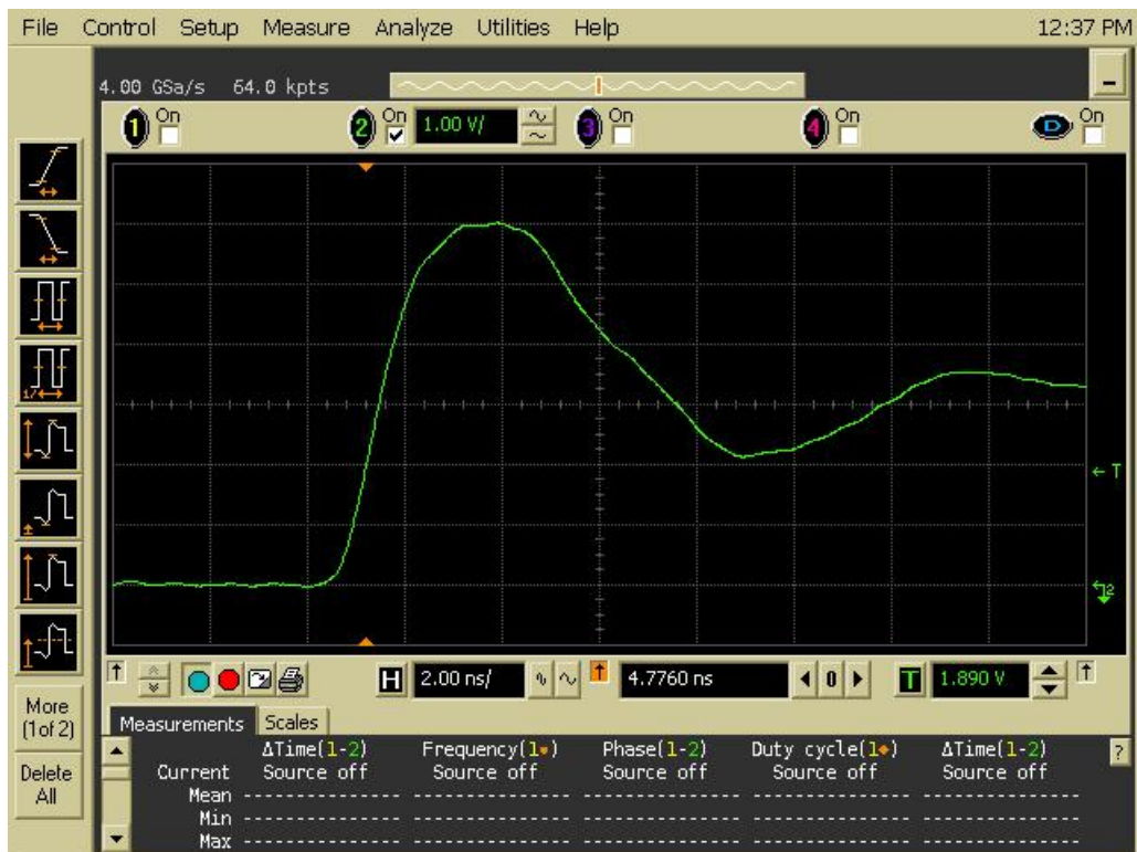
Figure 11b DUT 249 Post-Annealing Rising edge
