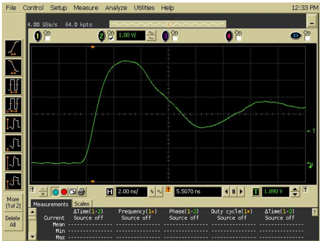
Figure 10b DUT 243 Post-Annealing Rising Edge
