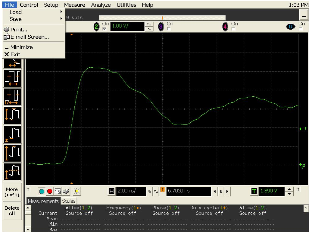
Figure 14a DUT 296 Pre-Irradiation Rising Edge
