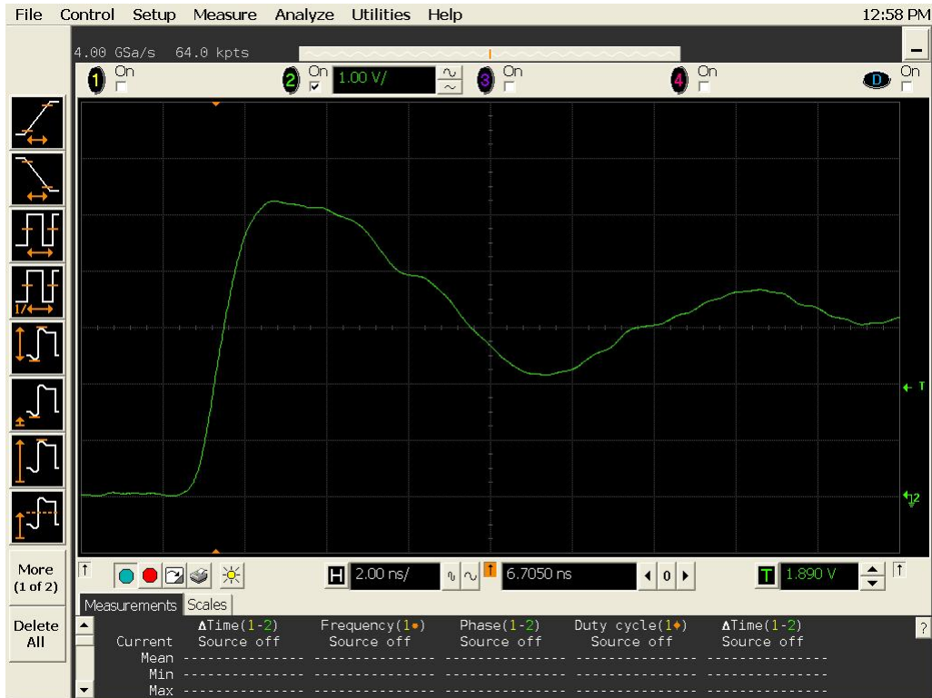
Figure 12a DUT 261 Pre-Irradiation Rising Edge
