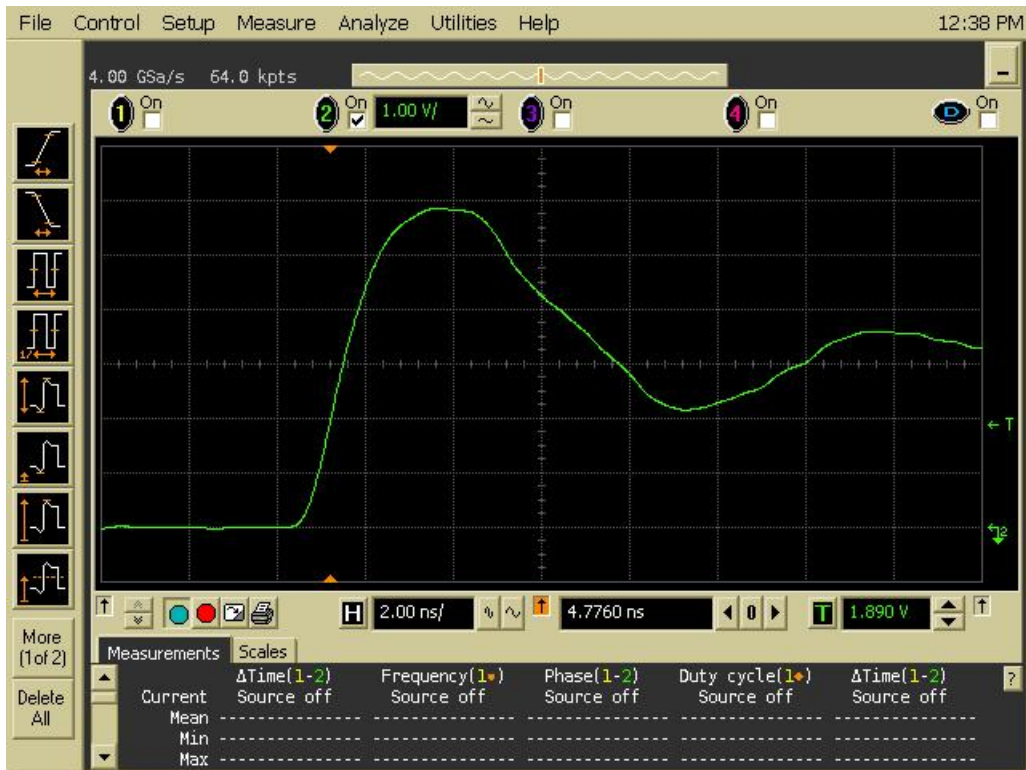
Figure 12b DUT 261 Post-Annealing Rising Edge
