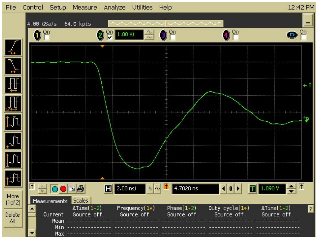
Figure 20b DUT 296 Post-Annealing Falling Edge
