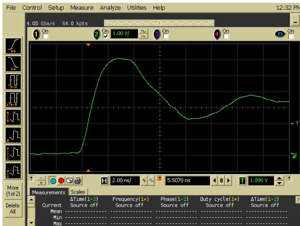
Figure 9b DUT 209 Post-Annealing Rising Edge
