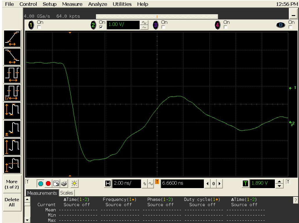
Figure 17a DUT 249 Pre-Irradiation Falling Edge
