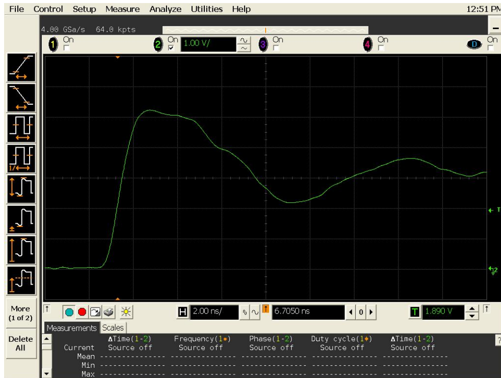
Figure 9a DUT 209 Pre-Irradiation Rising Edge
