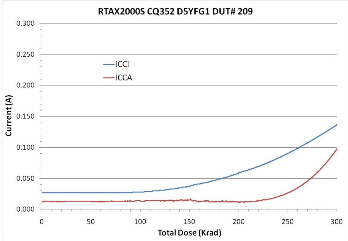
Figure 2 DUT 209 Influx ICCA and ICCI
