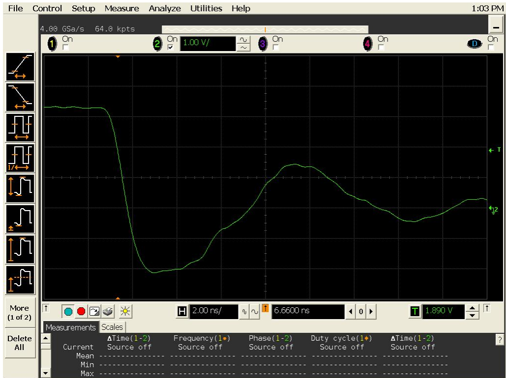
Figure 20a DUT 296 Pre-Irradiation Falling Edge
