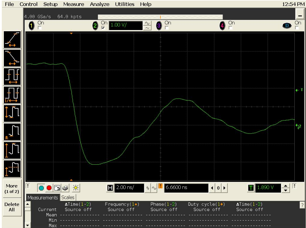
Figure 16a DUT 243 Pre-Irradiation Falling Edge
