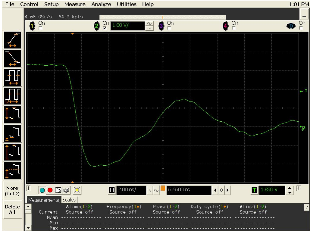
Figure 19a DUT 275 Pre-Irradiation Falling Edge
