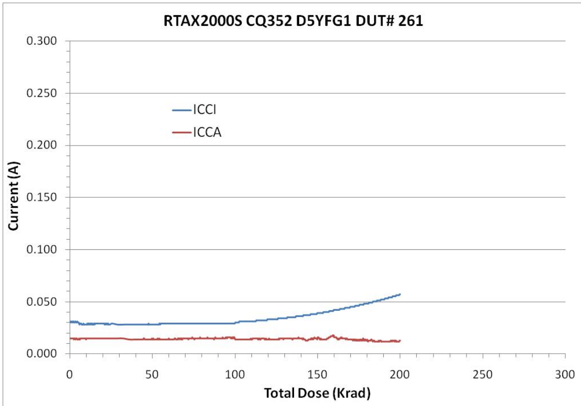
Figure 5 DUT 261 Influx ICCA and ICCI
