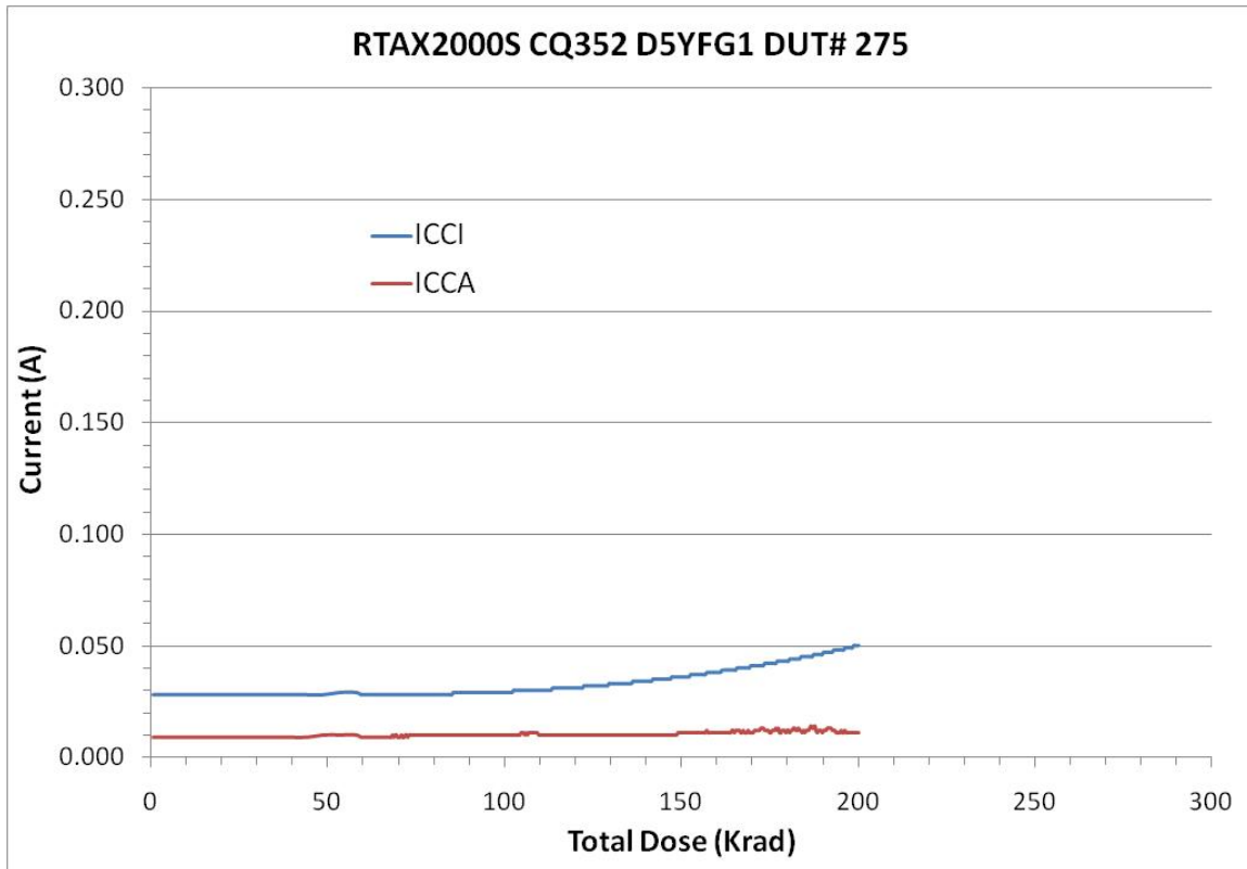
Figure 6 DUT 275 Influx ICCA and ICCI
