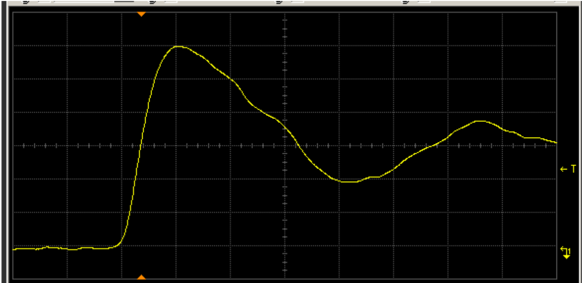
Figure 9(a) DUT 4139 pre-irradiation rising edge. The ordinate is 1 V/div, and abscissa 2 ns/div.
