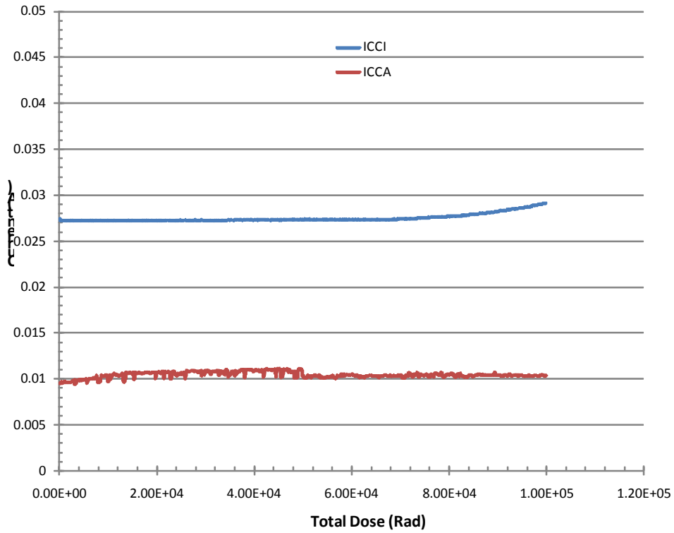
Figure 7 DUT 4149 in-flux I_{CCA} and I_{CCI} .
