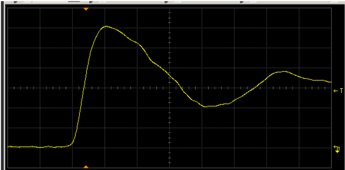
Figure 11(b) DUT 4142 post-annealing rising edge. The ordinate is 1 V/div, and abscissa 2 ns/div.
