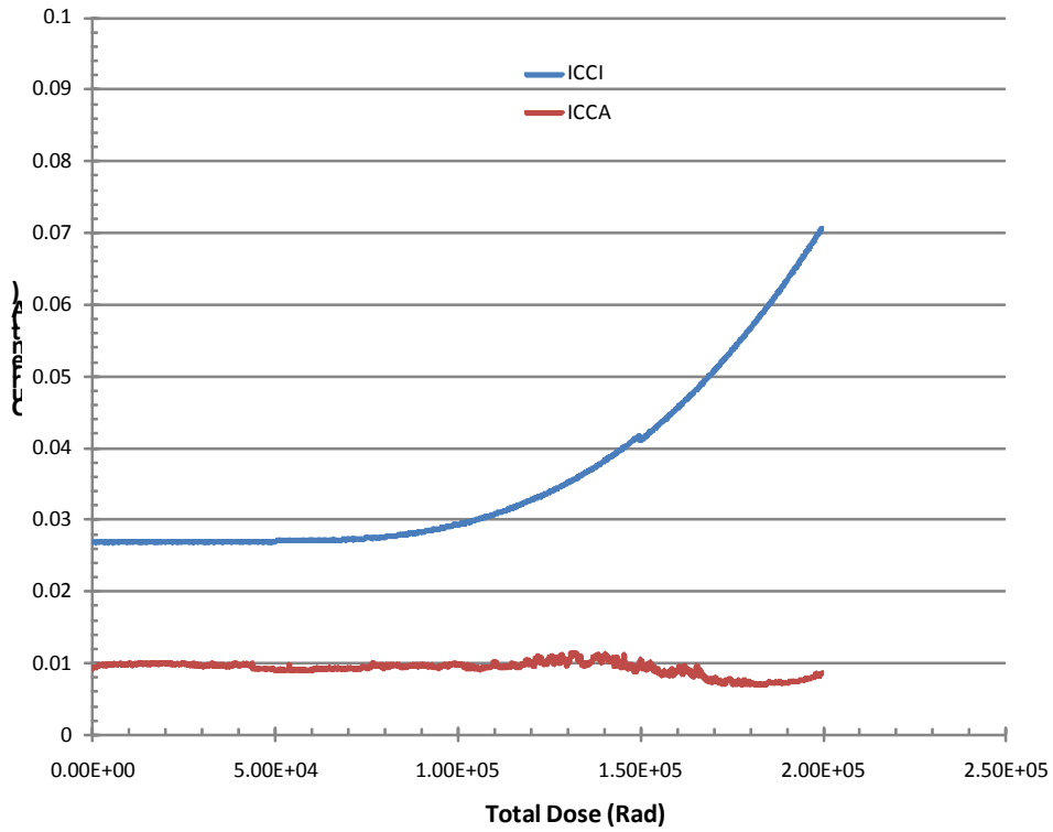
Figure 5 DUT 4146 in-flux I_{CCA} and I_{CCI} .
