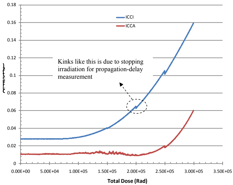
Figure 2 DUT 4139 in-flux I_{CCA} and I_{CCI} .
