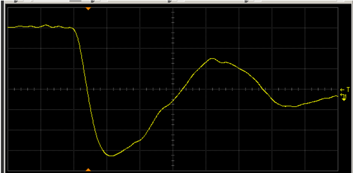
Figure 14(b) DUT 4140 post-annealing falling edge. The ordinate is 1 V/div, and abscissa 2 ns/div.
