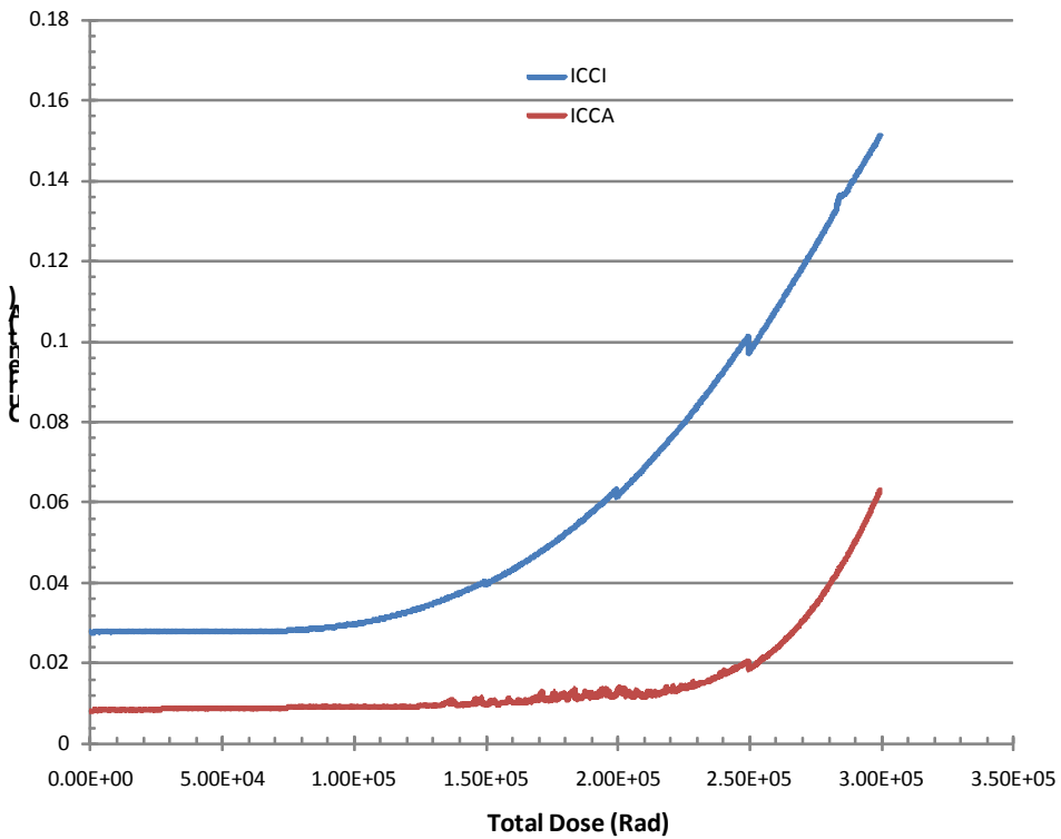
Figure 3 DUT 4140 in-flux I_{CCA} and I_{CCI} .
