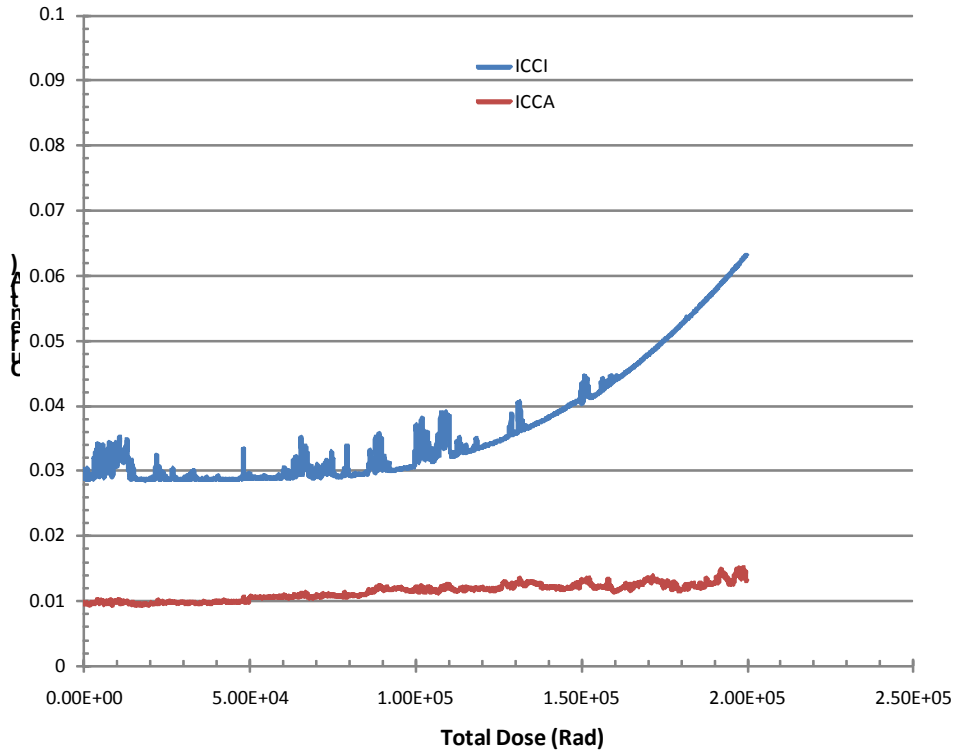
Figure 4 DUT 4142 in-flux I_{CCA} and I_{CCI} .
