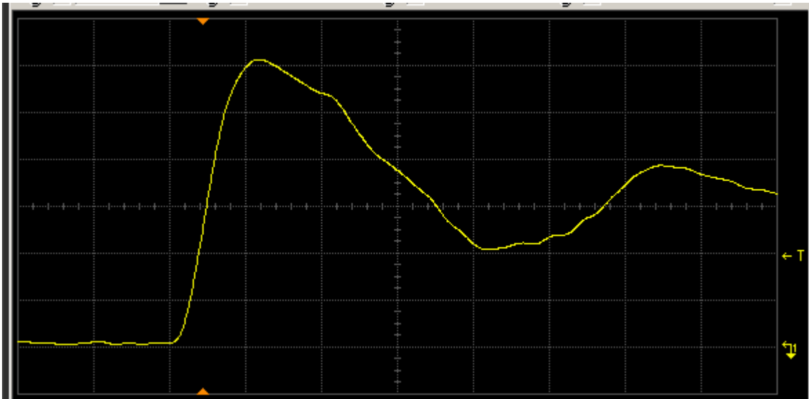
Figure 10(b) DUT 4140 post-annealing rising edge. The ordinate is 1 V/div, and abscissa 2 ns/div.
