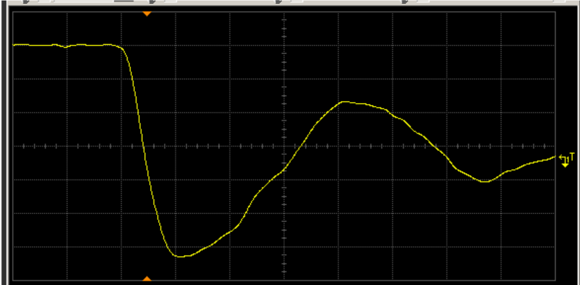
Figure 16(a) DUT 4146 pre-irradiation falling edge. The ordinate is 1 V/div, and abscissa 2 ns/div.
