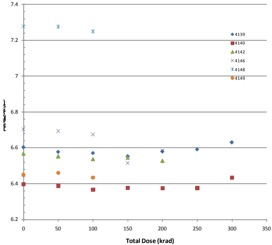
Figure 8 In-situ propagation delay versus total dose. The measurement was performed when irradiation was temporarily stopped.
