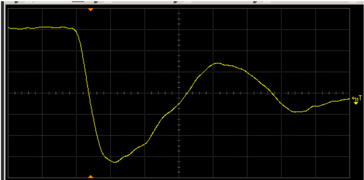
Figure 15(a) DUT 4142 pre-radiation falling edge. The ordinate is 1 V/div, and abscissa 2 ns/div.
