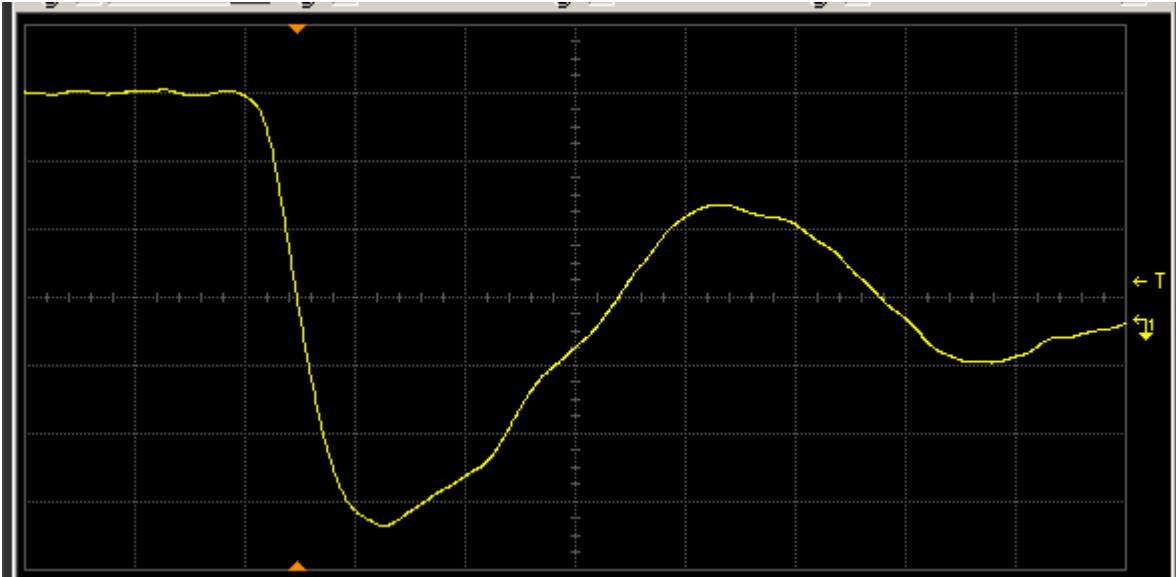
Figure 16(b) DUT 4146 post-annealing falling edge. The ordinate is 1 V/div, and abscissa 2 ns/div.
