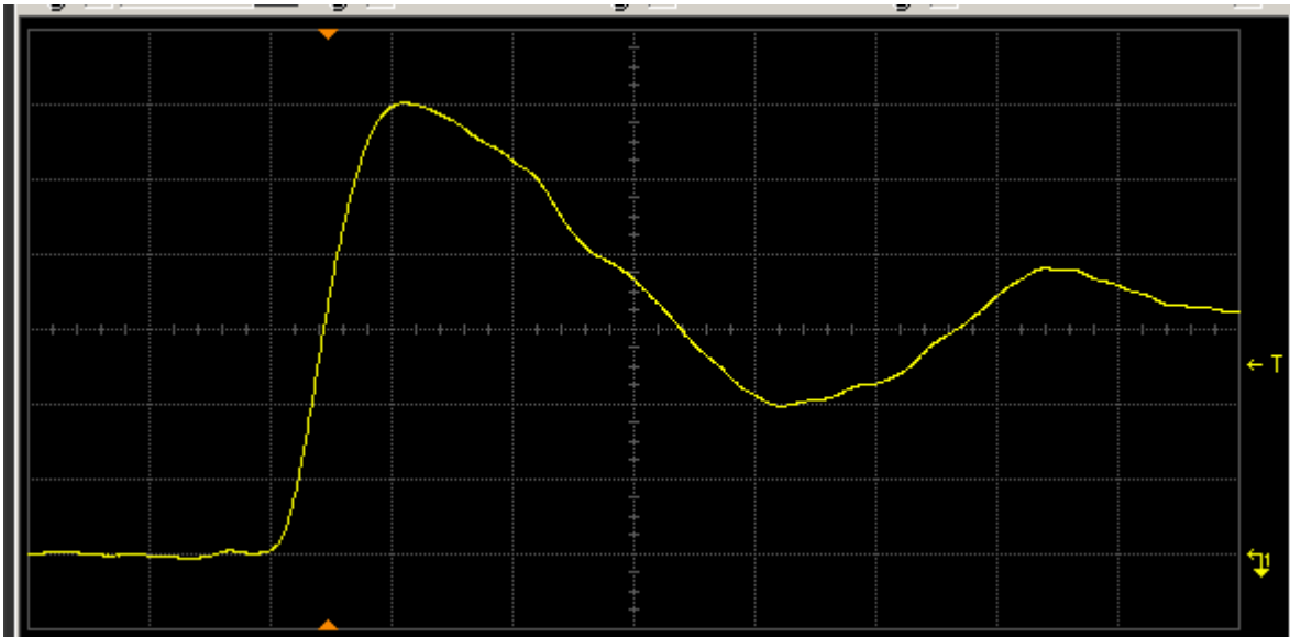
Figure 12(b) DUT 4146 post-annealing rising edge. The ordinate is 1 V/div, and abscissa 2 ns/div.
