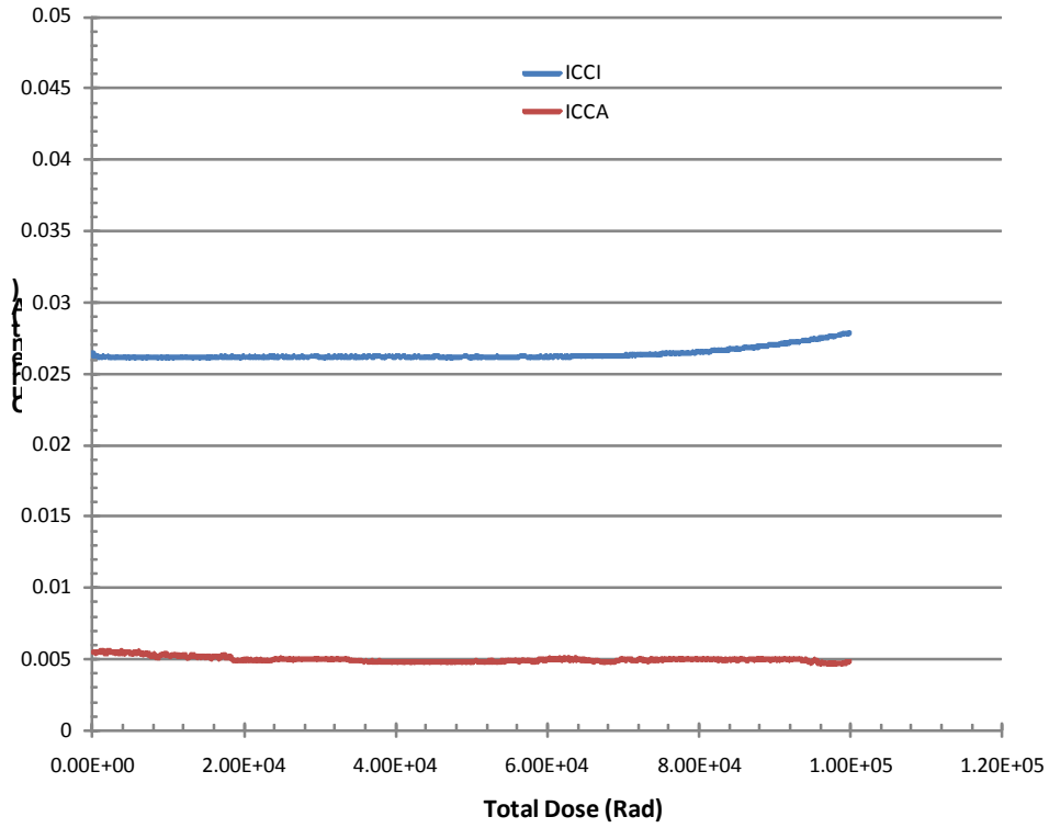
Figure 6 DUT 4148 in-flux I_{CCA} and I_{CCI} .
