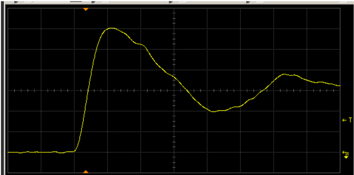
Figure 10(a) DUT 4140 pre-irradiation rising edge. The ordinate is 1 V/div, and abscissa 2 ns/div.
