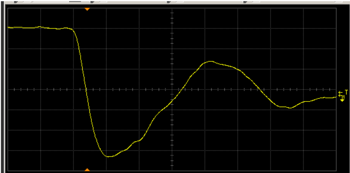
Figure 15(b) DUT 4142 post-annealing falling edge. The ordinate is 1 V/div, and abscissa 2 ns/div.
