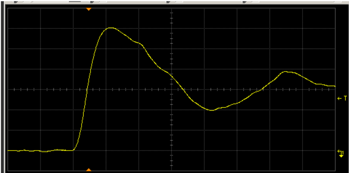
Figure 12(a) DUT 4146 pre-irradiation rising edge. The ordinate is 1 V/div, and abscissa 2 ns/div.
