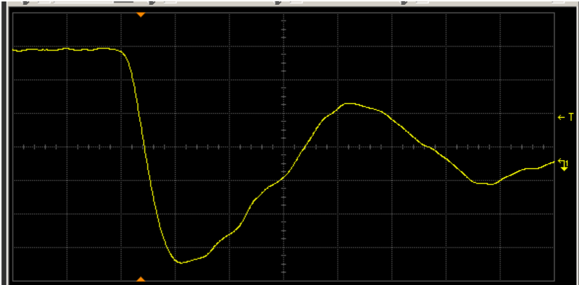
Figure 13(a) DUT 4139 pre-irradiation falling edge. The ordinate is 1 V/div, and abscissa 2 ns/div.
