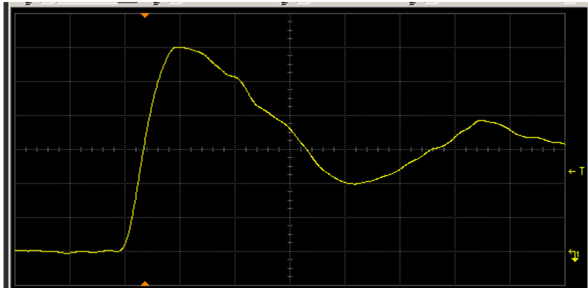
Figure 9(b) DUT 4139 post-annealing rising edge. The ordinate is 1 V/div, and abscissa 2 ns/div.
