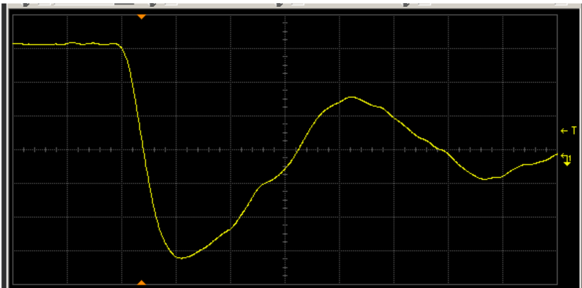
Figure 13(b) DUT 4139 post-annealing falling edge. The ordinate is 1 V/div, and abscissa 2 ns/div.
