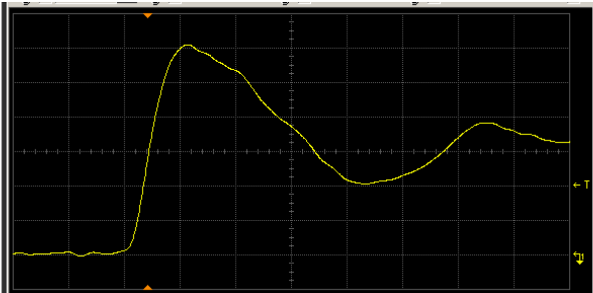
Figure 11(a) DUT 4142 pre-radiation rising edge. The ordinate is 1 V/div, and abscissa 2 ns/div.
