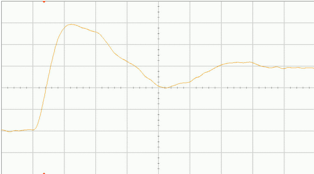
Figure 9(b) DUT 8514 post-annealing rising edge, abscissa scale is 1 V/div and ordinate scale is 2 ns/div.
