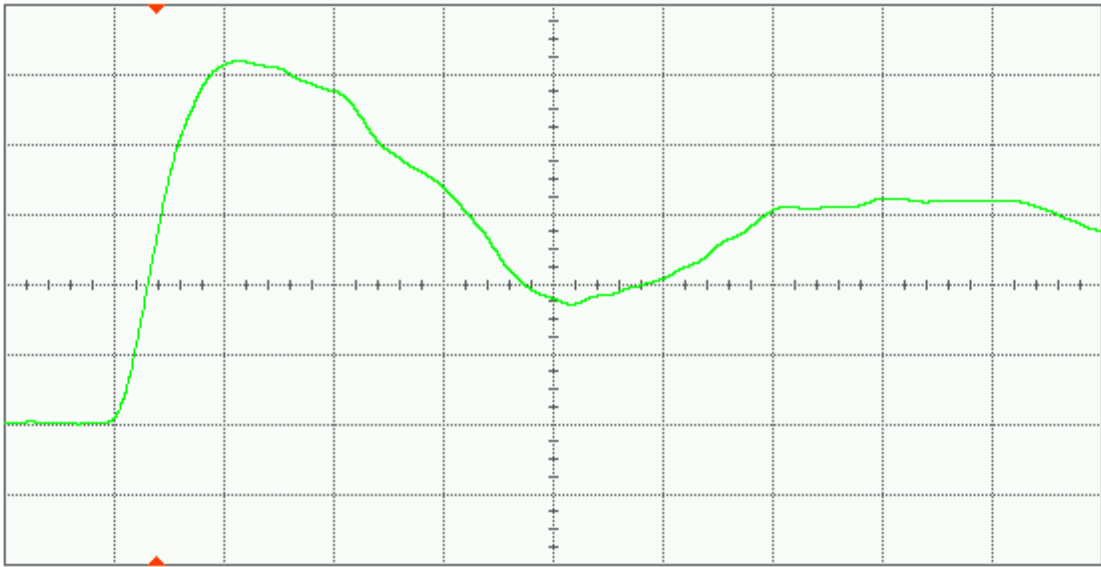
Figure 13(a) DUT 8547 pre-irradiation rising edge, abscissa scale is 1 V/div and ordinate scale is 2 ns/div.
