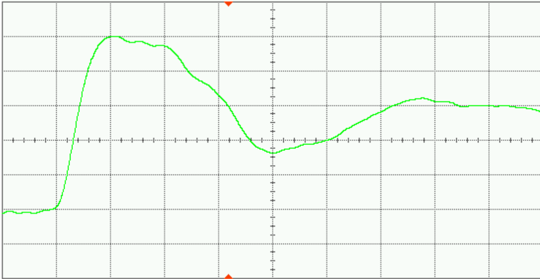
Figure 8(a) DUT 8510 pre-irradiation rising edge, abscissa scale is 1 V/div and ordinate scale is 2 ns/div.
