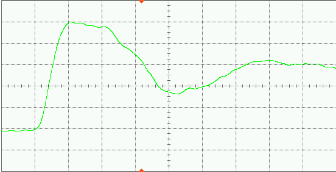
Figure 9(a) DUT 8514 pre-irradiation rising edge, abscissa scale is 1 V/div and ordinate scale is 2 ns/div.
