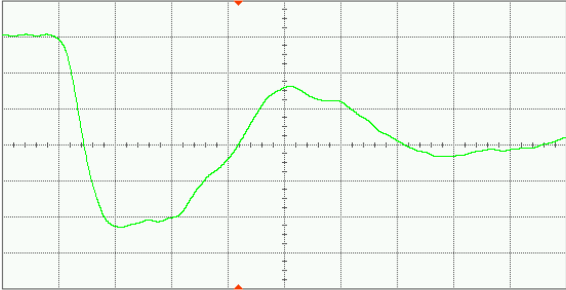
Figure 15(a) DUT 8514 pre-irradiation falling edge, abscissa scale is 1 V/div and ordinate scale is 2 ns/div.
