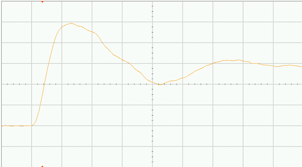
Figure 11(b) DUT 8533 post-annealing rising edge, abscissa scale is 1 V/div and ordinate scale is 2 ns/div.
