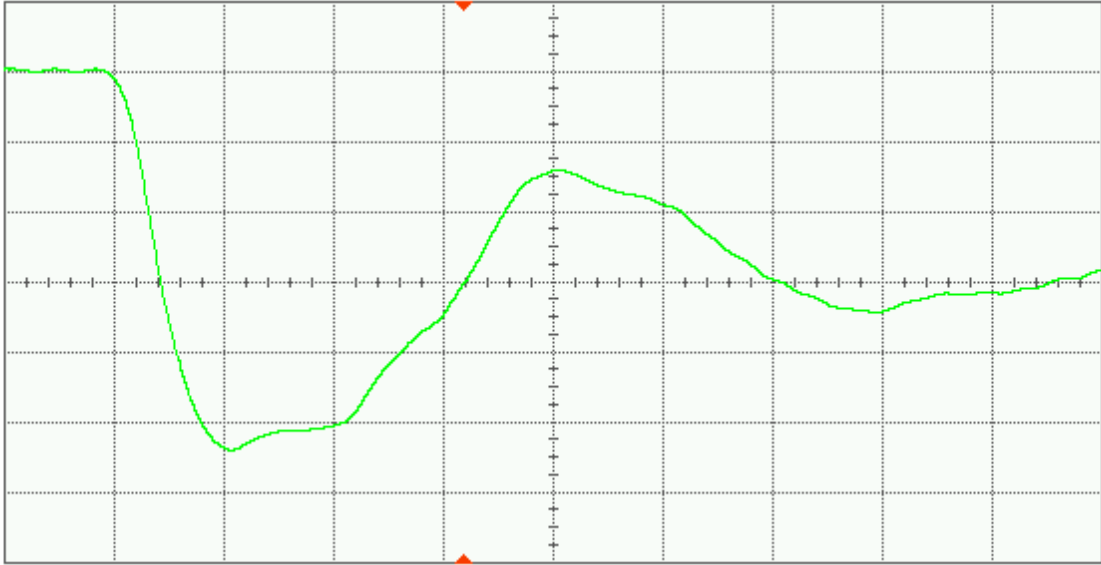
Figure 14(a) DUT 8510 pre-irradiation falling edge, abscissa scale is 1 V/div and ordinate scale is 2 ns/div.
