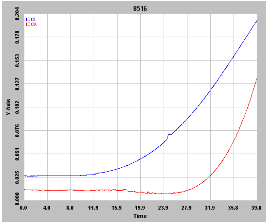
Figure 4 DUT 8516 in-flux I_{CCA} and I_{CCI} . The unit of time is in minutes.
