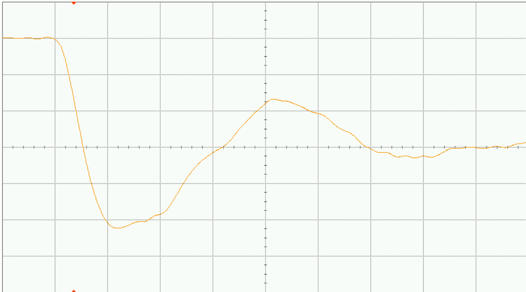
Figure 18(b) DUT 8536 pre-irradiation falling edge, abscissa scale is 1 V/div and ordinate scale is 2 ns/div.
