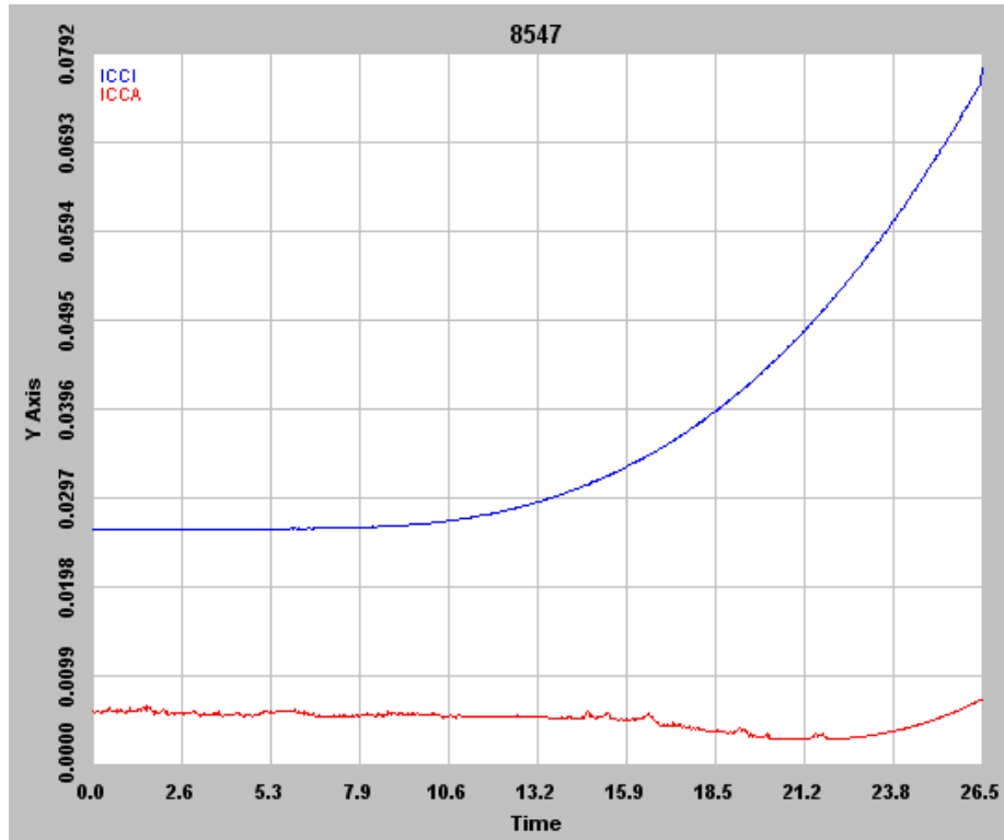
Figure 7 DUT 8547 in-flux I_{CCA} and I_{CCI} . The unit of time is in minutes.
