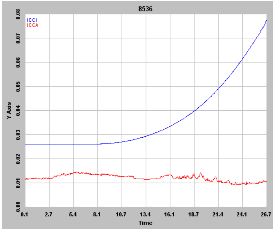
Figure 6 DUT 8536 in-flux I_{CCA} and I_{CCI} . The unit of time is in minutes.
