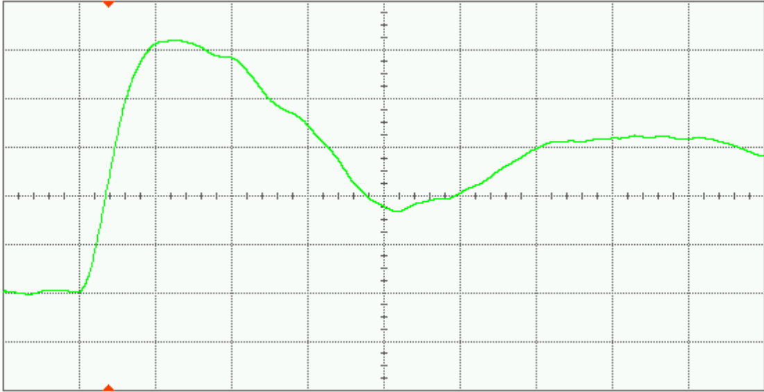
Figure 10(a) DUT 8516 pre-radiation rising edge, abscissa scale is 1 V/div and ordinate scale is 2 ns/div.
