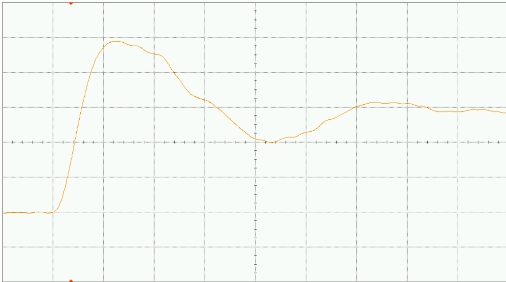
Figure 13(b) DUT 8547 post-annealing rising edge, abscissa scale is 1 V/div and ordinate scale is 2 ns/div.
