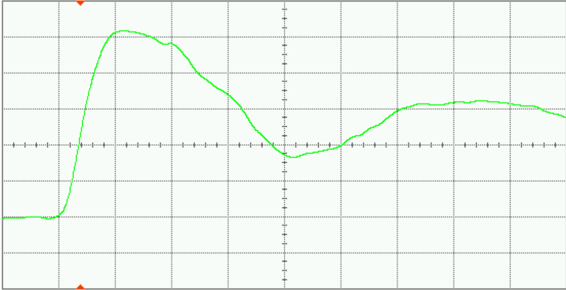
Figure 12(a) DUT 8536 pre-irradiation rising edge, abscissa scale is 1 V/div and ordinate scale is 2 ns/div.
