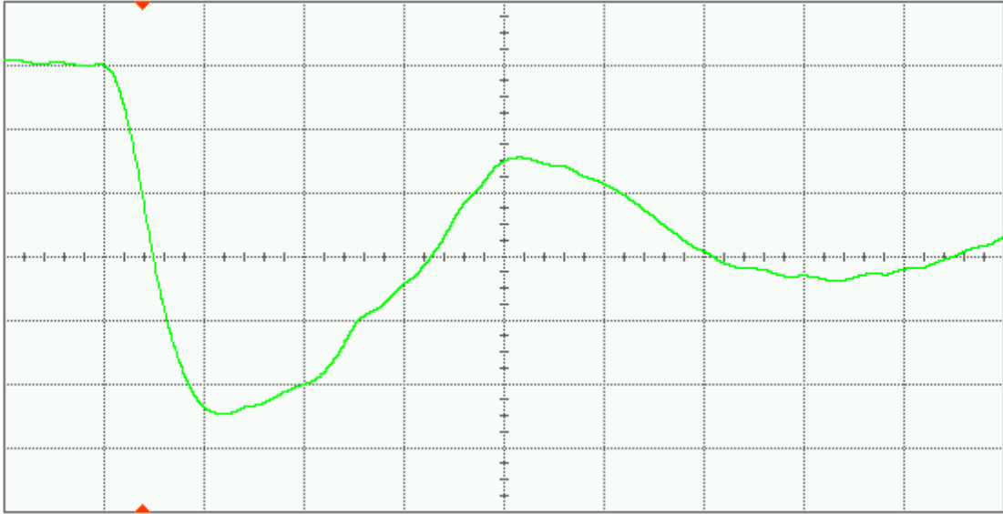
Figure 17(a) DUT 8533 pre-irradiation falling edge, abscissa scale is 1 V/div and ordinate scale is 2 ns/div.
