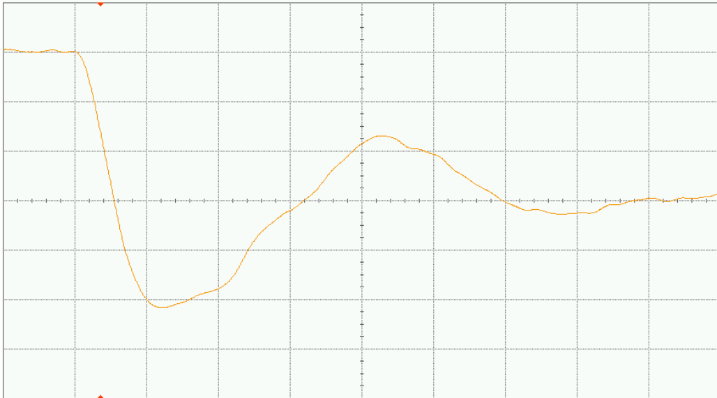
Figure 17(b) DUT 8533 post-annealing falling edge, abscissa scale is 1 V/div and ordinate scale is 2 ns/div.
