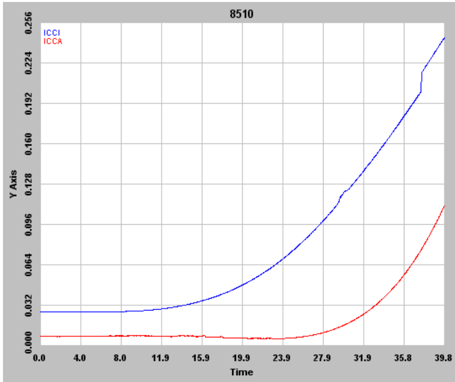
Figure 2 DUT 8510 in-flux I_{CCA} and I_{CCI} . The unit of time is in minutes.
