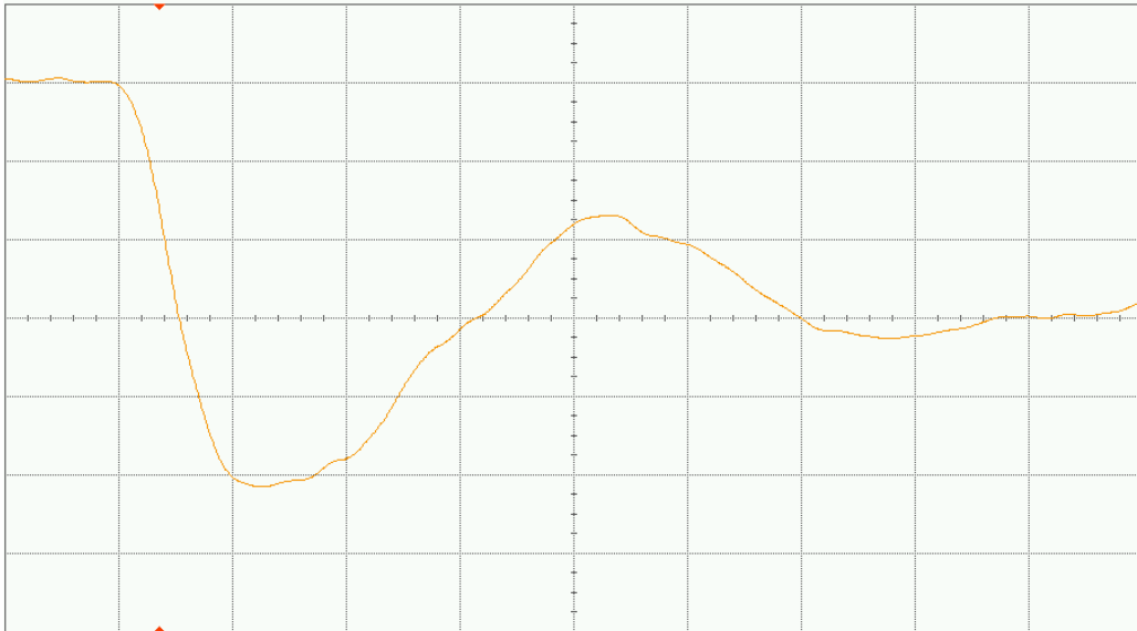
Figure 15(b) DUT 8514 post-annealing falling edge, abscissa scale is 1 V/div and ordinate scale is 2 ns/div.
