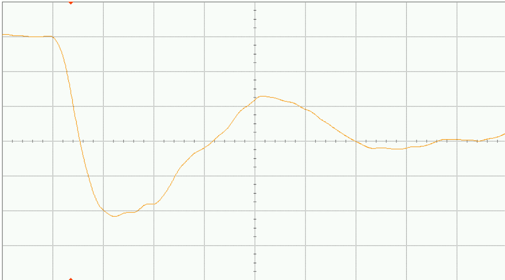
Figure 19(b) DUT 8547 pre-irradiation falling edge, abscissa scale is 1 V/div and ordinate scale is 2 ns/div.
