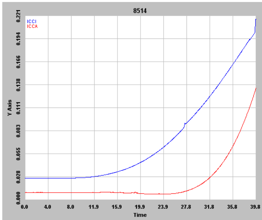
Figure 3 DUT 8514 in-flux I_{CCA} and I_{CCI} . The unit of time is in minutes.
