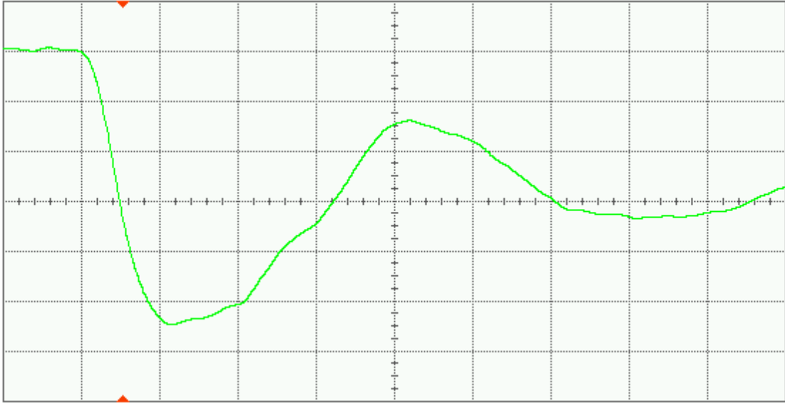
Figure 18(a) DUT 8536 pre-irradiation falling edge, abscissa scale is 1 V/div and ordinate scale is 2 ns/div.
