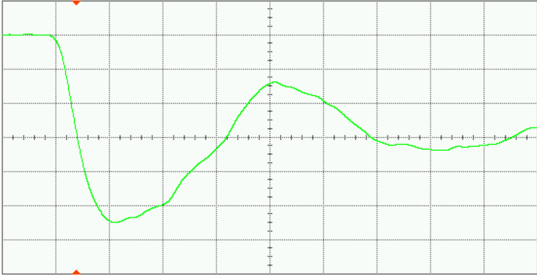
Figure 16(a) DUT 8516 pre-irradiation falling edge, abscissa scale is 1 V/div and ordinate scale is 2 ns/div.
