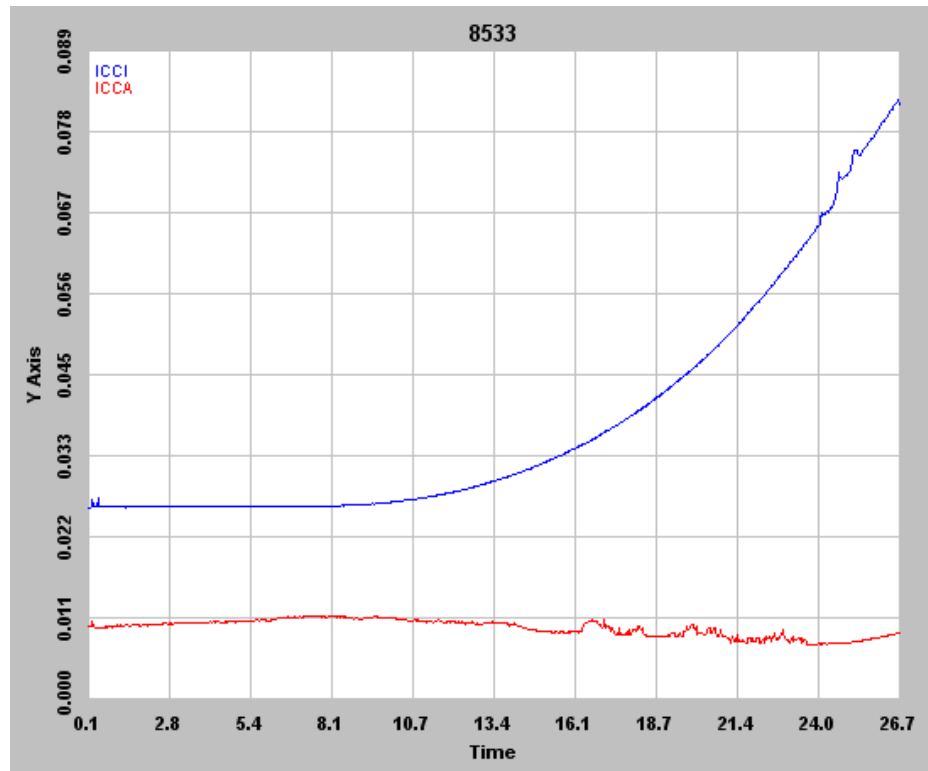
Figure 5 DUT 8533 in-flux I_{CCA} and I_{CCI} . The unit of time is in minutes.
