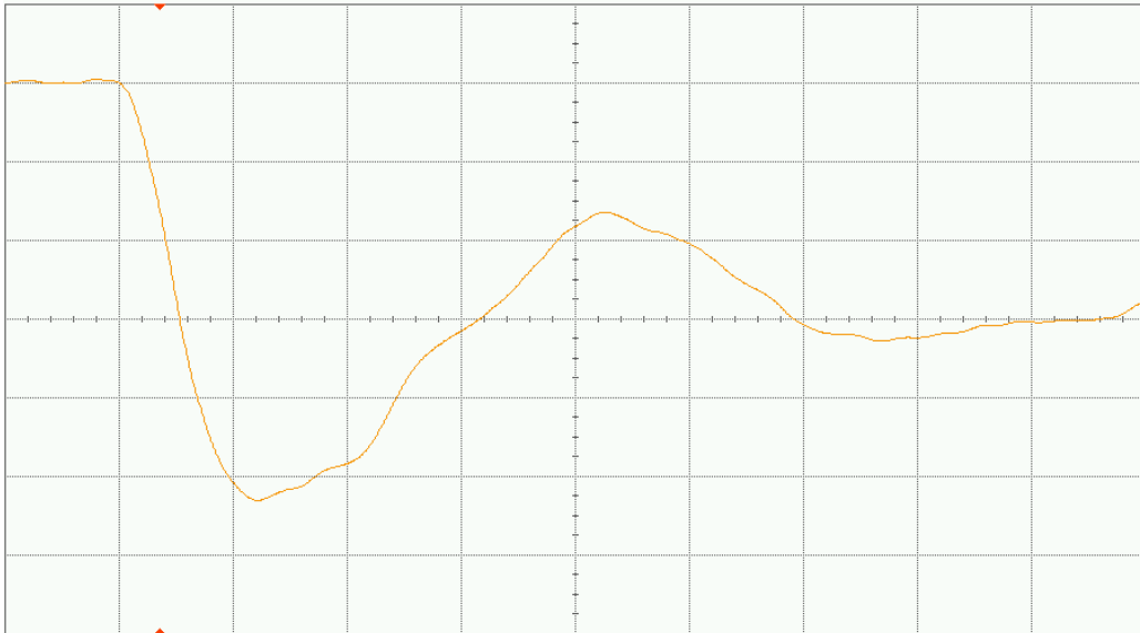
Figure 14(b) DUT 8510 post-annealing falling edge, abscissa scale is 1 V/div and ordinate scale is 2 ns/div.
