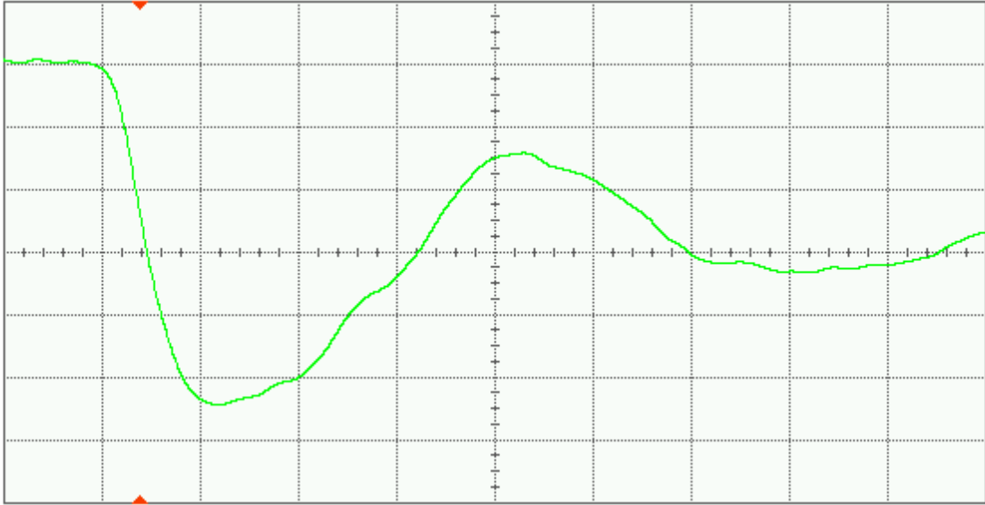
Figure 19(a) DUT 8547 pre-irradiation falling edge, abscissa scale is 1 V/div and ordinate scale is 2 ns/div.
