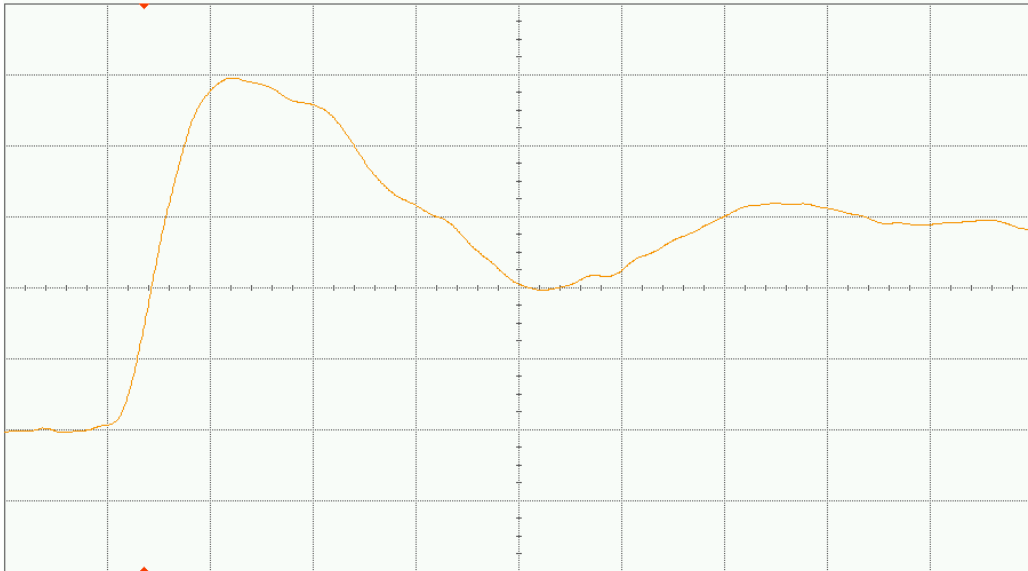
Figure 12(b) DUT 8536 post-annealing rising edge, abscissa scale is 1 V/div and ordinate scale is 2 ns/div.
