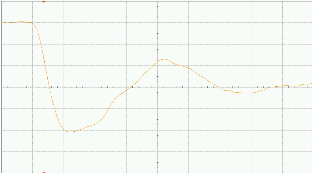
Figure 16(b) DUT 8516 post-annealing falling edge, abscissa scale is 1 V/div and ordinate scale is 2 ns/div.
