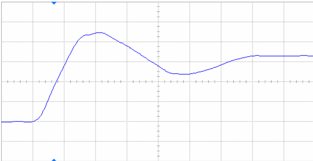
Figure 9(b) DUT 3284 post-annealing rising edge, abscissa scale is 1 V/div and ordinate scale is 2 ns/div.
