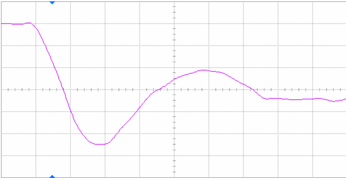
Figure 15(a) DUT 3284 pre-irradiation falling edge, abscissa scale is 1 V/div and ordinate scale is 2 ns/div.
