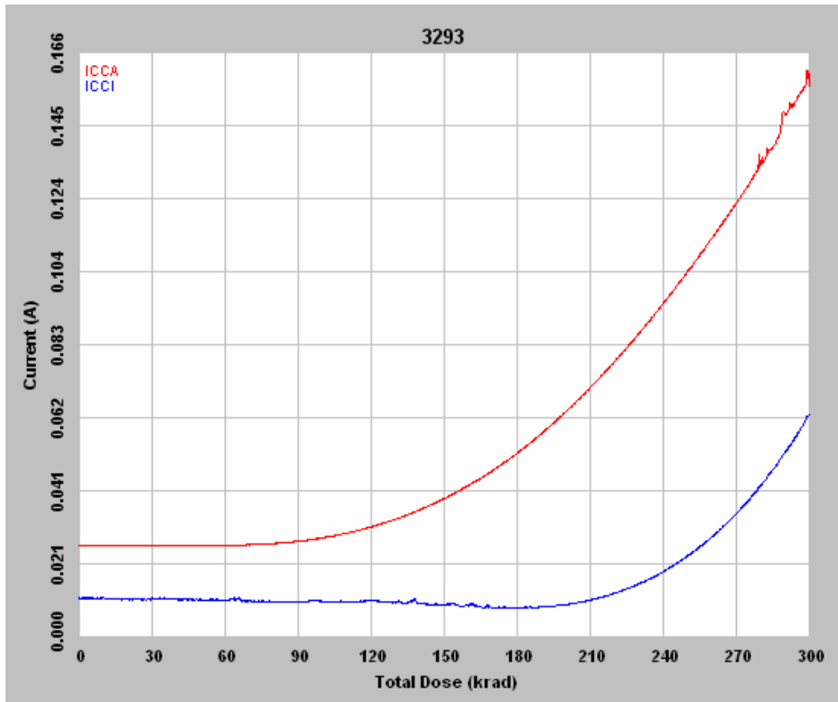
Figure 4 DUT 3293 in-flux I_{CCA} and I_{CCI}
