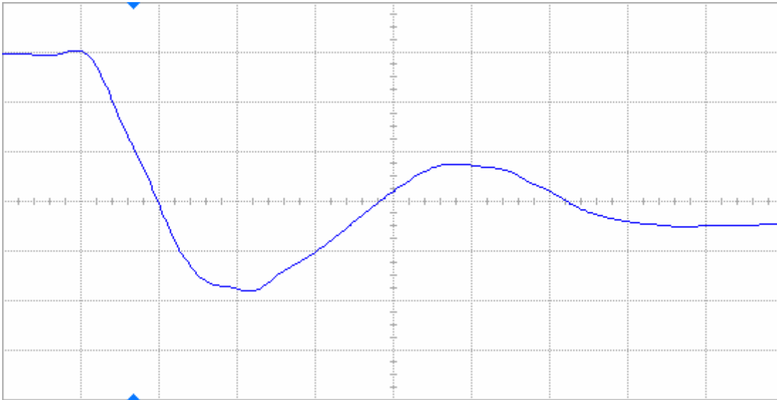
Figure 19(b) DUT 3323 post-annealing falling edge, abscissa scale is 1 V/div and ordinate scale is 2 ns/div.
