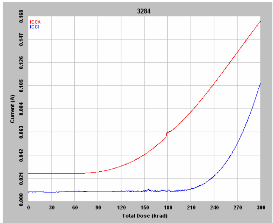
Figure 3 DUT 3284 in-flux I_{CCA} and I_{CCI}
