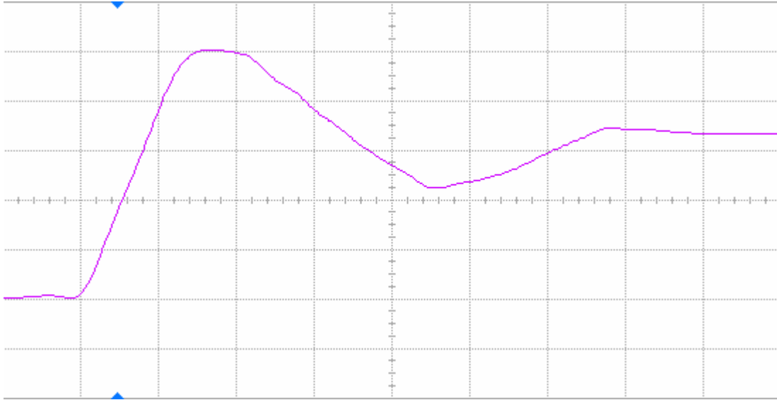
Figure 10(a) DUT 3293 pre-radiation rising edge, abscissa scale is 1 V/div and ordinate scale is 2 ns/div.
