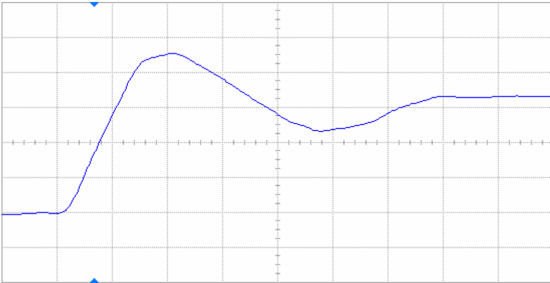
Figure 10(b) DUT 3293 post-annealing rising edge, abscissa scale is 1 V/div and ordinate scale is 2 ns/div.
