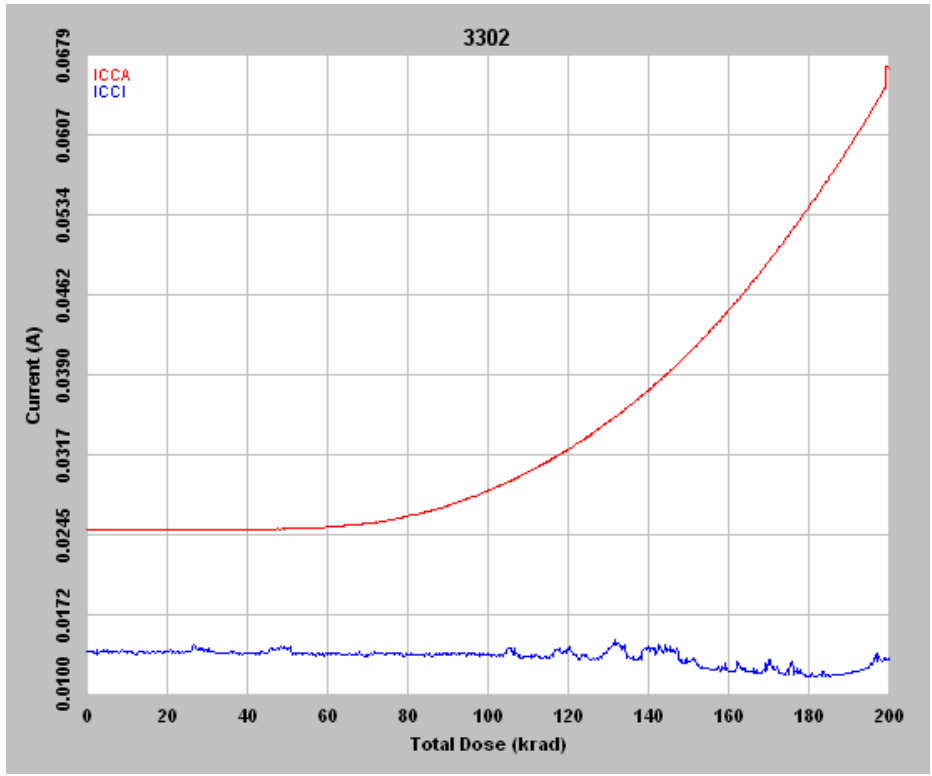
Figure 6 DUT 3302 in-flux I_{CCA} and I_{CCI}
