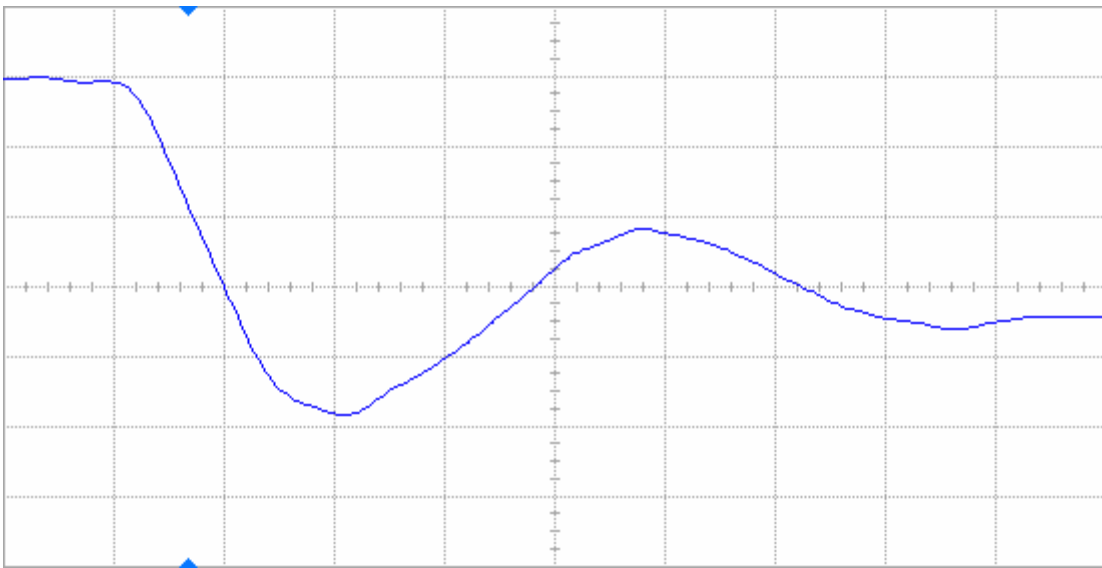
Figure 15(b) DUT 3284 post-annealing falling edge, abscissa scale is 1 V/div and ordinate scale is 2 ns/div.
