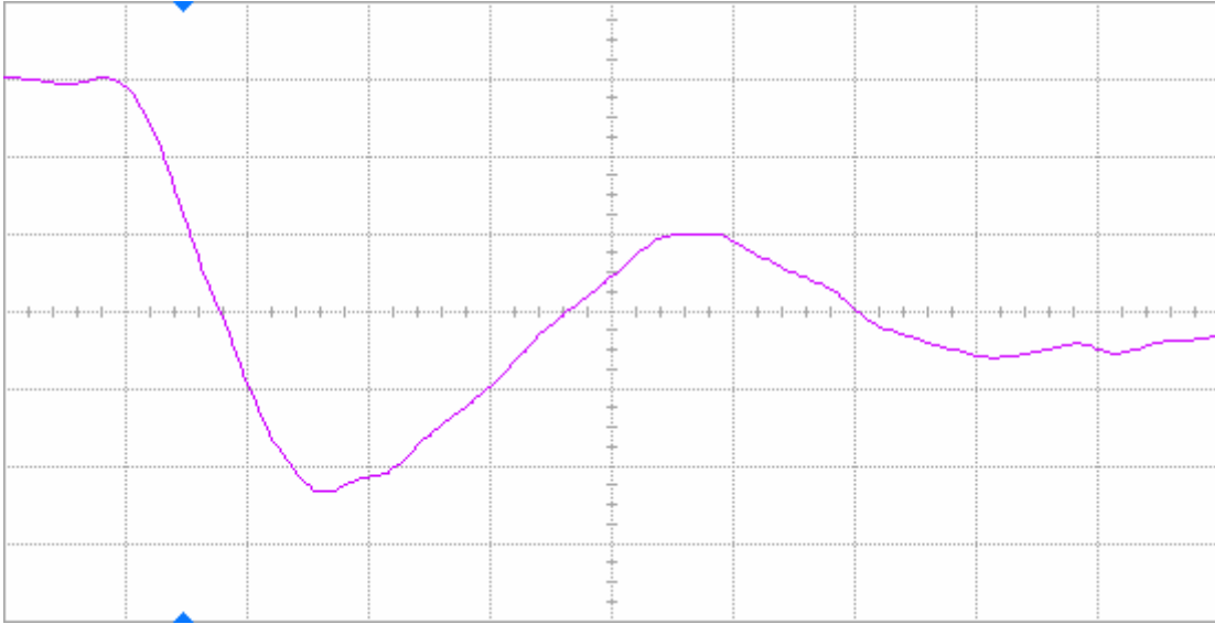
Figure 18(a) DUT 3302 pre-irradiation falling edge, abscissa scale is 1 V/div and ordinate scale is 2 ns/div.
