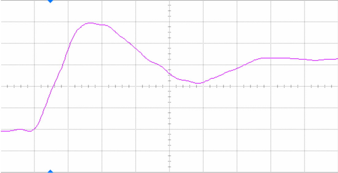
Figure 11(a) DUT 3301 pre-irradiation rising edge, abscissa scale is 1 V/div and ordinate scale is 2 ns/div.
