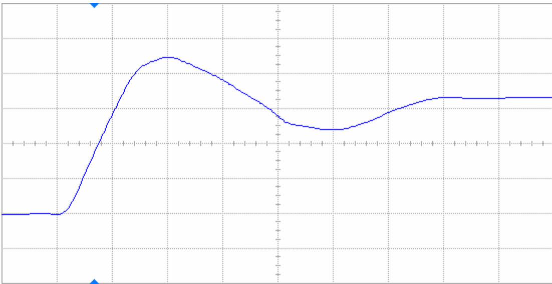
Figure 13(b) DUT 3323 post-annealing rising edge, abscissa scale is 1 V/div and ordinate scale is 2 ns/div.
