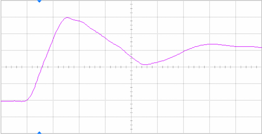
Figure 12(a) DUT 3302 pre-irradiation rising edge, abscissa scale is 1 V/div and ordinate scale is 2 ns/div.
