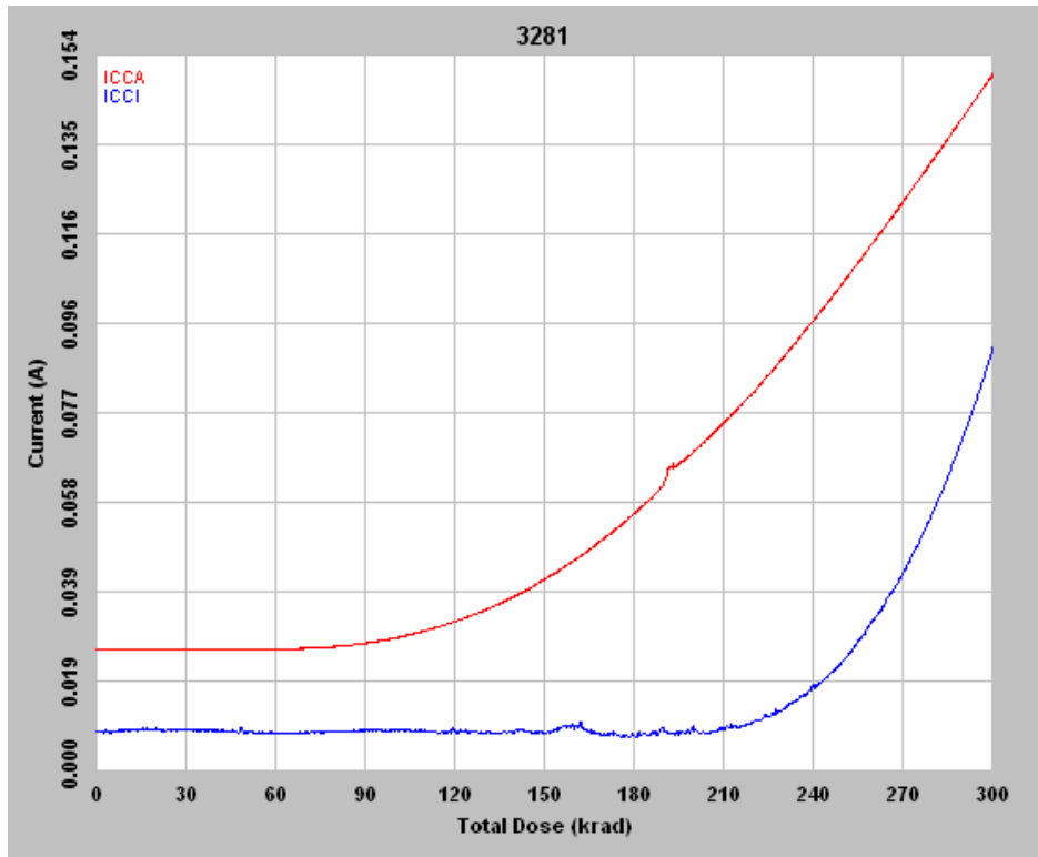
Figure 2 DUT 3281 in-flux I_{CCA} and I_{CCI}
