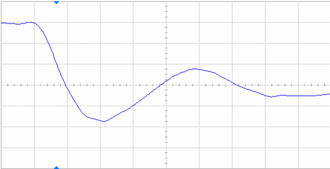
Figure 18(b) DUT 3302 post-annealing falling edge, abscissa scale is 1 V/div and ordinate scale is 2 ns/div.
