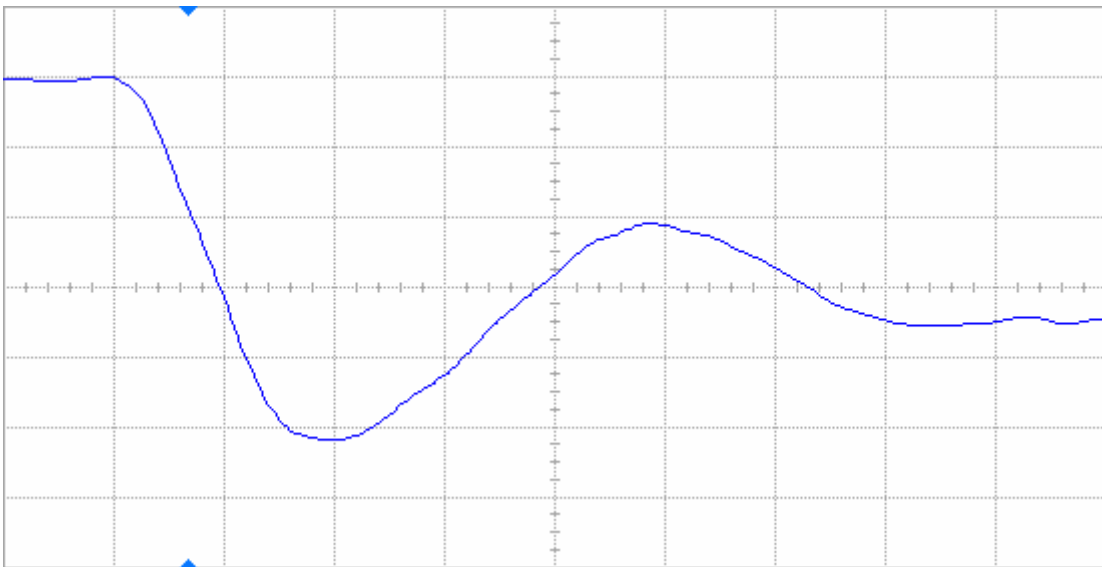
Figure 14(b) DUT 3281 post-annealing falling edge, abscissa scale is 1 V/div and ordinate scale is 2 ns/div.
