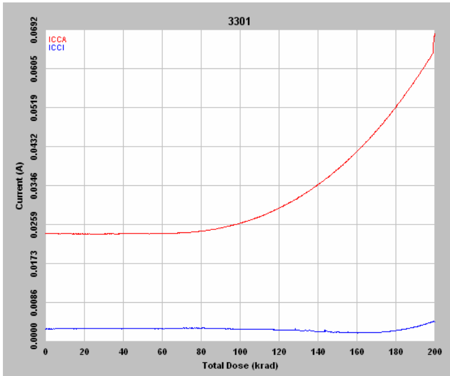
Figure 5 DUT 3301 in-flux I_{CCA} and I_{CCI}
