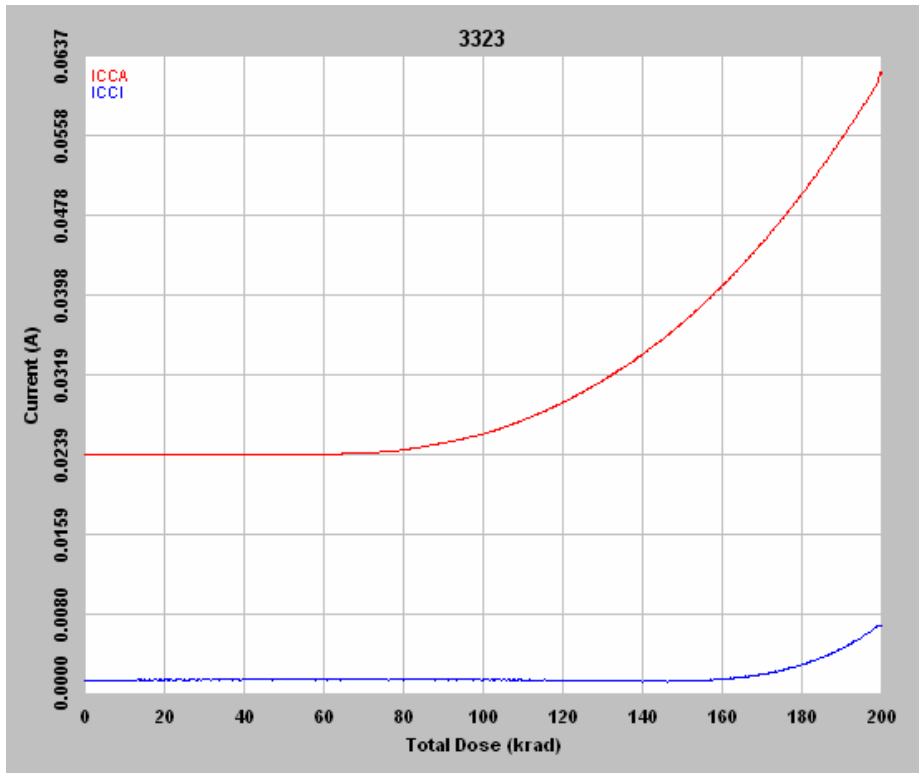
Figure 7 DUT 3323 in-flux I_{CCA} and I_{CCI}
