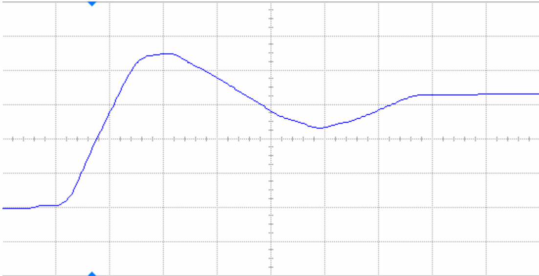
Figure 11(b) DUT 3301 post-annealing rising edge, abscissa scale is 1 V/div and ordinate scale is 2 ns/div.
