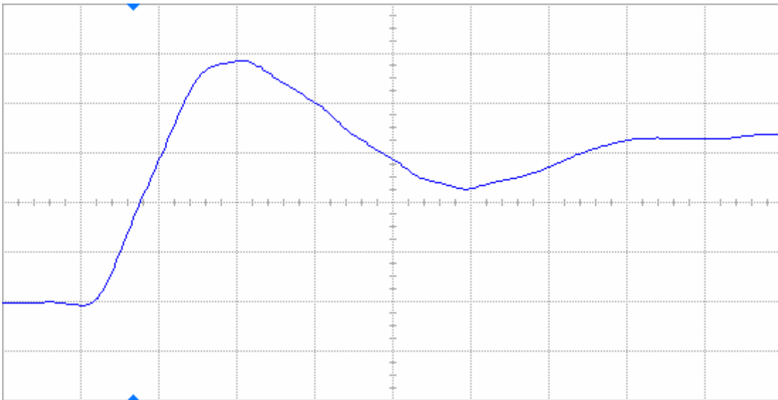
Figure 8(b) DUT 3281 post-annealing rising edge, abscissa scale is 1 V/div and ordinate scale is 2 ns/div.
