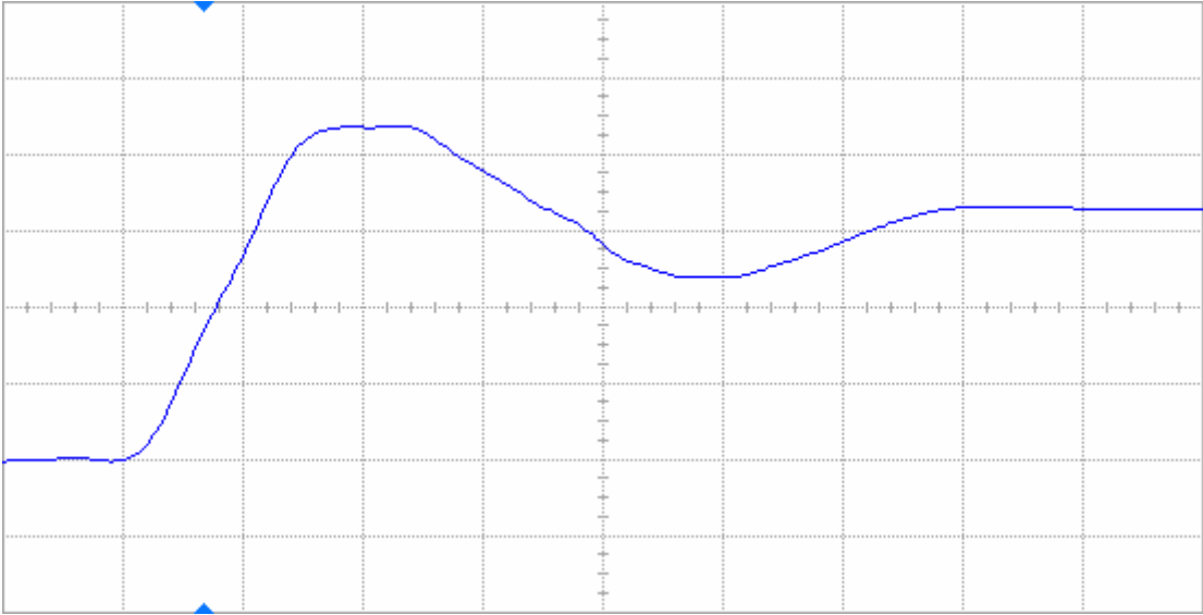
Figure 12(b) DUT 3302 post-annealing rising edge, abscissa scale is 1 V/div and ordinate scale is 2 ns/div.
