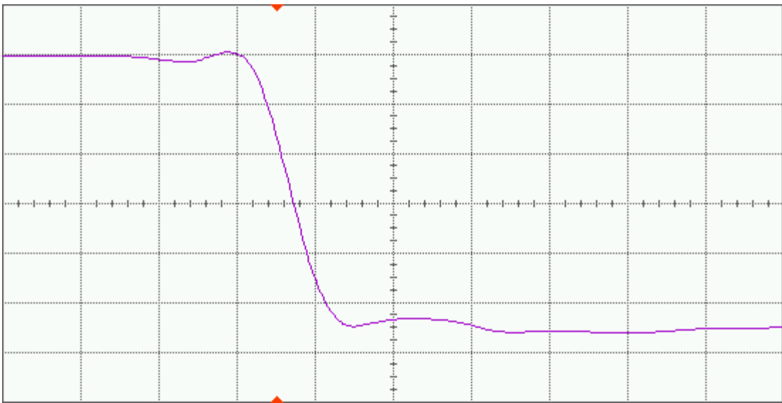
Figure 17(b) DUT 7406 post-annealing falling edge, abscissa scale is 1 V/div and ordinate scale is 1 ns/div.
