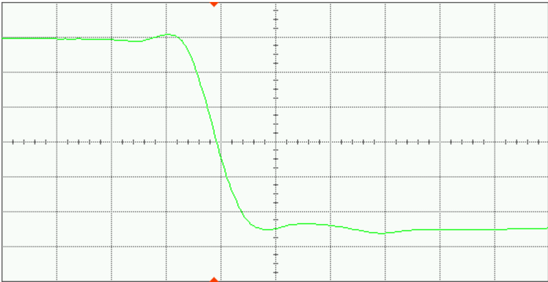
Figure 16(a) DUT 7402 pre-irradiation falling edge, abscissa scale is 1 V/div and ordinate scale is 1 ns/div.
