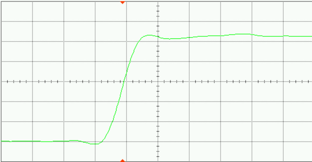
Figure 13(a) DUT 7429 pre-irradiation rising edge, abscissa scale is 1 V/div and ordinate scale is 1 ns/div.
