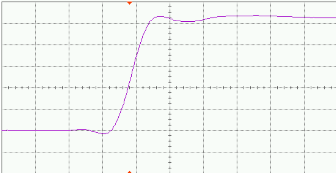
Figure 8(b) DUT 7388 post-annealing rising edge, abscissa scale is 1 V/div and ordinate scale is 1 ns/div.
