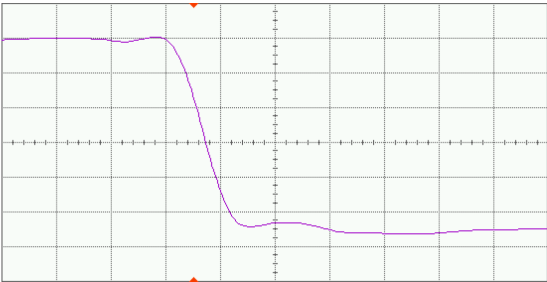
Figure 16(b) DUT 7402 post-annealing falling edge, abscissa scale is 1 V/div and ordinate scale is 1 ns/div.
