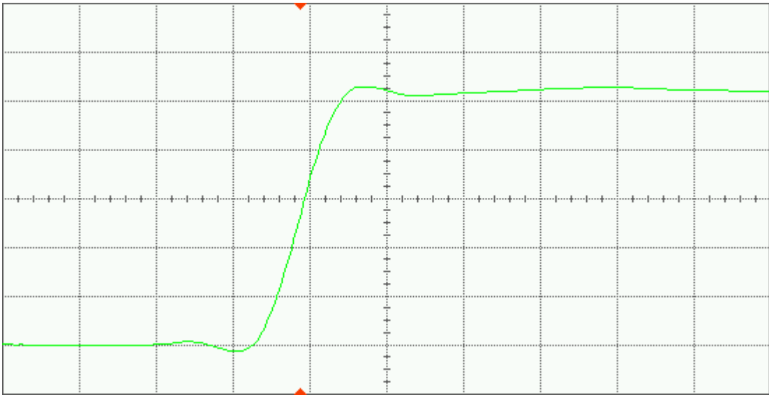
Figure 12(a) DUT 7407 pre-irradiation rising edge, abscissa scale is 1 V/div and ordinate scale is 1 ns/div.
