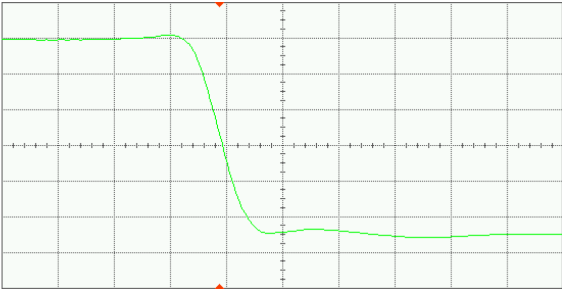
Figure 17(a) DUT 7406 pre-irradiation falling edge, abscissa scale is 1 V/div and ordinate scale is 1 ns/div.
