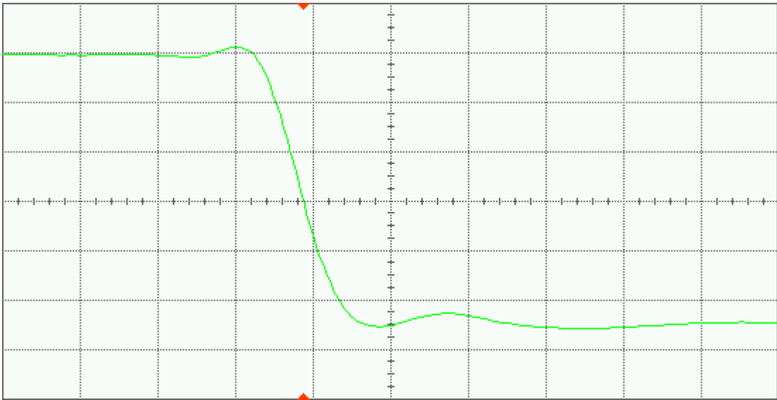
Figure 15(a) DUT 7389 pre-irradiation falling edge, abscissa scale is 1 V/div and ordinate scale is 1 ns/div.
