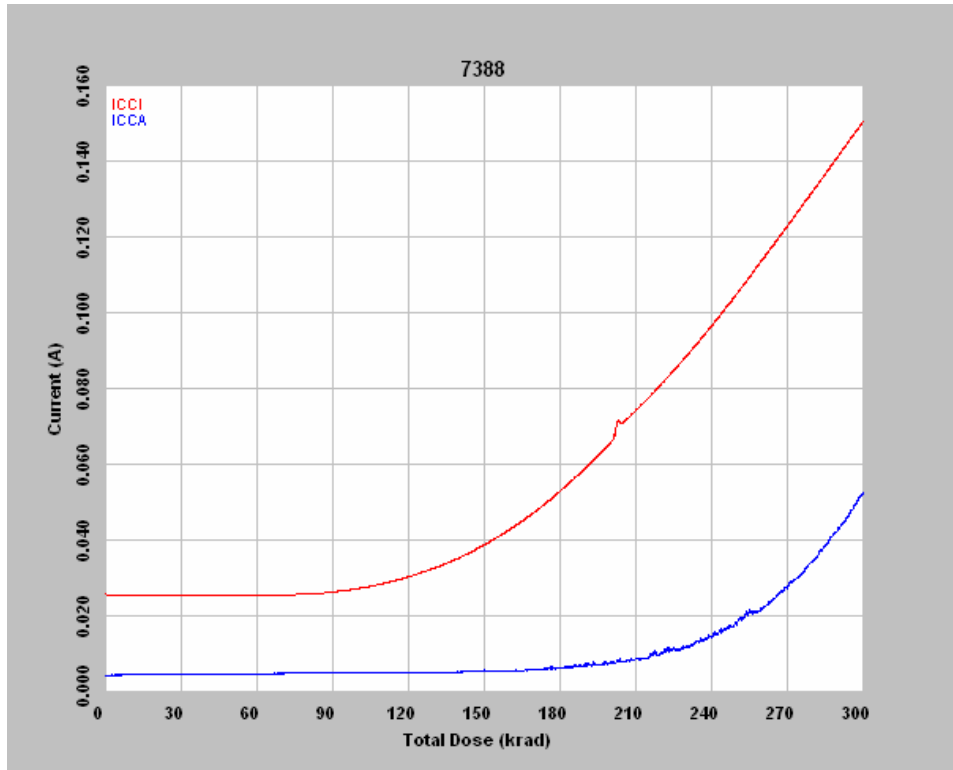
Figure 2 DUT 7388 in-flux I_{CCA} and I_{CCI}
