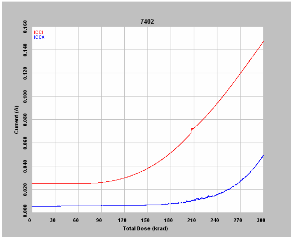
Figure 4 DUT 7402 in-flux I_{CCA} and I_{CCI}
