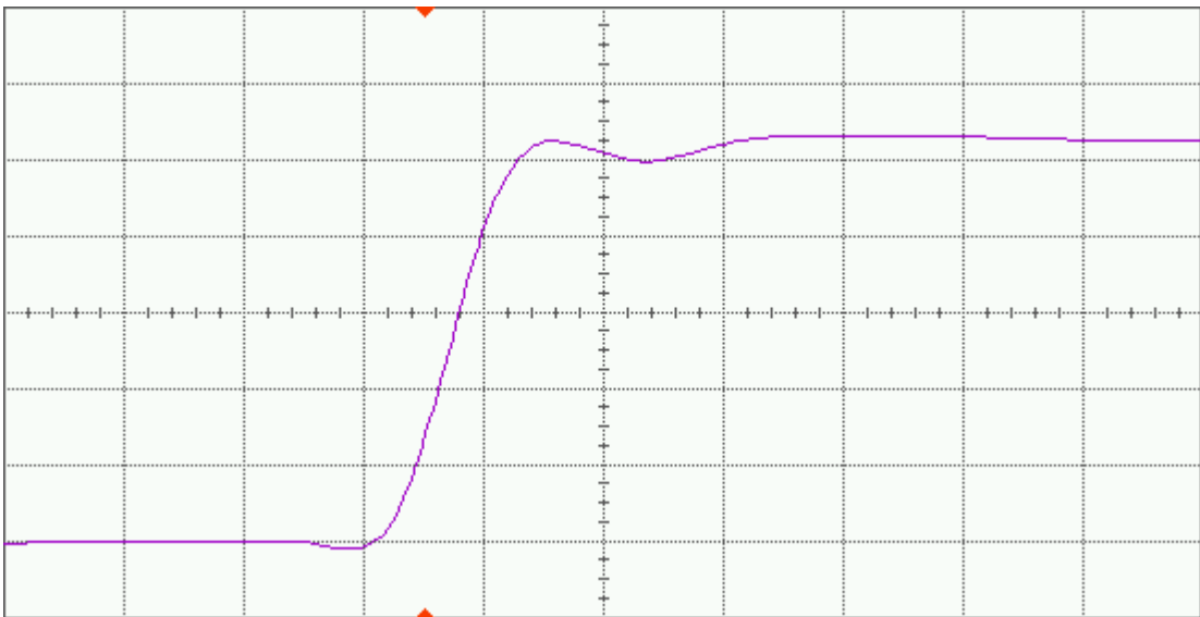
Figure 12(b) DUT 7407 post-annealing rising edge, abscissa scale is 1 V/div and ordinate scale is 1 ns/div.
