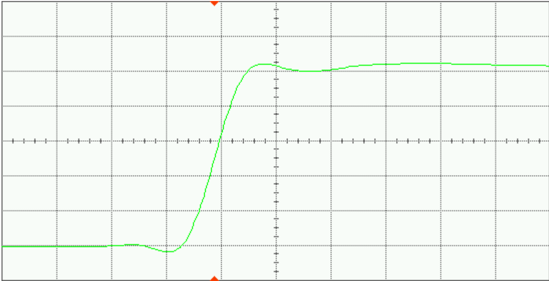
Figure 8(a) DUT 7388 pre-irradiation rising edge, abscissa scale is 1 V/div and ordinate scale is 1 ns/div.
