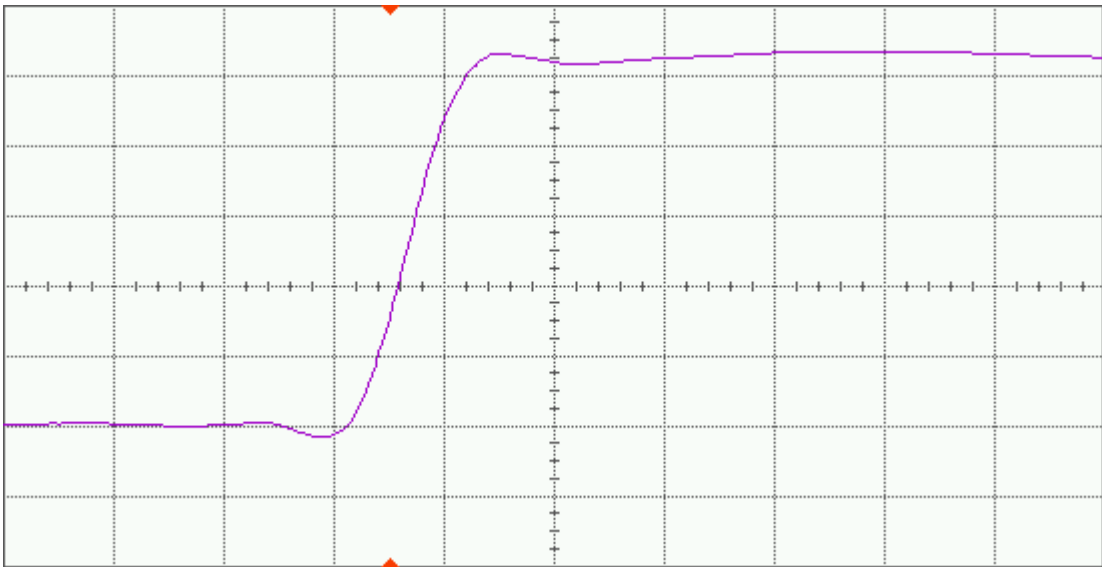
Figure 9(b) DUT 7389 post-annealing rising edge, abscissa scale is 1 V/div and ordinate scale is 1 ns/div.
