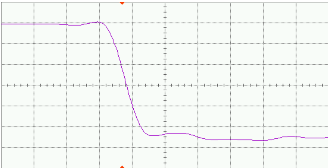
Figure 14(b) DUT 7388 post-annealing falling edge, abscissa scale is 1 V/div and ordinate scale is 1 ns/div.
