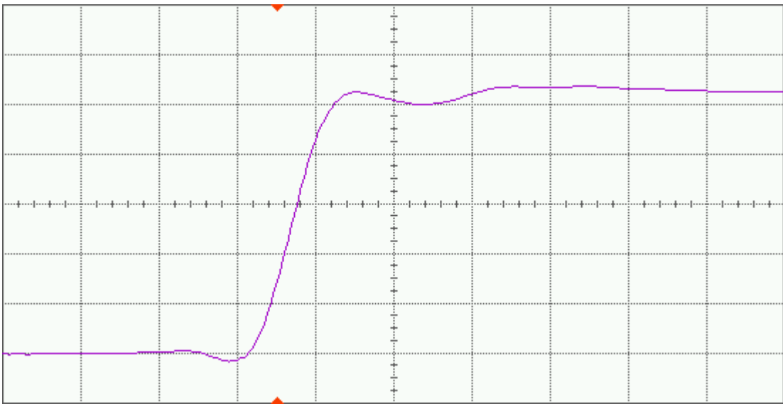
Figure 11(b) DUT 7406 post-annealing rising edge, abscissa scale is 1 V/div and ordinate scale is 1 ns/div.
