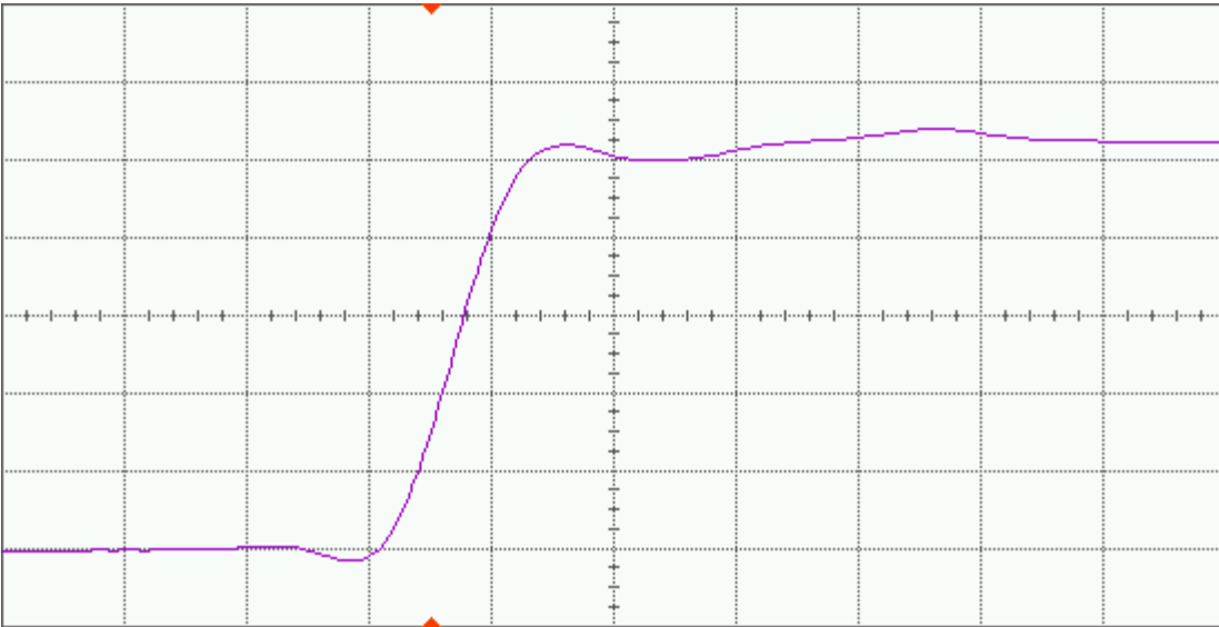
Figure 13(b) DUT 7429 post-annealing rising edge, abscissa scale is 1 V/div and ordinate scale is 1 ns/div.
