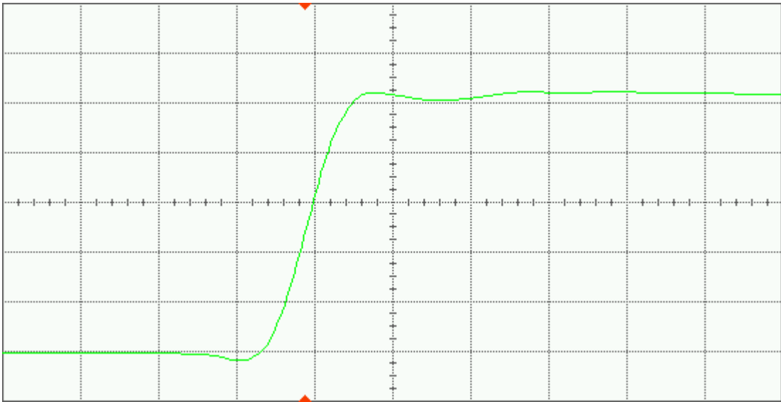
Figure 10(a) DUT 7402 pre-radiation rising edge, abscissa scale is 1 V/div and ordinate scale is 1 ns/div.
