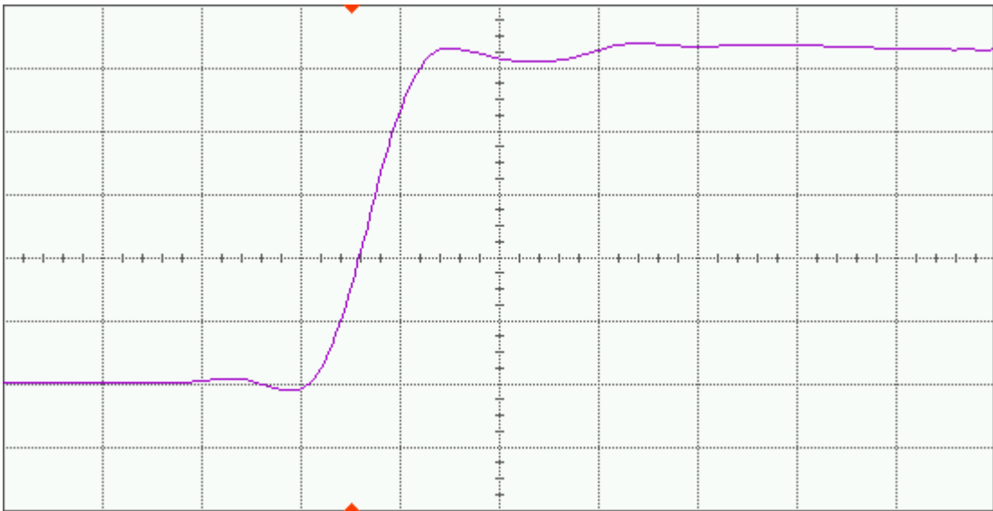
Figure 10(b) DUT 7402 post-annealing rising edge, abscissa scale is 1 V/div and ordinate scale is 1 ns/div.
