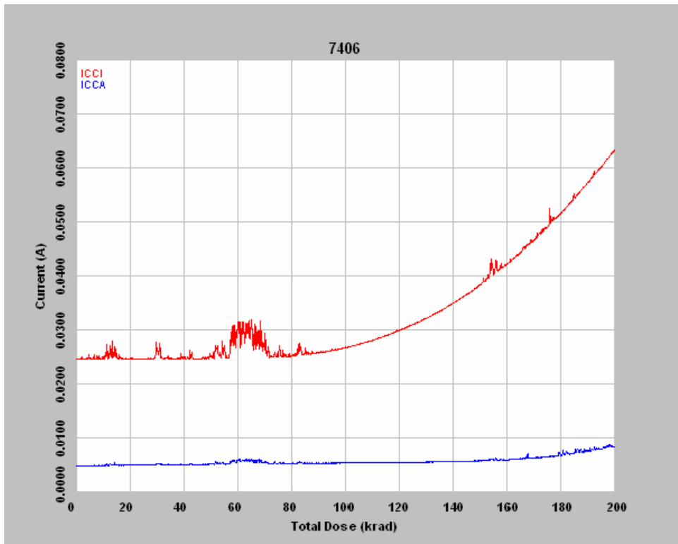
Figure 5 DUT 7406 in-flux I_{CCA} and I_{CCI}
