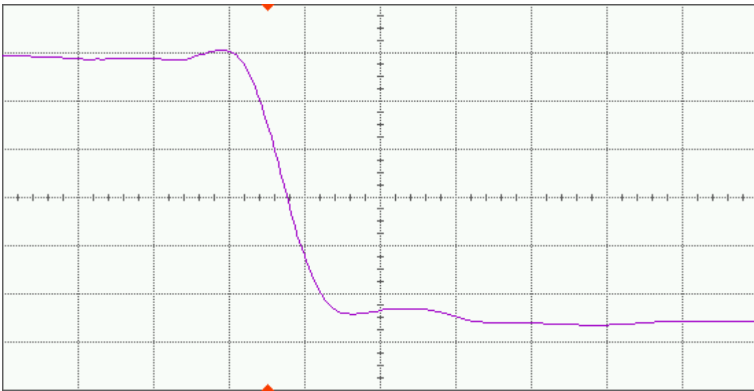
Figure 19(b) DUT 7429 post-annealing falling edge, abscissa scale is 1 V/div and ordinate scale is 1 ns/div.
