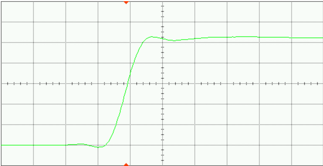
Figure 11(a) DUT 7406 pre-irradiation rising edge, abscissa scale is 1 V/div and ordinate scale is 1 ns/div.
