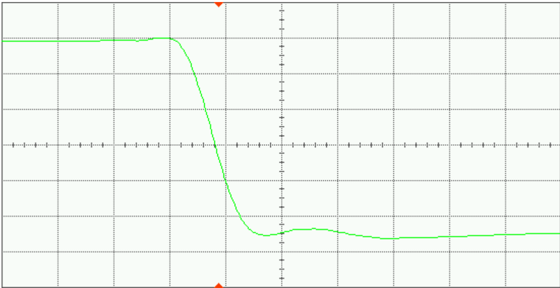
Figure 18(a) DUT 7407 pre-irradiation falling edge, abscissa scale is 1 V/div and ordinate scale is 1 ns/div.
