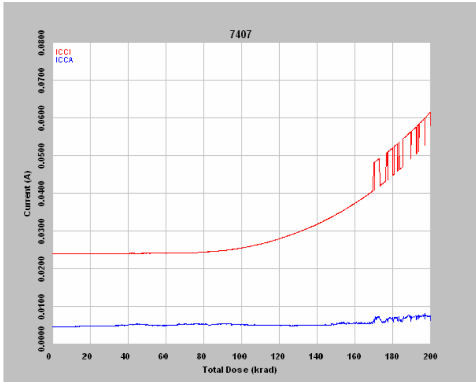
Figure 6 DUT 7407 in-flux I_{CCA} and I_{CCI}
