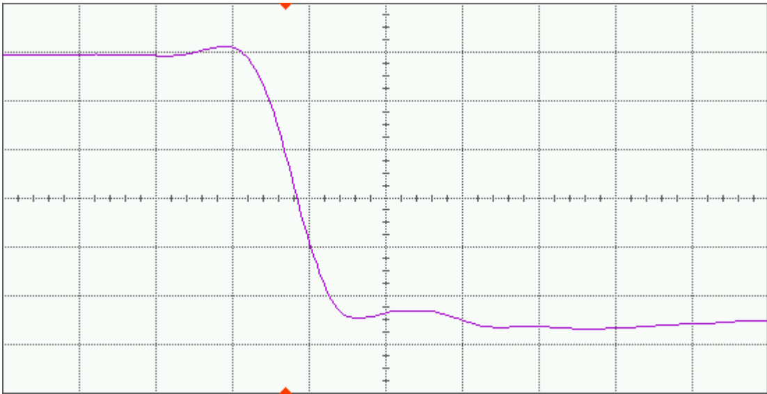
Figure 15(b) DUT 7389 post-annealing falling edge, abscissa scale is 1 V/div and ordinate scale is 1 ns/div.
