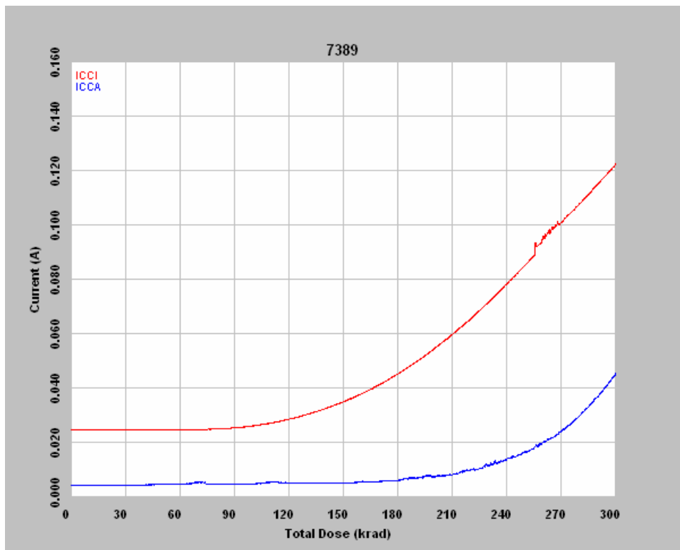
Figure 3 DUT 7389 in-flux I_{CCA} and I_{CCI}
