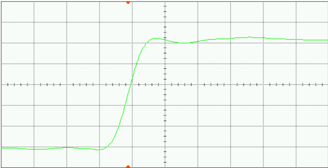
Figure 9(a) DUT 7389 pre-irradiation rising edge, abscissa scale is 1 V/div and ordinate scale is 1 ns/div.
