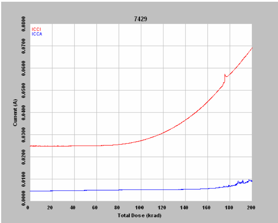
Figure 7 DUT 7429 in-flux I_{CCA} and I_{CCI}
