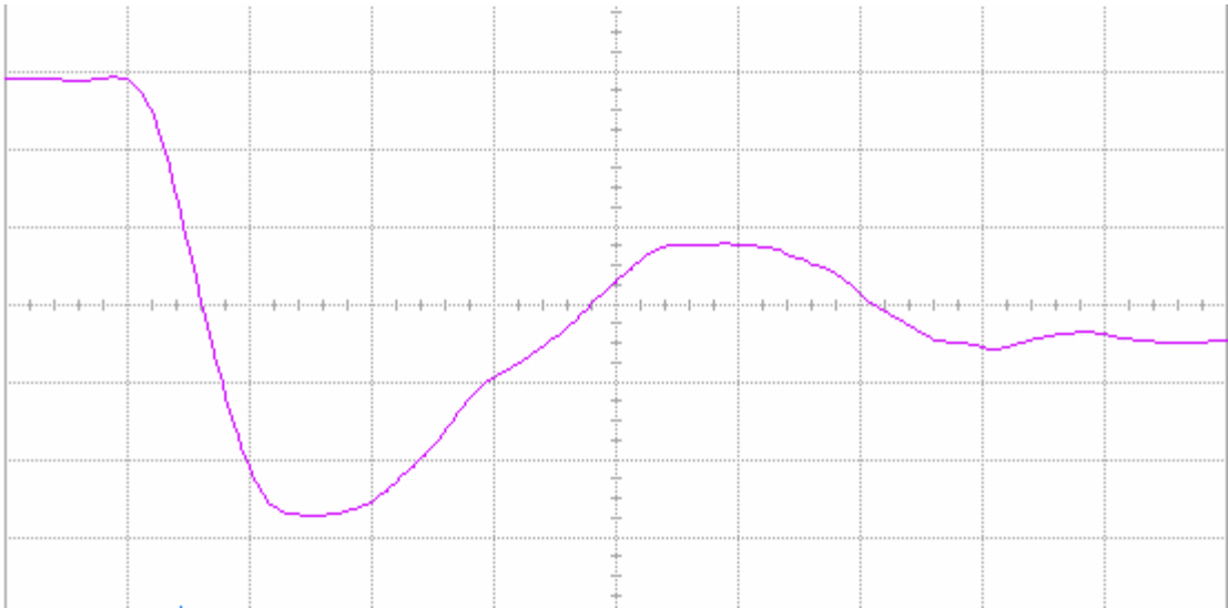
Figure 15(b) DUT 3662 post-annealing falling edge, abscissa scale is 1 V/div and ordinate scale is 2 ns/div.
