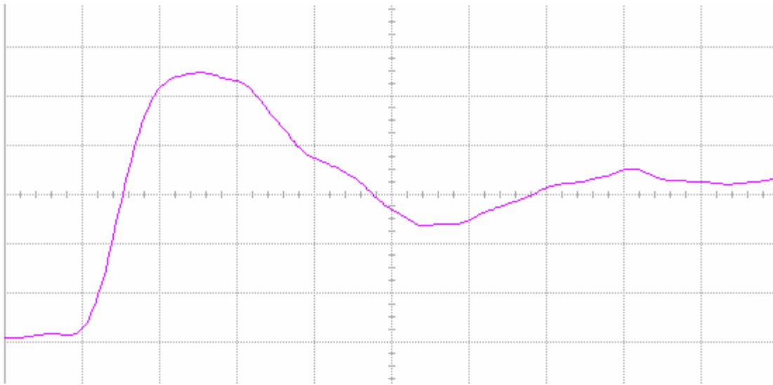
Figure 11(b) DUT 3676 post-annealing rising edge, abscissa scale is 1 V/div and ordinate scale is 2 ns/div.
