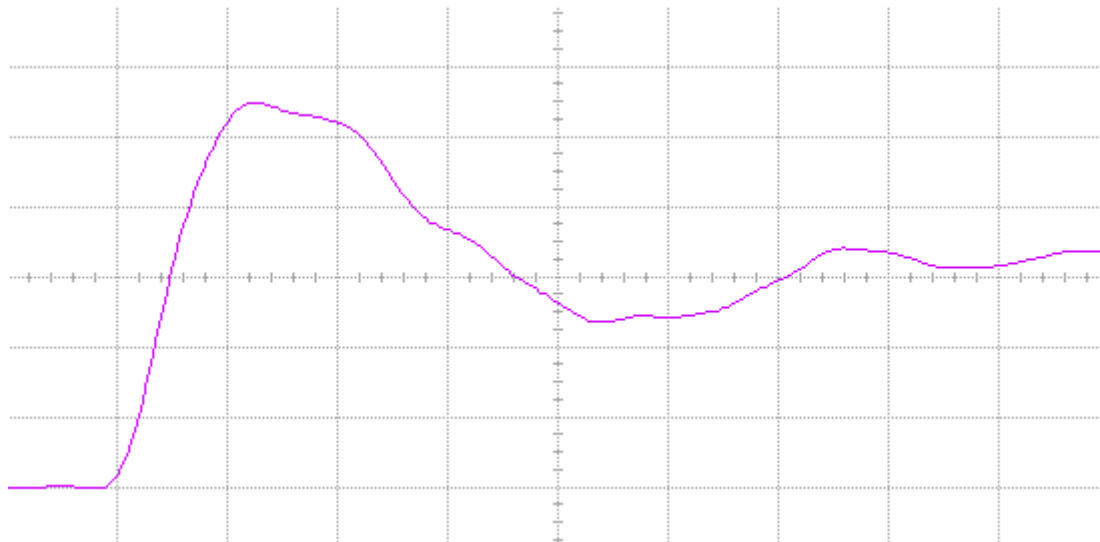
Figure 8(b) DUT 3643 post-annealing rising edge, abscissa scale is 1 V/div and ordinate scale is 2 ns/div.
