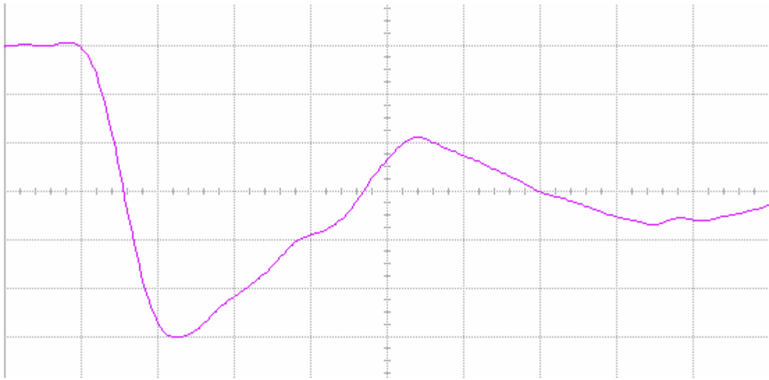
Figure 17(a) DUT 3676 pre-irradiation falling edge, abscissa scale is 1 V/div and ordinate scale is 2 ns/div.
