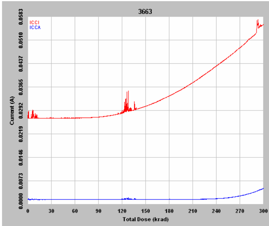
Figure 4 DUT 3663 in-flux I_{CCA} and I_{CCI}
