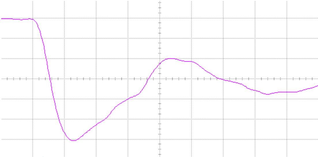
Figure 19(a) DUT 3738 pre-irradiation falling edge, abscissa scale is 1 V/div and ordinate scale is 2 ns/div.
