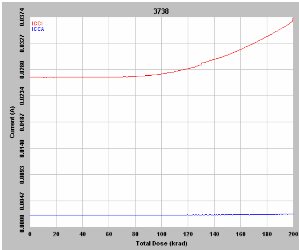
Figure 7 DUT 3738 in-flux I_{CCA} and I_{CCI}
