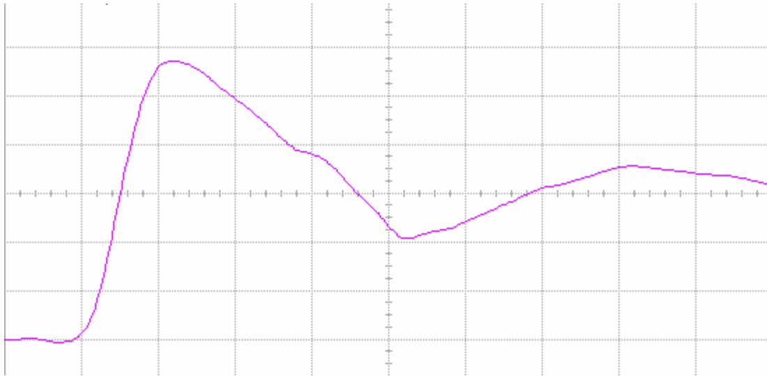
Figure 8(a) DUT 3643 pre-irradiation rising edge, abscissa scale is 1 V/div and ordinate scale is 2 ns/div.
