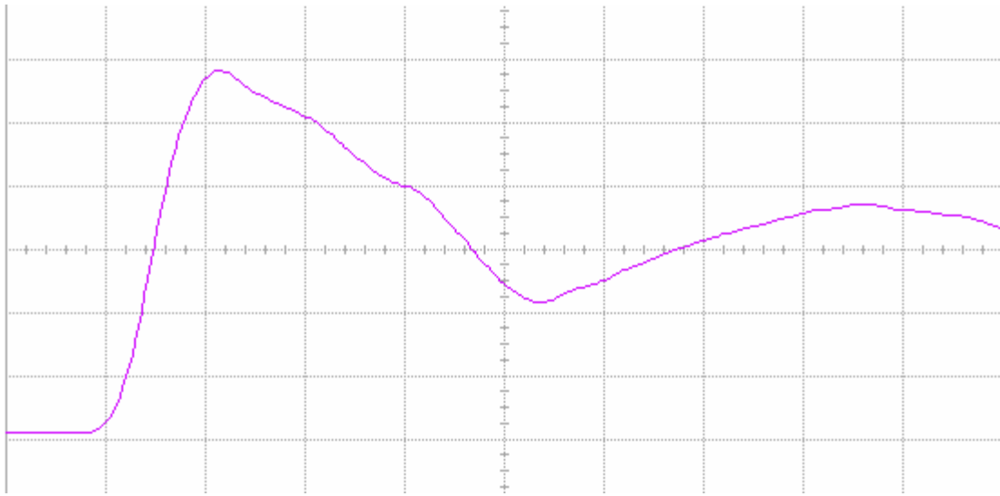
Figure 13(a) DUT 3738 pre-irradiation rising edge, abscissa scale is 1 V/div and ordinate scale is 2 ns/div.
