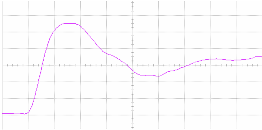
Figure 13(b) DUT 3738 post-annealing rising edge, abscissa scale is 1 V/div and ordinate scale is 2 ns/div.
