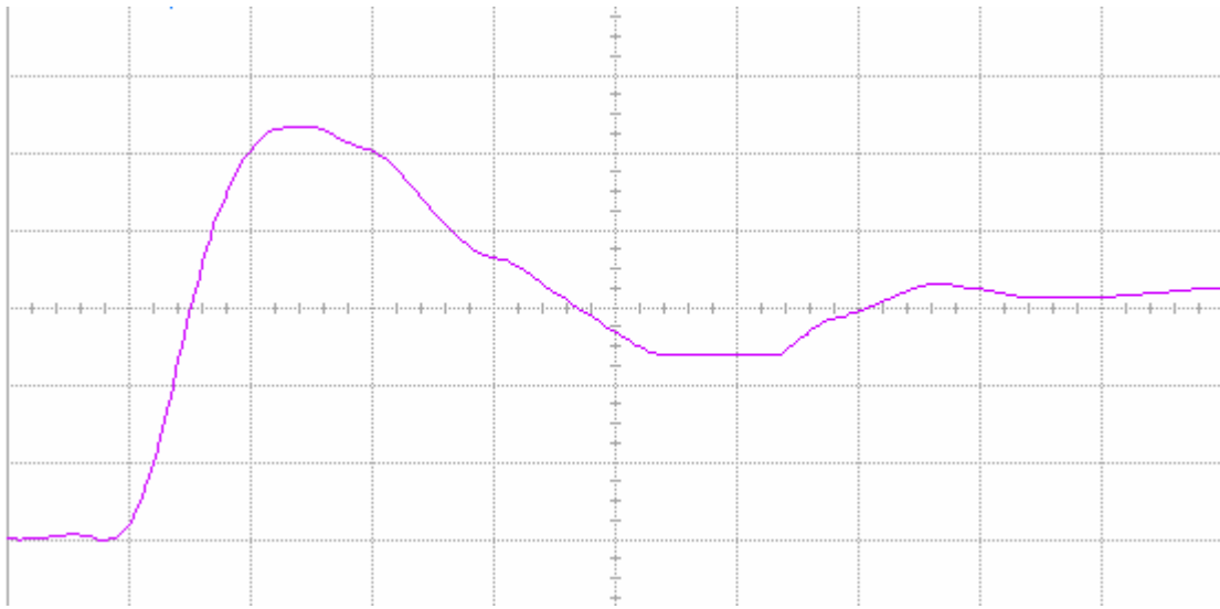
Figure 9(b) DUT 3662 post-annealing rising edge, abscissa scale is 1 V/div and ordinate scale is 2 ns/div.
