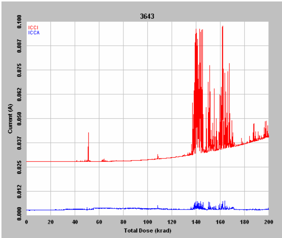
Figure 2 DUT 3643 in-flux I_{CCA} and I_{CCI} . The spikes are due to bad contacts.
