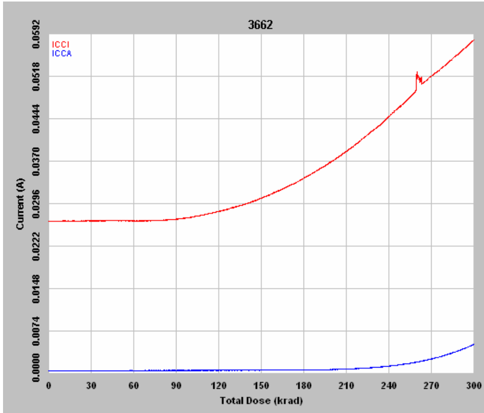
Figure 3 DUT3662 in-flux I_{CCA} and I_{CCI}
