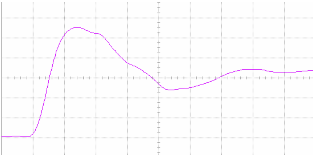
Figure 10(b) DUT 3663 post-annealing rising edge, abscissa scale is 1 V/div and ordinate scale is 2 ns/div.
