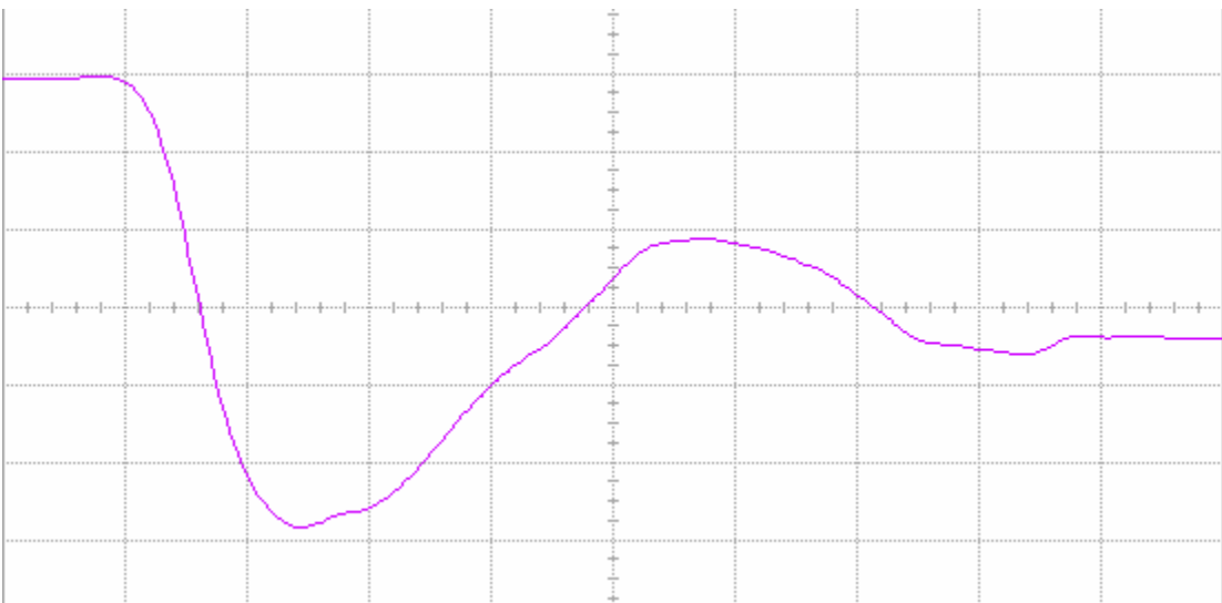
Figure 16(b) DUT 3663 post-annealing falling edge, abscissa scale is 1 V/div and ordinate scale is 2 ns/div.
