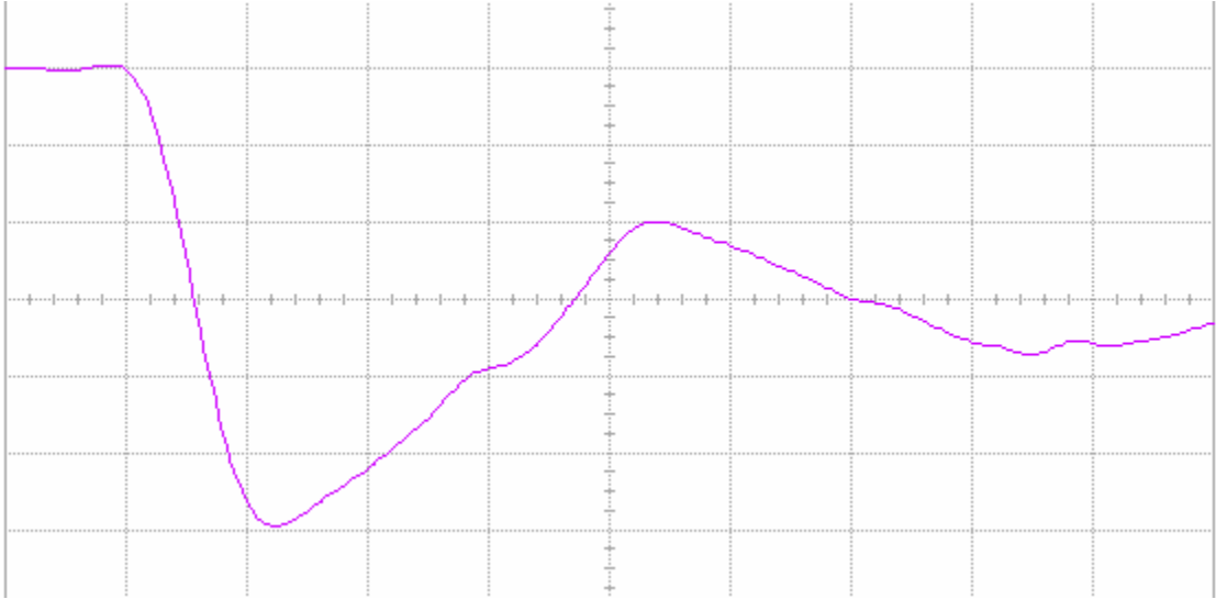
Figure 15(a) DUT 3662 pre-irradiation falling edge, abscissa scale is 1 V/div and ordinate scale is 2 ns/div.
