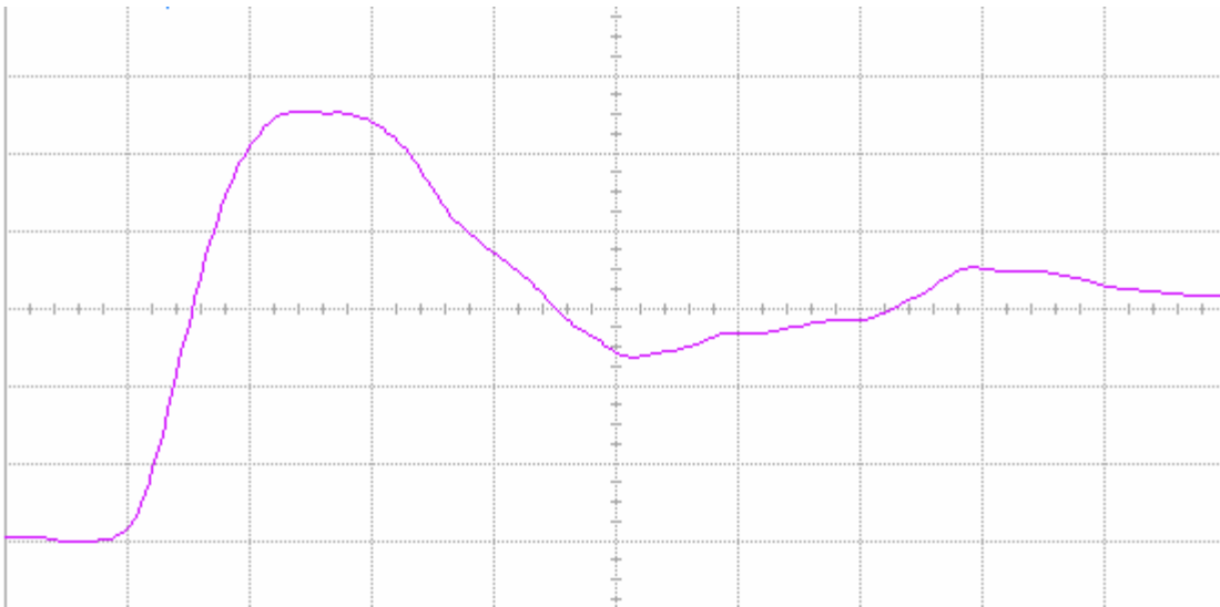
Figure 12(b) DUT 3695 post-annealing rising edge, abscissa scale is 1 V/div and ordinate scale is 2 ns/div.
