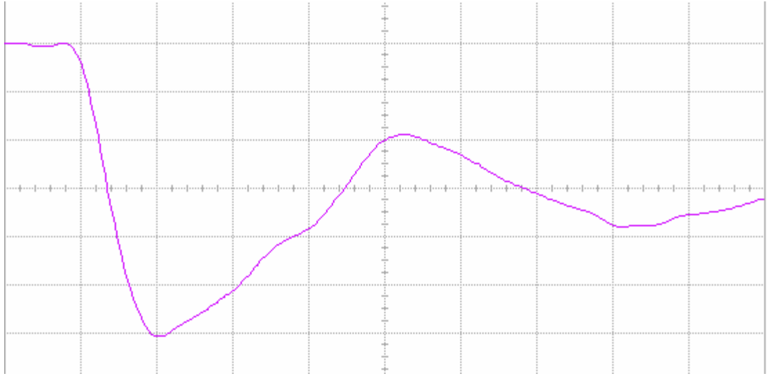
Figure 18(a) DUT 3695 post-annealing falling edge, abscissa scale is 1 V/div and ordinate scale is 2 ns/div.
