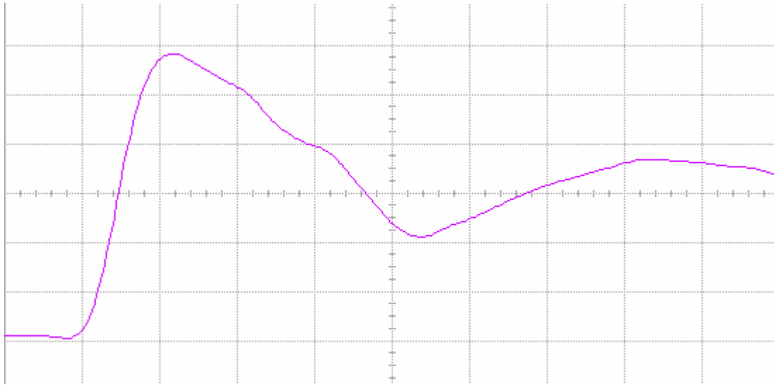
Figure 12(a) DUT 3695 pre-irradiation rising edge, abscissa scale is 1 V/div and ordinate scale is 2 ns/div.
