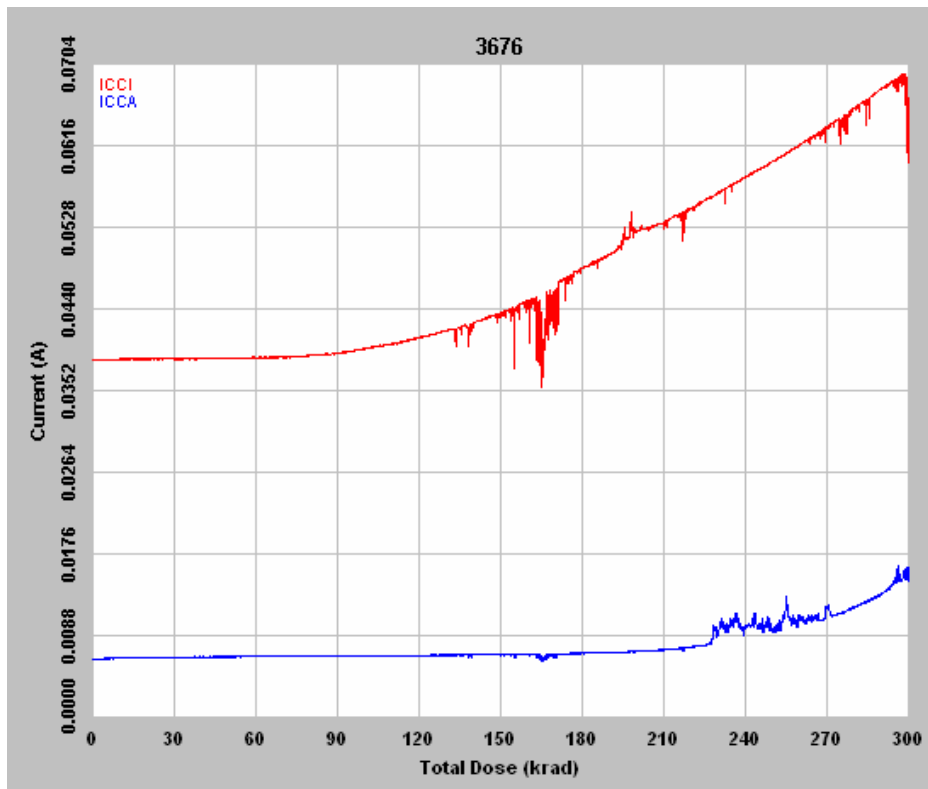
Figure 5 DUT 3676 in-flux I_{CCA} and I_{CCI}
