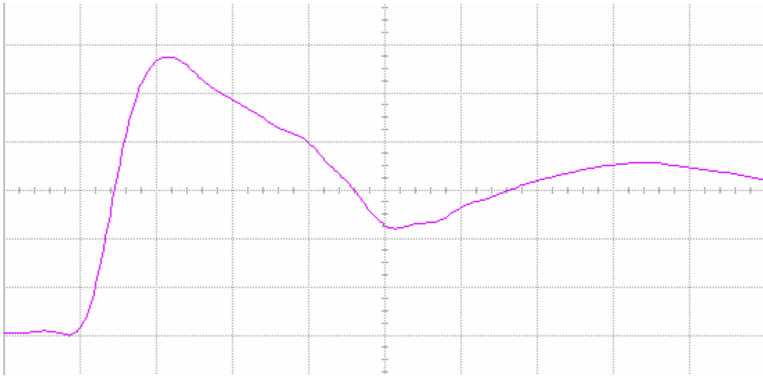
Figure 10(a) DUT 3663 pre-radiation rising edge, abscissa scale is 1 V/div and ordinate scale is 2 ns/div.
