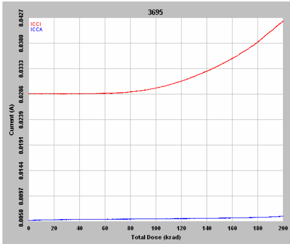
Figure 6 DUT 3695 in-flux I_{CCA} and I_{CCI}
