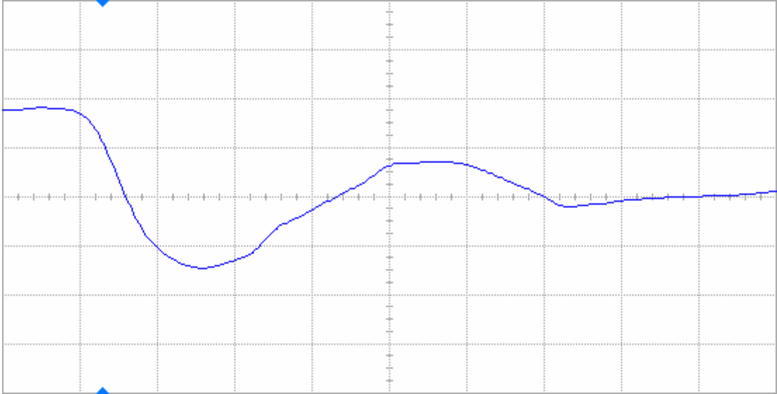
Figure 13(a) DUT 466 pre-irradiation falling edge, abscissa scale is 2 V/div and ordinate scale is 2 ns/div.
