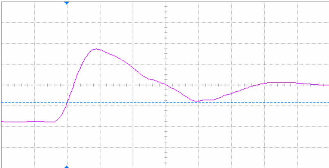
Figure 7(b) DUT 465 post-annealing rising edge, abscissa scale is 2 V/div and ordinate scale is 2 ns/div.
