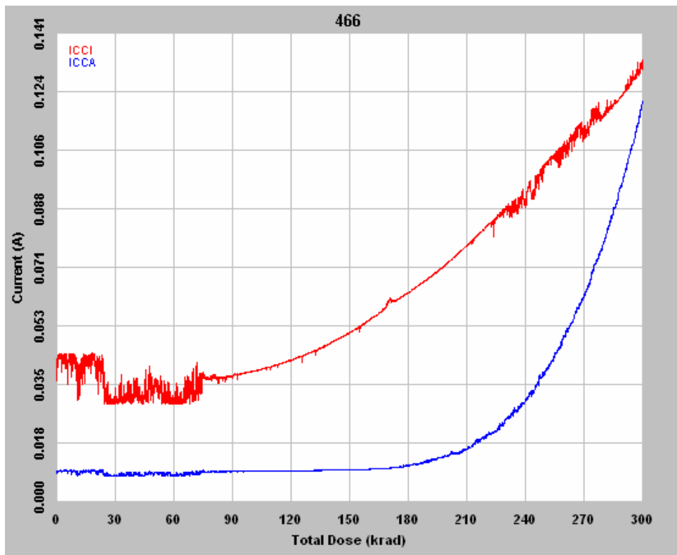
Figure 3 DUT 3175 in-flux I_{CCA} and I_{CCI}
