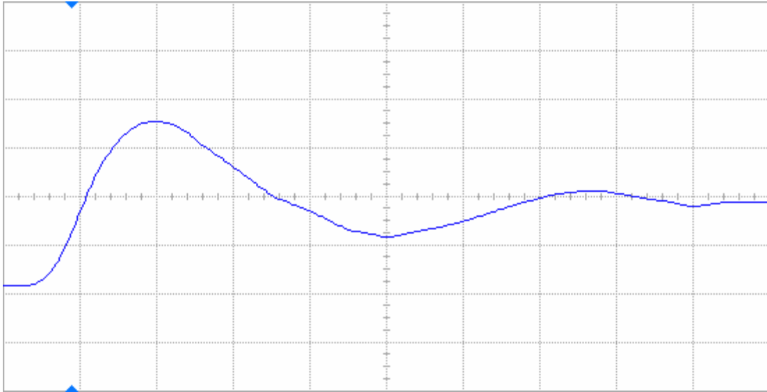
Figure 7(a) DUT 465 pre-irradiation rising edge, abscissa scale is 2 V/div and ordinate scale is 2 ns/div.
