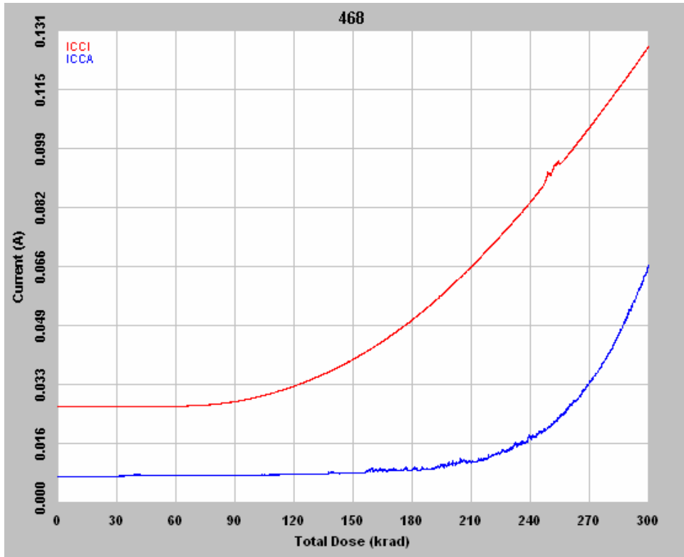
Figure 4 DUT 468 in-flux I_{CCA} and I_{CCI}
