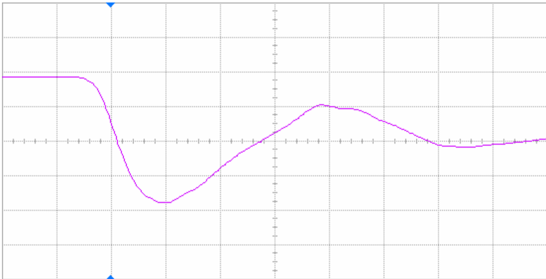
Figure 11(b) DUT 462 post-annealing falling edge, abscissa scale is 2 V/div and ordinate scale is 2 ns/div.
