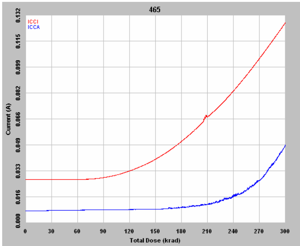
Figure 2 DUT 465 in-flux I_{CCA} and I_{CCI}
