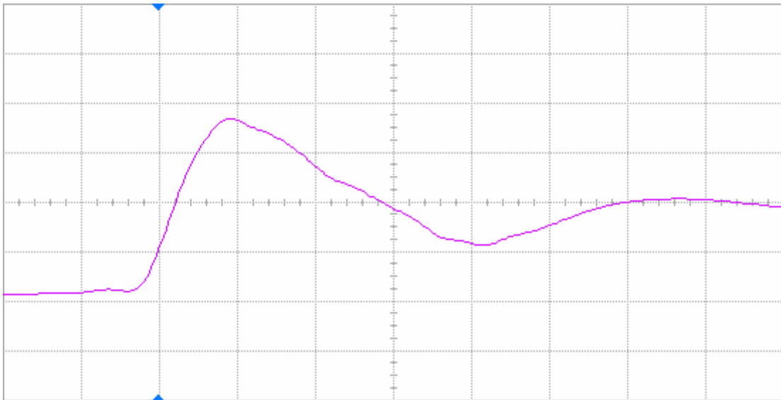
Figure 10(b) DUT 469 post-annealing rising edge, abscissa scale is 2 V/div and ordinate scale is 2 ns/div.
