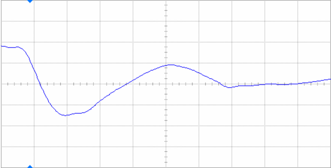
Figure 14(a) DUT 468 pre-irradiation falling edge, abscissa scale is 2 V/div and ordinate scale is 2 ns/div.
