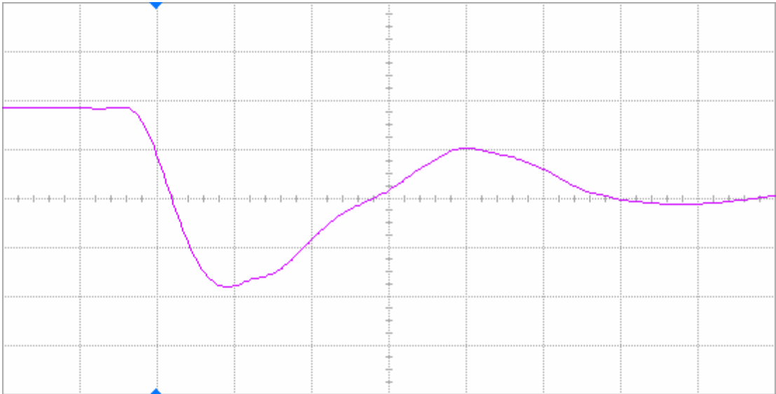
Figure 12(b) DUT 465 post-annealing falling edge, abscissa scale is 2 V/div and ordinate scale is 2 ns/div.
