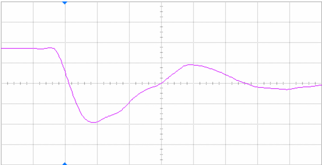
Figure 14(b) DUT 468 post-annealing falling edge, abscissa scale is 2 V/div and ordinate scale is 2 ns/div.
