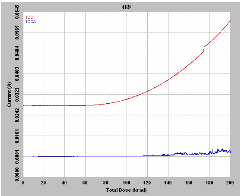
Figure 5 DUT 469 in-flux I_{CCA} and I_{CCI}
