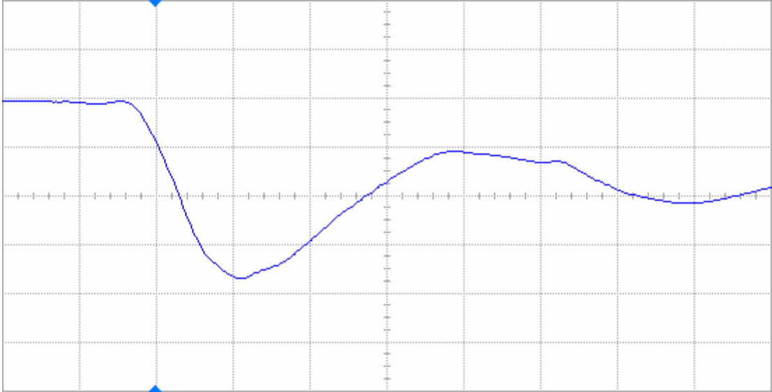
Figure 15(a) DUT 469 pre-irradiation falling edge, abscissa scale is 2 V/div and ordinate scale is 2 ns/div.
