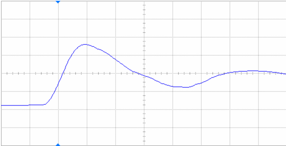
Figure 6(a) DUT 462 pre-irradiation rising edge, abscissa scale is 2 V/div and ordinate scale is 2 ns/div.
