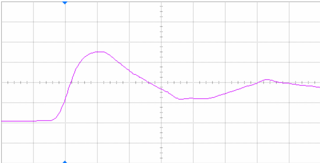
Figure 9(b) DUT 468 post-annealing rising edge, abscissa scale is 2 V/div and ordinate scale is 2 ns/div.
