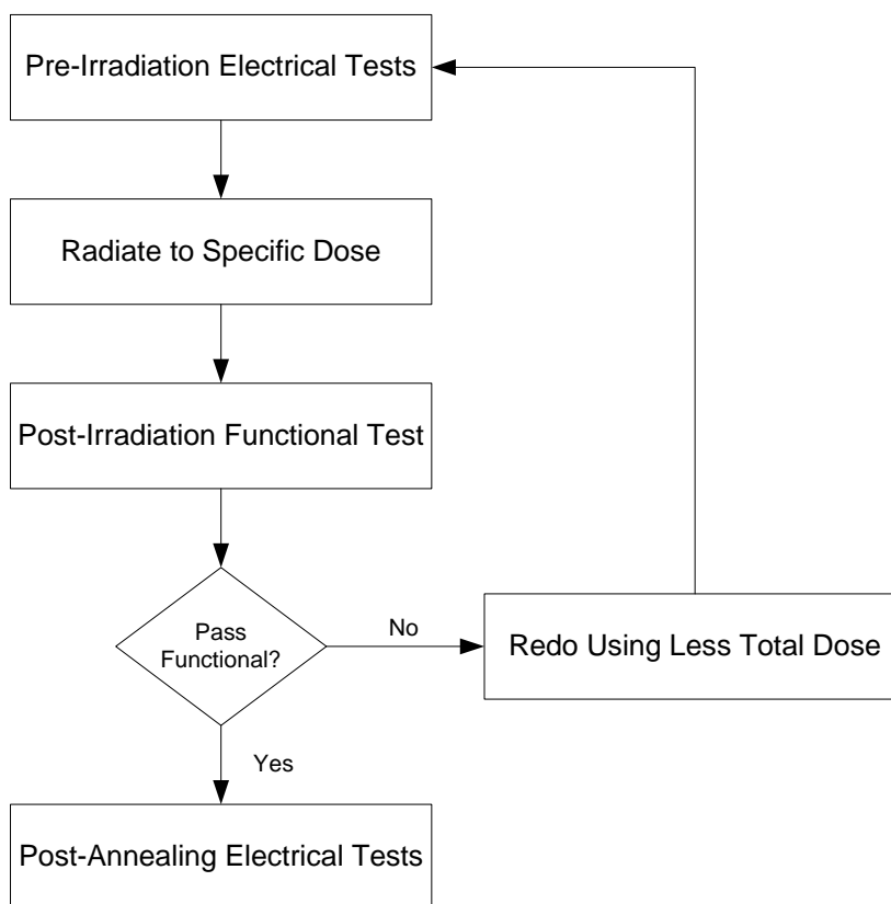
Figure 1 Parametric test flow chart
