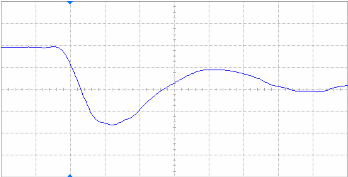
Figure 11(a) DUT 462 pre-irradiation falling edge, abscissa scale is 2 V/div and ordinate scale is 2 ns/div.
