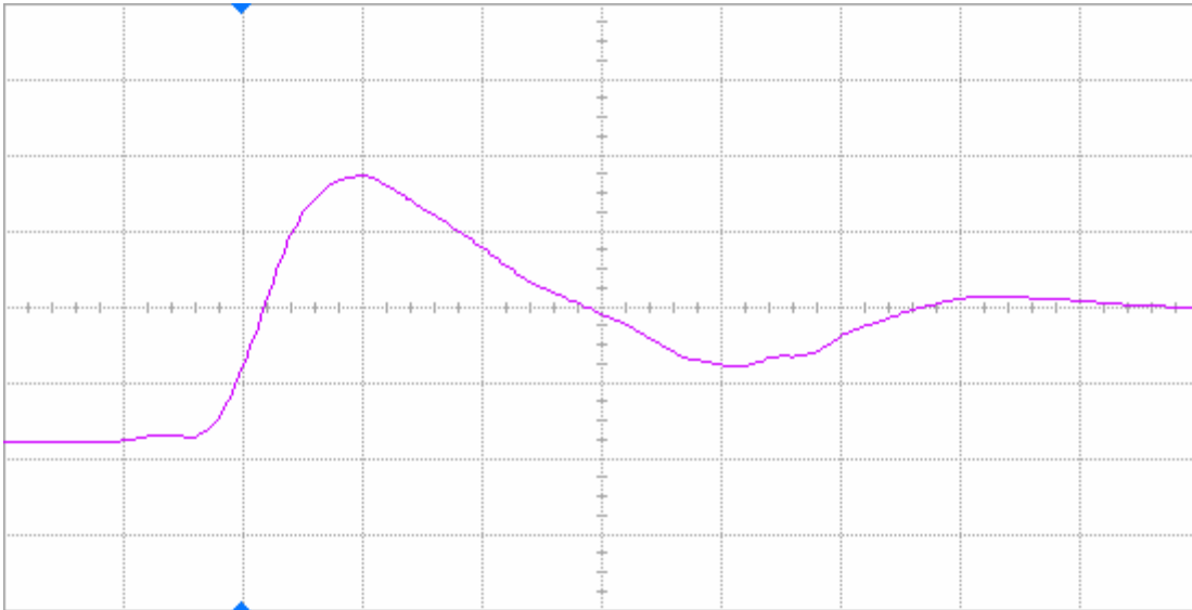
Figure 8(b) DUT 466 post-annealing rising edge, abscissa scale is 2 V/div and ordinate scale is 2 ns/div.
