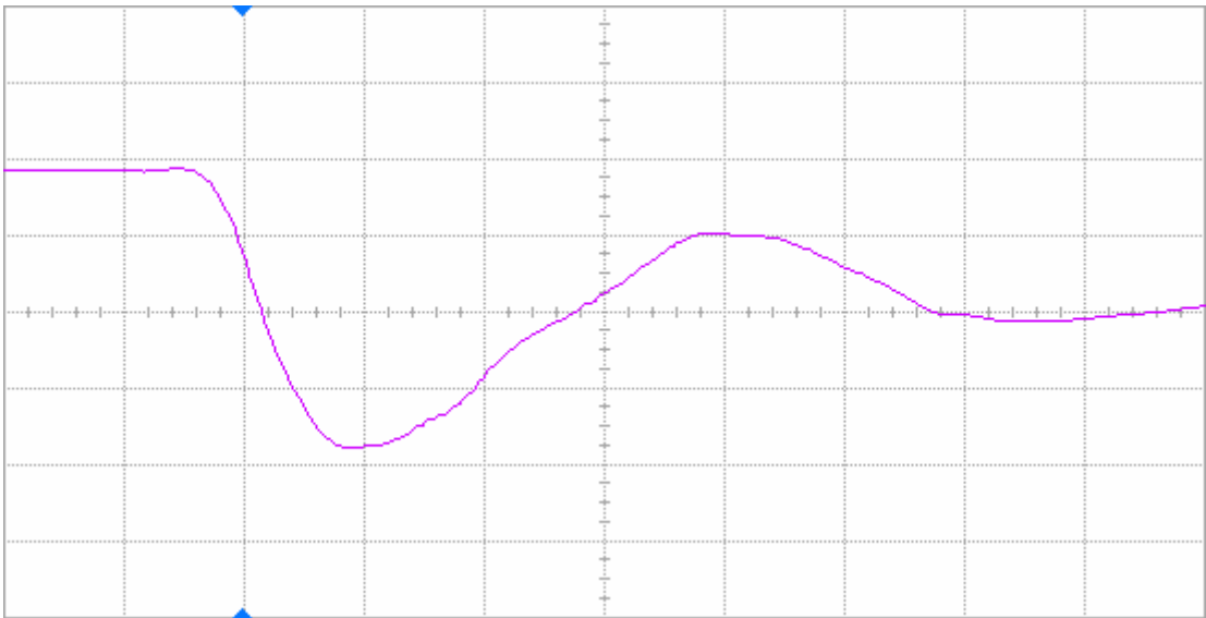
Figure 13(b) DUT 466 post-annealing falling edge, abscissa scale is 2 V/div and ordinate scale is 2 ns/div.
