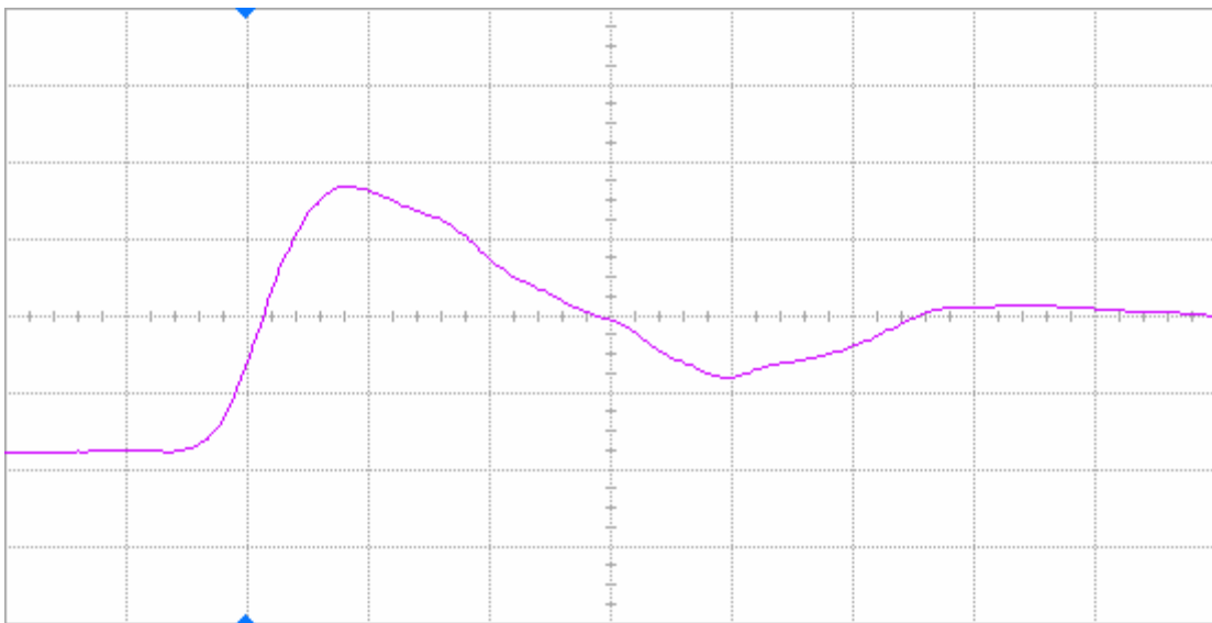
Figure 6(b) DUT 462 post-annealing rising edge, abscissa scale is 2 V/div and ordinate scale is 2 ns/div.
