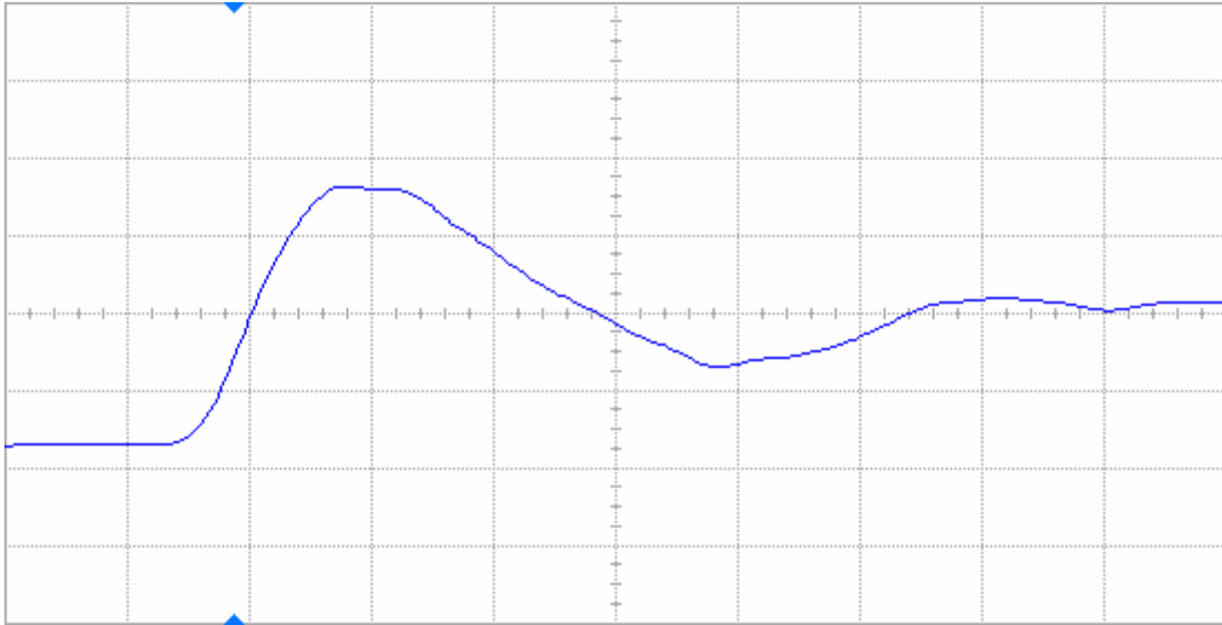
Figure 9(a) DUT 468 pre-irradiation rising edge, abscissa scale is 2 V/div and ordinate scale is 2 ns/div.
