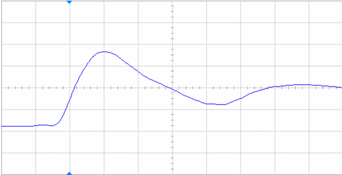
Figure 10(a) DUT 469 pre-irradiation rising edge, abscissa scale is 2 V/div and ordinate scale is 2 ns/div.
