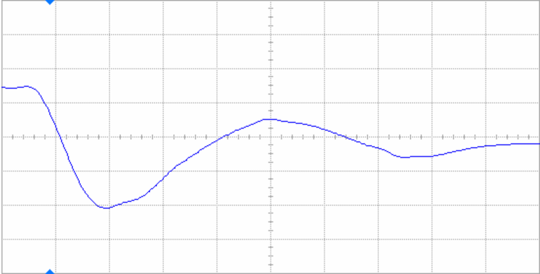
Figure 12(a) DUT 465 pre-irradiation falling edge, abscissa scale is 2 V/div and ordinate scale is 2 ns/div.
