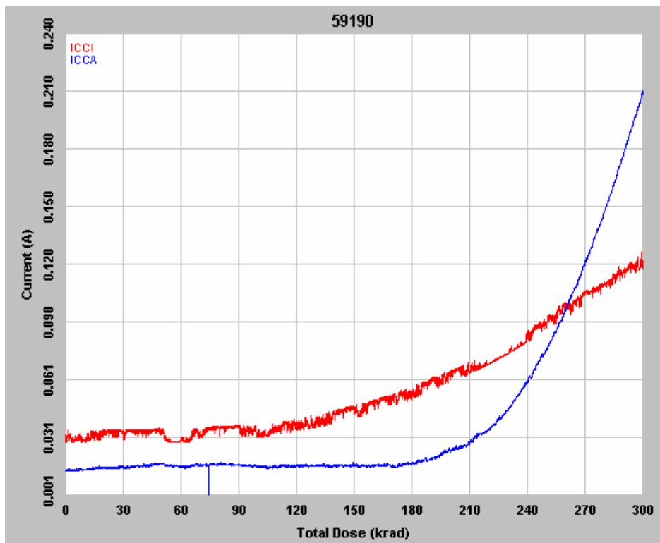
Figure 7 DUT 59190 in-flux I_{CCA} and I_{CCI}
