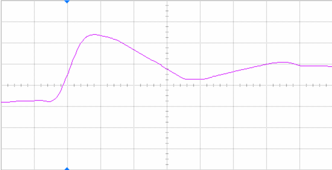
Figure 9(a) DUT 59170 pre-irradiation rising edge, abscissa scale is 2 V/div and ordinate scale is 2 ns/div.
