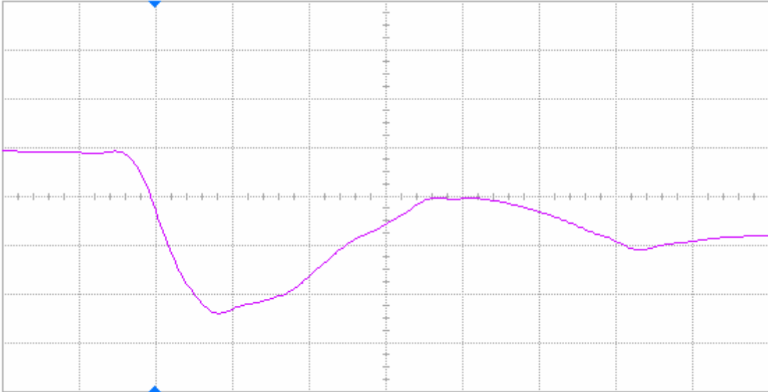
Figure 16(a) DUT 59206 pre-irradiation falling edge, abscissa scale is 2 V/div and ordinate scale is 2 ns/div.
