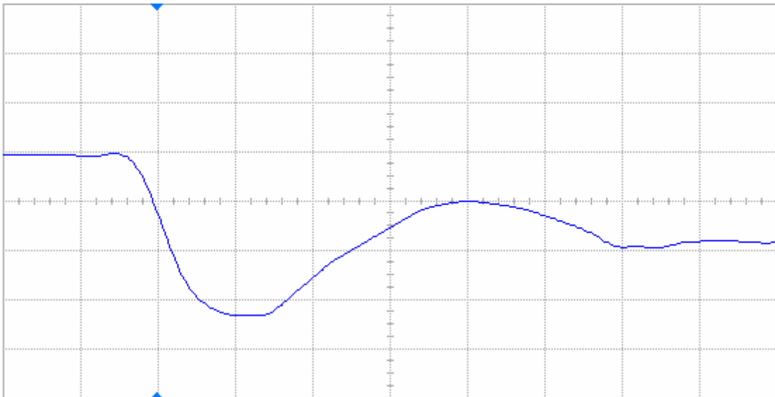
Figure 19(b) DUT 59190 post-annealing falling edge, abscissa scale is 2 V/div and ordinate scale is 2 ns/div.
