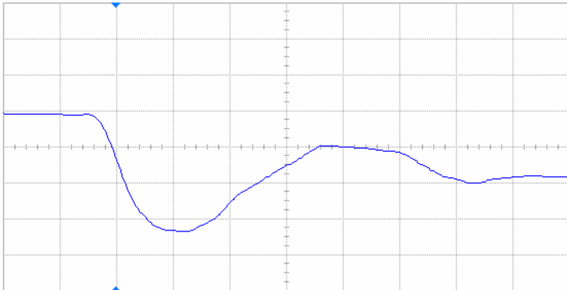
Figure 16(b) DUT 59206 post-annealing falling edge, abscissa scale is 2 V/div and ordinate scale is 2 ns/div.
