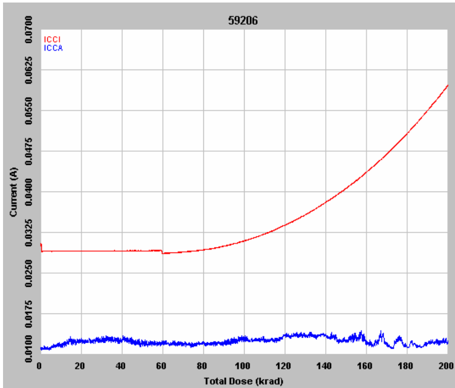
Figure 4 DUT 59206 in-flux I_{CCA} and I_{CCI}
