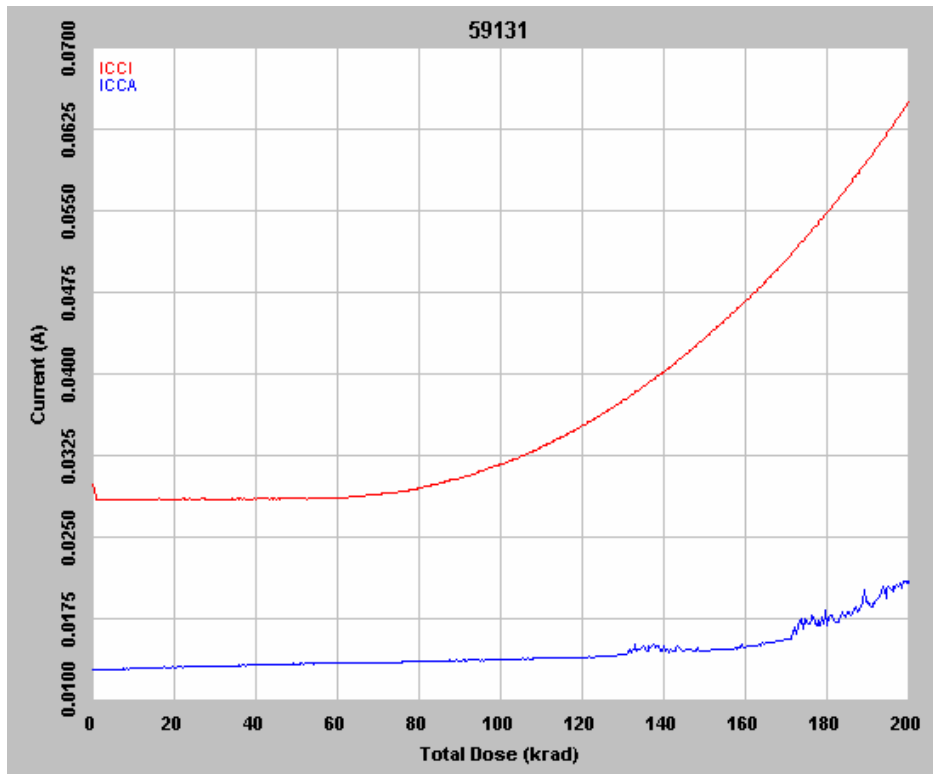
Figure 2 DUT 59131 in-flux I_{CCA} and I_{CCI}
