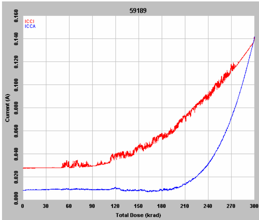
Figure 6 DUT 59189 in-flux I_{CCA} and I_{CCI}
