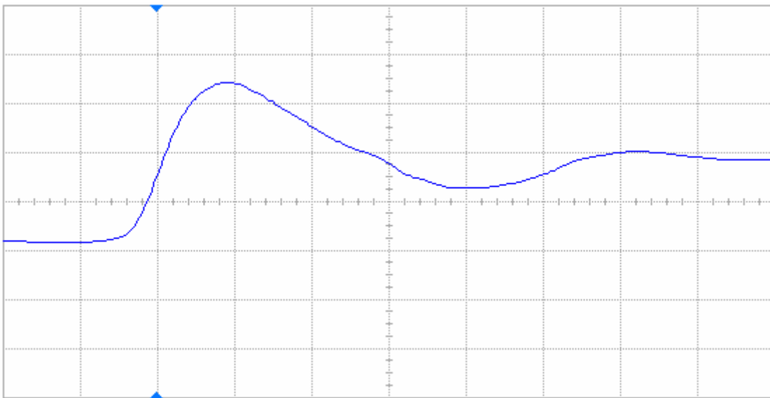
Figure 8(b) DUT 59131 post-annealing rising edge, abscissa scale is 2 V/div and ordinate scale is 2 ns/div.
