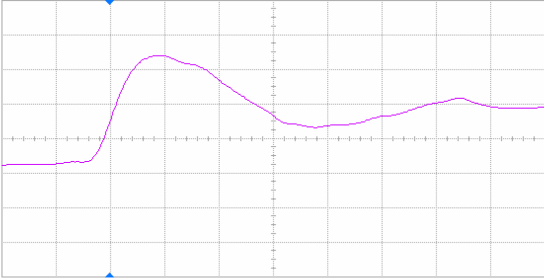
Figure 12(a) DUT 59189 pre-irradiation rising edge, abscissa scale is 2 V/div and ordinate scale is 2 ns/div.
