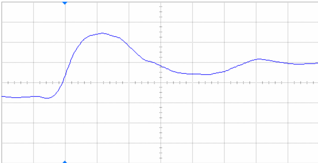
Figure 10(b) DUT 59206 post-annealing rising edge, abscissa scale is 2 V/div and ordinate scale is 2 ns/div.
