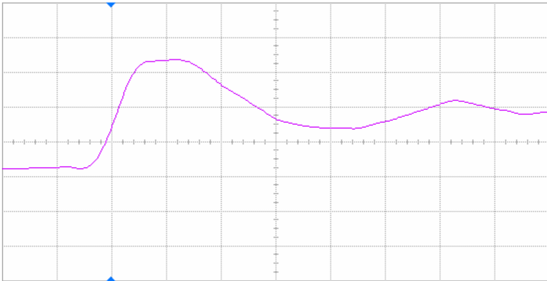
Figure 8(a) DUT 59131 pre-irradiation rising edge, abscissa scale is 2 V/div and ordinate scale is 2 ns/div.
