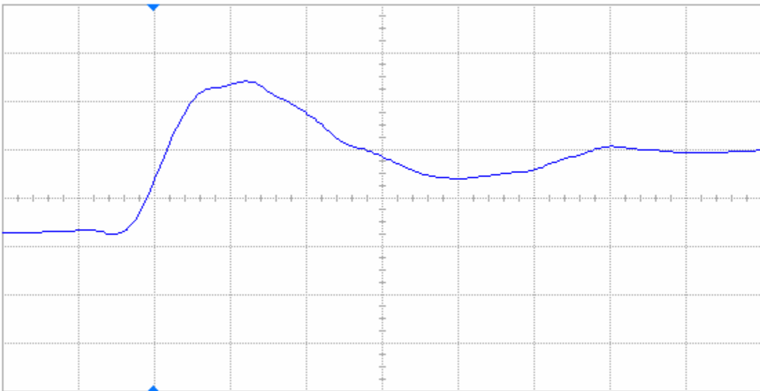
Figure 13(b) DUT 59190 post-annealing rising edge, abscissa scale is 2 V/div and ordinate scale is 2 ns/div.
