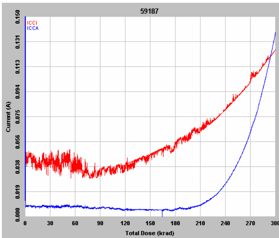
Figure 5 DUT 59187 in-flux I_{CCA} and I_{CCI}
