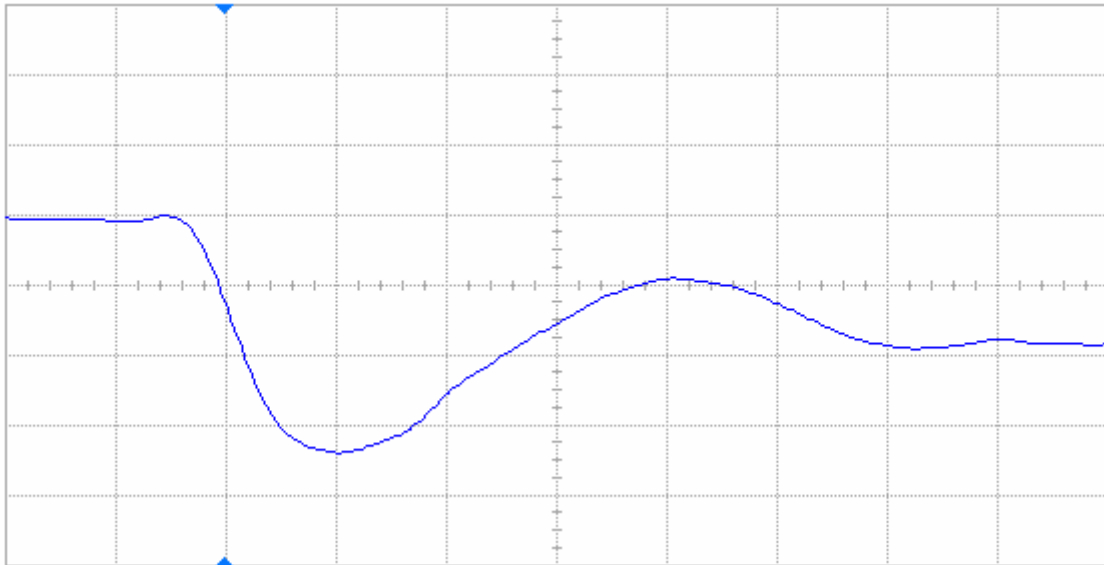
Figure 15(b) DUT 59170 post-annealing falling edge, abscissa scale is 2 V/div and ordinate scale is 2 ns/div.
