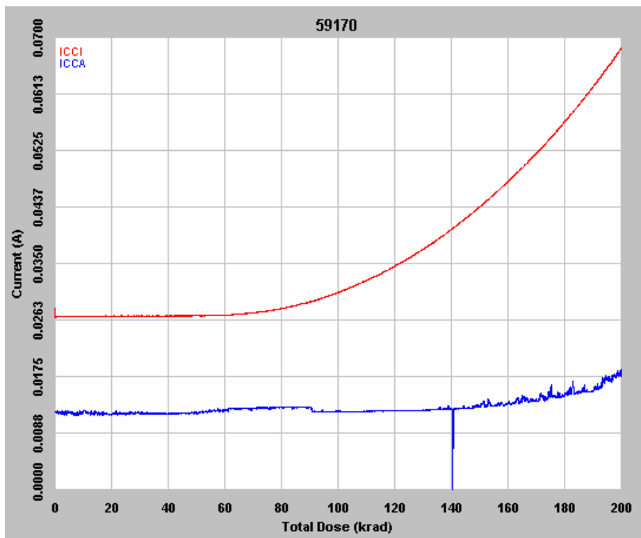
Figure 3 DUT 59170 in-flux I_{CCA} and I_{CCI}
