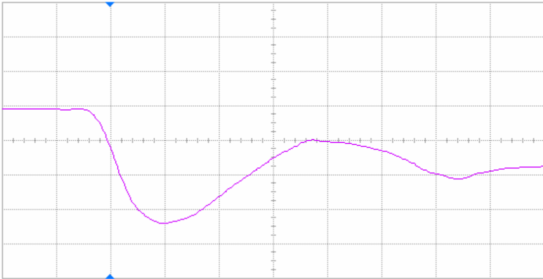
Figure 14(a) DUT 59131 pre-irradiation falling edge, abscissa scale is 2 V/div and ordinate scale is 2 ns/div.
