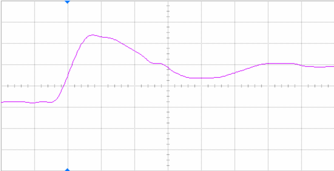
Figure 13(a) DUT 59190 pre-irradiation rising edge, abscissa scale is 2 V/div and ordinate scale is 2 ns/div.
