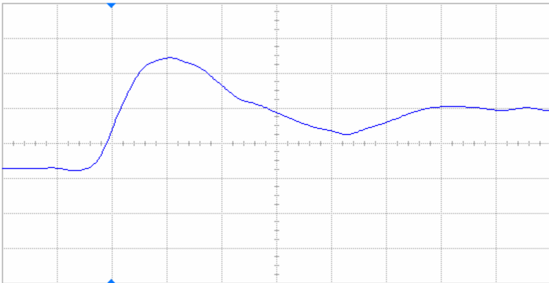
Figure 11(b) DUT 59187 post-annealing rising edge, abscissa scale is 2 V/div and ordinate scale is 2 ns/div.
