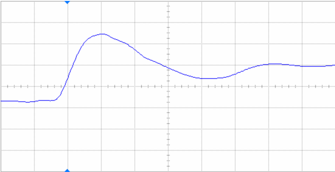
Figure 9(b) DUT 59170 post-annealing rising edge, abscissa scale is 2 V/div and ordinate scale is 2 ns/div.
