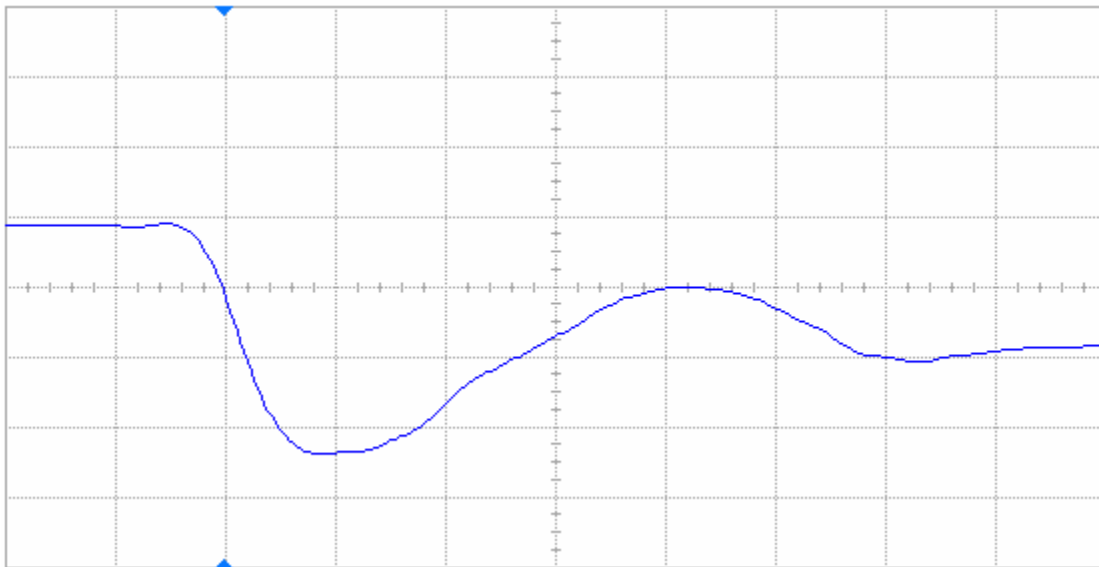
Figure 14(b) DUT 59131 post-annealing falling edge, abscissa scale is 2 V/div and ordinate scale is 2 ns/div.
