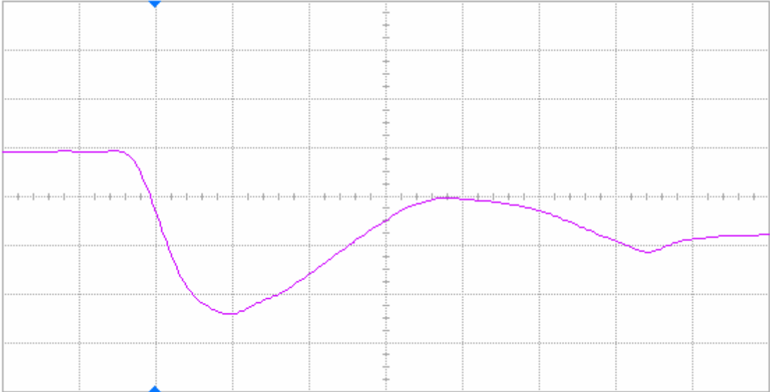
Figure 18(a) DUT 59189 pre-irradiation falling edge, abscissa scale is 2 V/div and ordinate scale is 2 ns/div.
