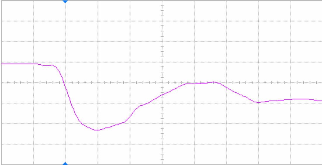
Figure 15(a) DUT 61544 pre-irradiation falling edge, abscissa scale is 2 V/div and ordinate scale is 2 ns/div.
