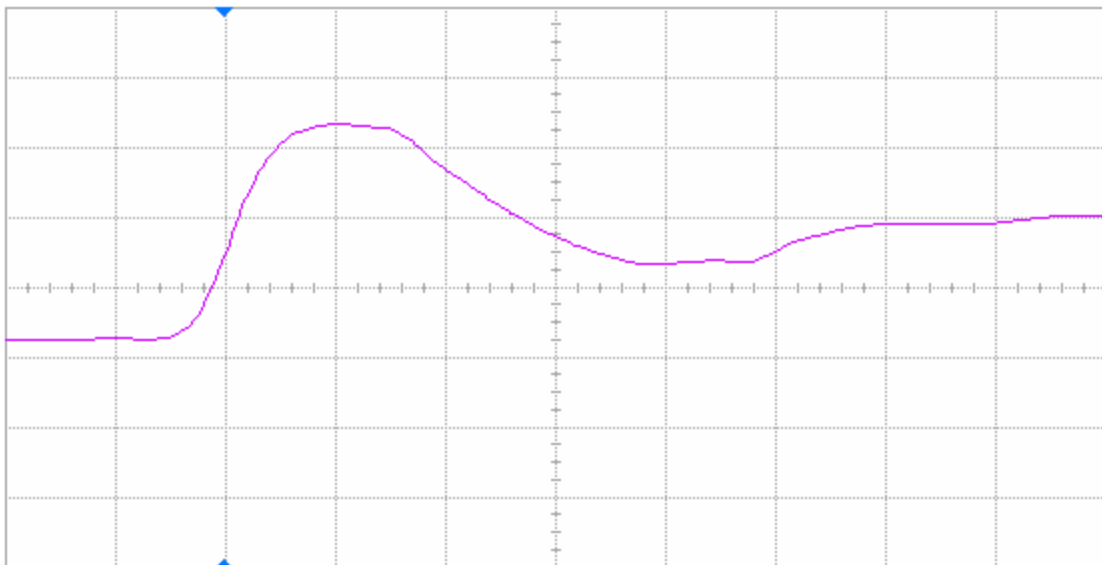
Figure 13(b) DUT 61561 post-annealing rising edge, abscissa scale is 2 V/div and ordinate scale is 2 ns/div.
