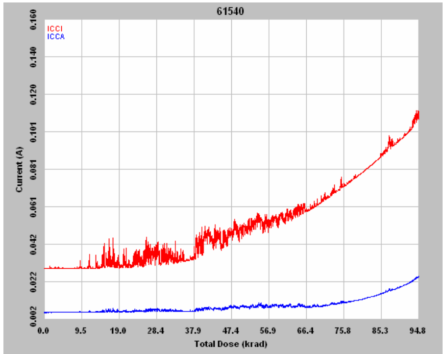
Figure 2 DUT 61540 in-flux I_{CCA} and I_{CCI}
