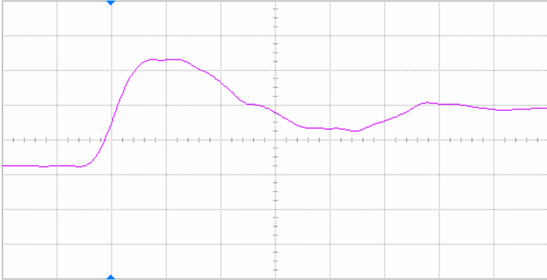
Figure 12(a) DUT 61547 pre-irradiation rising edge, abscissa scale is 2 V/div and ordinate scale is 2 ns/div.
