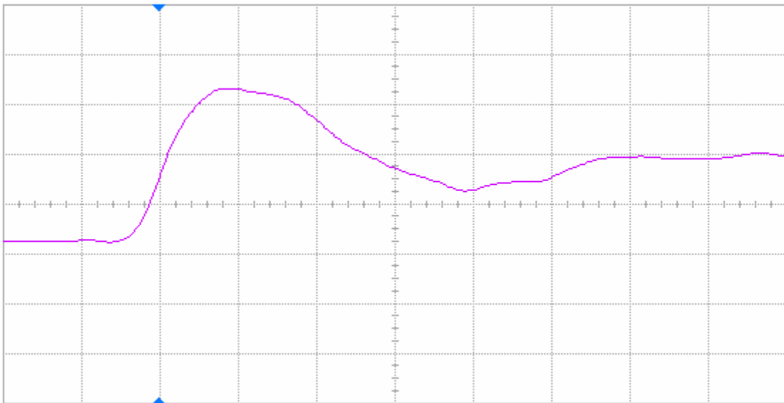
Figure 9(b) DUT 61544 post-annealing rising edge, abscissa scale is 2 V/div and ordinate scale is 2 ns/div.
