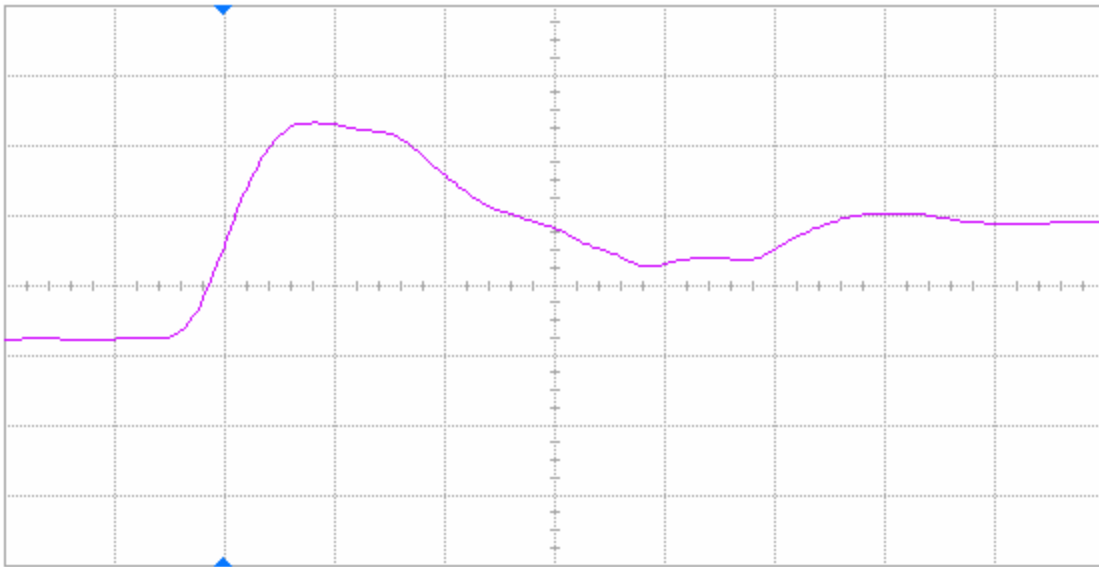
Figure 8(a) DUT 61540 pre-irradiation rising edge, abscissa scale is 2 V/div and ordinate scale is 2 ns/div.
