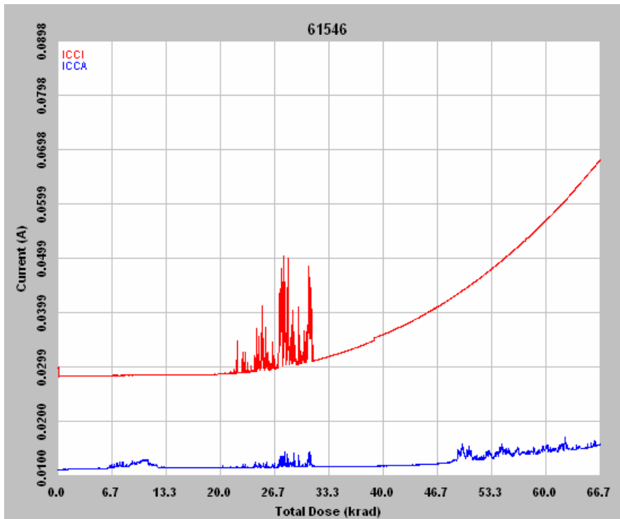
Figure 5 DUT 61546 in-flux I_{CCA} and I_{CCI}
