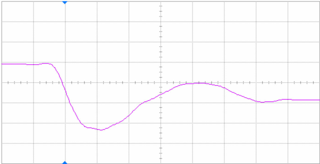
Figure 14(a) DUT 61540 pre-irradiation falling edge, abscissa scale is 2 V/div and ordinate scale is 2 ns/div.
