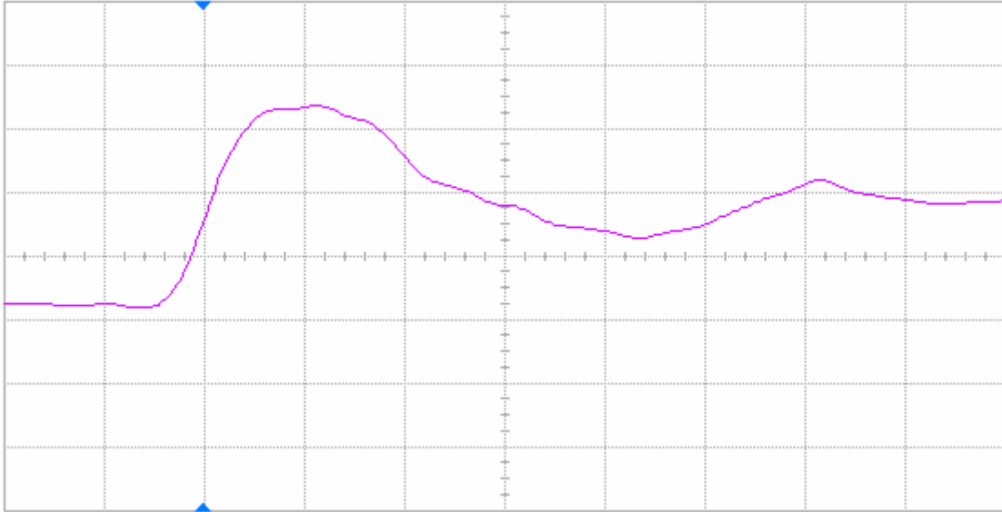
Figure 11(a) DUT 61546 pre-irradiation rising edge, abscissa scale is 2 V/div and ordinate scale is 2 ns/div.
