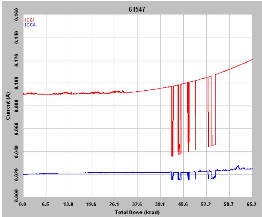
Figure 6 DUT 61547 in-flux I CCA and I CCI
