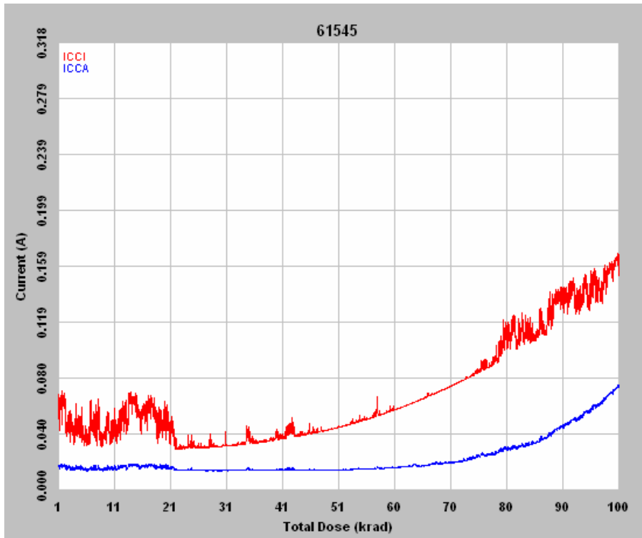
Figure 4 DUT 61545 in-flux I_{CCA} and I_{CCI}
