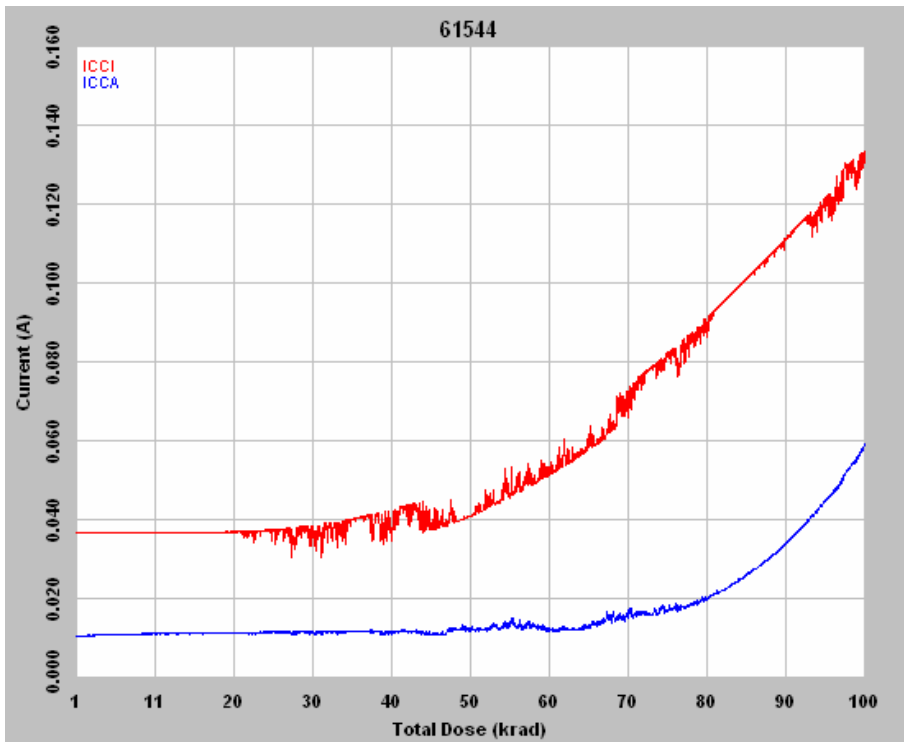
Figure 3 DUT 61544 in-flux I_{CCA} and I_{CCI}
