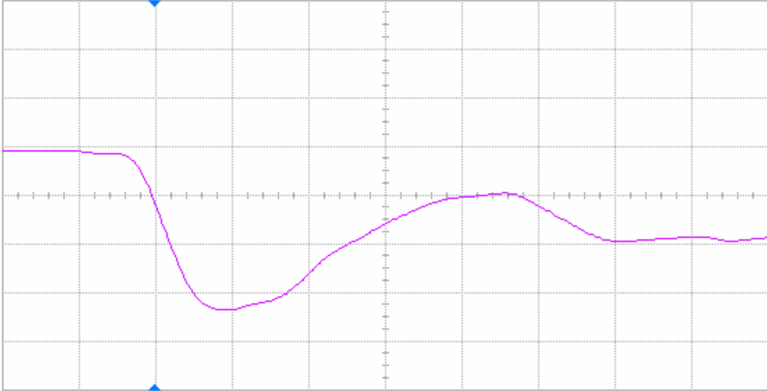
Figure 16(a) DUT 61545 pre-irradiation falling edge, abscissa scale is 2 V/div and ordinate scale is 2 ns/div.
