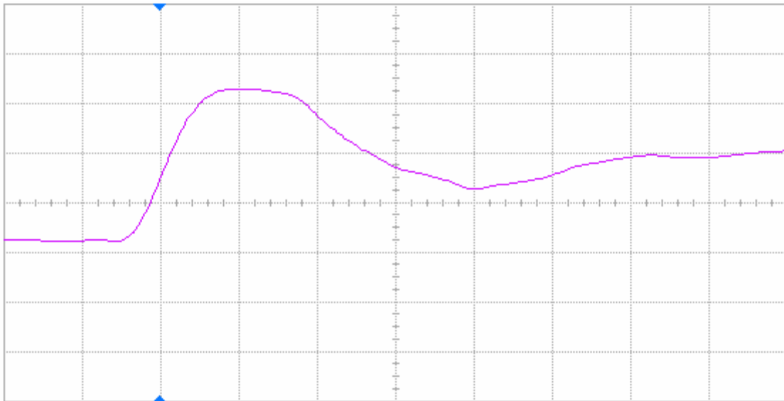
Figure 11(b) DUT 61546 post-annealing rising edge, abscissa scale is 2 V/div and ordinate scale is 2 ns/div.
