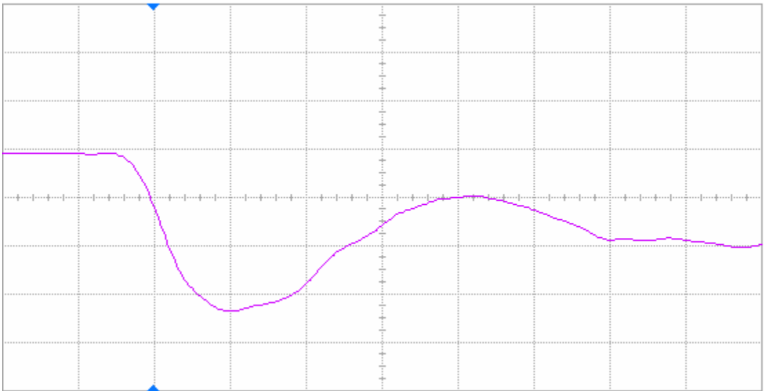
Figure 17(b) DUT 61546 post-annealing falling edge, abscissa scale is 2 V/div and ordinate scale is 2 ns/div.
