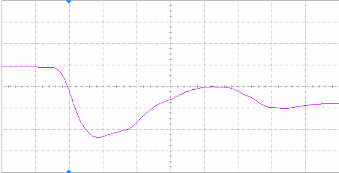
Figure 17(a) DUT 61546 pre-irradiation falling edge, abscissa scale is 2 V/div and ordinate scale is 2 ns/div.
