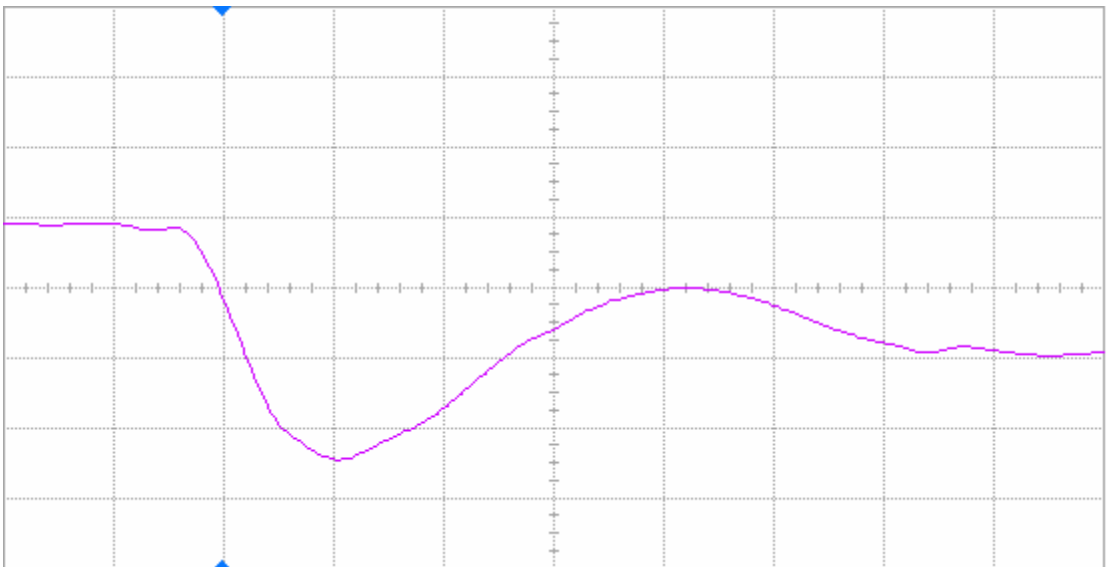
Figure 19(b) DUT 61561 post-annealing falling edge, abscissa scale is 2 V/div and ordinate scale is 2 ns/div.
