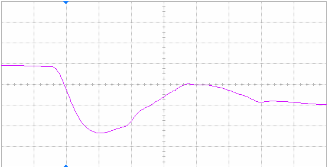
Figure 18(b) DUT 61547 post-annealing falling edge, abscissa scale is 2 V/div and ordinate scale is 2 ns/div.
