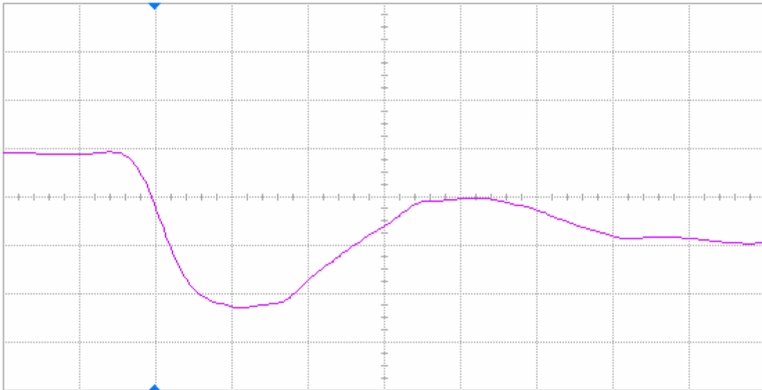
Figure 15(b) DUT 61544 post-annealing falling edge, abscissa scale is 2 V/div and ordinate scale is 2 ns/div.
