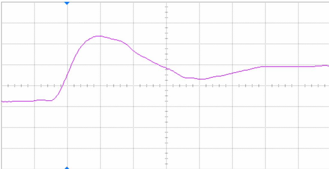
Figure 8(b) DUT 61540 post-annealing rising edge, abscissa scale is 2 V/div and ordinate scale is 2 ns/div.
