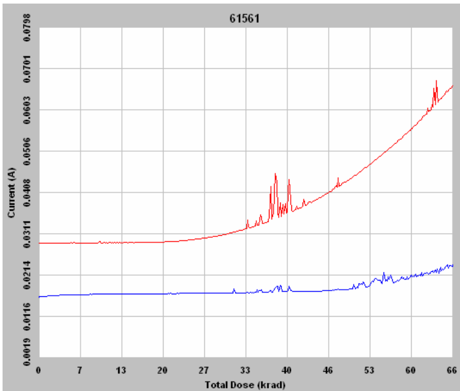
Figure 7 DUT 61561 in-flux I CCA and I CCI
