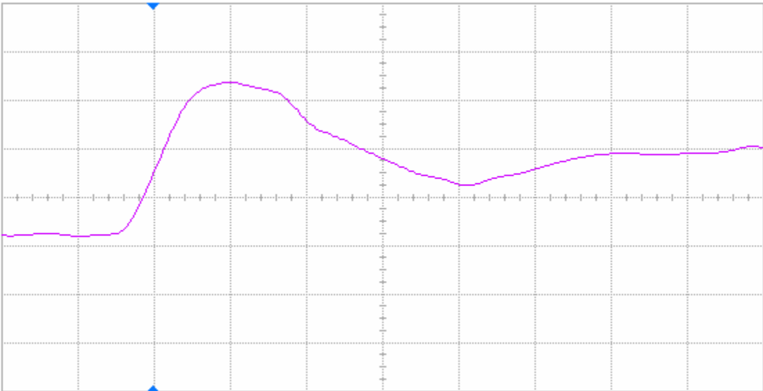
Figure 12(b) DUT 61547 post-annealing rising edge, abscissa scale is 2 V/div and ordinate scale is 2 ns/div.
