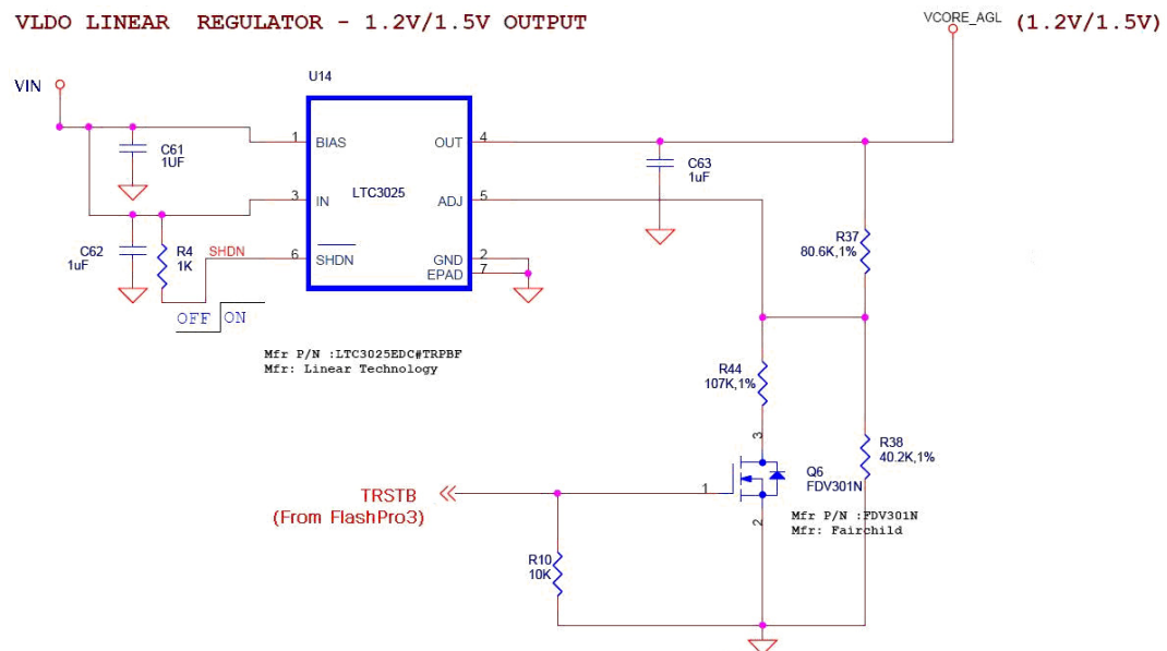
Figure 13-1 • Circuit Diagram
