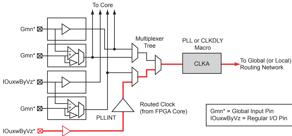
For Fusion devices, the input reference clock can also be from the embedded RC oscillator and crystal oscillator. In this case, the CCC configuration is the same as the hardwired I/O clock source, and users are required to instantiate the RC oscillator or crystal oscillator macro and connect its output to the input reference clock of the CCC block.
