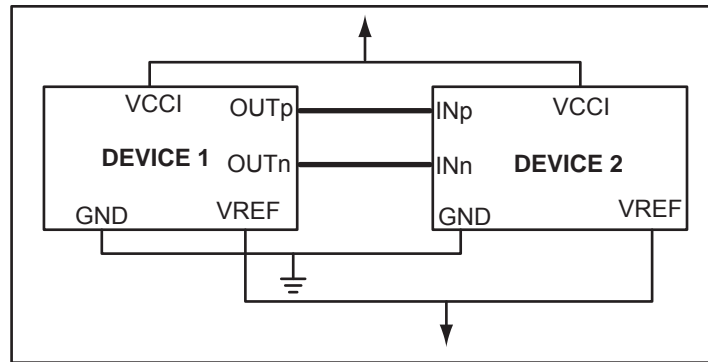
Figure 7-8 • Differential Topology
