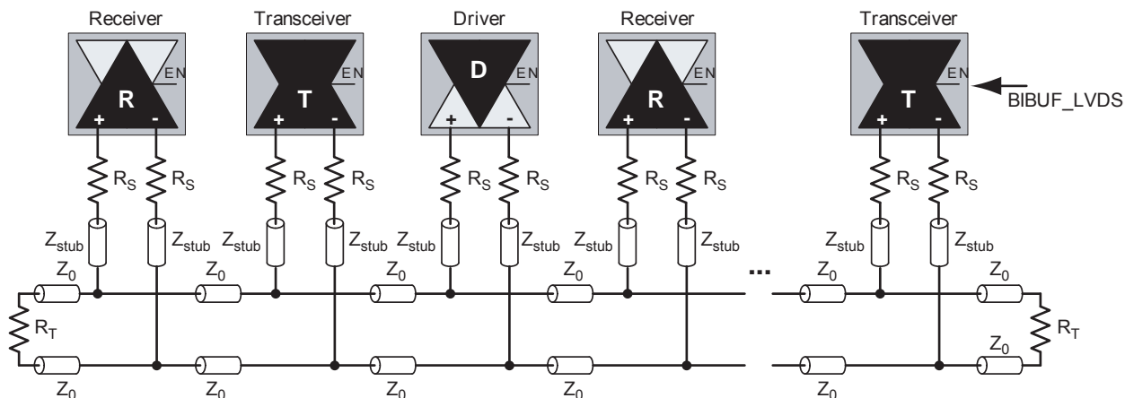
Figure 6-8 • A B-LVDS/M-LVDS Multipoint Application Using LVDS I/O Buffers
