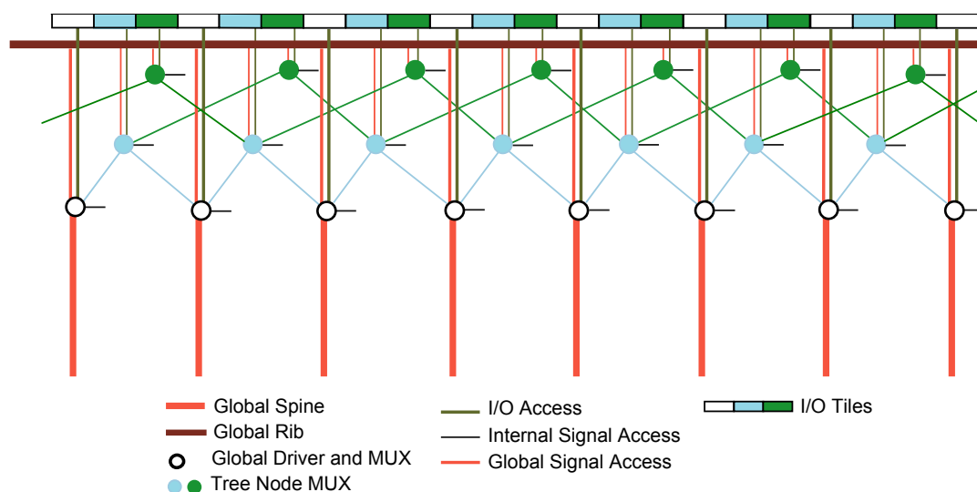
Figure 4-9 • Clock Aggregation Tree Architecture
