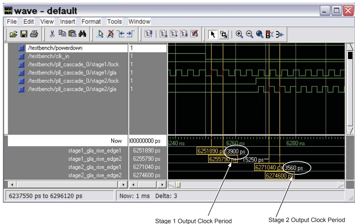
Figure 5-37 • ModelSim Simulation Results
