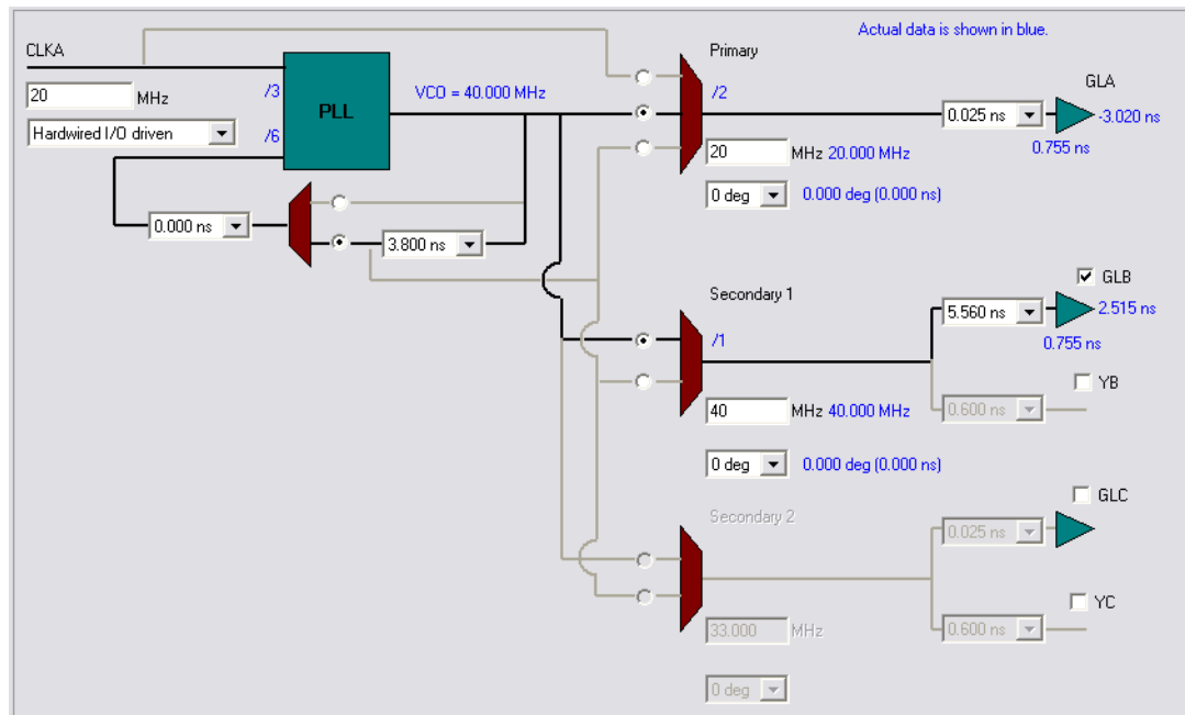
Figure 5-29 • SmartGen Settings
