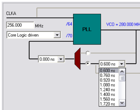
Figure 5-25 • Internal Feedback with Selectable Feedback Delay
