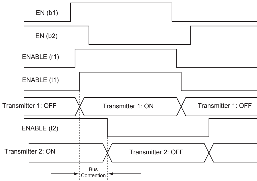
Figure 6-17 • Timing Diagram (bypasses skew circuit)
