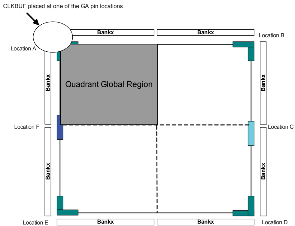
Figure 4-13 • Quadrant Global Region
