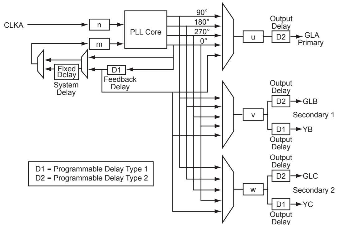
Figure 5-20 • PLL Block Diagram
