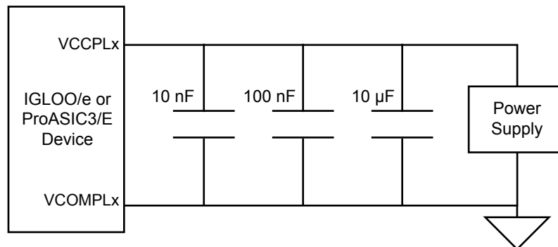
Figure 5-38 • Decoupling Scheme for One PLL (should be replicated for each PLL used)
