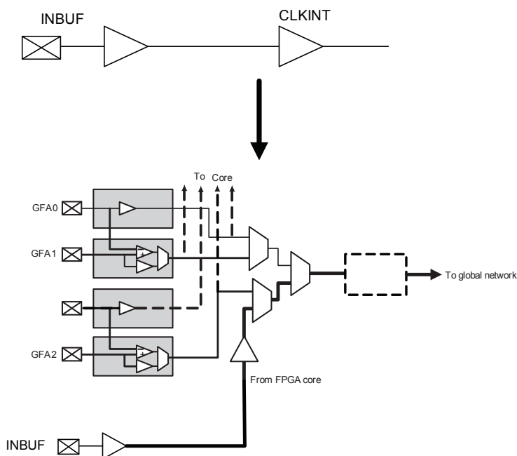
Figure 4-14 • CLKINT Macro
