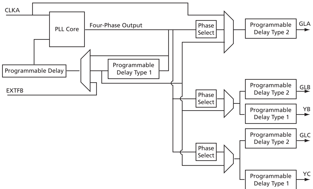
Figure 5-6 • CCC with PLL Block
