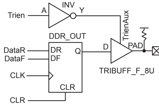
Figure 11-7 • DDR Tristate Output Register, LOW Enable, 8 mA, Pull-Up (LVTTL)
