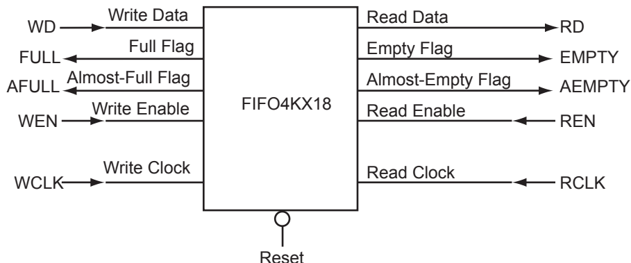
Figure 9-6 • FIFO4KX18 Block Diagram
