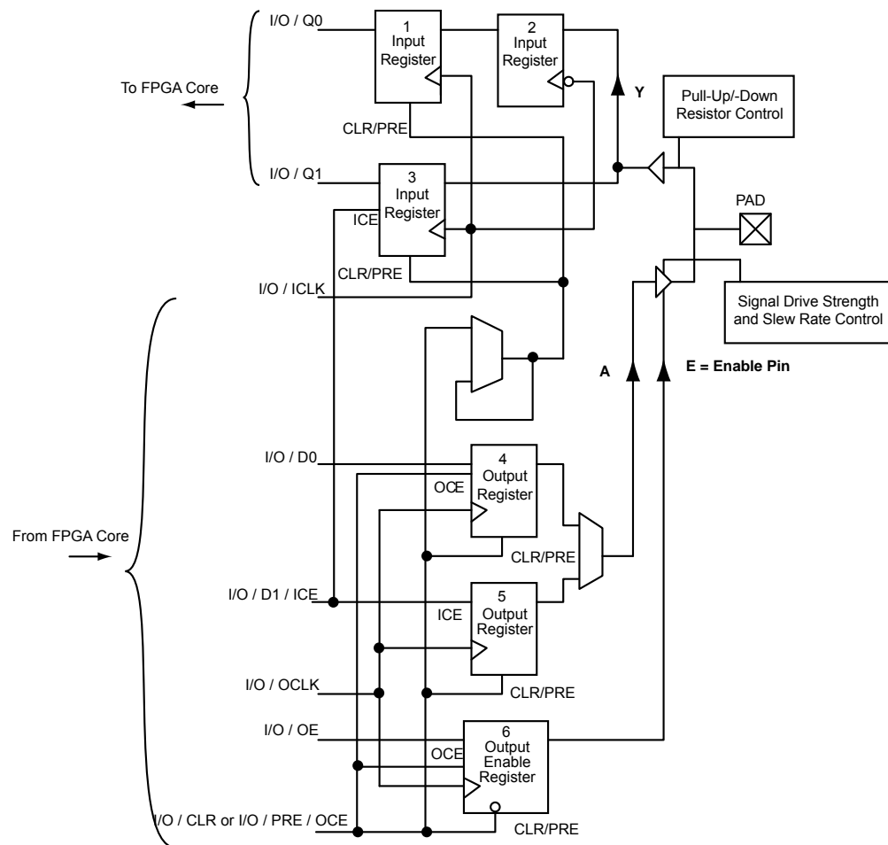
Figure 6-2 • DDR Configured I/O Block Logical Representation
