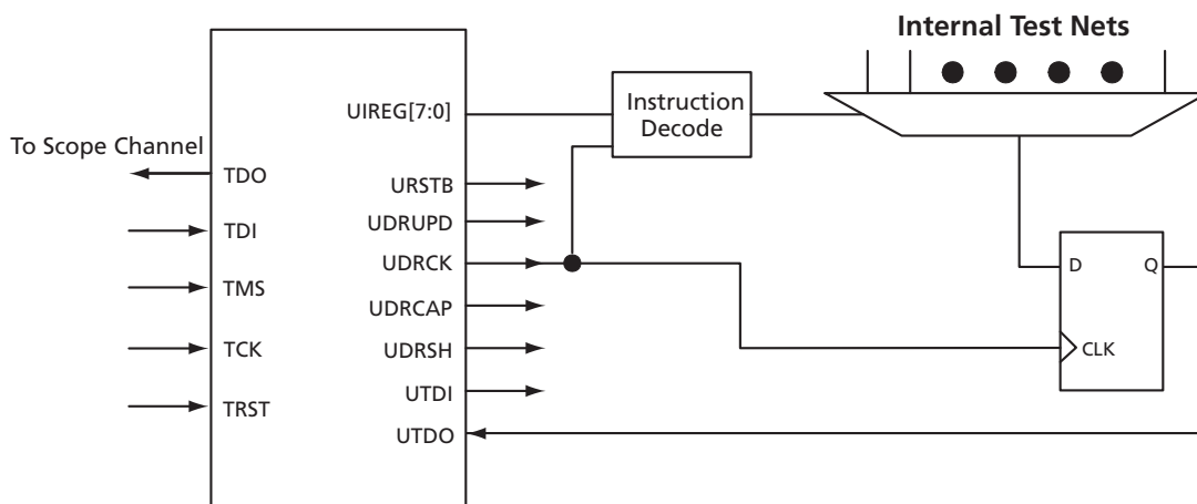
Figure 18-6 • UJTAG Usage Example in Test and Debug Applications
