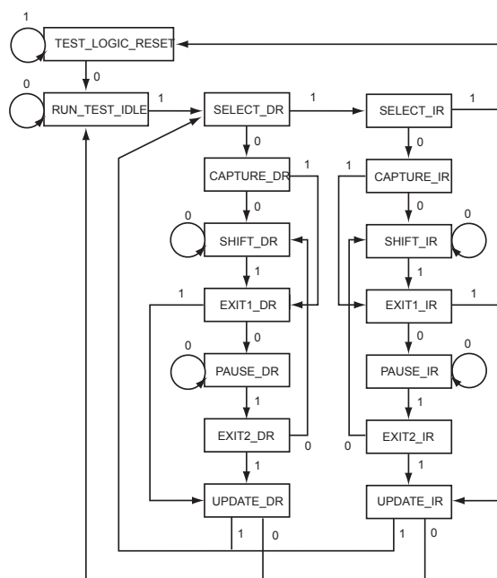
Figure 17-1 • TAP Controller State Machine
