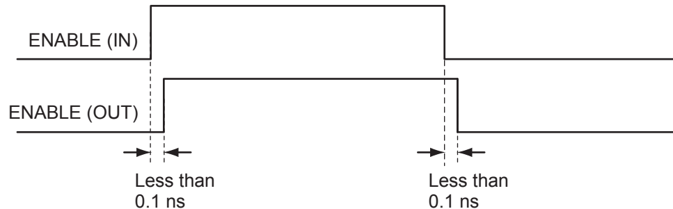
Figure 6-14 • Timing Diagram (option 1: bypasses skew circuit)
