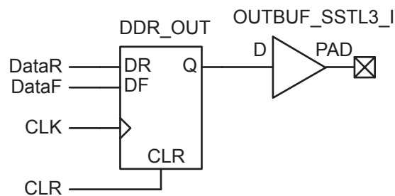
Figure 11-3 • DDR Output Register (SSTL3 Class I)
