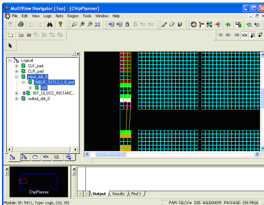
Figure 11-11 • DDR Input/Output Cells as Seen by ChipPlanner for IGLOO/e Devices
