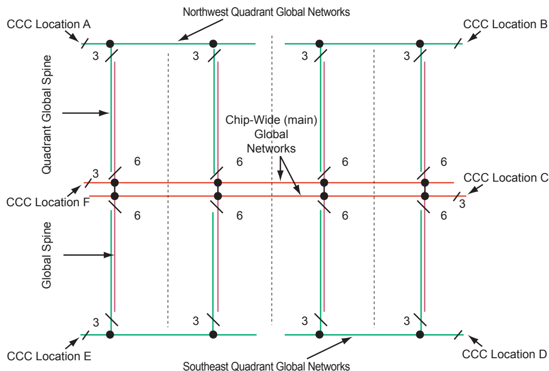
Figure 5-13 • Global Network Architecture for 60 k Gate Devices and Above
