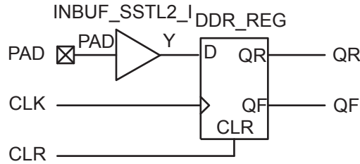
Figure 11-5 • DDR Input Register (SSTL2 Class I)
