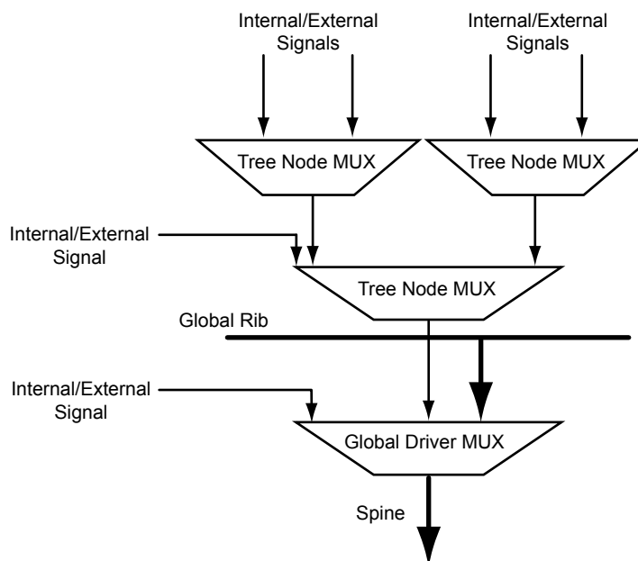
Figure 4-8 • Spine Selection MUX of Global Tree
