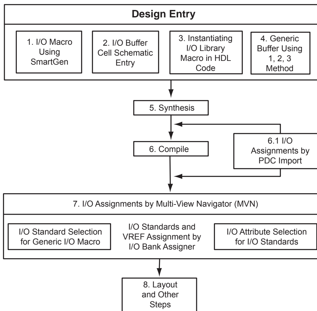
Figure 10-1 • User I/O Assignment Flow Chart
