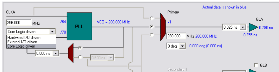
Figure 5-36 • Second-Stage PLL Showing Input of 256 MHz from First Stage and Final Output of 280 MHz
