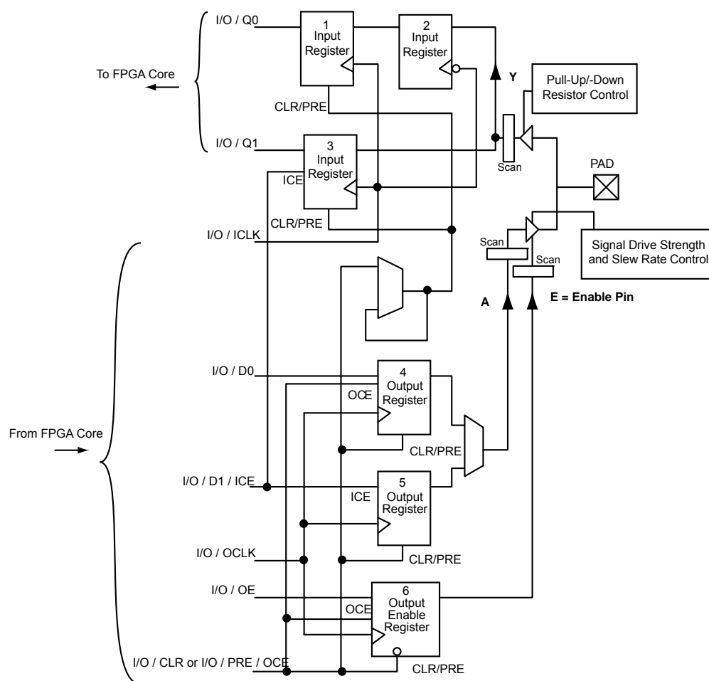
Figure 6-1 • DDR Configured I/O Block Logical Representation
