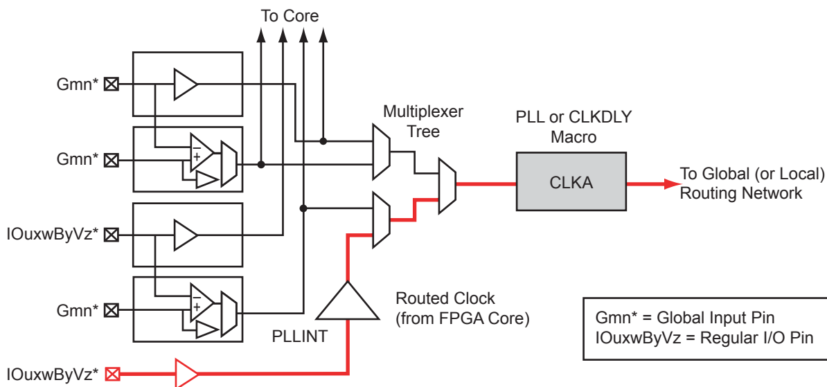
Figure 5-11 • Illustration of External I/O Usage
