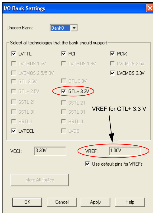
Figure 10-13 • Selecting VREF Voltage for the I/O Bank
