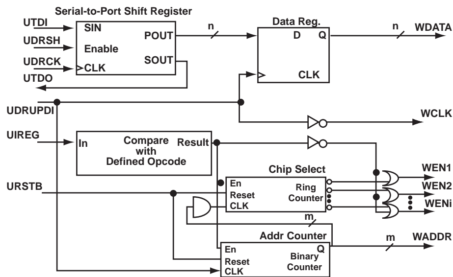
Figure 9-9 • Block Diagram of a Sample User Interface
