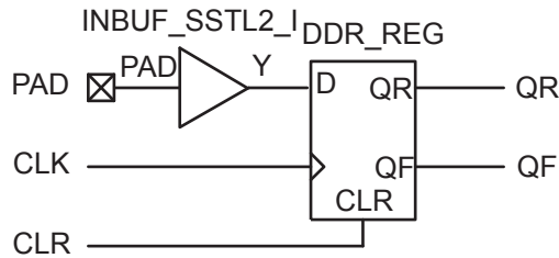
Figure 11-2 • DDR Input Register Support in Low Power Flash Devices
