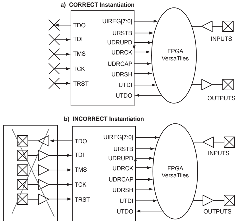
Figure 18-3 • Connectivity Method of UJTAG Macro
