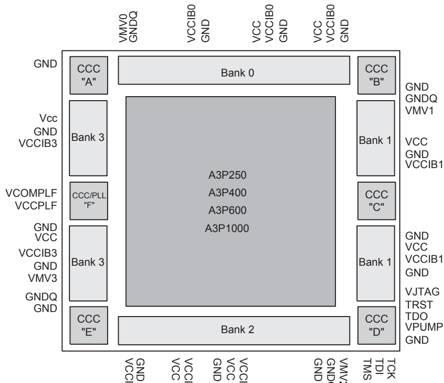
Figure 6-20 • Naming Conventions of IGLOO and ProASIC3 Devices with Four I/O Banks – Top View
