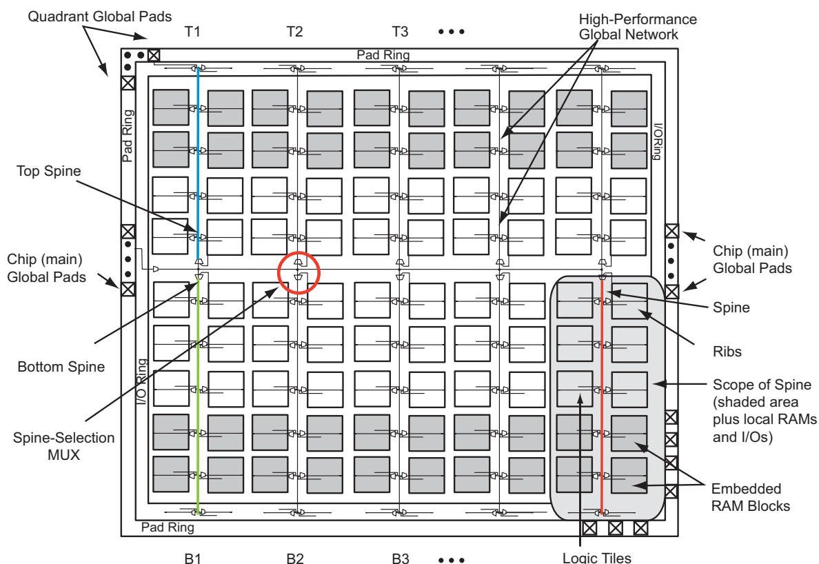
Figure 4-1 • Overview of VersaNet Global Network and Device Architecture
