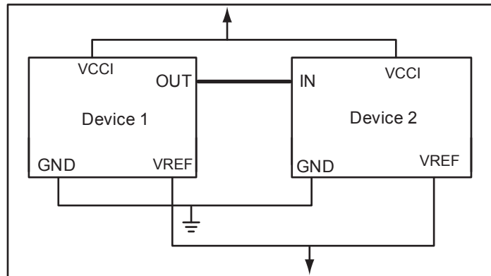
Figure 6-6 • SSTL and HSTL Topology
