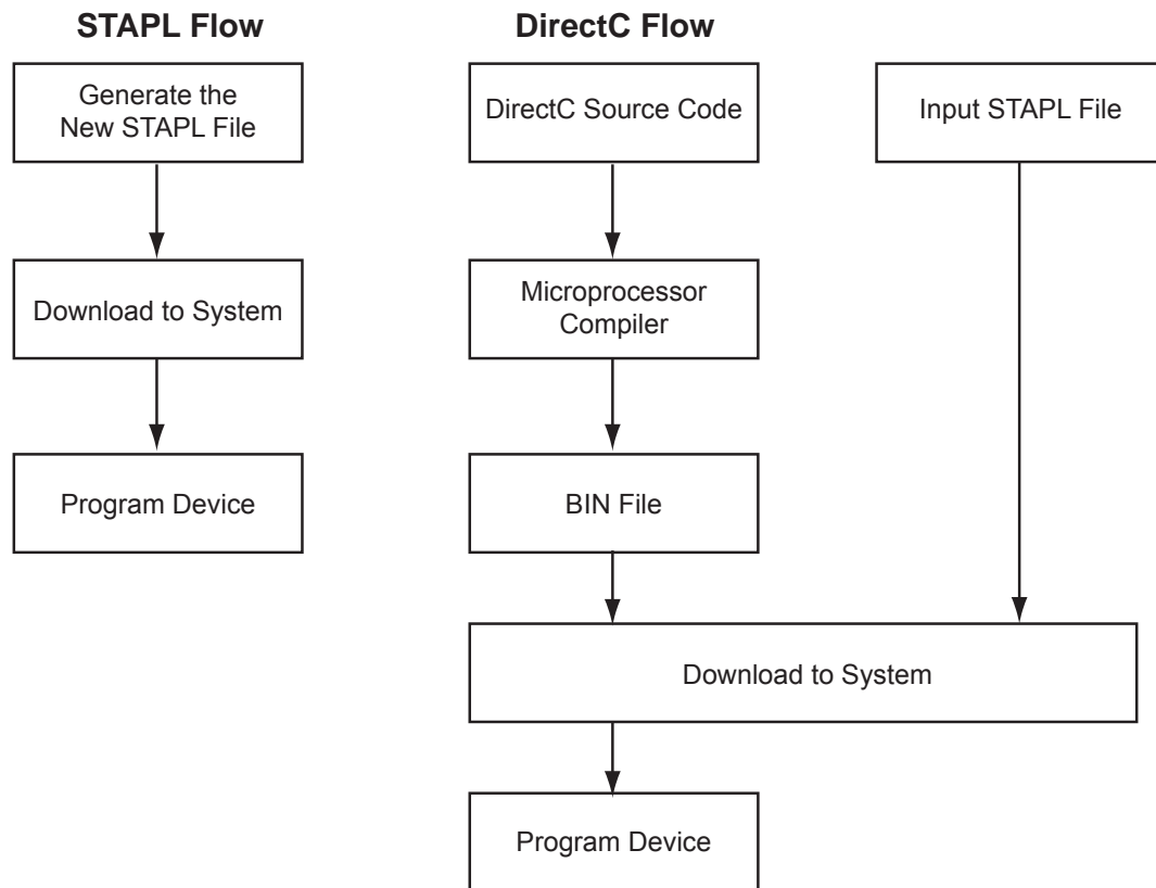
Figure 16-4 • STAPL vs. DirectC
