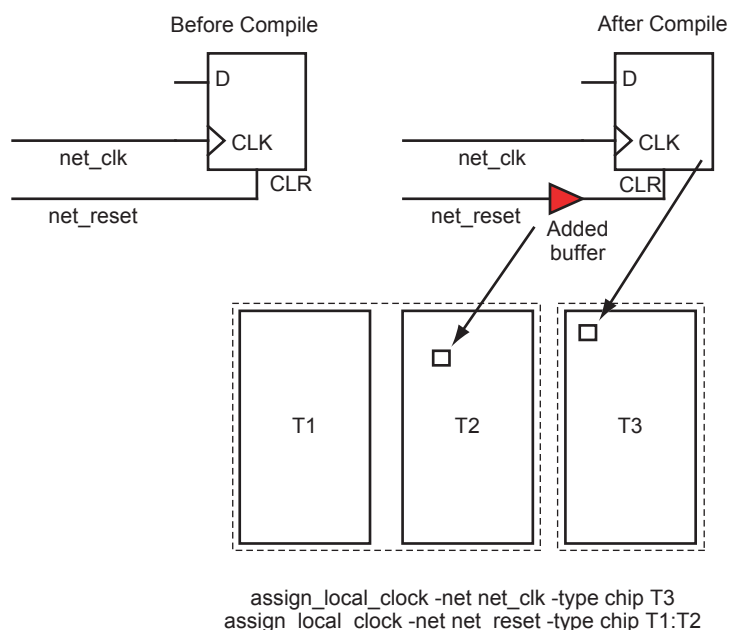
Figure 4-16 • Adding a Buffer for Shared Instances
