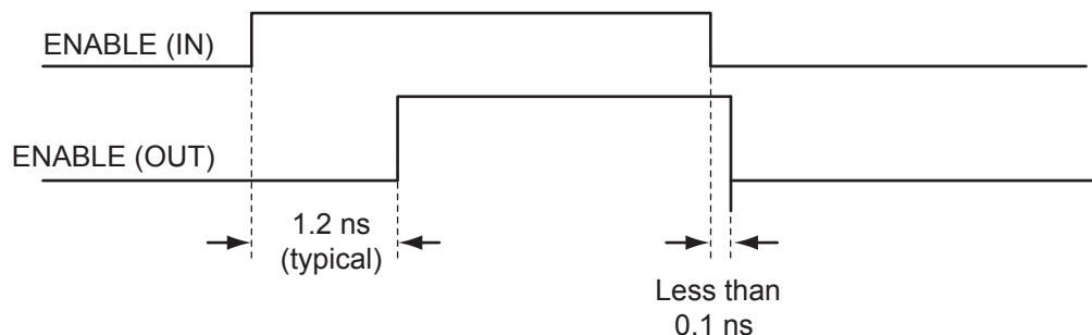
Figure 6-15 • Timing Diagram (option 2: enables skew circuit)
