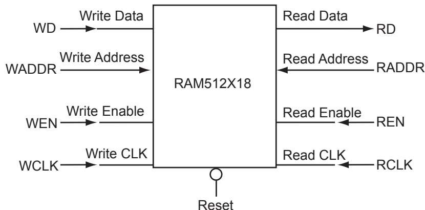
Figure 9-5 • 512X18 Two-Port RAM Block Diagram
