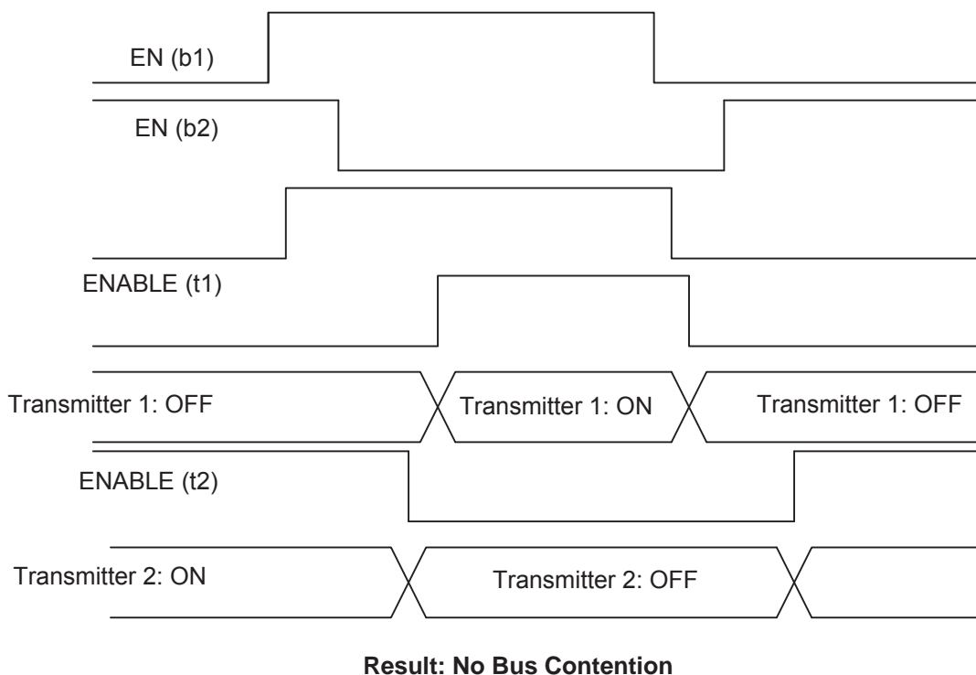
Figure 6-18 • Timing Diagram (with skew circuit selected)
