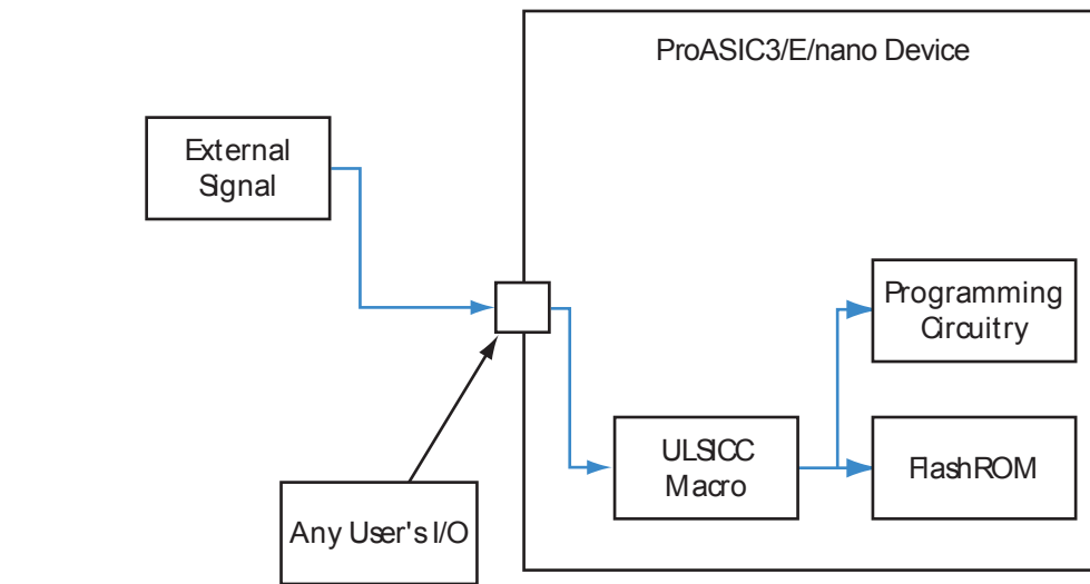
Figure 3-3 • User Low Static (Idle) Mode Application—External Control Signal
