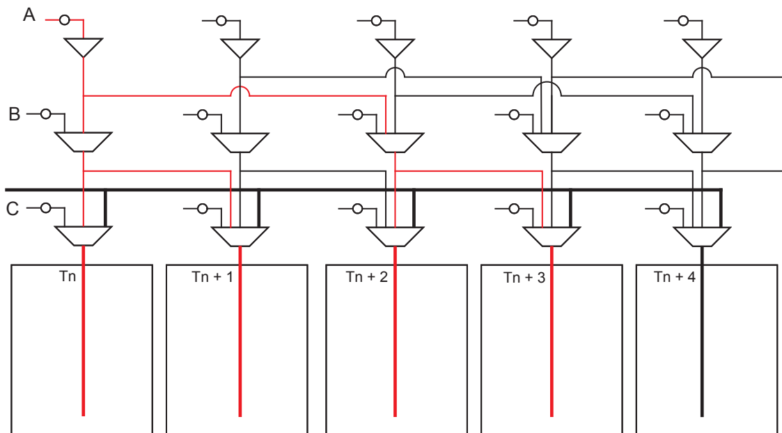
Figure 4-10 • Four Spines Aggregation
