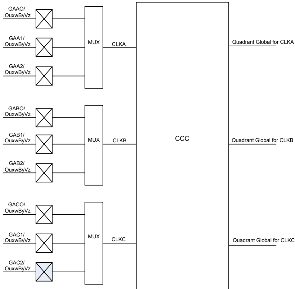
Figure 4-6 • Global Inputs
