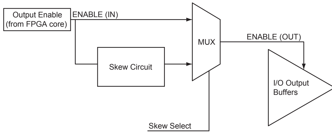
Figure 6-13 • Block Diagram of Output Enable Path
