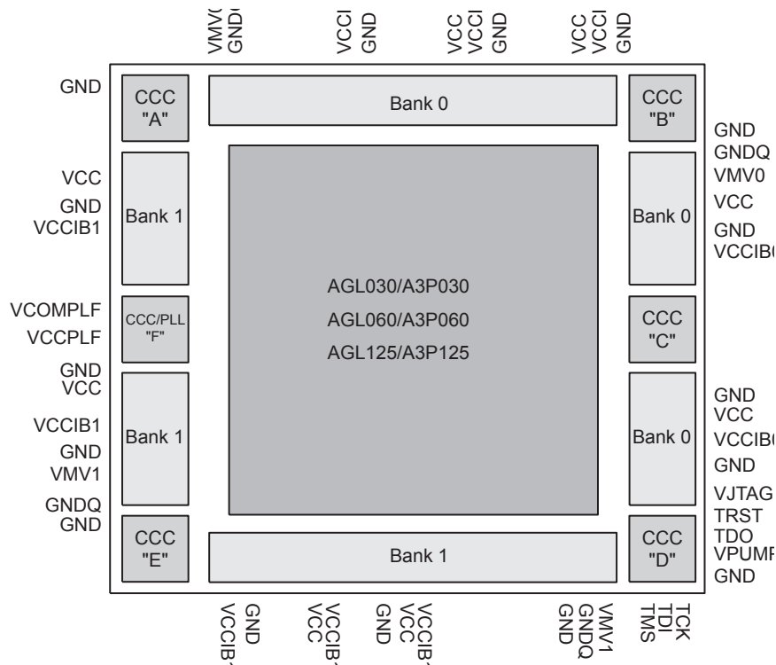
Figure 6-19 • Naming Conventions of IGLOO and ProASIC3 Devices with Two I/O Banks – Top View
