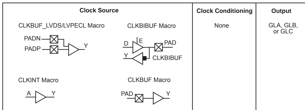
Figure 5-2 • CCC Options: Global Buffers with No Programmable Delay
