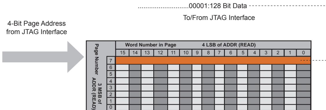
Figure 8-8 • Accessing FlashROM Using JTAG Port
