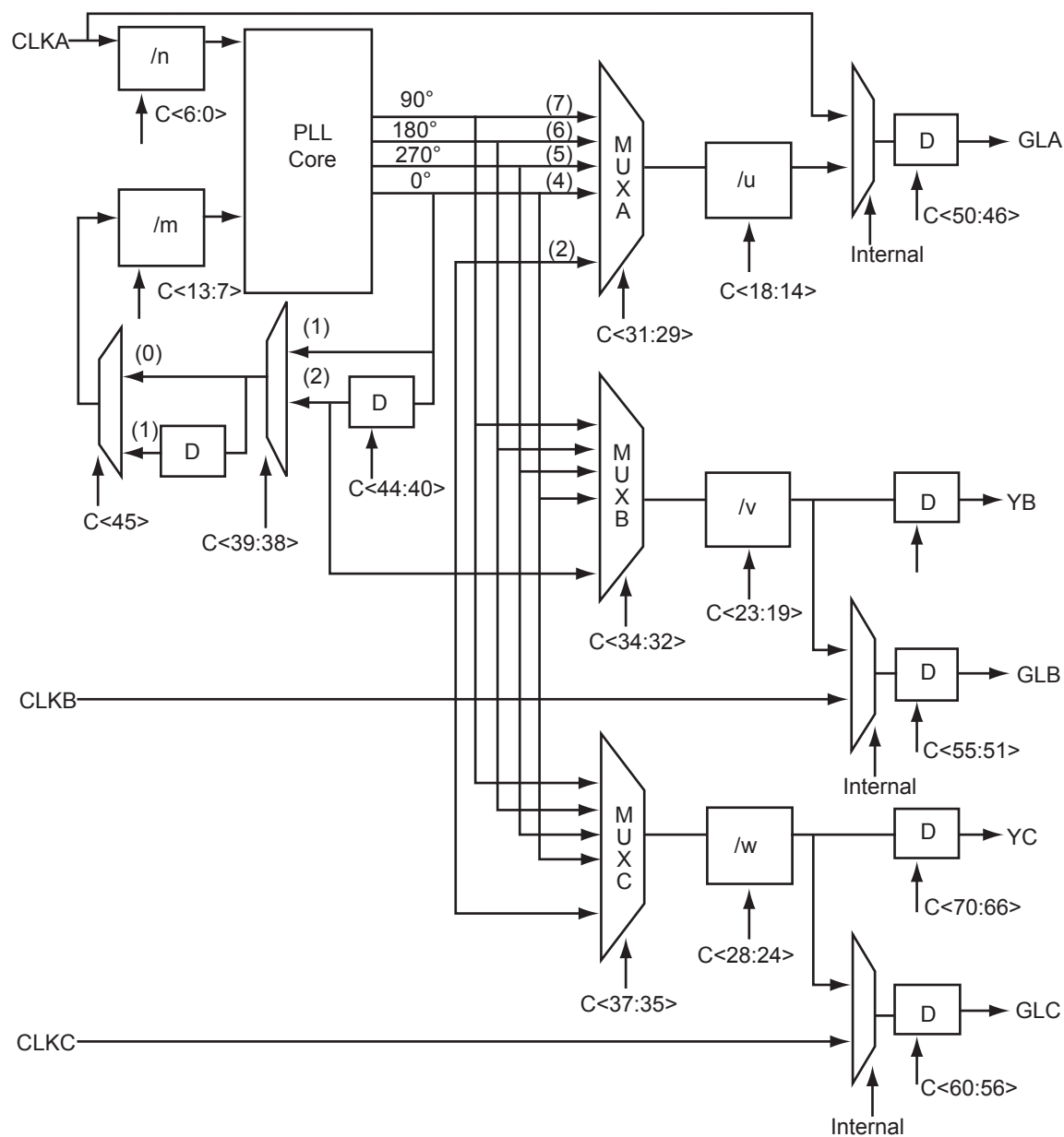
Figure 5-22 • CCC Block Control Bits – Graphical Representation of Assignments
