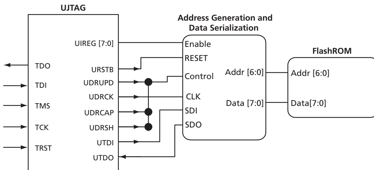
Figure 8-6 • Block Diagram of Using UJTAG to Read FlashROM Contents
