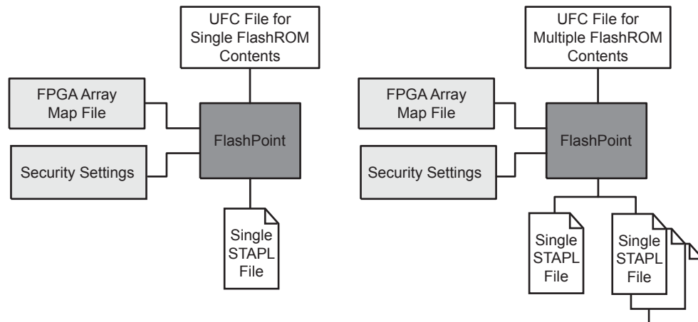
Figure 8-11 • Single or Multiple Programming File Generation
