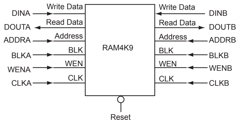
Figure 9-4 • RAM4K9 Simplified Configuration
