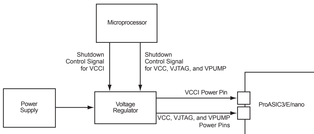
Figure 3-7 • Controlling Power On/Off State Using Microprocessor and Voltage Regulator
