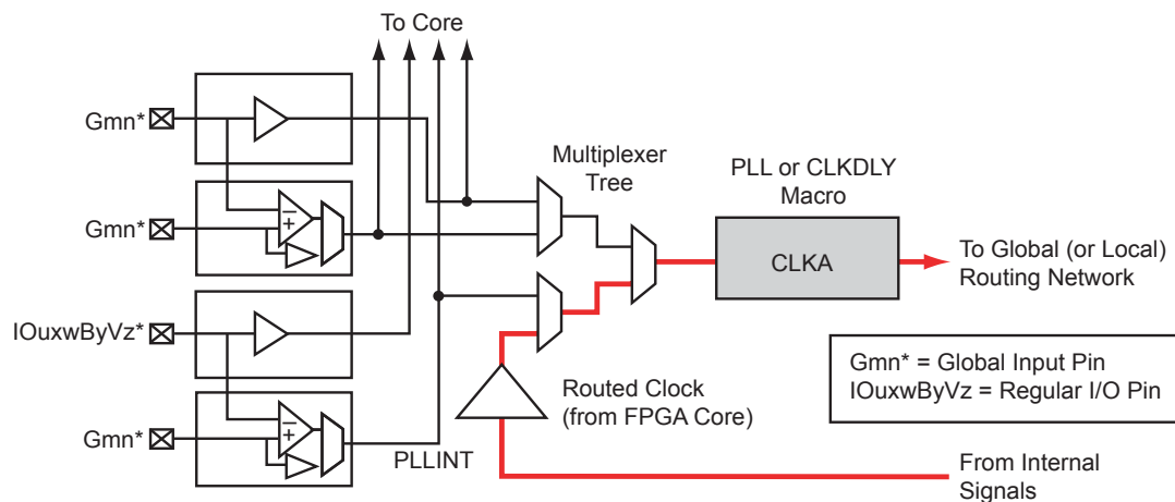
Figure 5-12 • Illustration of Core Logic Usage
