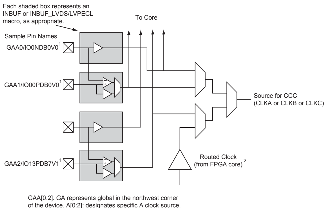
Figure 4-5 • Global I/O Overview
