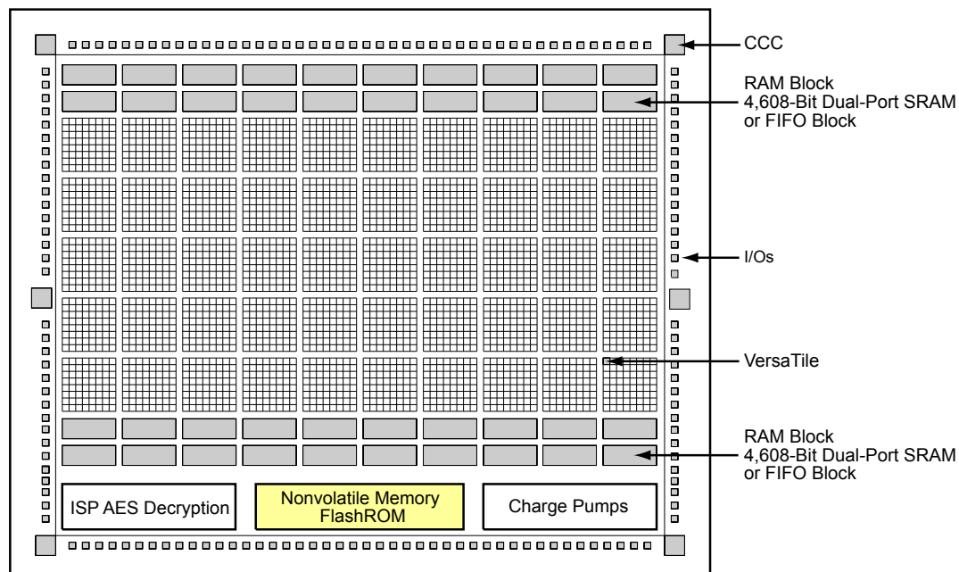
Figure 8-3 • ProASIC3 and IGLOO Device Architecture
