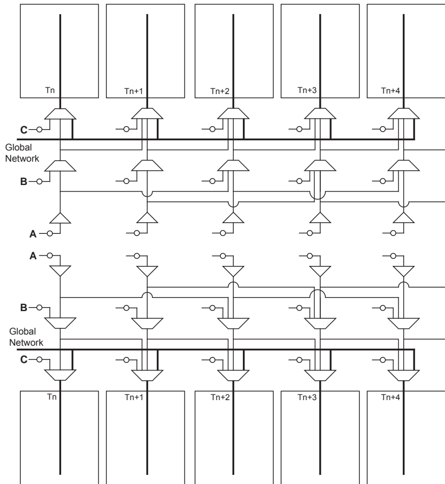
Figure 4-7 • Chip Global Aggregation
