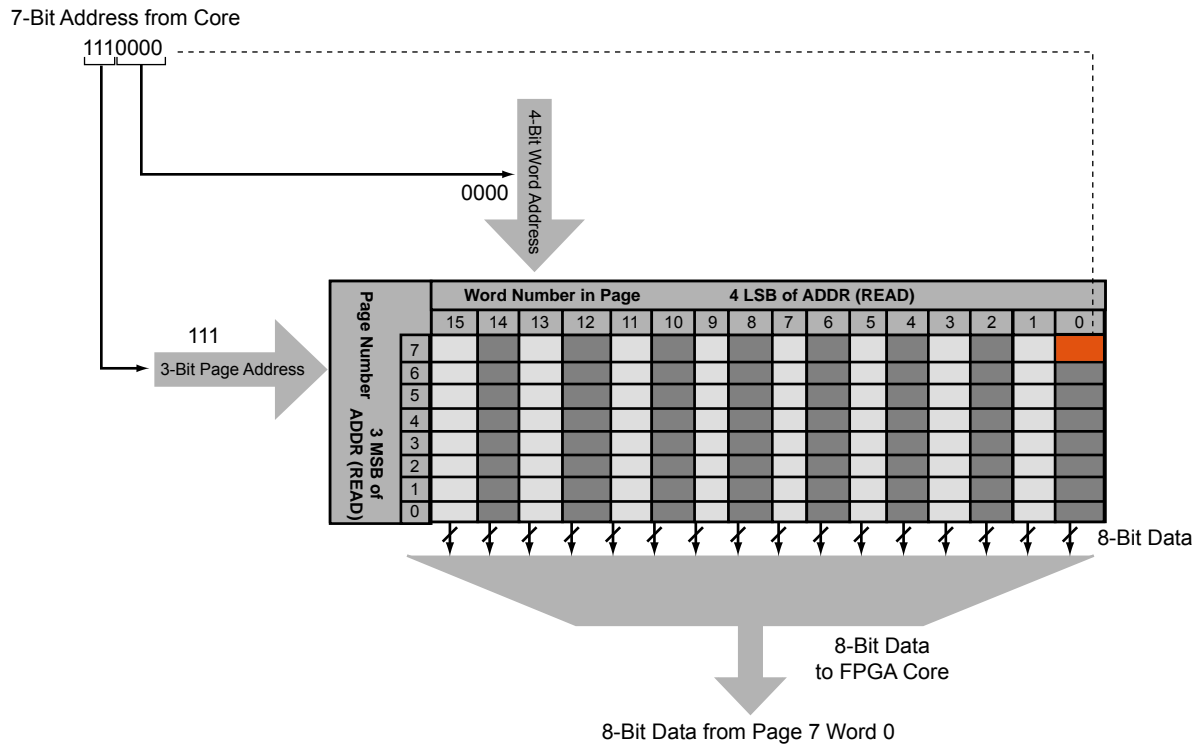
Figure 8-7 • Accessing FlashROM Using FPGA Core
