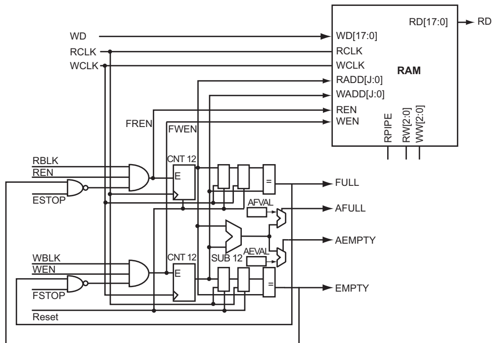
Figure 9-7 • RAM Block with Embedded FIFO Controller
