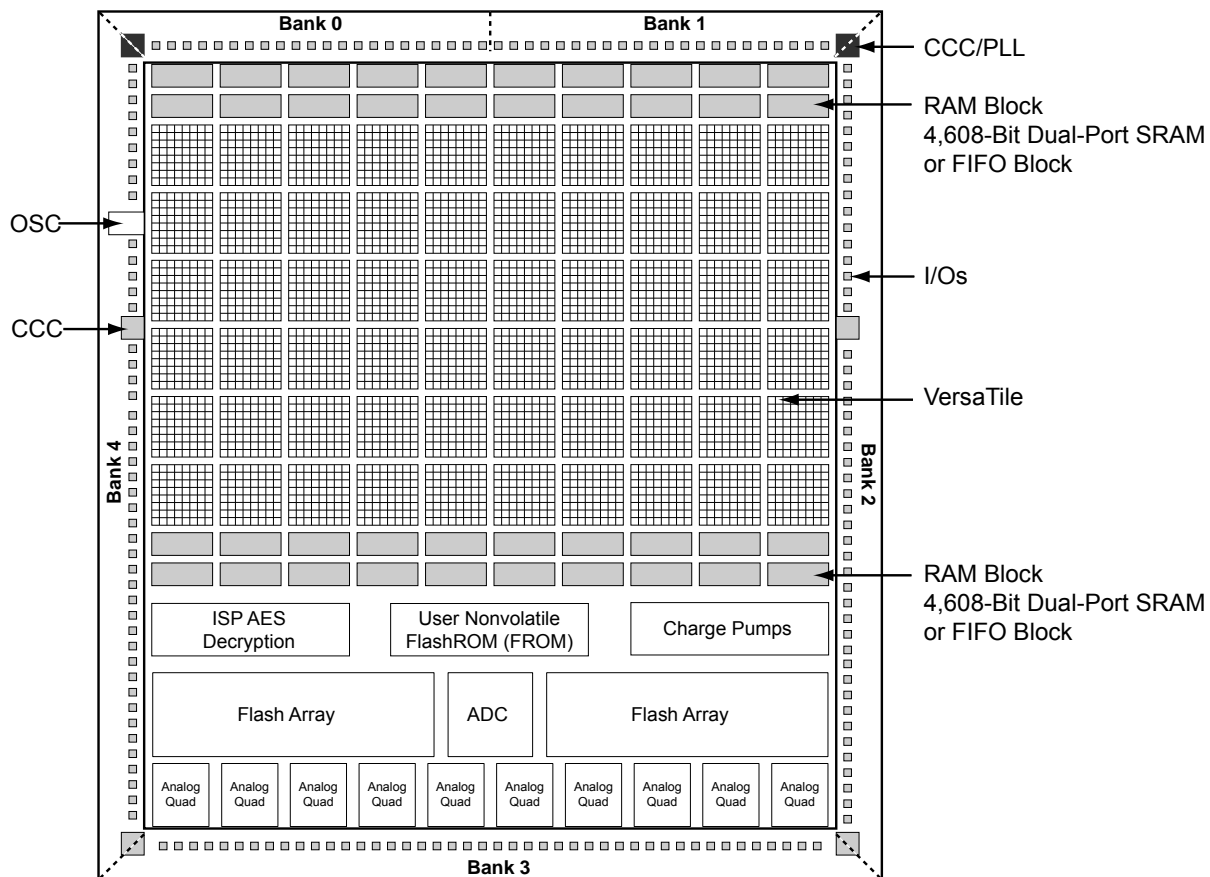
Figure 9-2 • Fusion Device Architecture Overview (AFS600)
