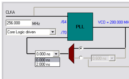
Figure 5-24 • Internal Feedback with Selectable System Delay
