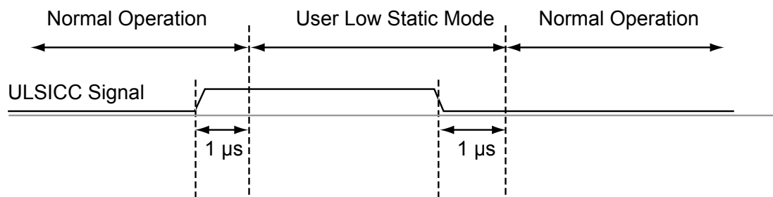
Figure 3-4 • User Low Static (Idle) Mode Timing Diagram
