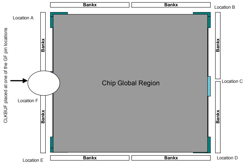
Figure 4-12 • Chip Global Region
