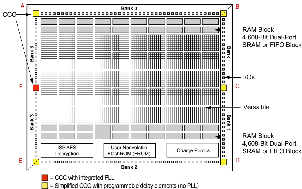
Figure 5-14 • CCC Locations in IGLOO and ProASIC3 Family Devices (except 10 k through 30 k gate devices)
