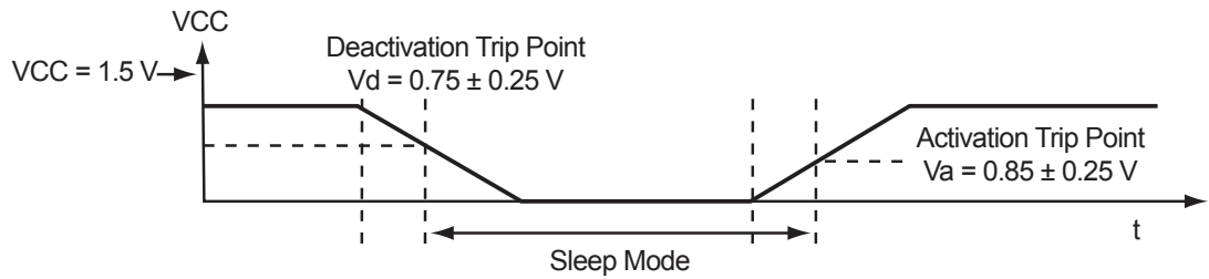
Figure 3-5 • Entering and Exiting Sleep Mode—Typical Timing Diagram
