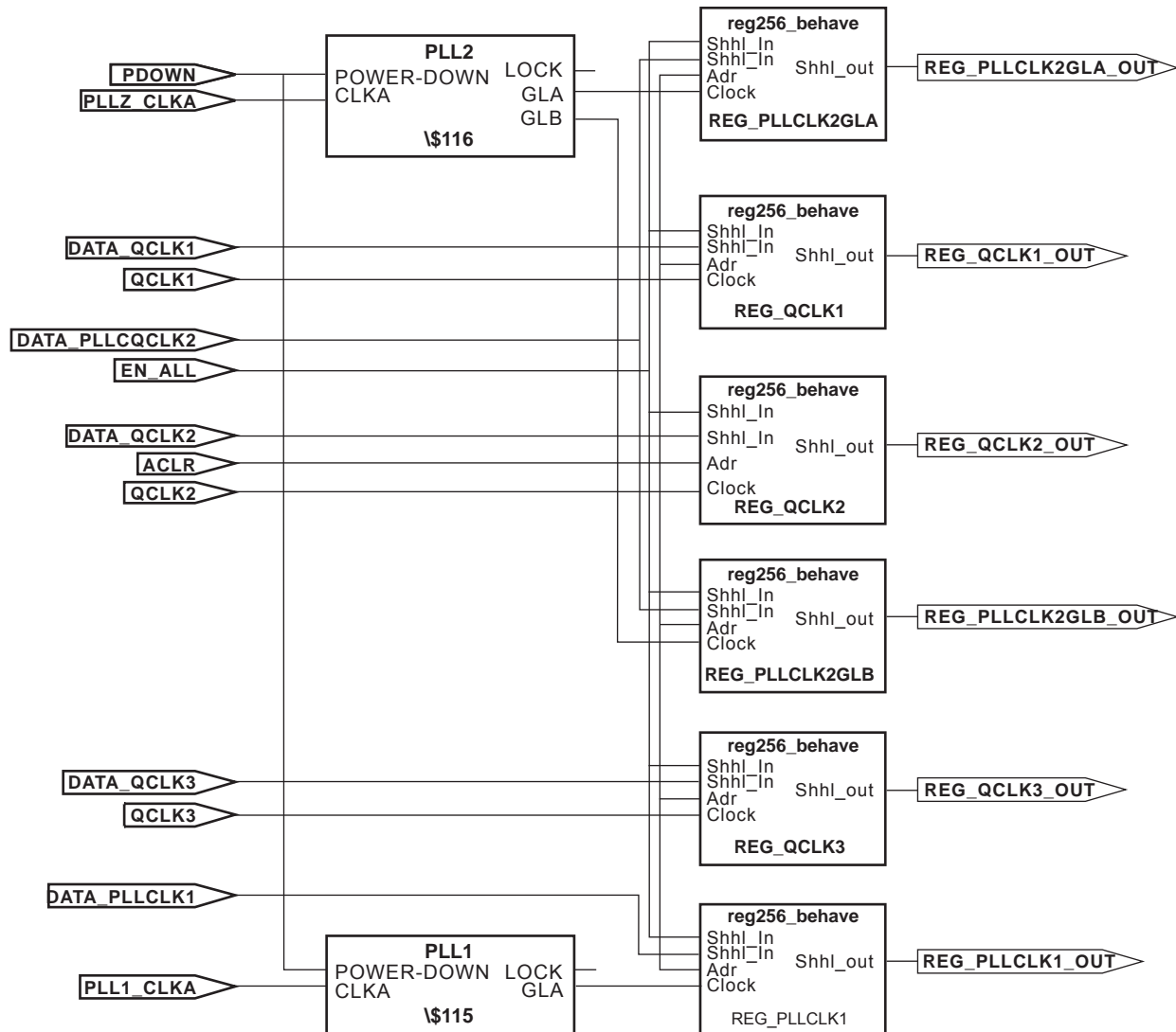
Figure 4-19 • Block Diagram of the Global Management Example Design
