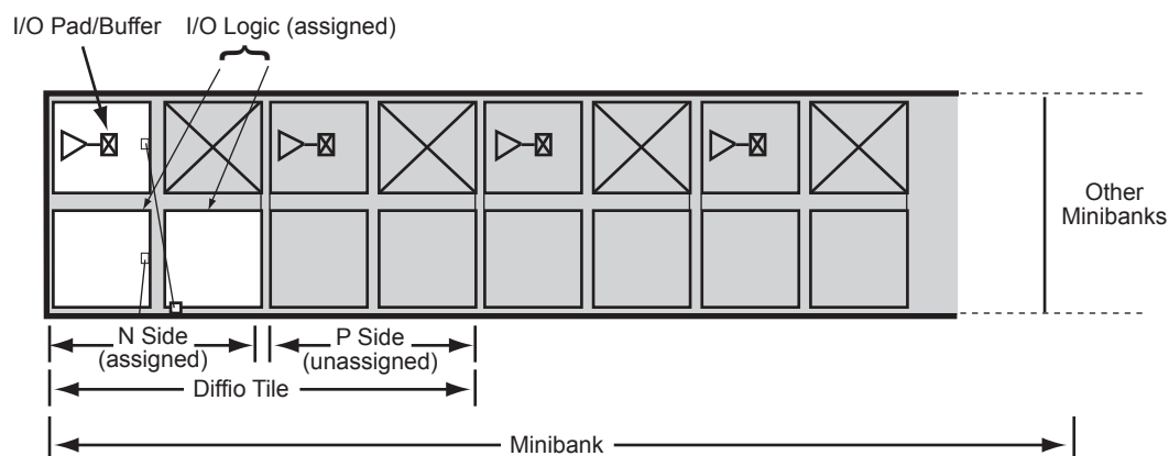
Figure 6-3 • Snapshot of an I/O Tile
