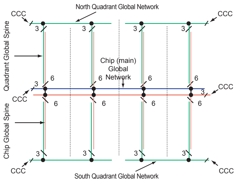
Figure 4-3 • Simplified VersaNet Global Network (60 k gates and above)
