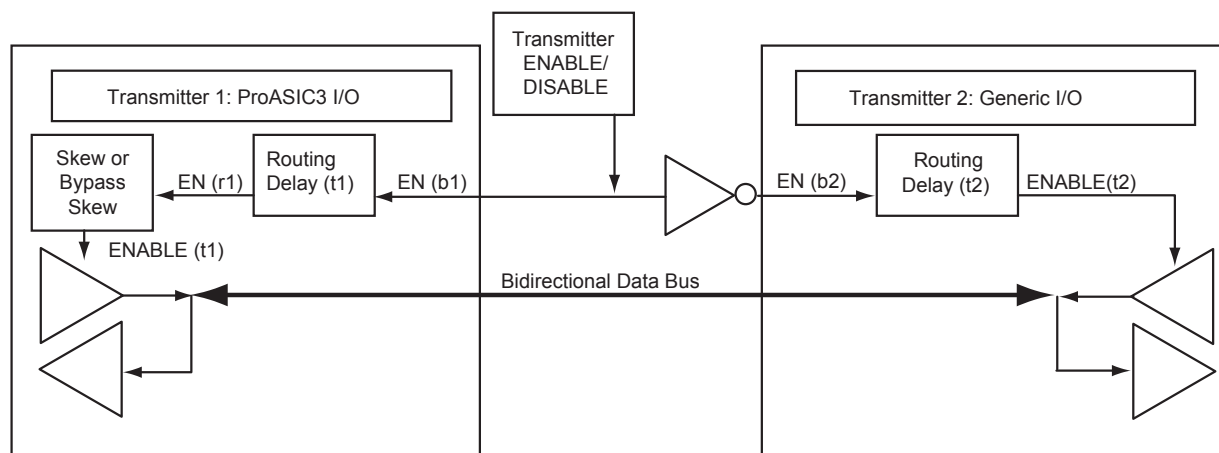
Figure 6-16 • Example of Implementation of Skew Circuits in Bidirectional Transmission Systems Using IGLOO or ProASIC3 Devices
