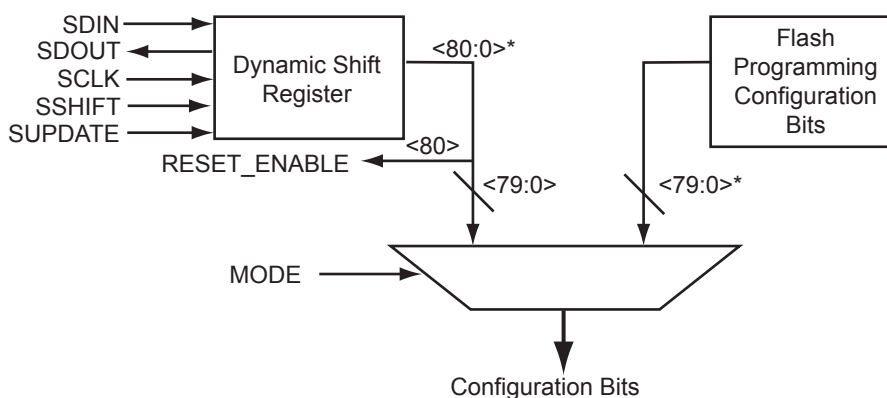
Figure 5-21 • The CCC Configuration MUX Architecture
