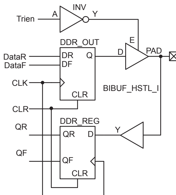
Figure 11-8 • DDR Bidirectional Buffer, LOW Output Enable (HSTL Class II)
