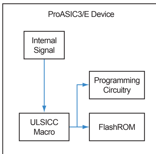
Figure 3-2 • User Low Static (Idle) Mode Application—Internal Control Signal
