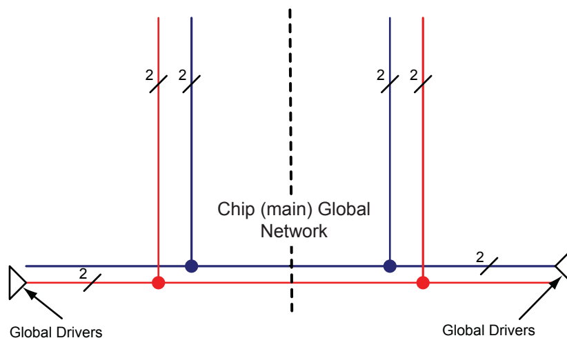
Figure 4-2 • Simplified VersaNet Global Network (30 k gates and below)
