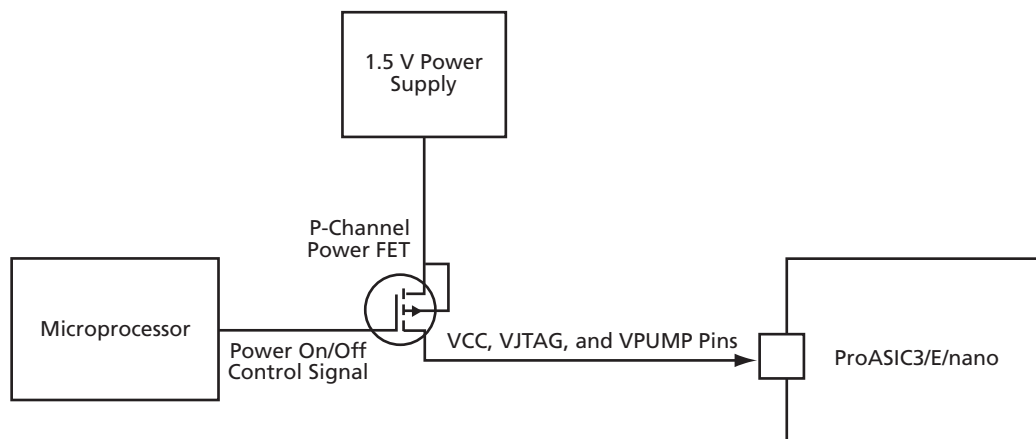
Figure 3-6 • Controlling Power On/Off State Using Microprocessor and Power FET
