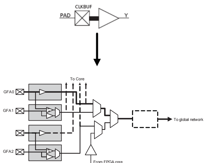
Figure 4-11 • CLKBUF Macro
