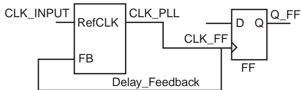
Figure 6 • Feedback from Worst Skew Point to the PLL
