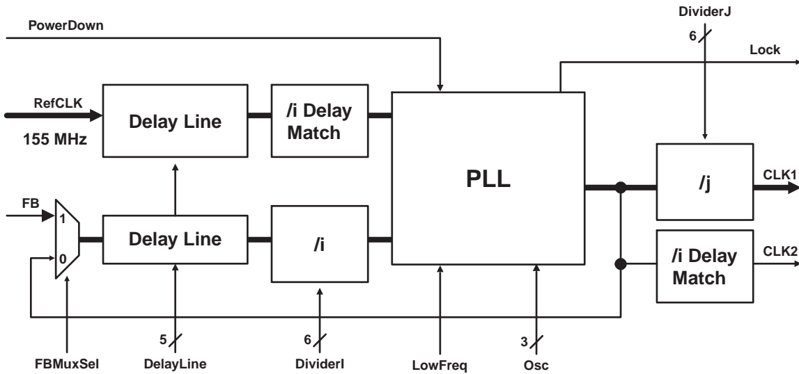
Figure 2 • Basic PLL Architecture in Axcelerator Devices
