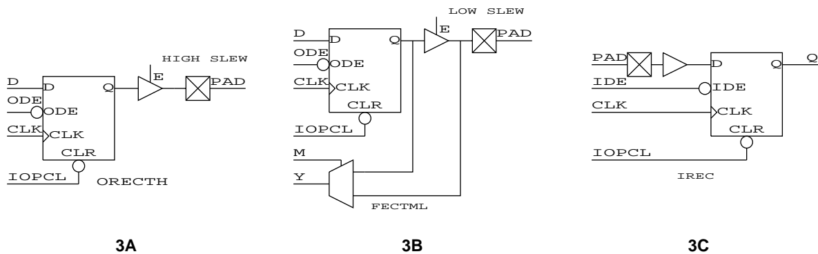
Figure 3 • I/O Macro Implementations
